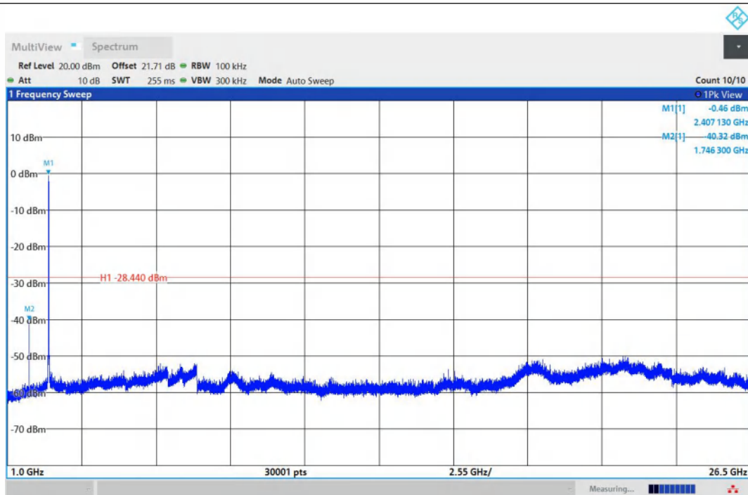
11N20SISO-Ant1-2412-1000~26500-PASS
