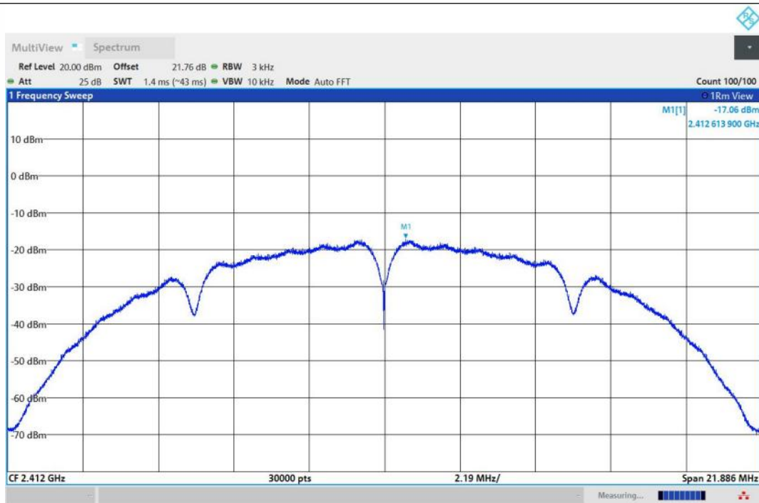
11B-Ant1-2412-PASS
