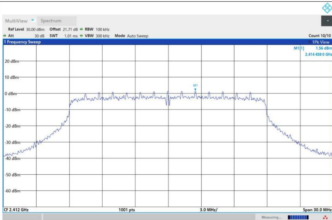
11N20SISO-Ant1-2412-0~Reference-PASS
