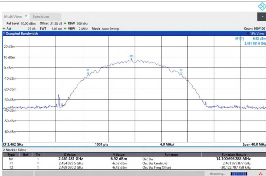
11B-Ant1-2462
