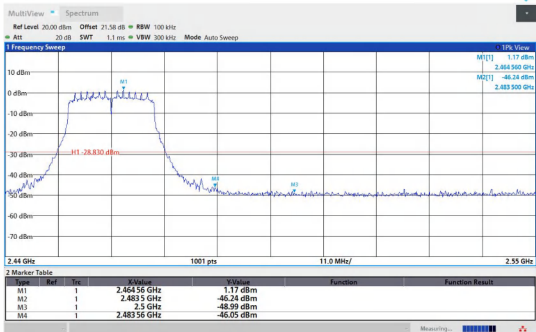
11N20SISO-Ant1-2462-PASS
