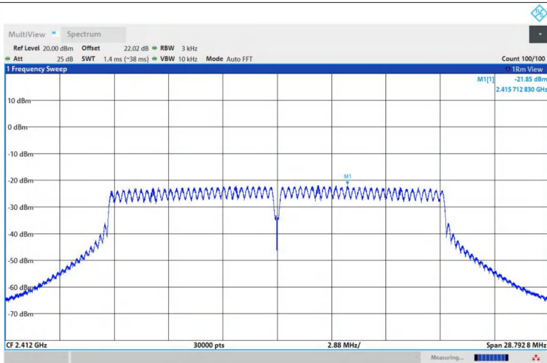
11N20SISO-Ant1-2412-PASS
