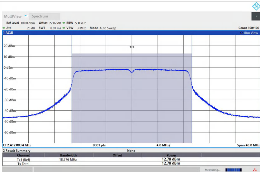
11N20SISO-Ant1-2412-PASS
