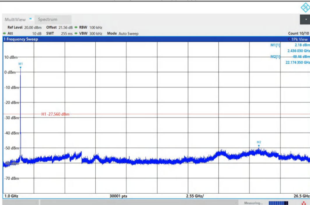
11N20SISO-Ant1-2437-1000~26500-PASS
