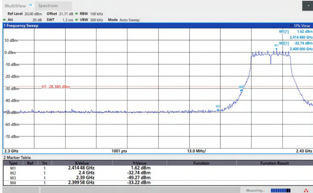
11G-Ant1-2412-PASS
