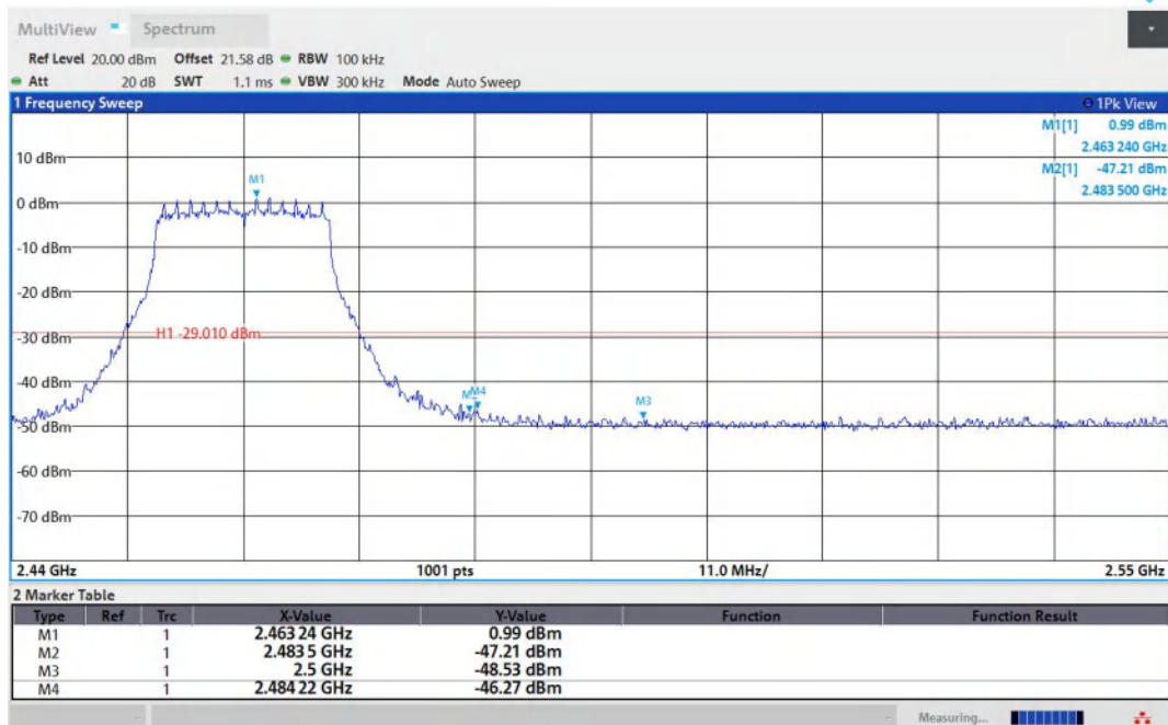
11G-Ant1-2462-PASS
