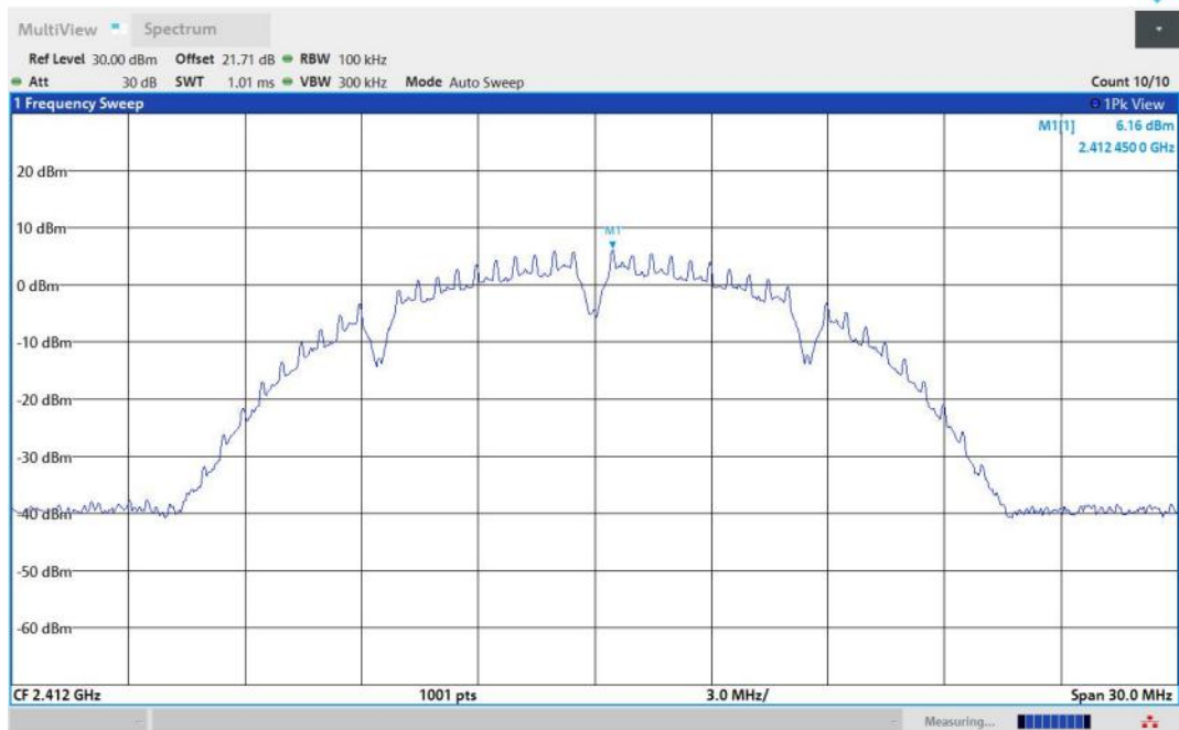
11B-Ant1-2412-0~Reference-PASS
