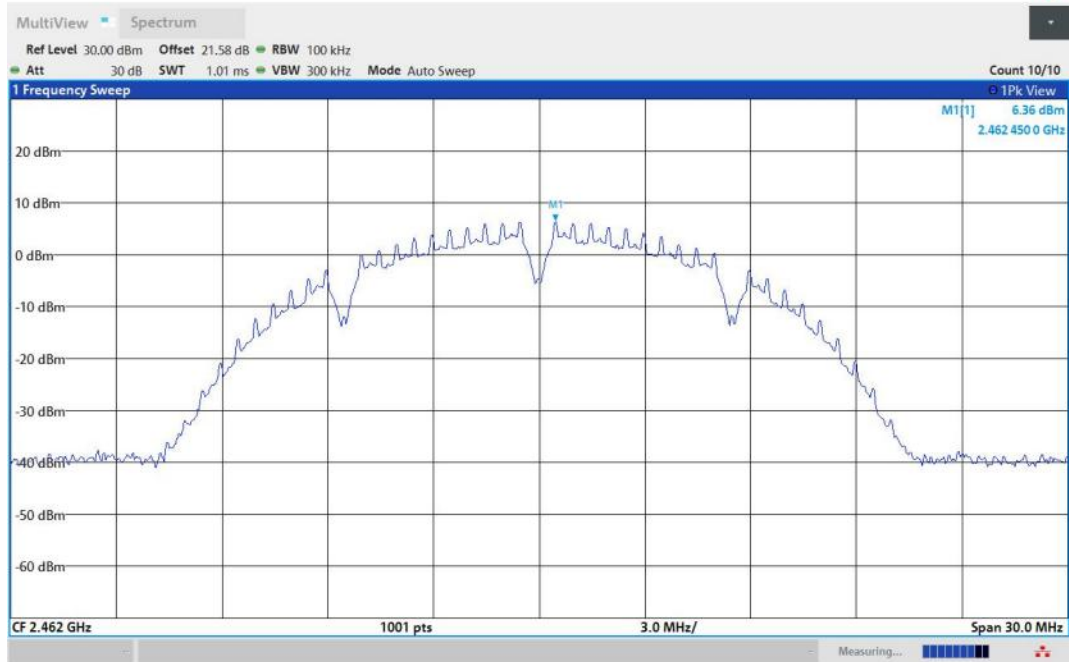
11B-Ant1-2462-0~Reference-PASS
