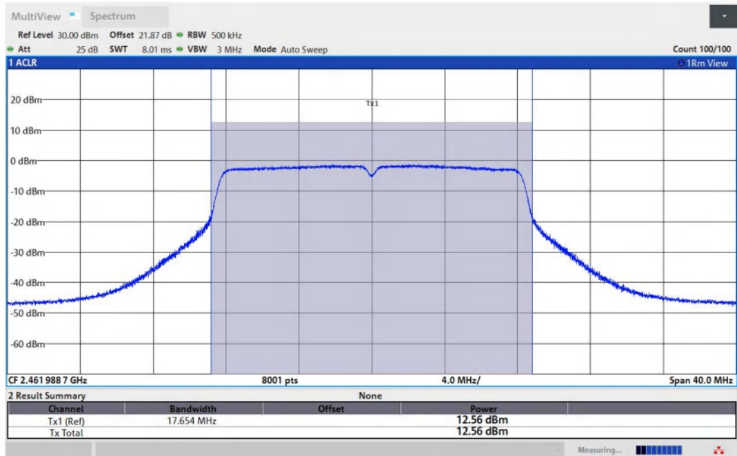
11G-Ant1-2462-PASS
