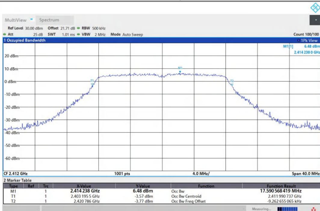
11G-Ant1-2412
