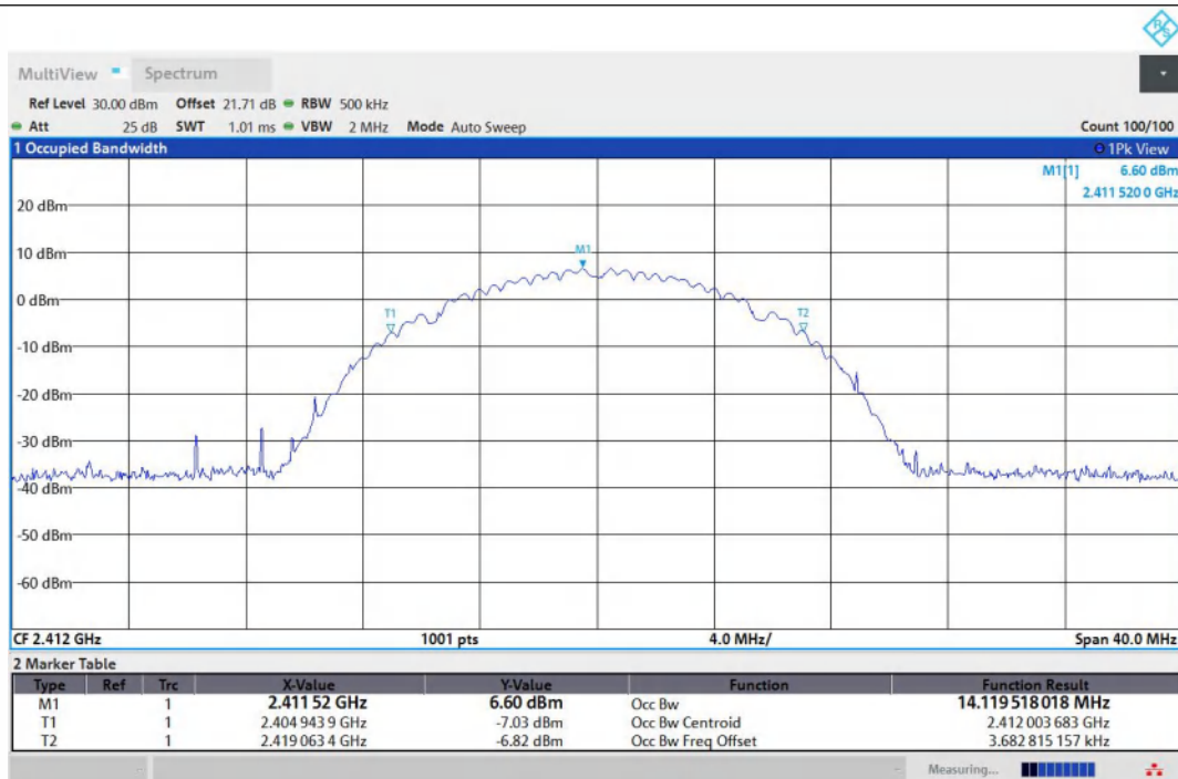
11B-Ant1-2412
