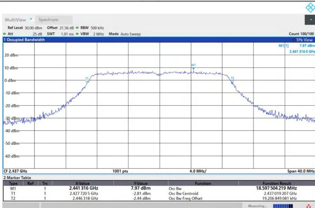
11N20SISO-Ant1-2437
