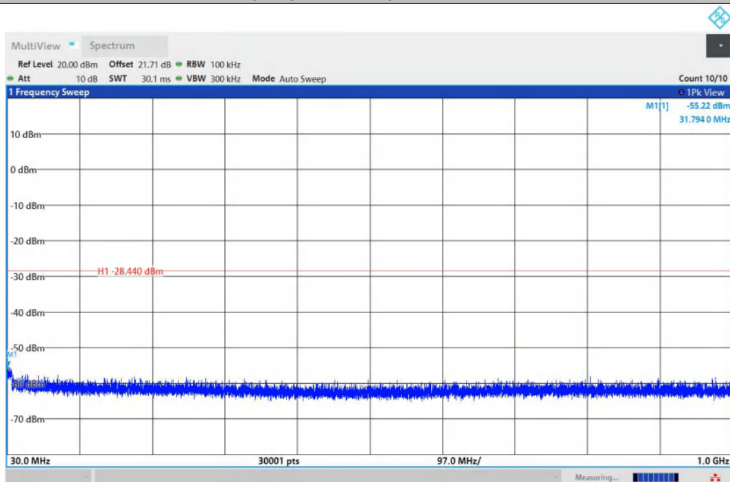
11N20SISO-Ant1-2412-30~1000-PASS
