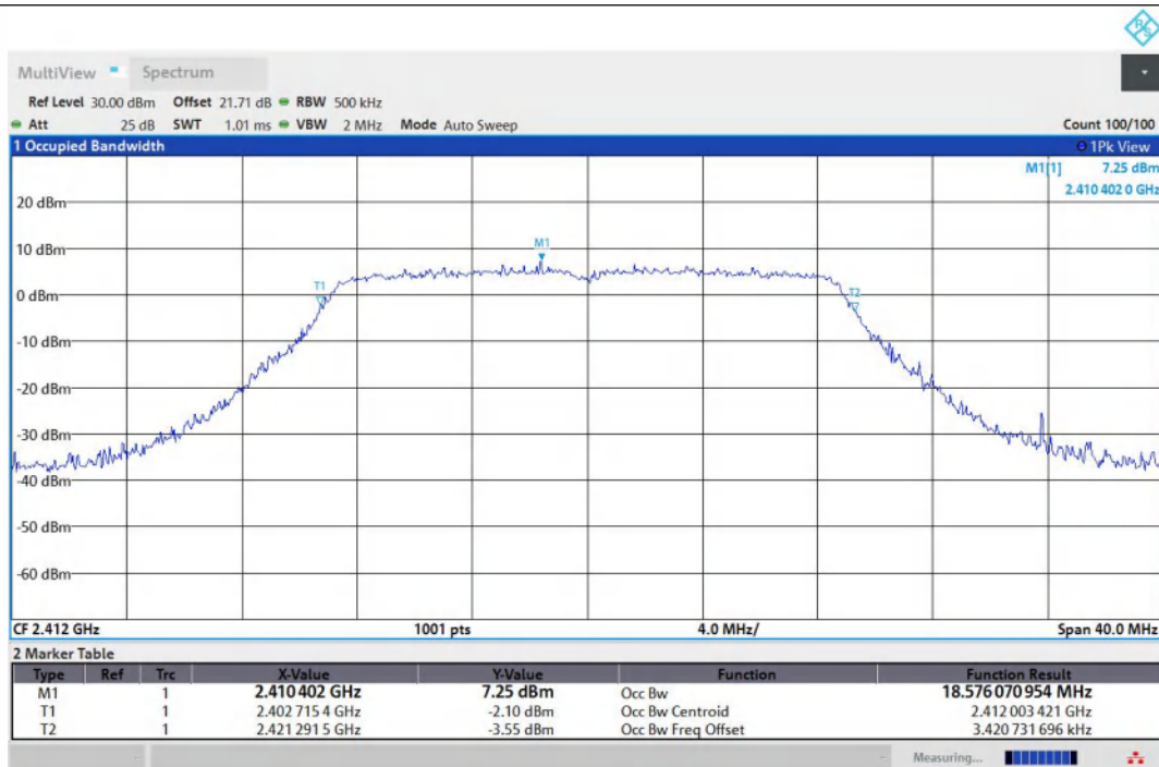
11N20SISO-Ant1-2412
