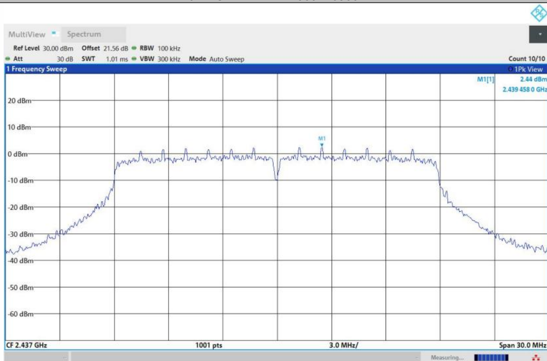
11N20SISO-Ant1-2437-0~Reference-PASS
