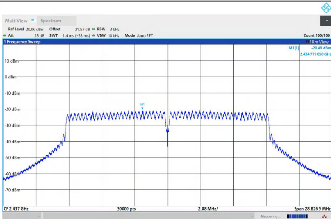
11N20SISO-Ant1-2437-PASS
