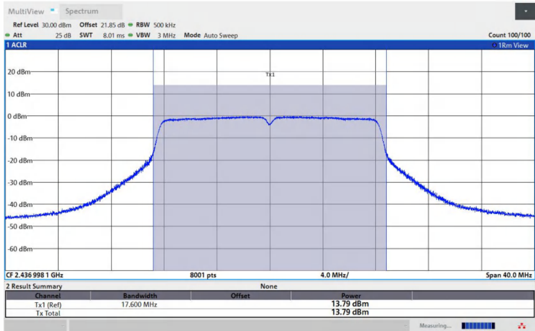
11G-Ant1-2437-PASS
