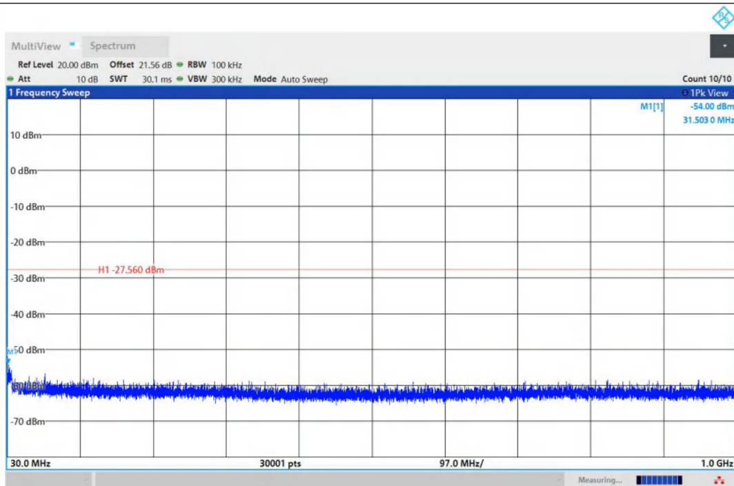
11N20SISO-Ant1-2437-30~1000-PASS
