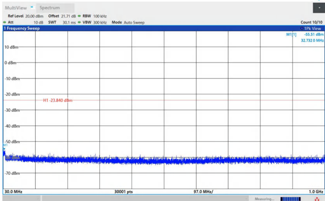
11B-Ant1-2412-30~1000-PASS
