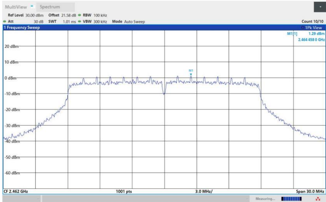
11N20SISO-Ant1-2462-0~Reference-PASS
