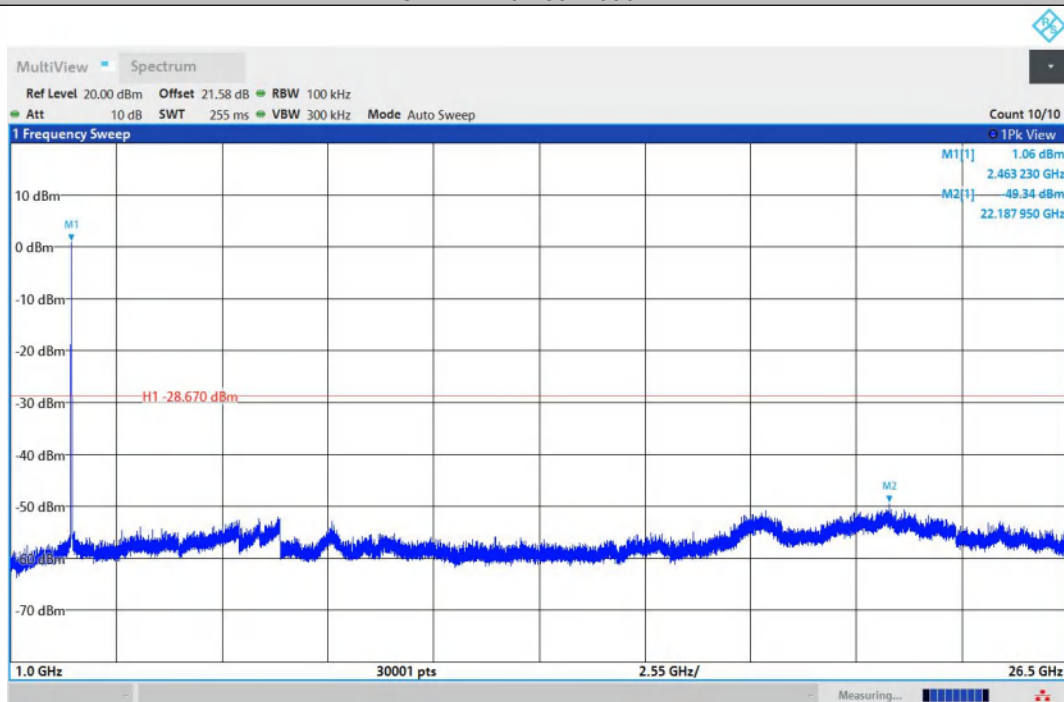
11G-Ant1-2462-1000~26500-PASS
