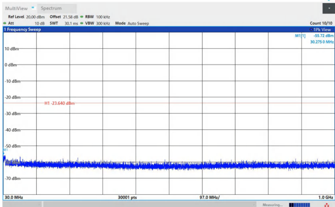
11B-Ant1-2462-30~1000-PASS
