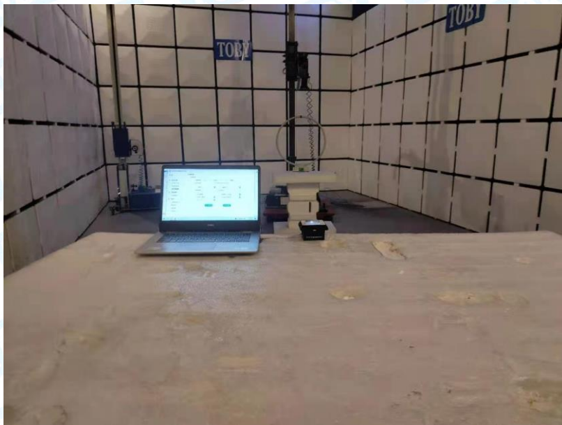
Photo of Setup for Radiated Emission (9KHz-30MHz)
