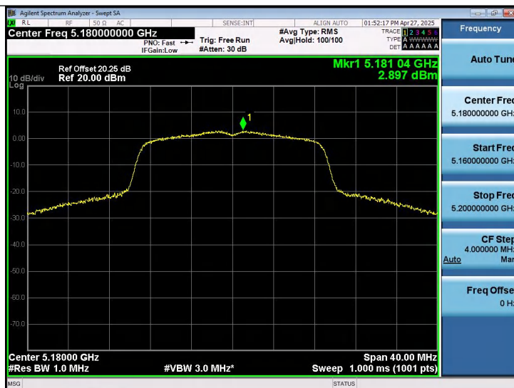
11N20SISO-Ant1-5180-PASS
