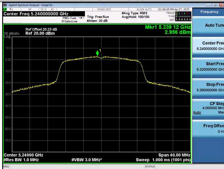
11N20SISO-Ant1-5240-PASS
