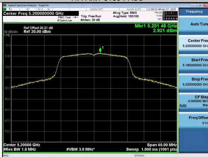
11A-Ant1-5200-PASS
