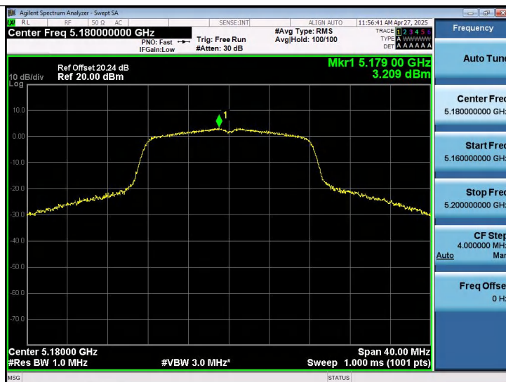
11A-Ant1-5180-PASS
