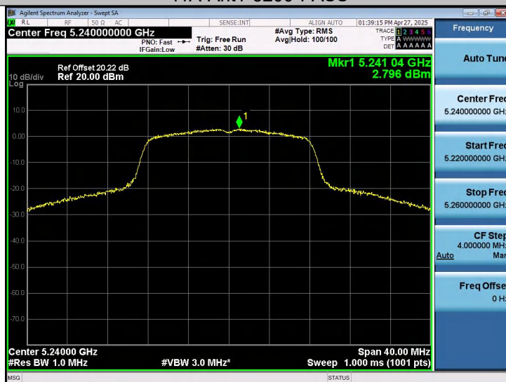
11A-Ant1-5240-PASS
