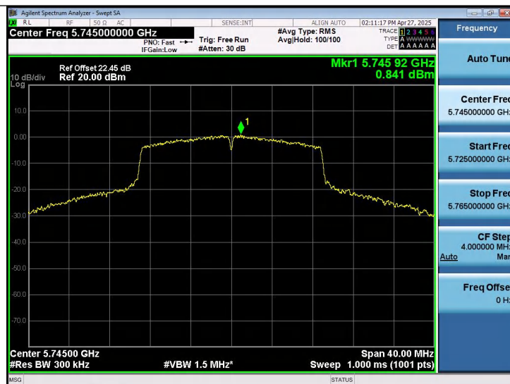
11N20SISO-Ant1-5745-PASS
