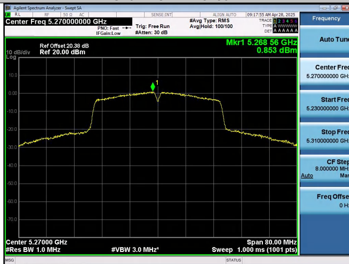
11AC40SISO-Ant1-5270-PASS
