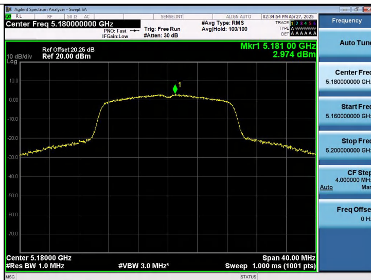
11AC20SISO-Ant1-5180-PASS
