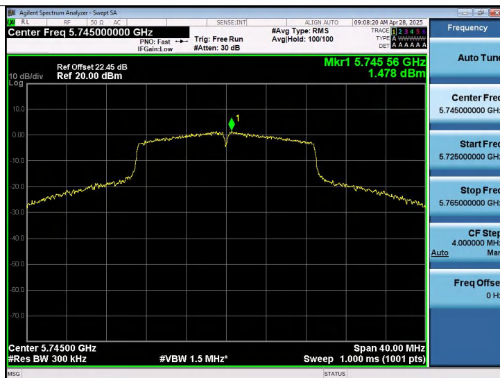
11AC20SISO-Ant1-5745-PASS
