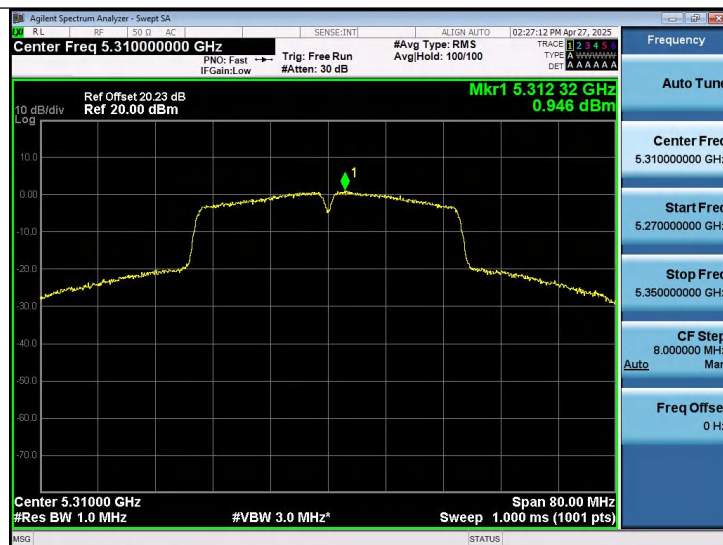
11N40SISO-Ant1-5310-PASS
