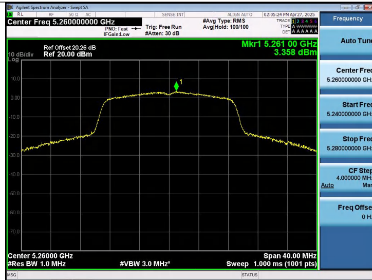
11N20SISO-Ant1-5260-PASS
