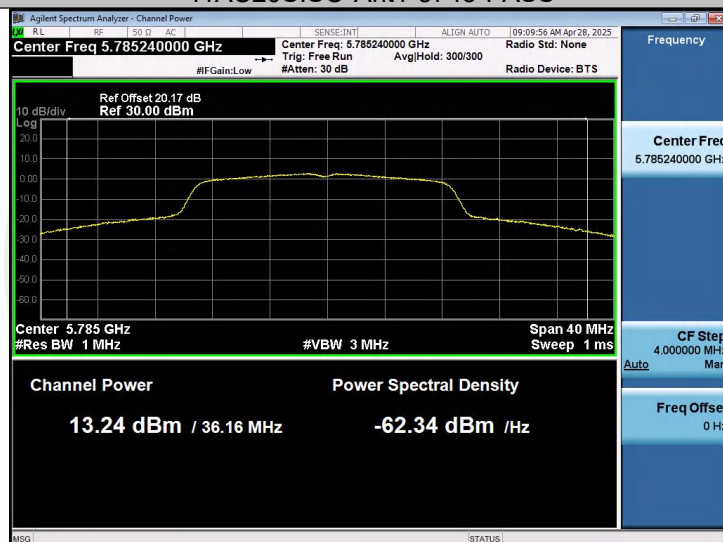
11AC20SISO-Ant1-5785-PASS
