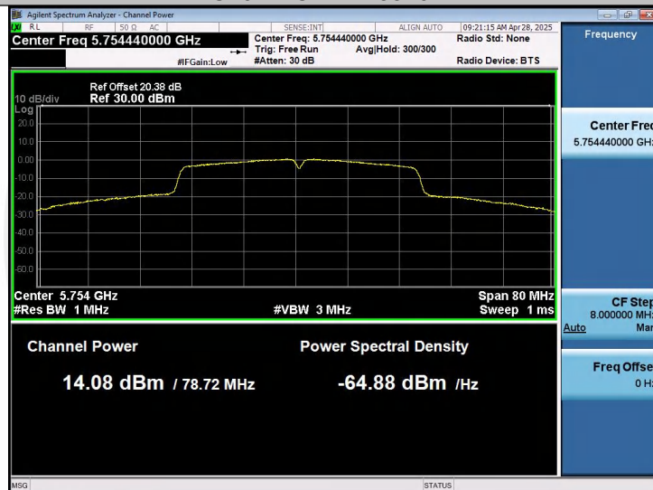
11AC40SISO-Ant1-5755-PASS
