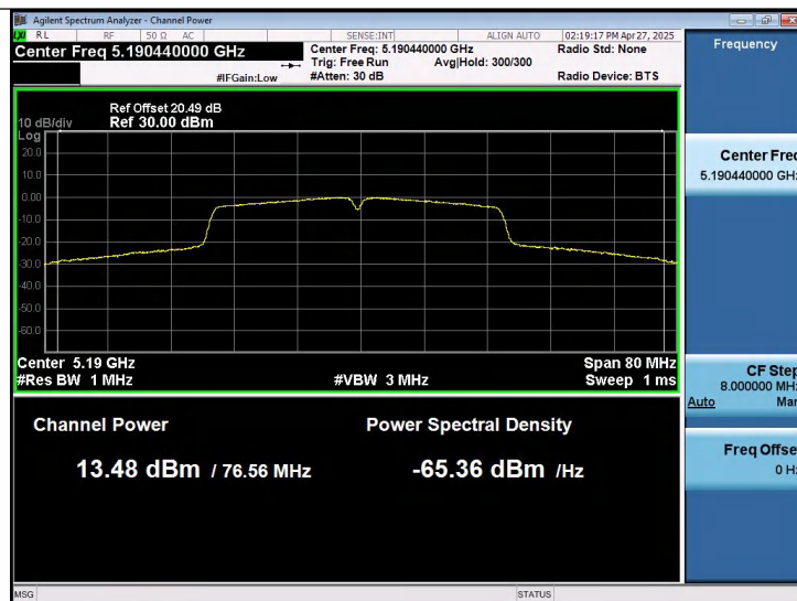
11N40SISO-Ant1-5190-PASS
