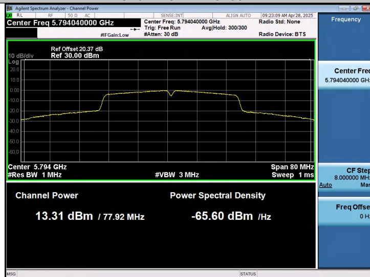
11AC40SISO-Ant1-5795-PASS
