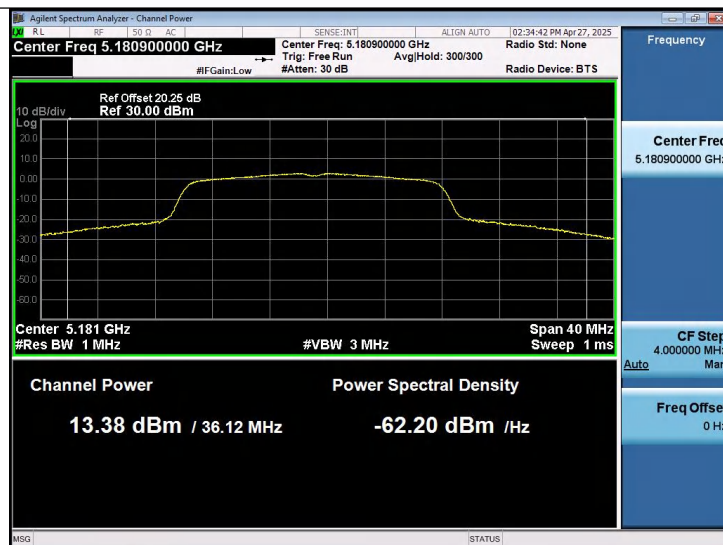
11AC20SISO-Ant1-5180-PASS
