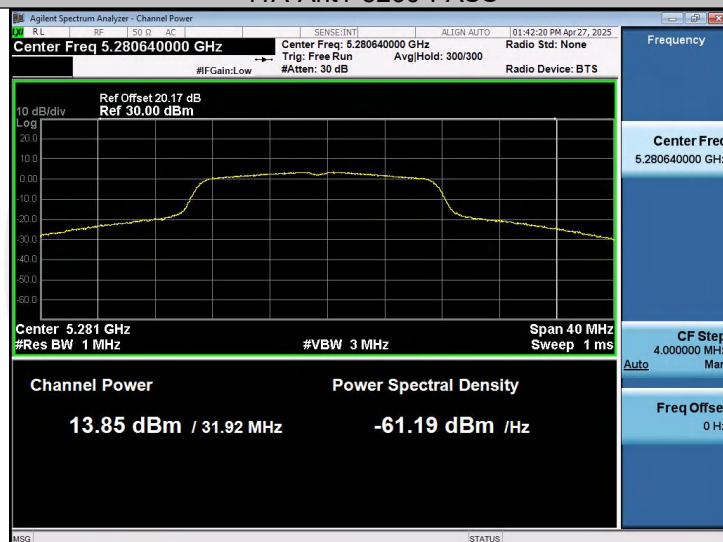
11A-Ant1-5280-PASS
