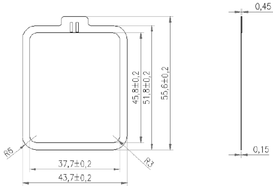
125KHz's antenna dimensions picture(Unit:mm)
