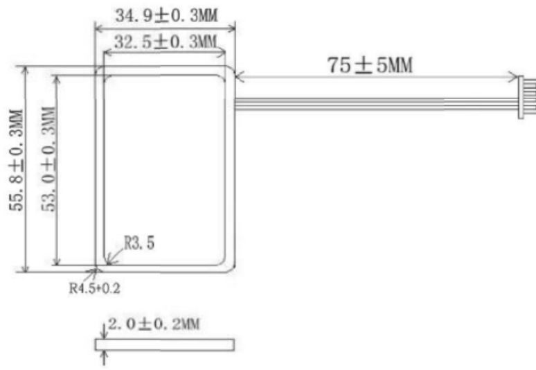
125KHz's antenna dimensions picture
