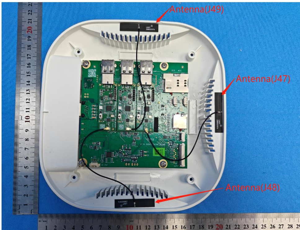
Antenna Location
