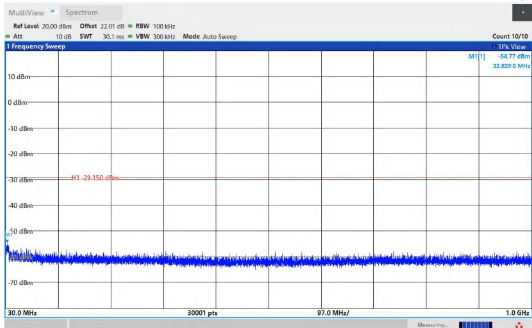
11B-Ant1-2412-30~1000-PASS
