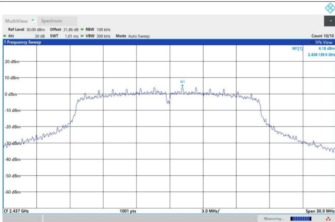
11G-Ant1-2437-0~Reference-PASS
