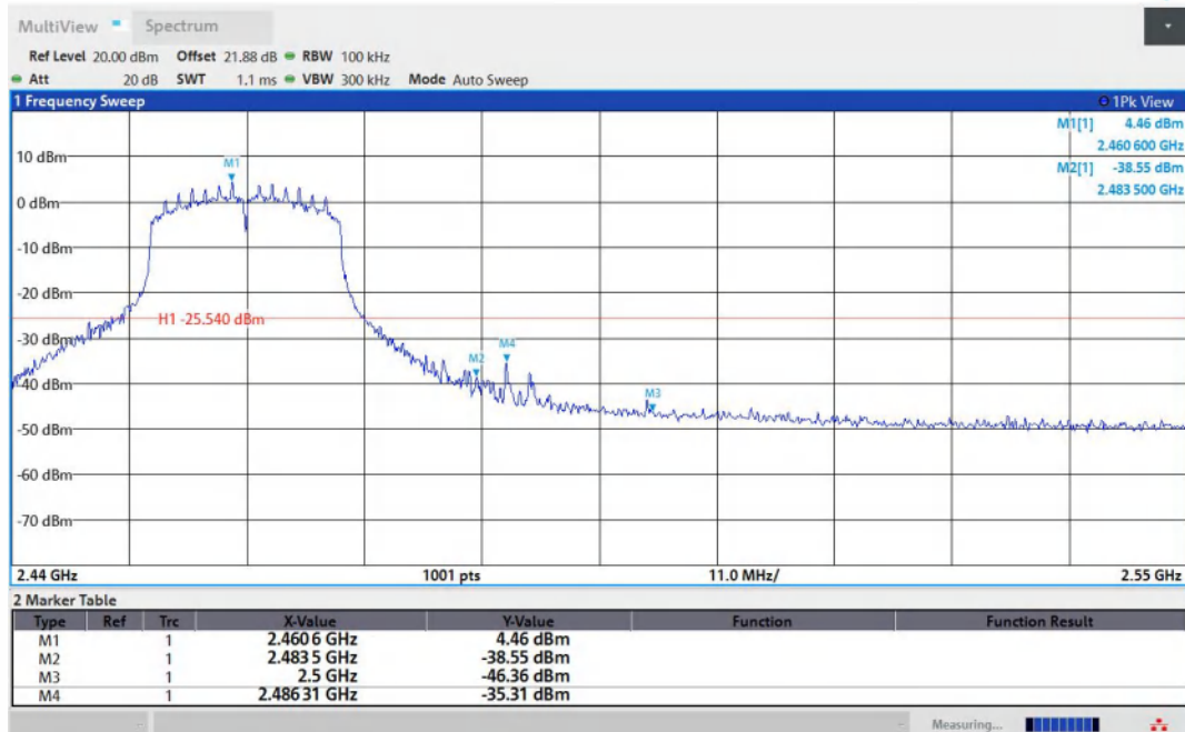
11N20SISO-Ant1-2462-PASS
