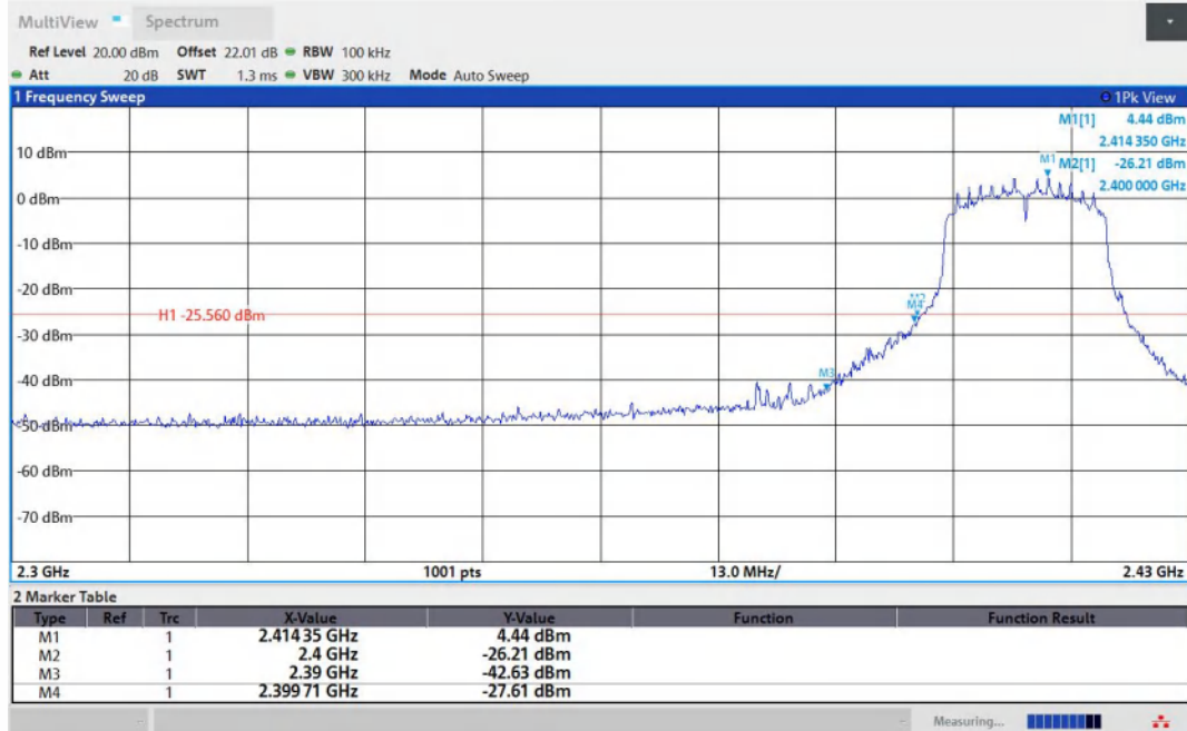
11N20SISO-Ant1-2412-PASS
