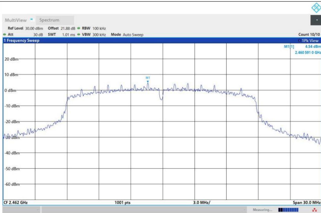
11N20SISO-Ant1-2462-0~Reference-PASS
