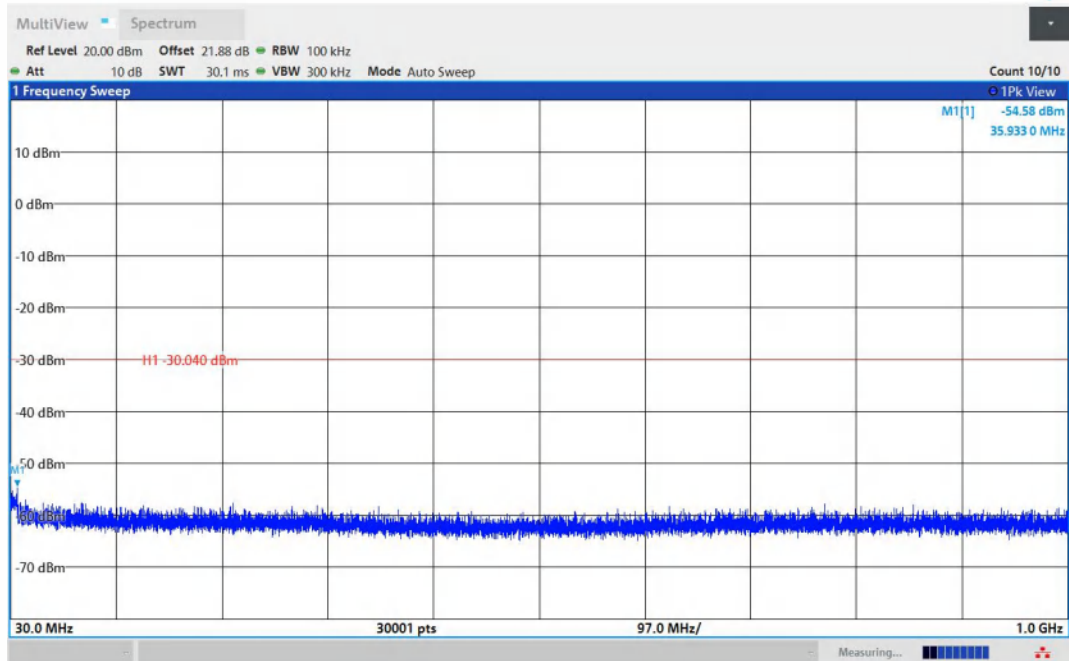
11B-Ant1-2462-30~1000-PASS
