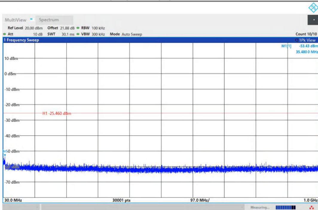
11N20SISO-Ant1-2462-30~1000-PASS
