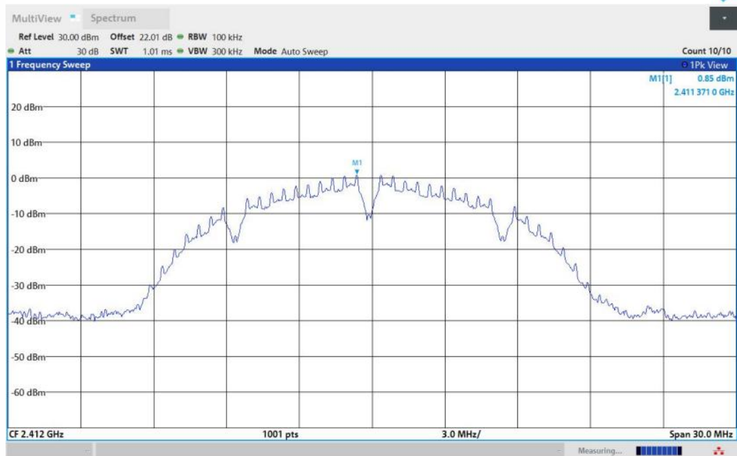
11B-Ant1-2412-0~Reference-PASS
