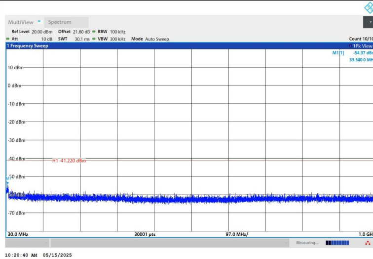
11N40SISO-Ant1-2422-30~1000-PASS
