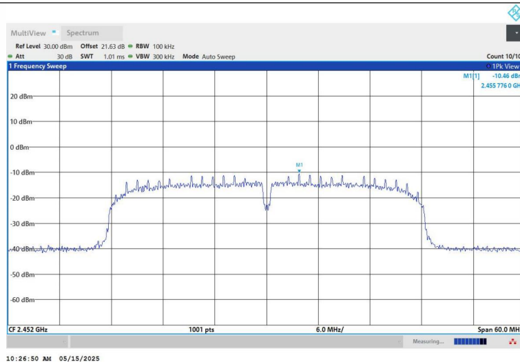
11N40SISO-Ant1-2452-0~Reference-PASS
