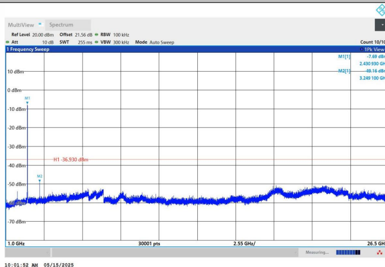
11G-Ant1-2437-1000~26500-PASS
