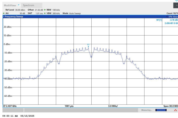
11B-Ant1-2437-0~Reference-PASS
