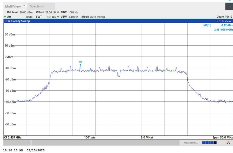
11N20SISO-Ant1-2437-0~Reference-PASS
