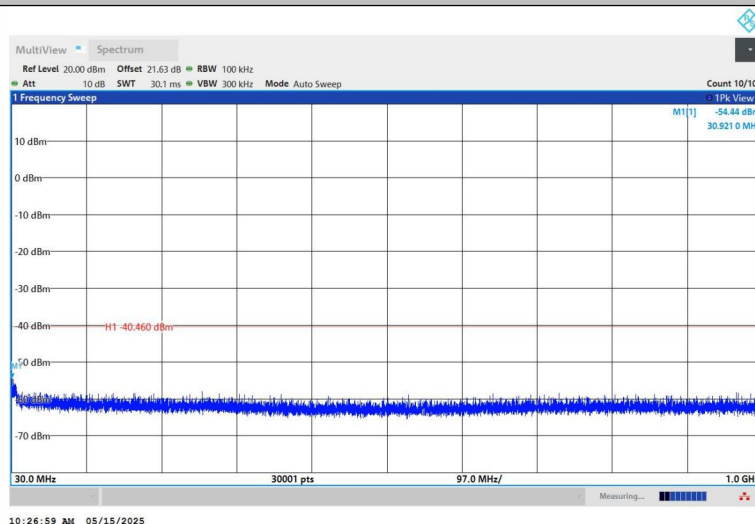
11N40SISO-Ant1-2452-30~1000-PASS
