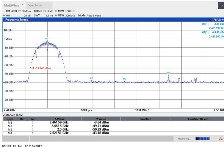
11B-Ant1-2462-PASS
