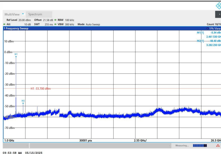
11B-Ant1-2462-1000~26500-PASS
