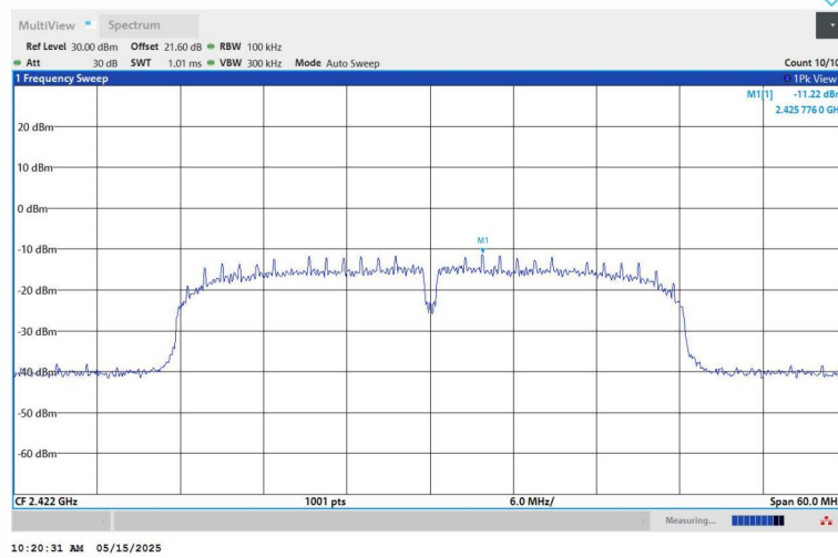
11N40SISO-Ant1-2422-0~Reference-PASS
