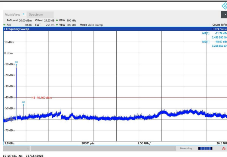
11N40SISO-Ant1-2452-1000~26500-PASS
