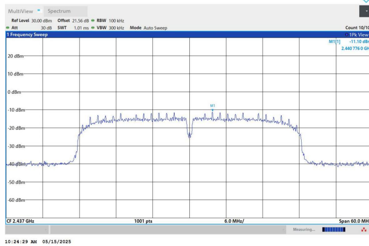
11N40SISO-Ant1-2437-0~Reference-PASS
