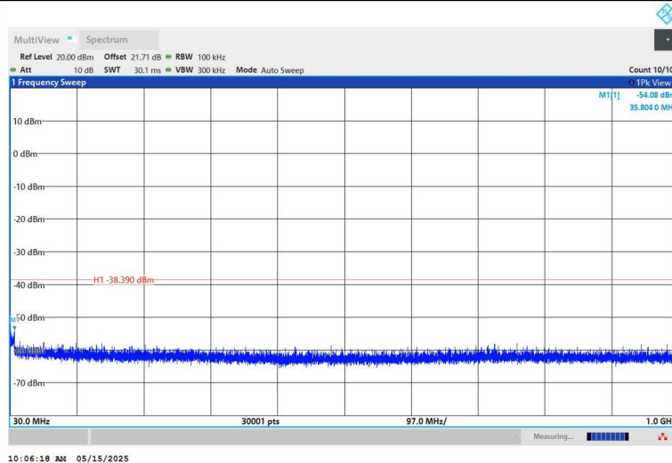
11N20SISO-Ant1-2412-30~1000-PASS
