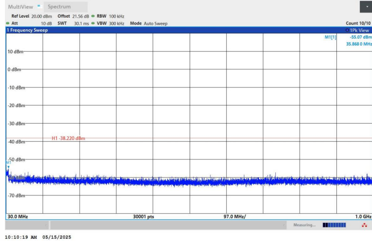
11N20SISO-Ant1-2437-30~1000-PASS
