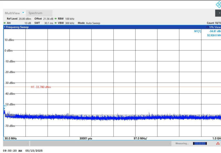
11B-Ant1-2437-30~1000-PASS
