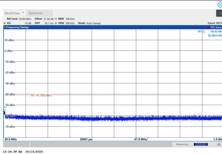
11N40SISO-Ant1-2437-30~1000-PASS
