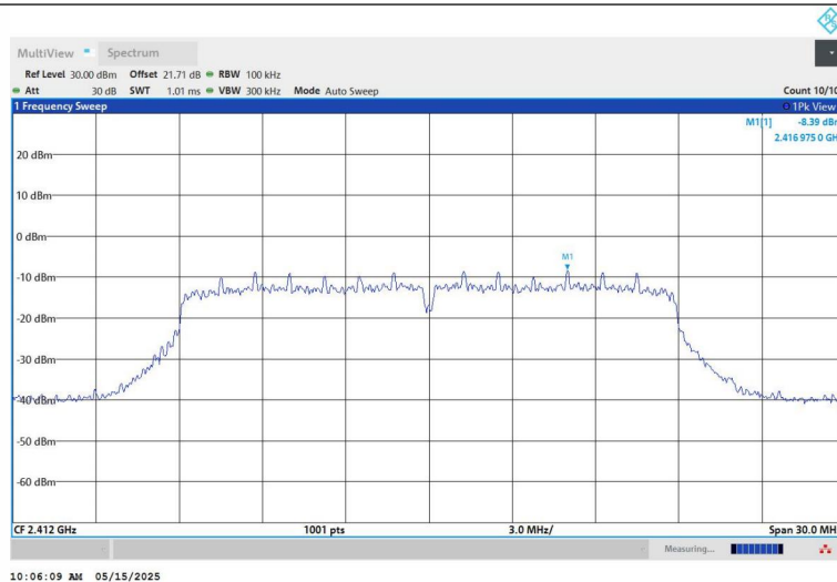
11N20SISO-Ant1-2412-0~Reference-PASS
