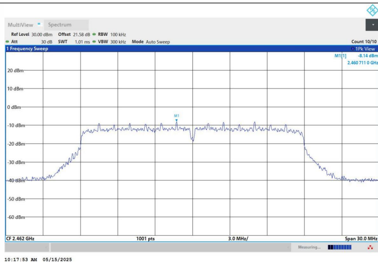
11N20SISO-Ant1-2462-0~Reference-PASS
