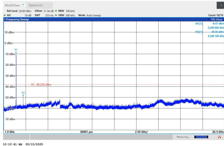
11N20SISO-Ant1-2437-1000~26500-PASS
