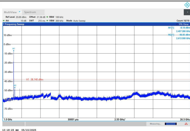
11N20SISO-Ant1-2462-1000~26500-PASS
