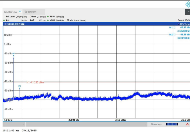
11N40SISO-Ant1-2422-1000~26500-PASS
