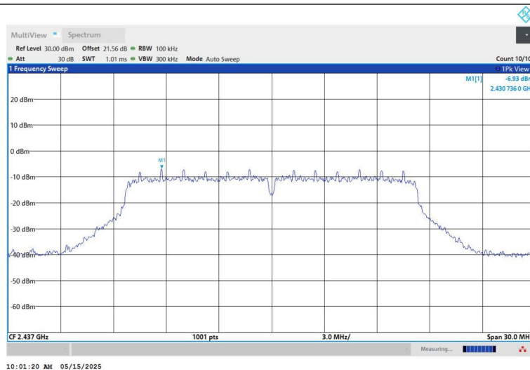
11G-Ant1-2437-0~Reference-PASS
