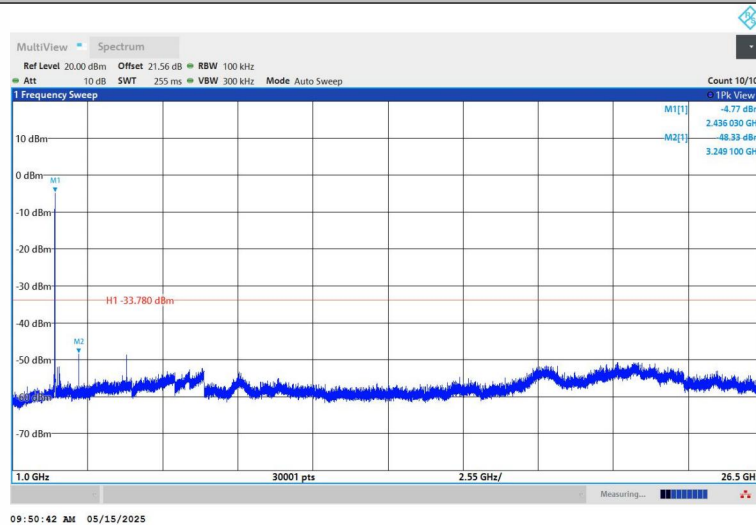
11B-Ant1-2437-1000~26500-PASS
