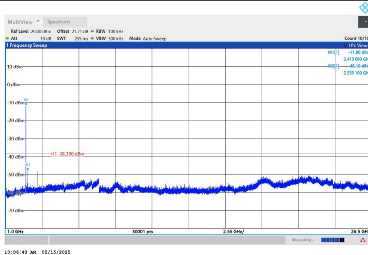
11N20SISO-Ant1-2412-1000~26500-PASS
