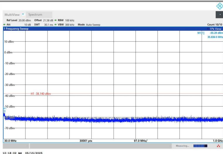
11N20SISO-Ant1-2462-30~1000-PASS
