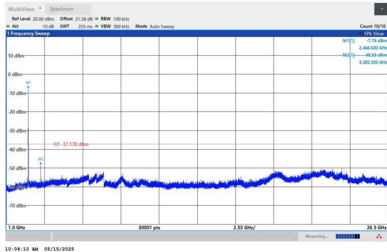
11G-Ant1-2462-1000~26500-PASS
