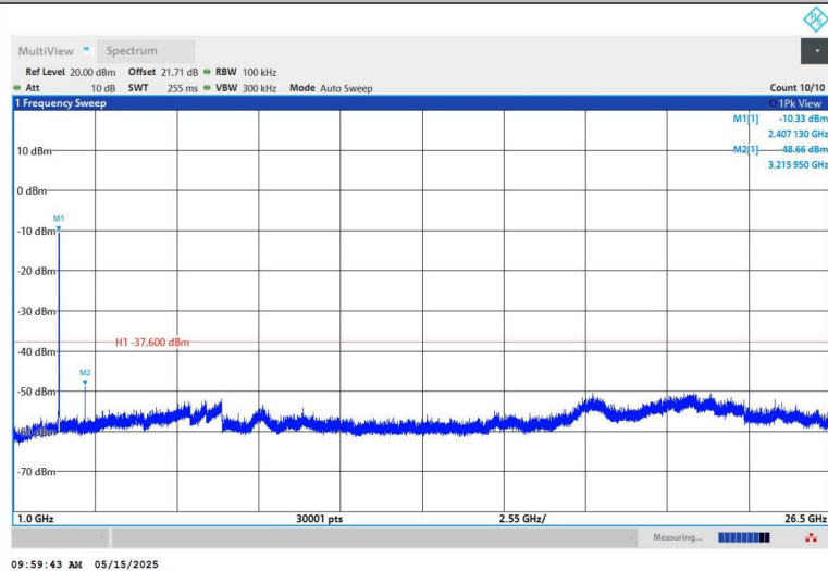
11G-Ant1-2412-1000~26500-PASS
