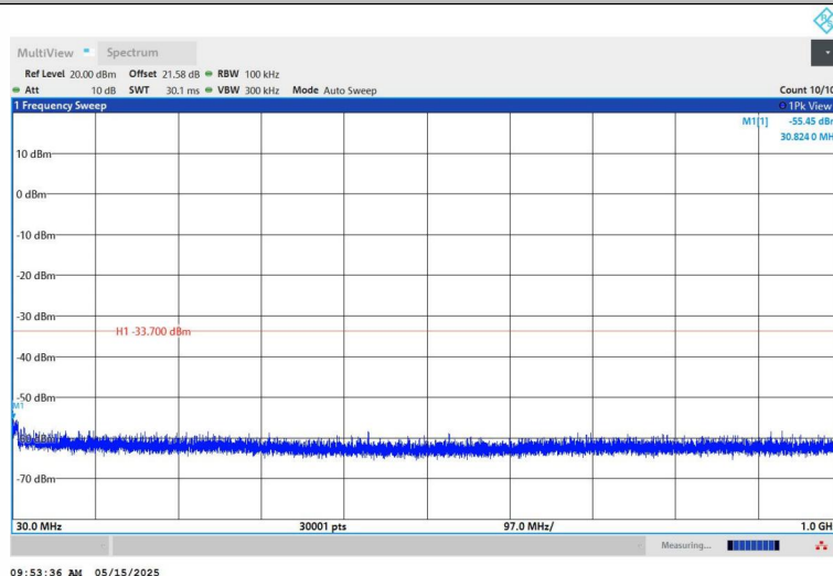
11B-Ant1-2462-30~1000-PASS
