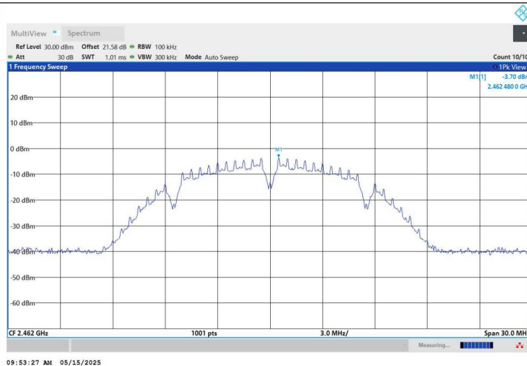
11B-Ant1-2462-0~Reference-PASS
