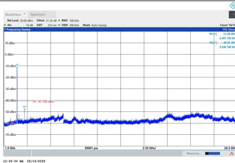
11N40SISO-Ant1-2437-1000~26500-PASS
