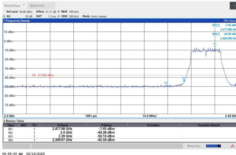
11G-Ant1-2412-PASS
