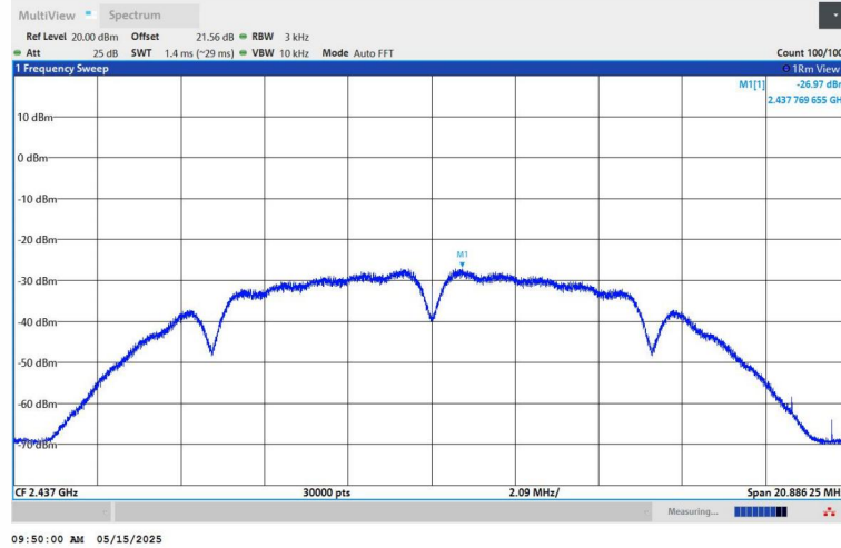
11B-Ant1-2437-PASS
