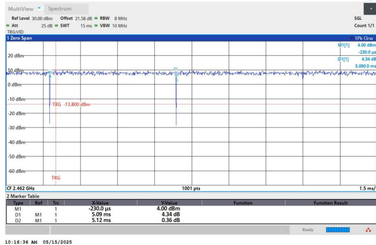
NTNV-11N20SISO-Ant1-2462
