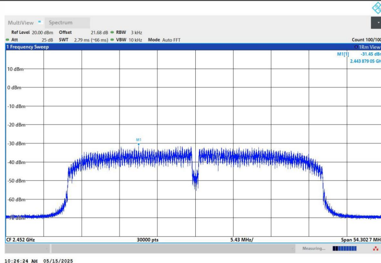
11N40SISO-Ant1-2452-PASS
