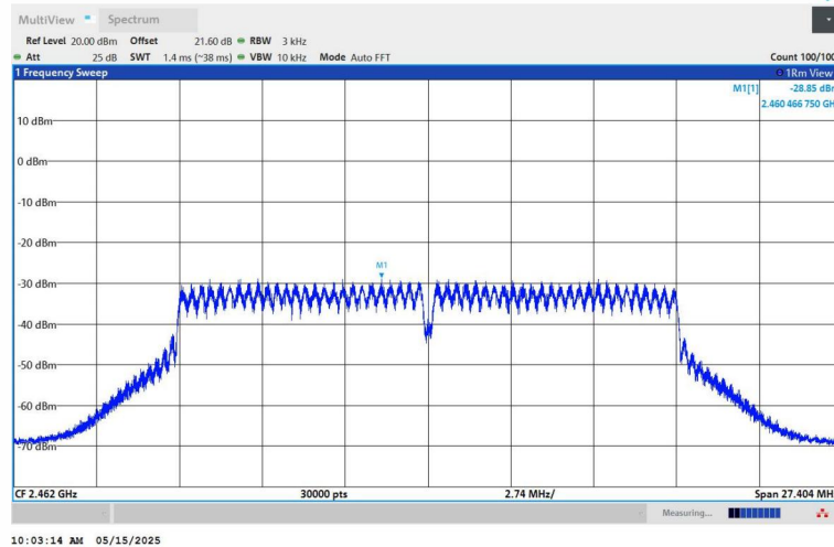
11G-Ant1-2462-PASS
