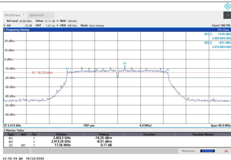
11N20SISO-Ant1-2412-PASS
