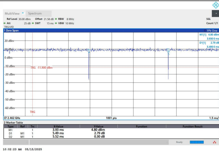
NTNV-11G-Ant1-2462
