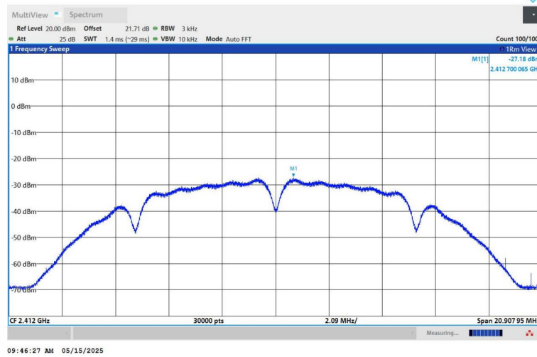
11B-Ant1-2412-PASS
