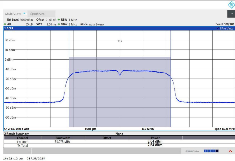
11N40SISO-Ant1-2437-PASS
