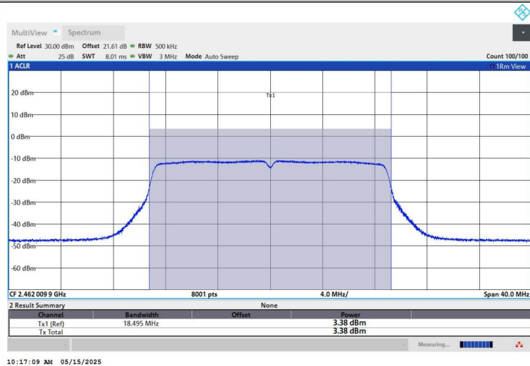
11N20SISO-Ant1-2462-PASS
