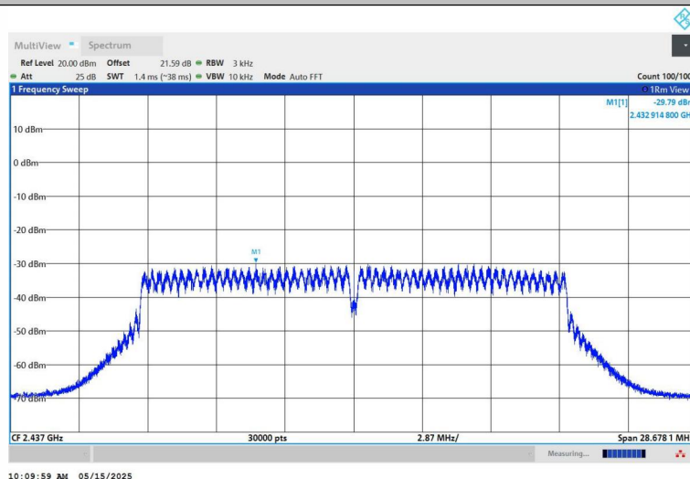
11N20SISO-Ant1-2437-PASS
