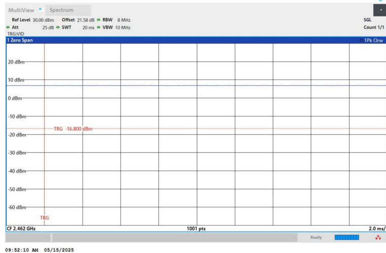
NTNV-11B-Ant1-2462
