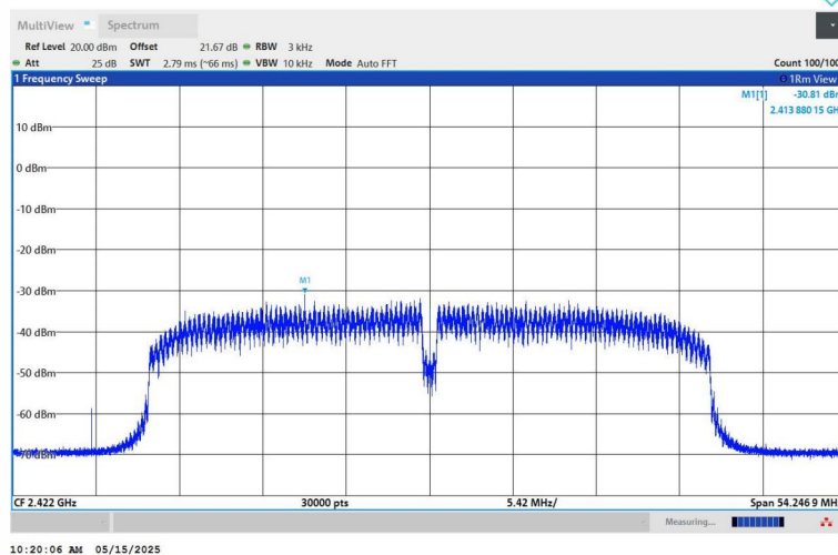
11N40SISO-Ant1-2422-PASS
