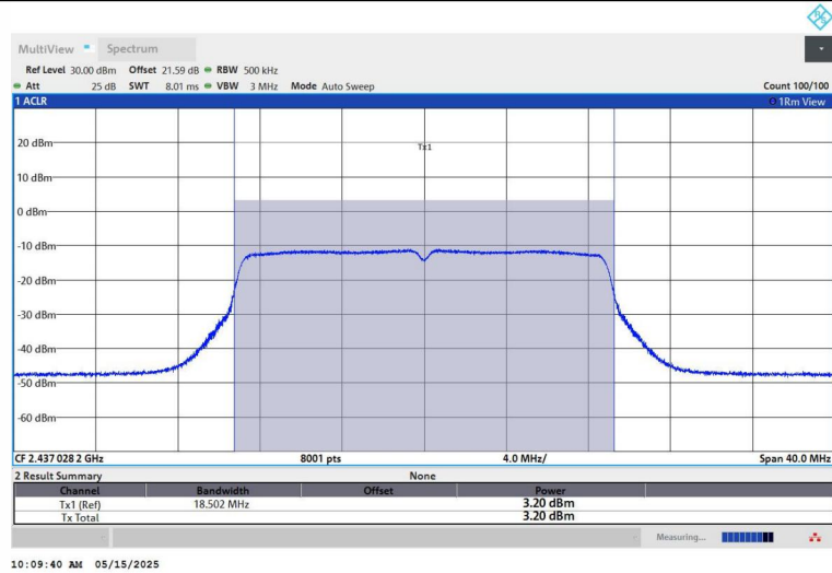
11N20SISO-Ant1-2437-PASS
