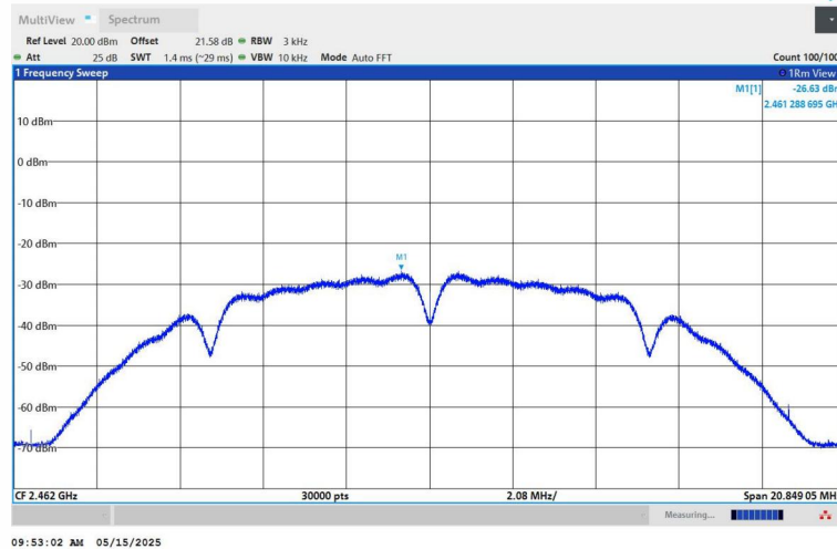
11B-Ant1-2462-PASS
