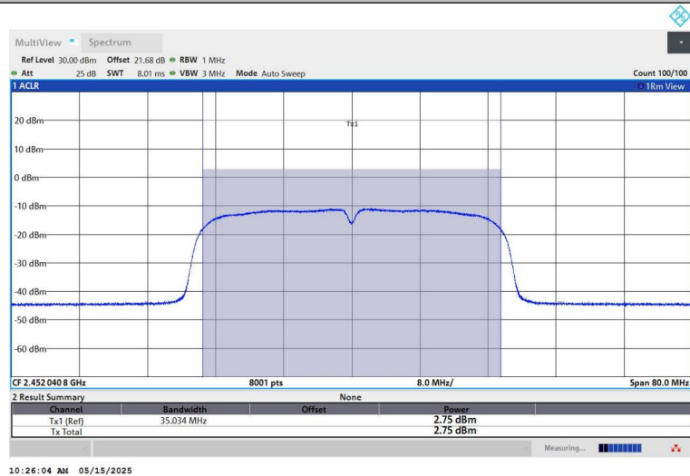
11N40SISO-Ant1-2452-PASS
