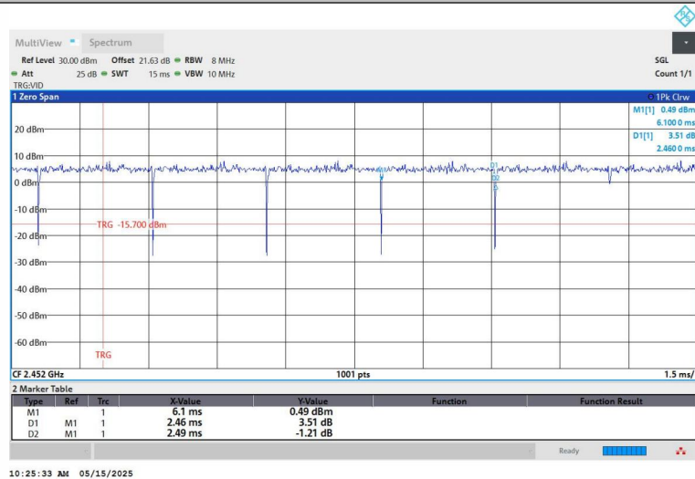
NTNV-11N40SISO-Ant1-2452
