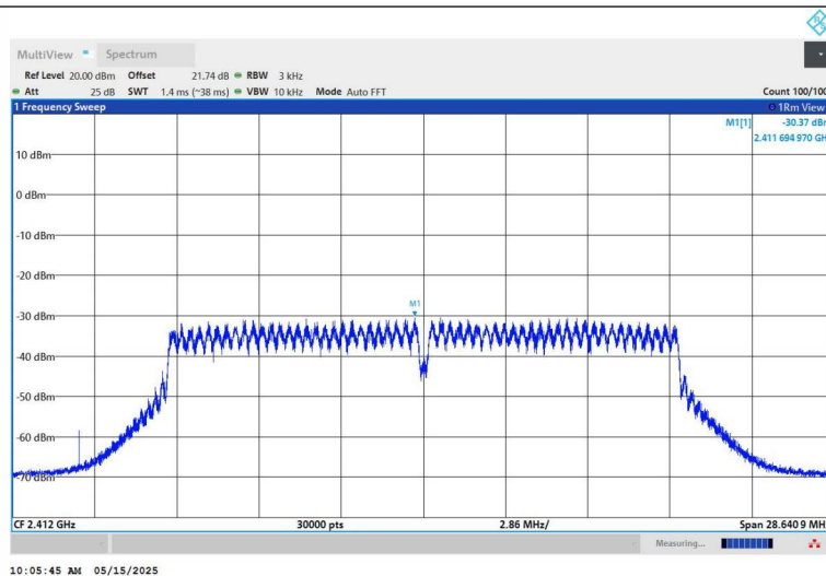
11N20SISO-Ant1-2412-PASS
