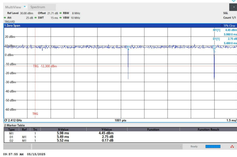
NTNV-11G-Ant1-2412
