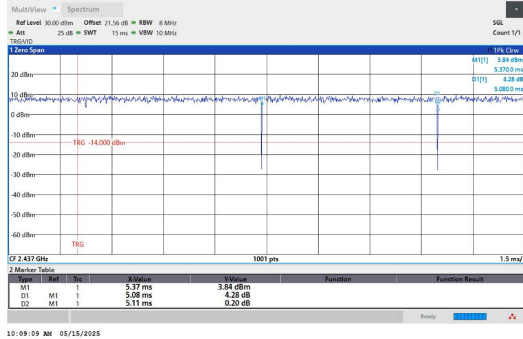
NTNV-11N20SISO-Ant1-2437
