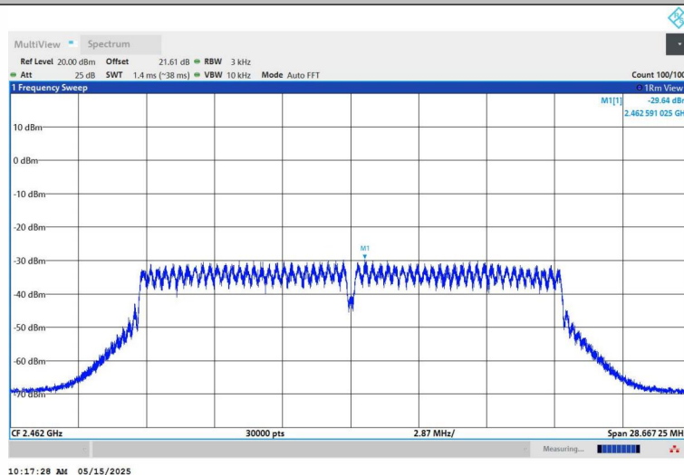
11N20SISO-Ant1-2462-PASS
