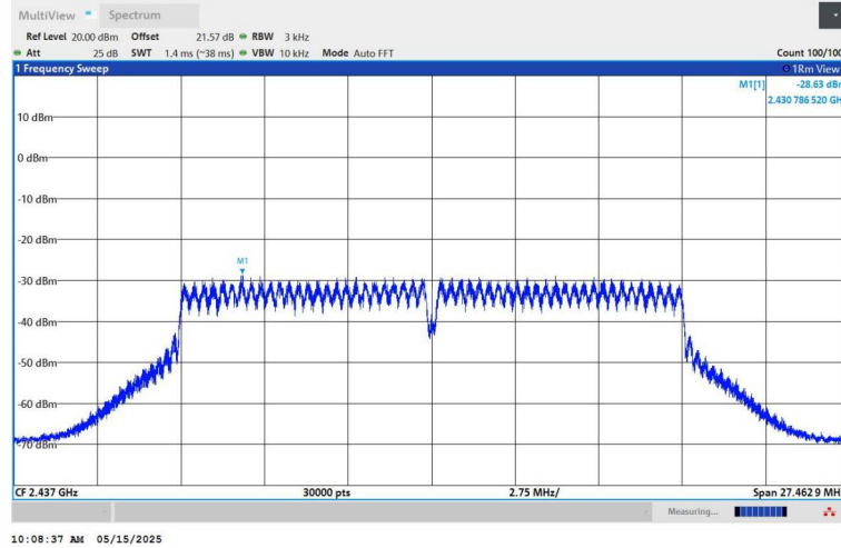
11G-Ant1-2437-PASS
