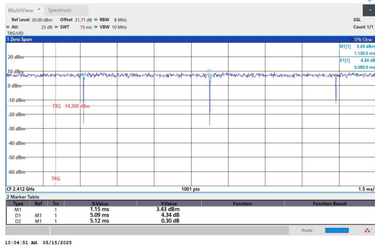
NTNV-11N20SISO-Ant1-2412
