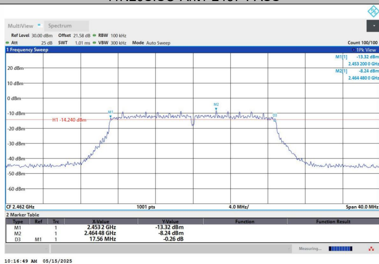
11N20SISO-Ant1-2462-PASS
