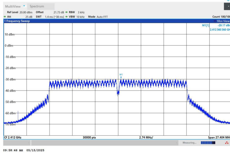
11G-Ant1-2412-PASS
