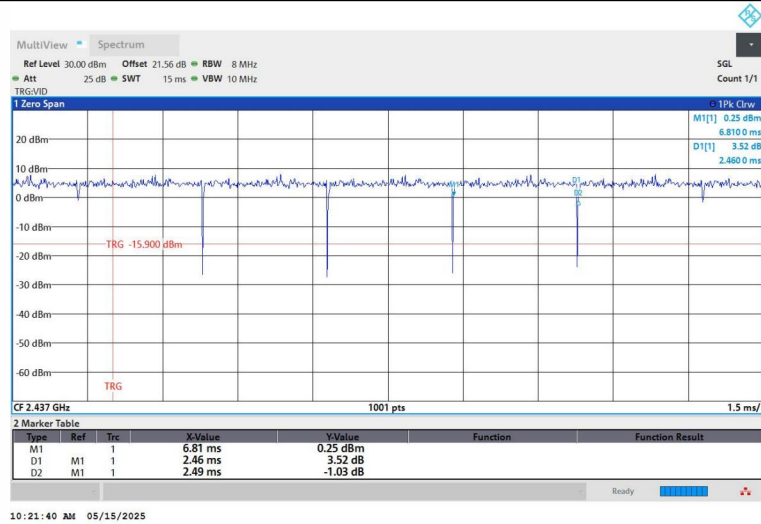
NTNV-11N40SISO-Ant1-2437
