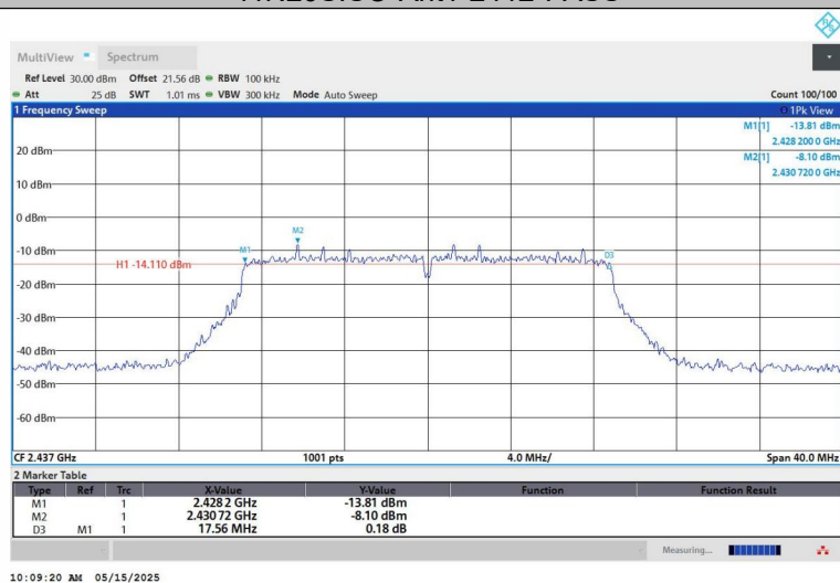
11N20SISO-Ant1-2437-PASS
