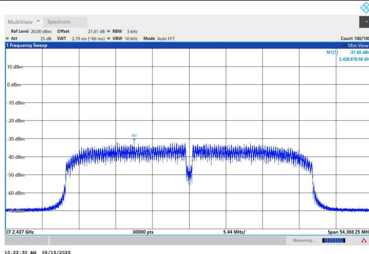
11N40SISO-Ant1-2437-PASS
