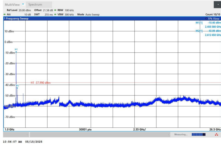
11N20SISO-Ant1-2462-1000~26500-PASS
