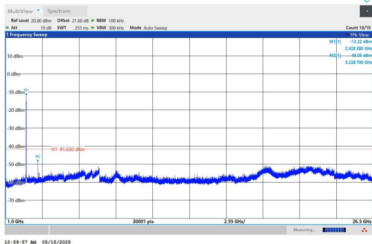
11N40SISO-Ant1-2422-1000~26500-PASS
