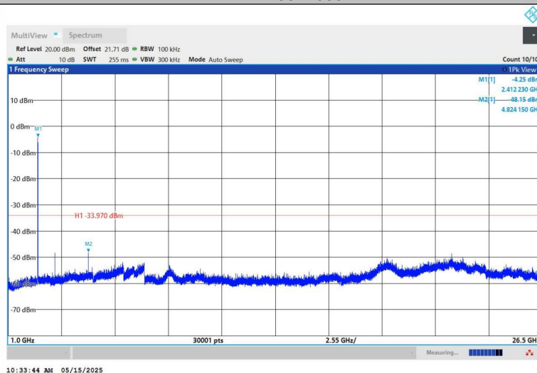
11B-Ant1-2412-1000~26500-PASS
