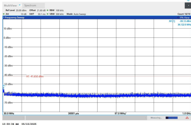
11N40SISO-Ant1-2422-30~1000-PASS
