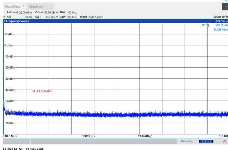
11N40SISO-Ant1-2437-30~1000-PASS
