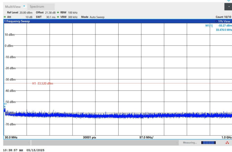
11B-Ant1-2462-30~1000-PASS
