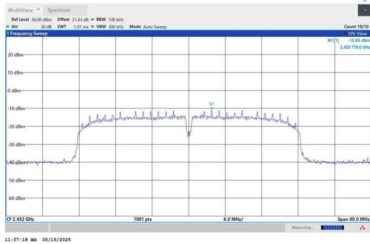
11N40SISO-Ant1-2452-0~Reference-PASS
