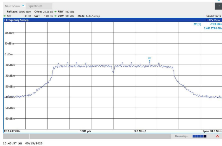
11G-Ant1-2437-0~Reference-PASS
