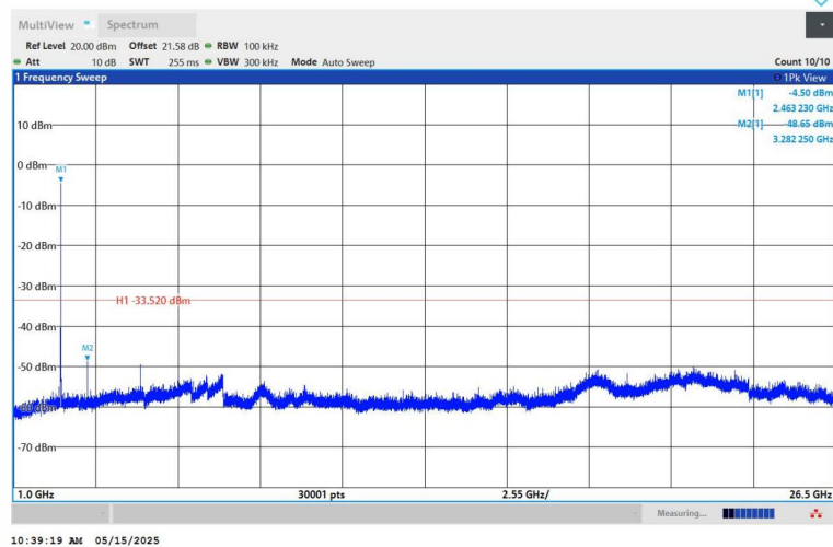
11B-Ant1-2462-1000~26500-PASS
