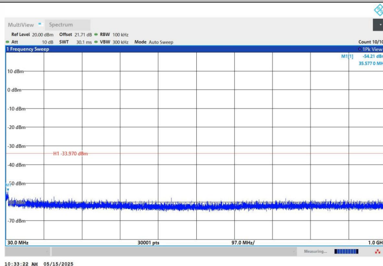
11B-Ant1-2412-30~1000-PASS
