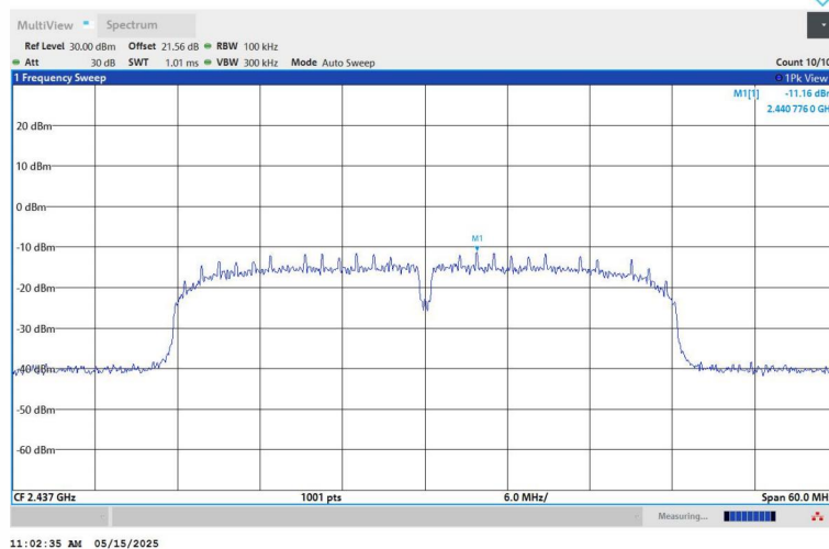
11N40SISO-Ant1-2437-0~Reference-PASS
