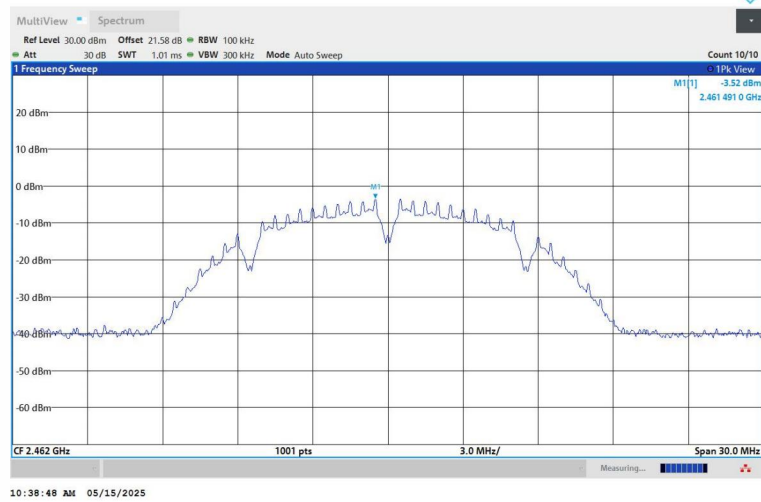
11B-Ant1-2462-0~Reference-PASS
