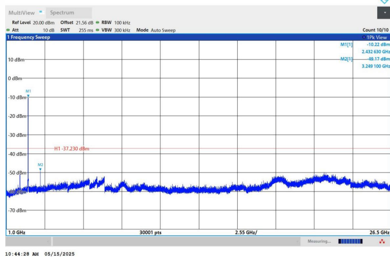
11G-Ant1-2437-1000~26500-PASS
