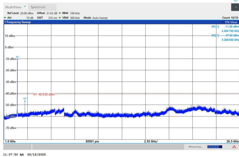
11N40SISO-Ant1-2452-1000~26500-PASS
