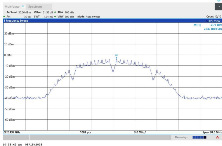
11B-Ant1-2437-0~Reference-PASS
