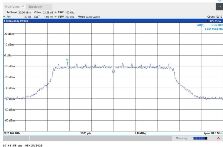
11G-Ant1-2462-0~Reference-PASS
