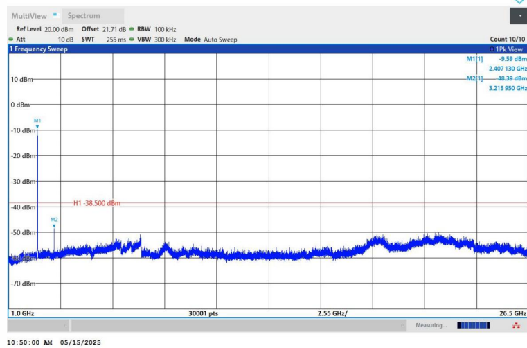
11N20SISO-Ant1-2412-1000~26500-PASS
