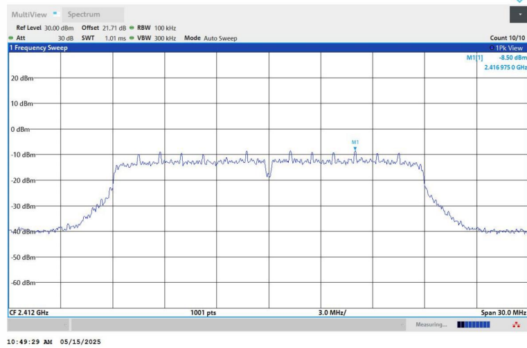
11N20SISO-Ant1-2412-0~Reference-PASS
