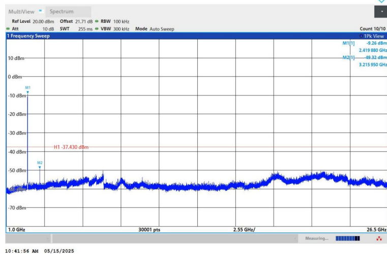
11G-Ant1-2412-1000~26500-PASS
