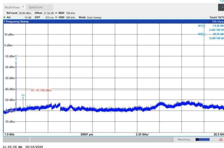
11N40SISO-Ant1-2437-1000~26500-PASS
