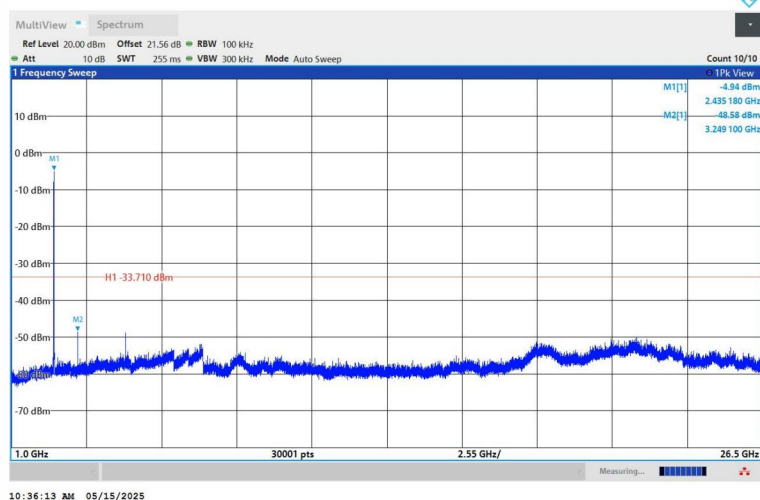
11B-Ant1-2437-1000~26500-PASS
