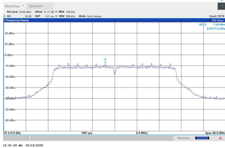
11G-Ant1-2412-0~Reference-PASS
