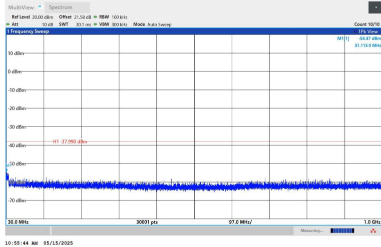
11N20SISO-Ant1-2462-30~1000-PASS
