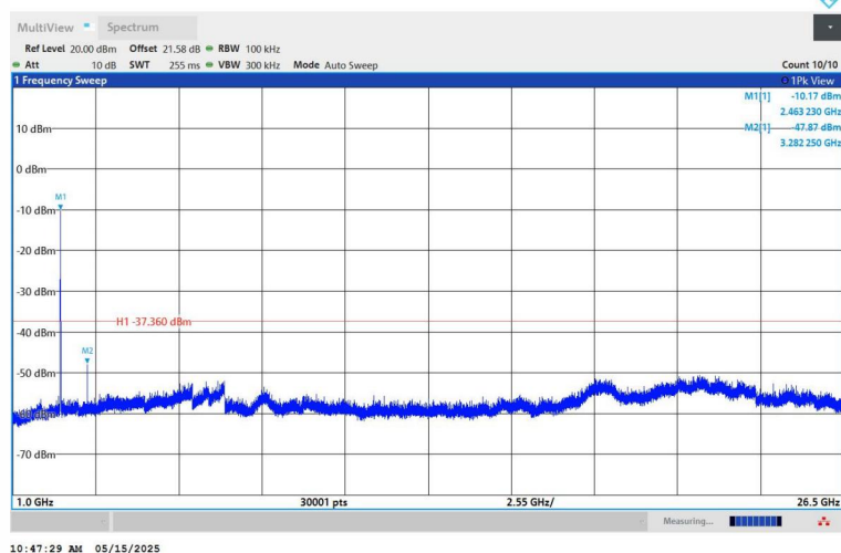
11G-Ant1-2462-1000~26500-PASS
