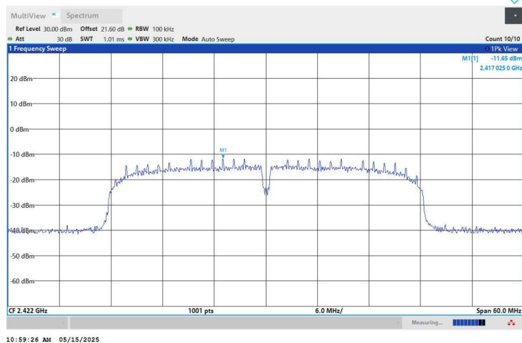
11N40SISO-Ant1-2422-0~Reference-PASS
