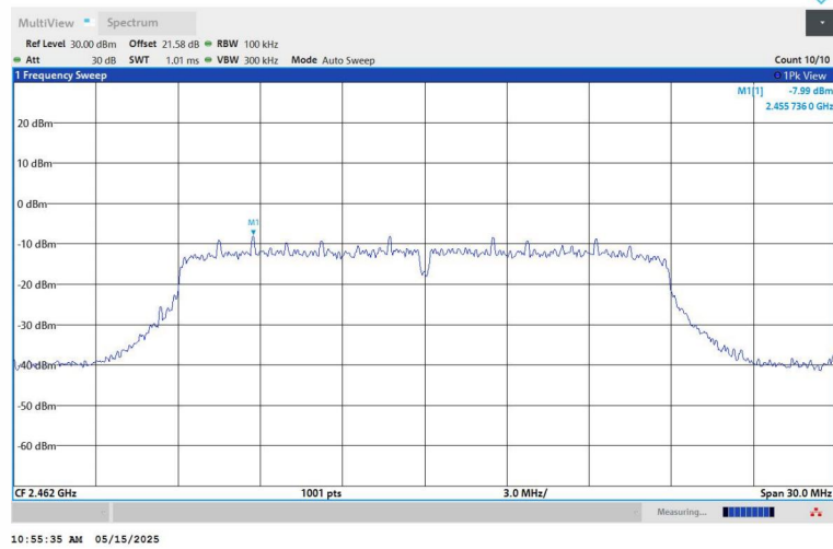
11N20SISO-Ant1-2462-0~Reference-PASS
