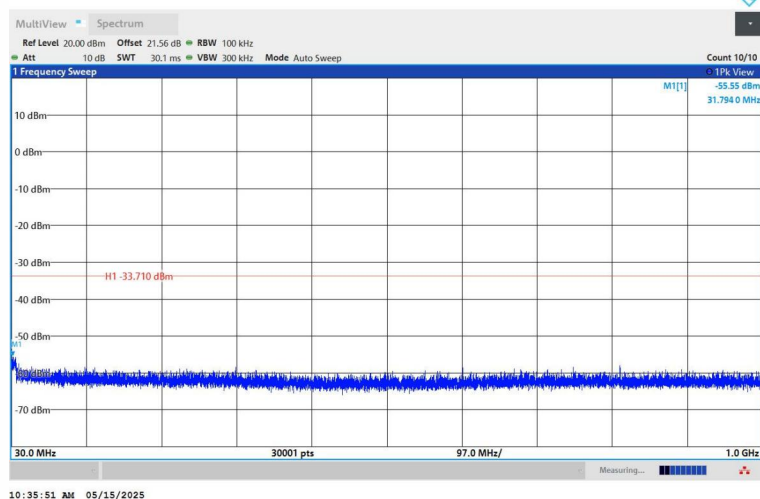
11B-Ant1-2437-30~1000-PASS
