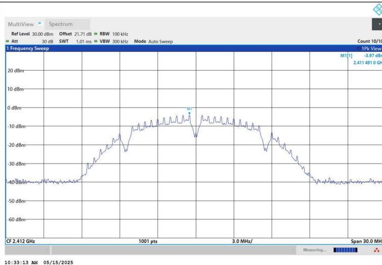
11B-Ant1-2412-0~Reference-PASS
