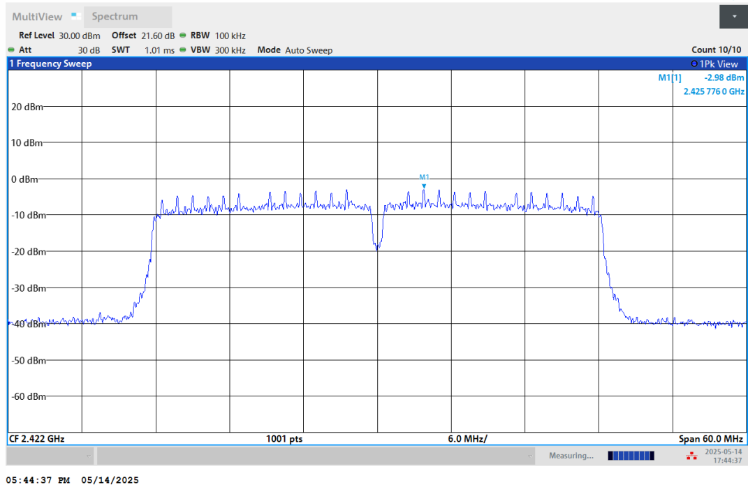
11N40SISO-Ant1-2422-0~Reference-PASS
