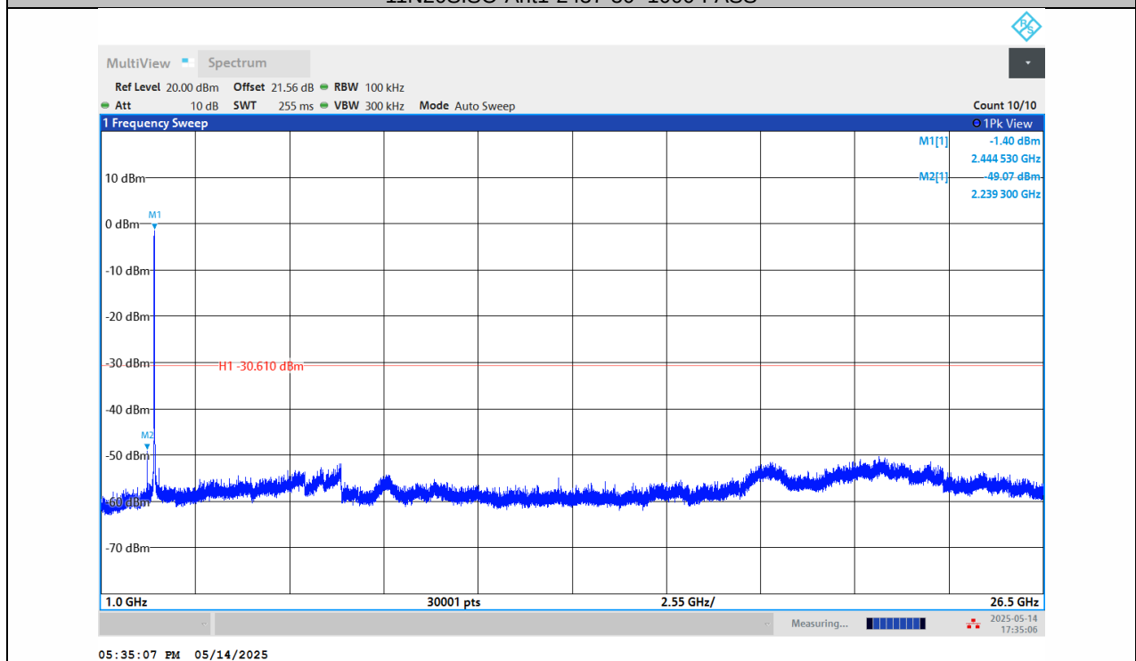
11N20SISO-Ant1-2437-1000~26500-PASS
