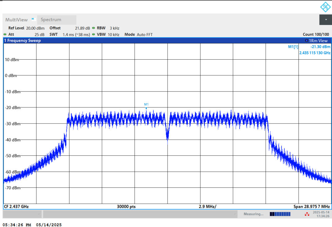
11N20SISO-Ant1-2437-PASS
