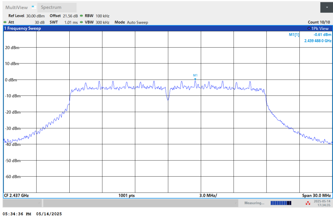
11N20SISO-Ant1-2437-0~Reference-PASS
