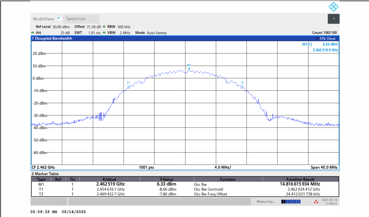
11B-Ant1-2462
