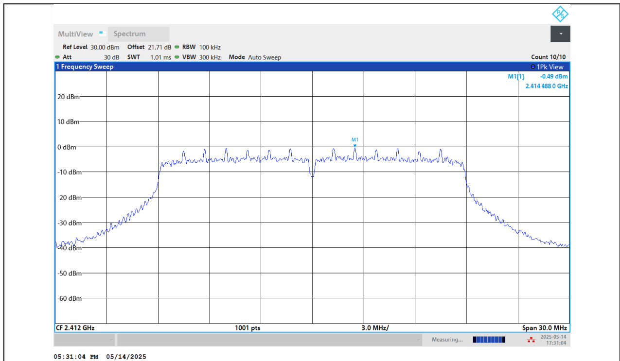
11N20SISO-Ant1-2412-0~Reference-PASS
