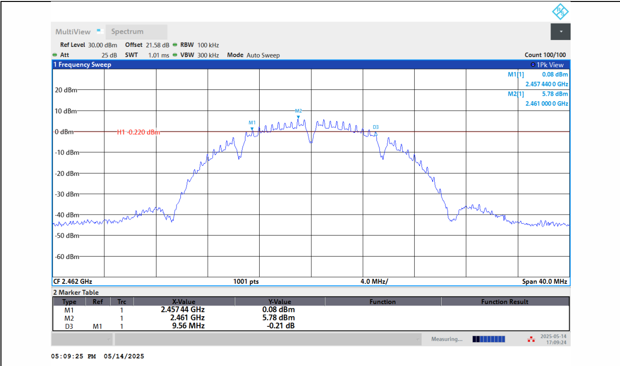
11B-Ant1-2462-PASS
