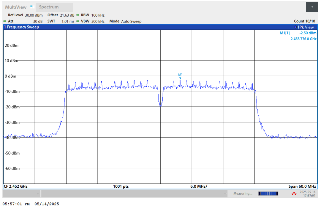
11N40SISO-Ant1-2452-0~Reference-PASS
