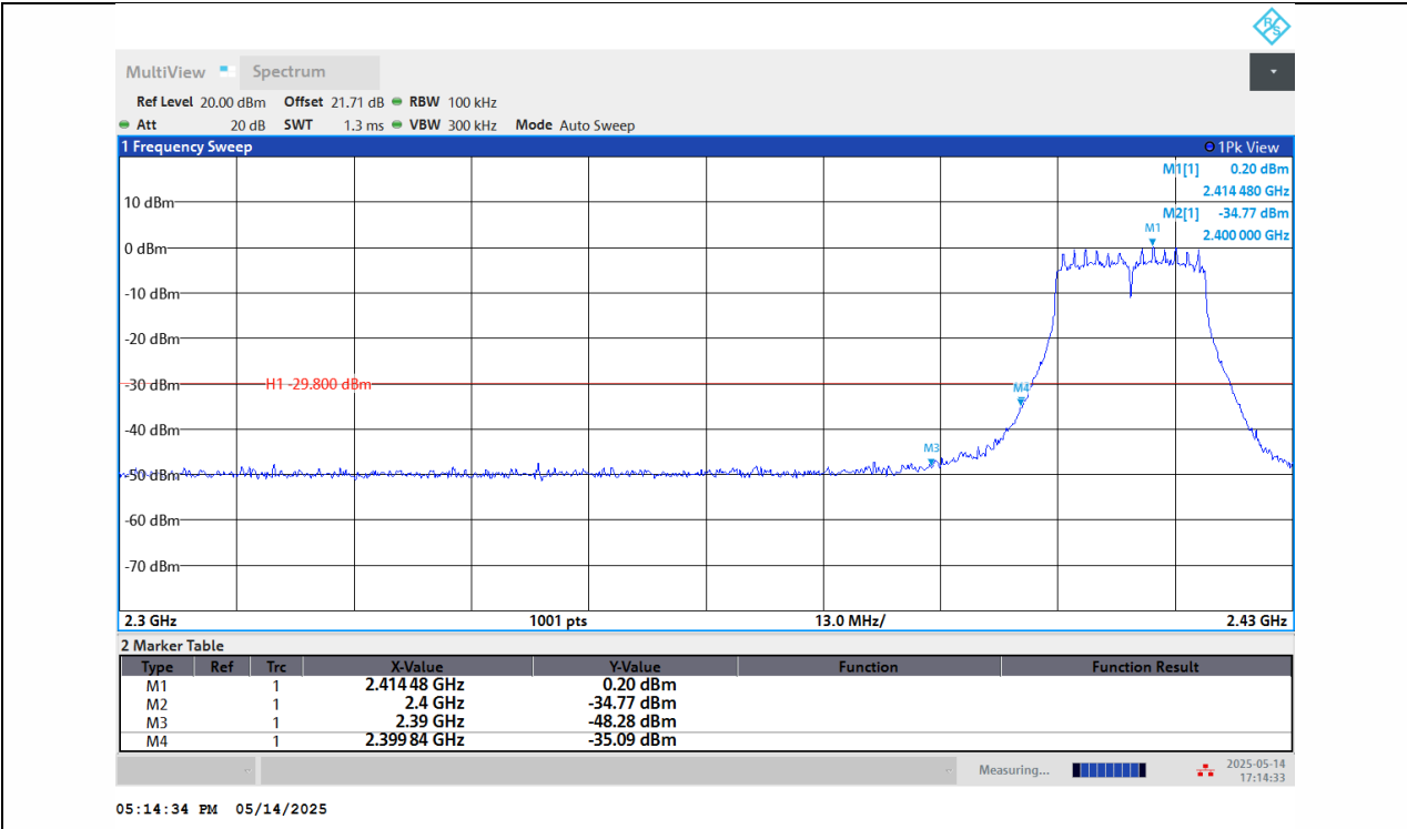
11G-Ant1-2412-PASS
