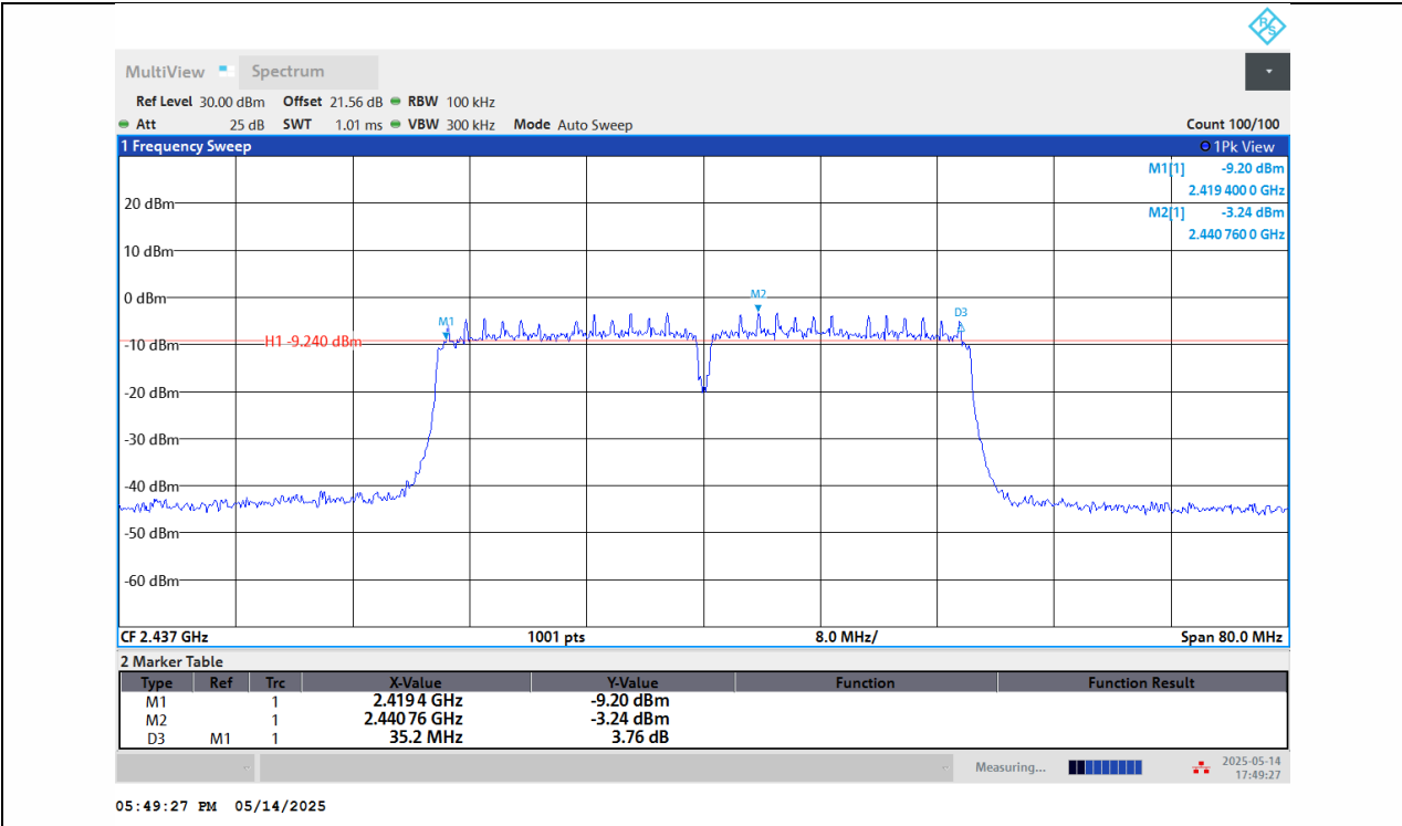
11N40SISO-Ant1-2437-PASS
