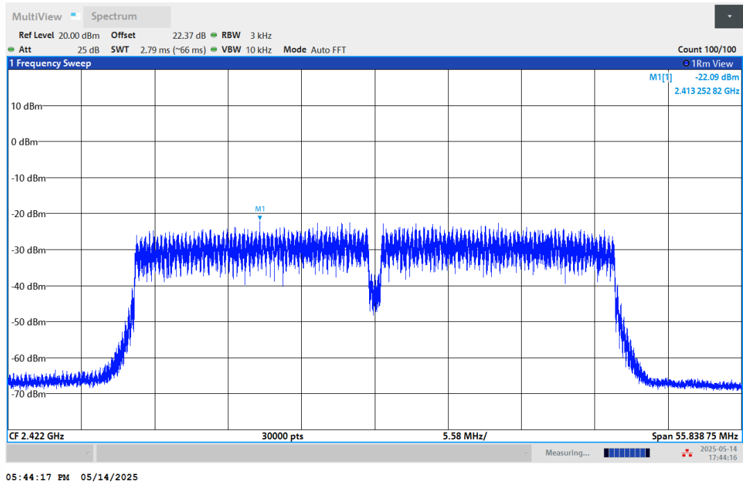
11N40SISO-Ant1-2422-PASS
