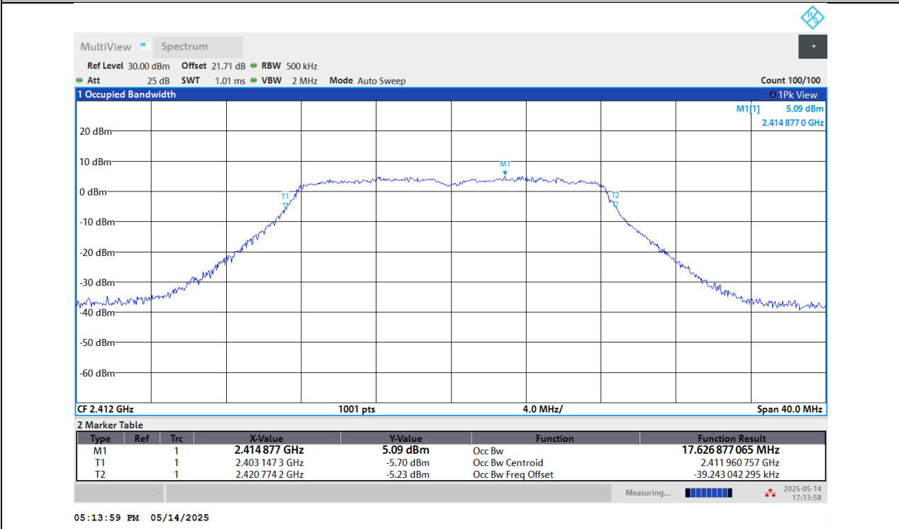
11G-Ant1-2412
