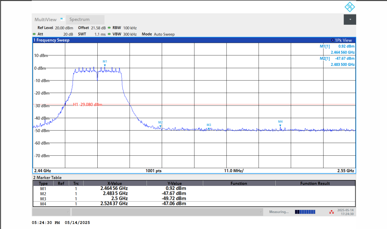
11G-Ant1-2462-PASS
