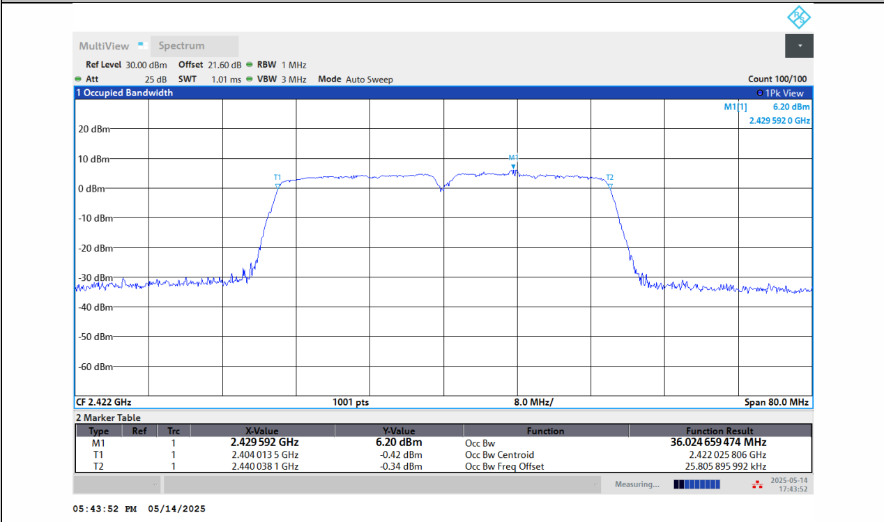
11N40SISO-Ant1-2422
