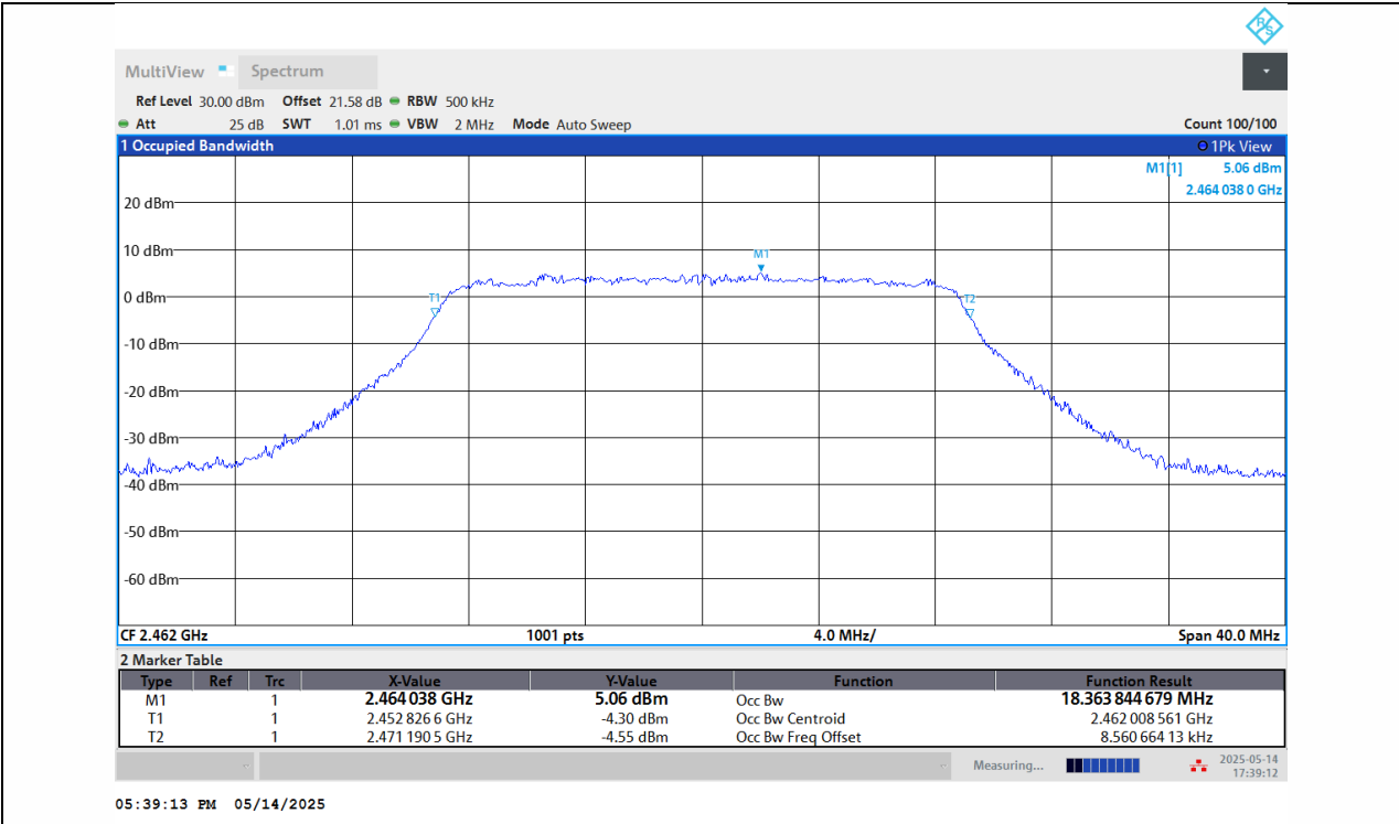
11N20SISO-Ant1-2462
