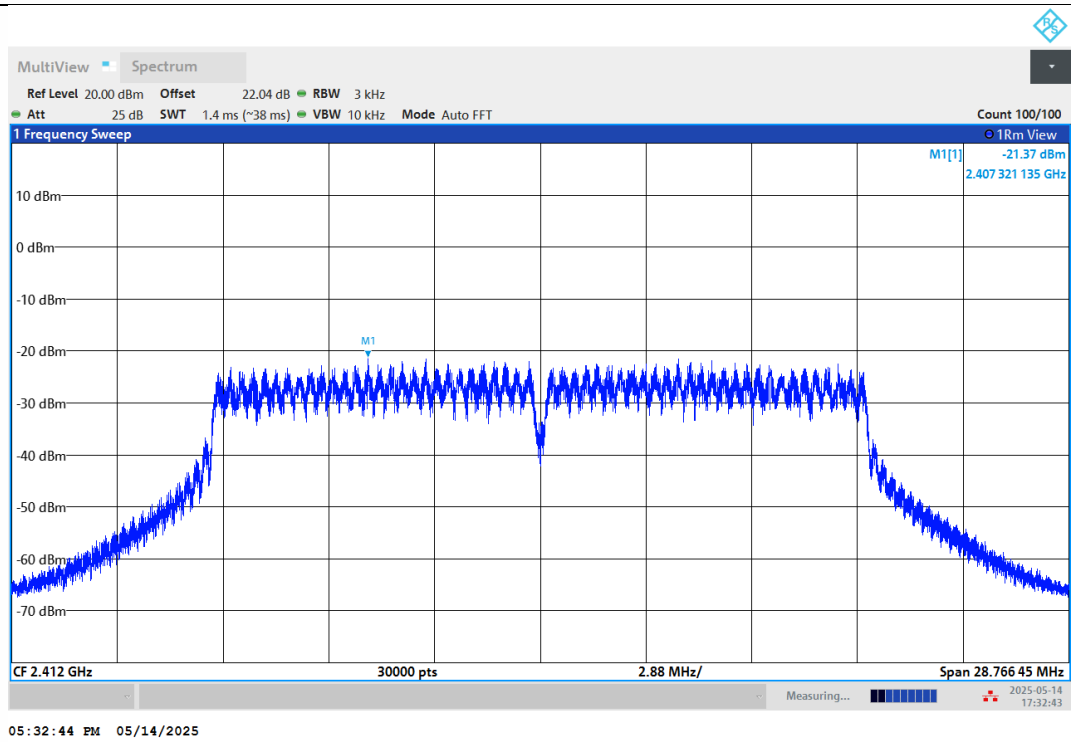
11N20SISO-Ant1-2412-PASS
