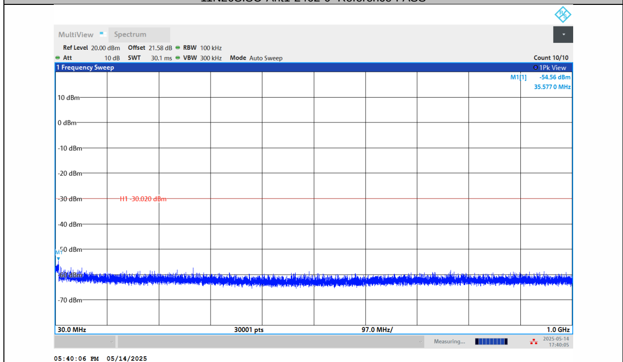
11N20SISO-Ant1-2462-30~1000-PASS
