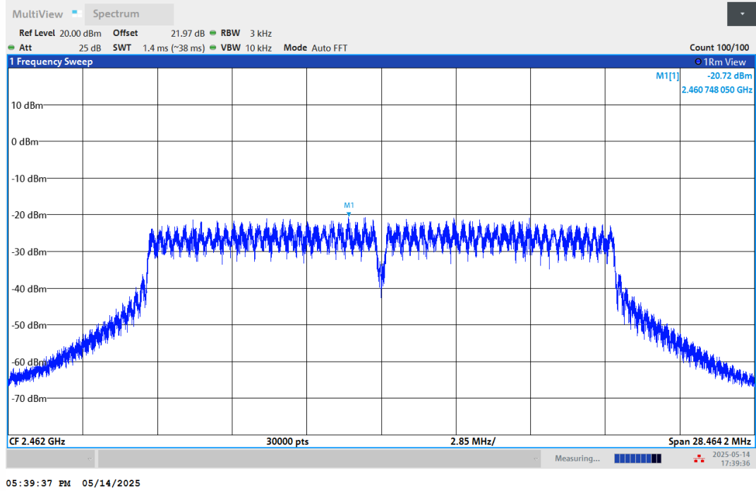
11N20SISO-Ant1-2462-PASS
