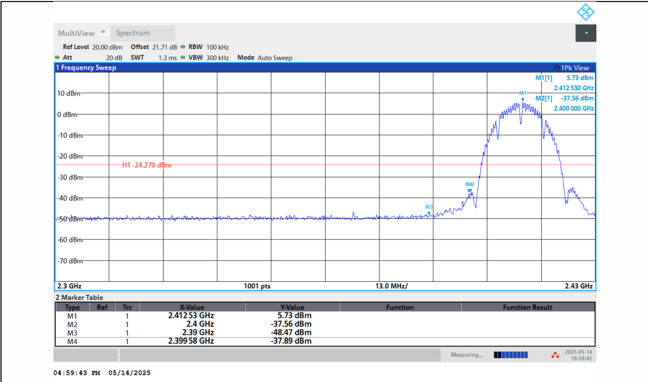
11B-Ant1-2412-PASS
