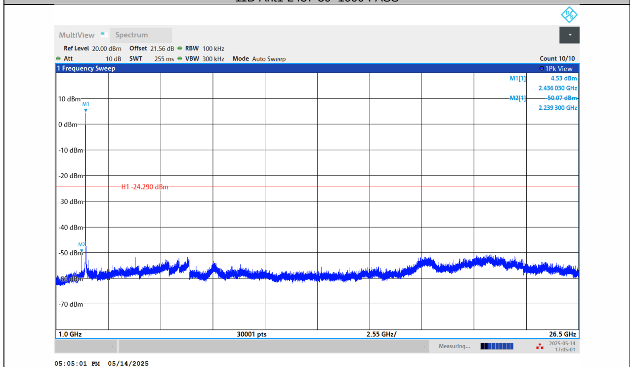
11B-Ant1-2437-1000~26500-PASS
