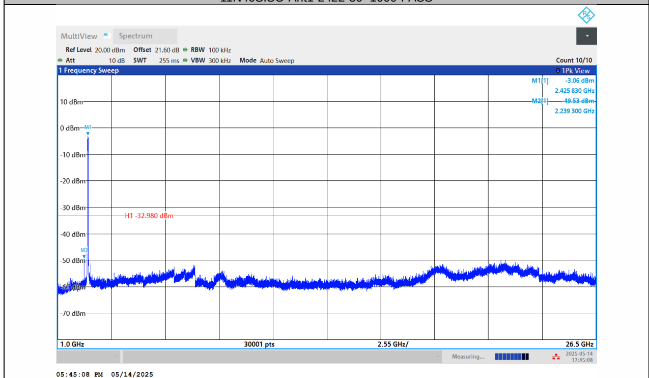
11N40SISO-Ant1-2422-1000~26500-PASS
