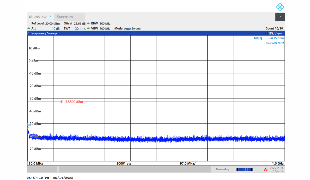
11N40SISO-Ant1-2452-30~1000-PASS
