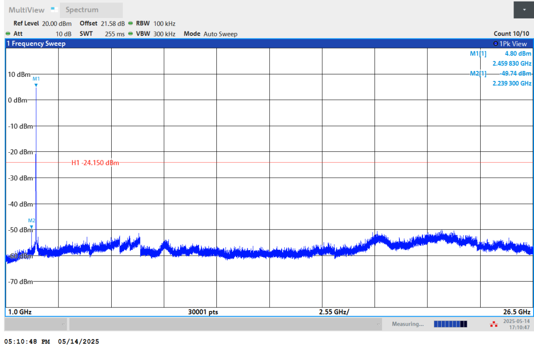
11B-Ant1-2462-1000~26500-PASS
