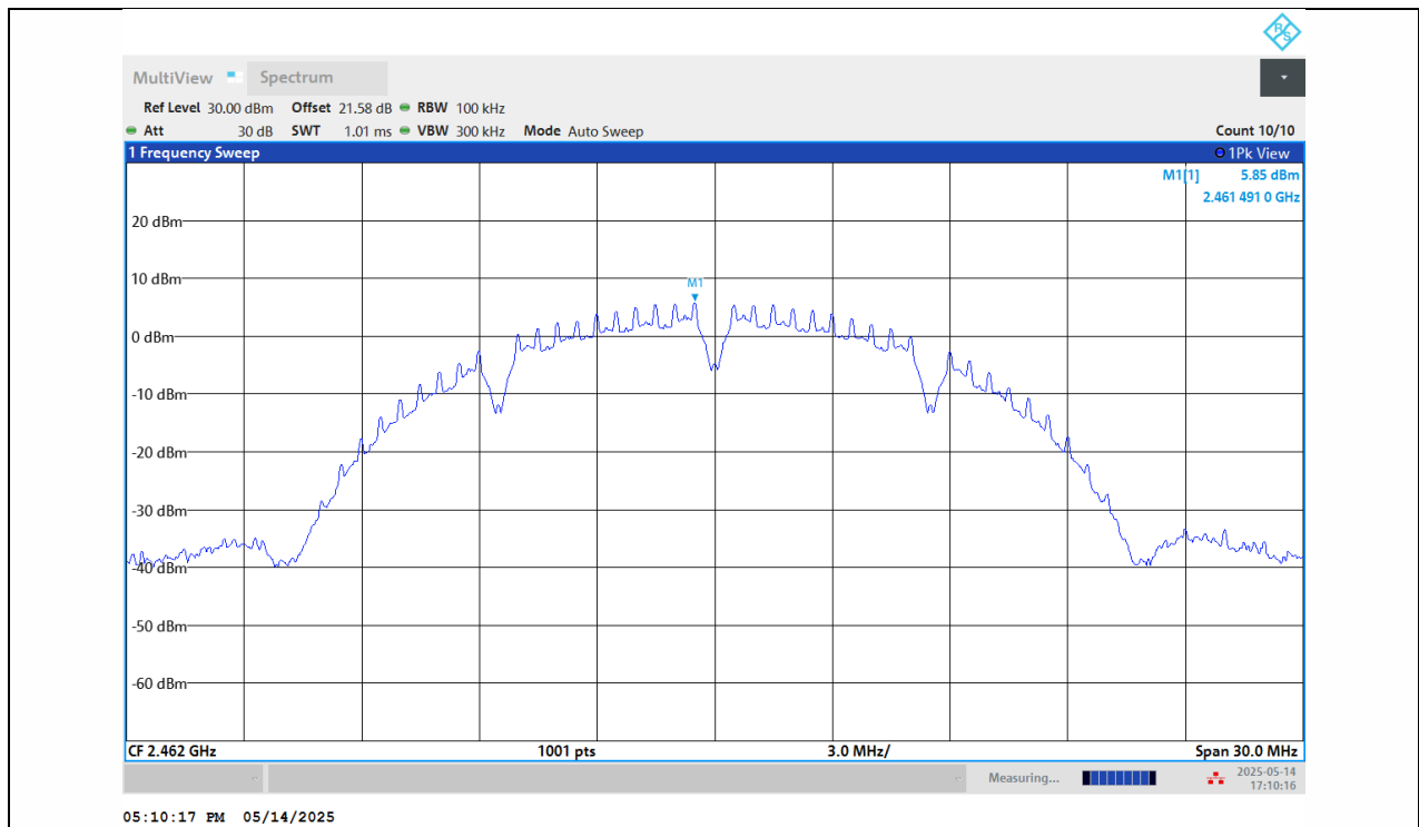
11B-Ant1-2462-0~Reference-PASS
