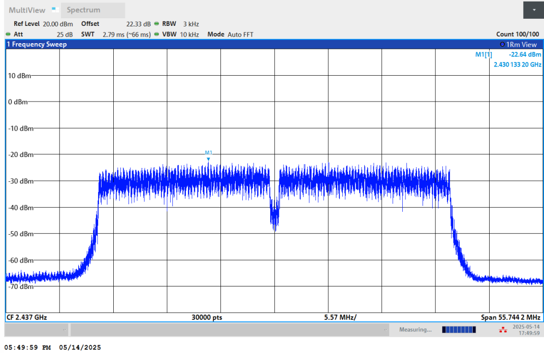
11N40SISO-Ant1-2437-PASS
