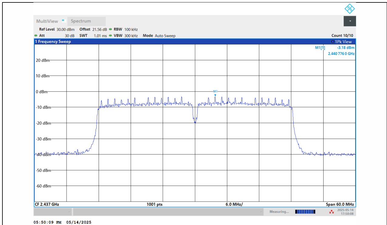
11N40ISO-Ant1-2437-0~Reference-PASS
