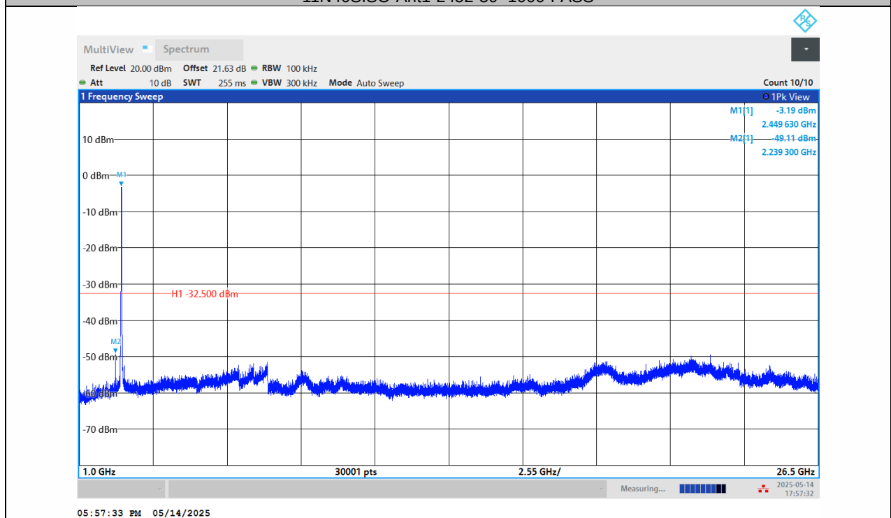
11N40SISO-Ant1-2452-1000~26500-PASS
