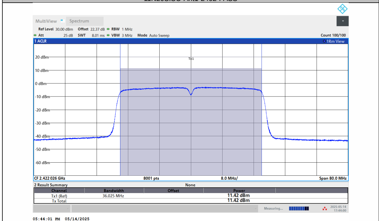
11N40SISO-Ant1-2422-PASS
