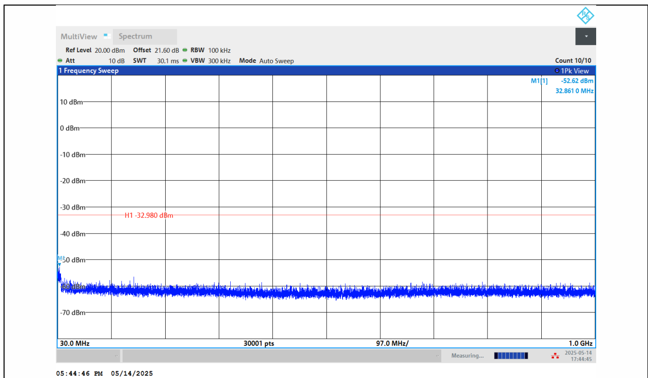
11N40SISO-Ant1-2422-30~1000-PASS
