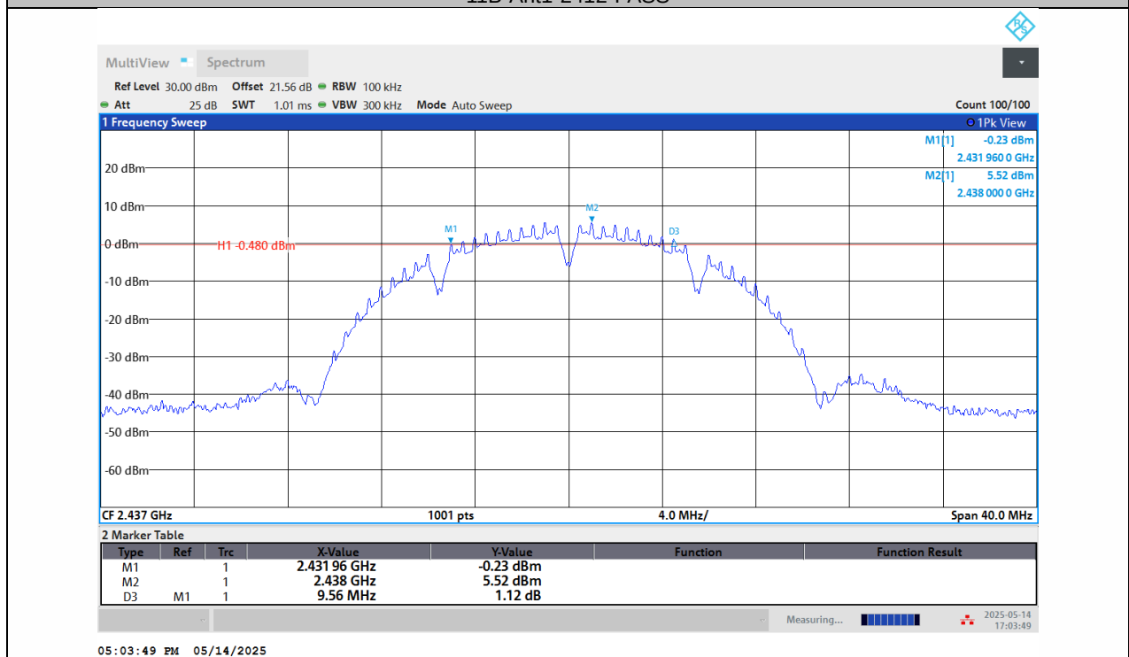
11B-Ant1-2437-PASS
