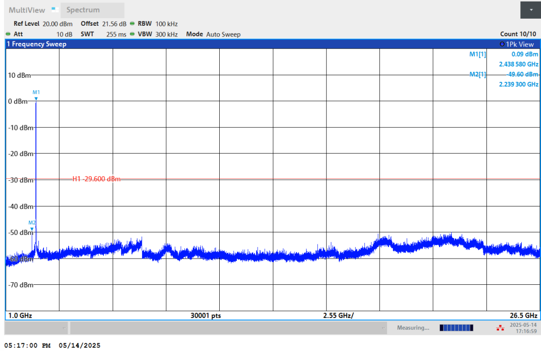
11G-Ant1-2437-1000~26500-PASS
