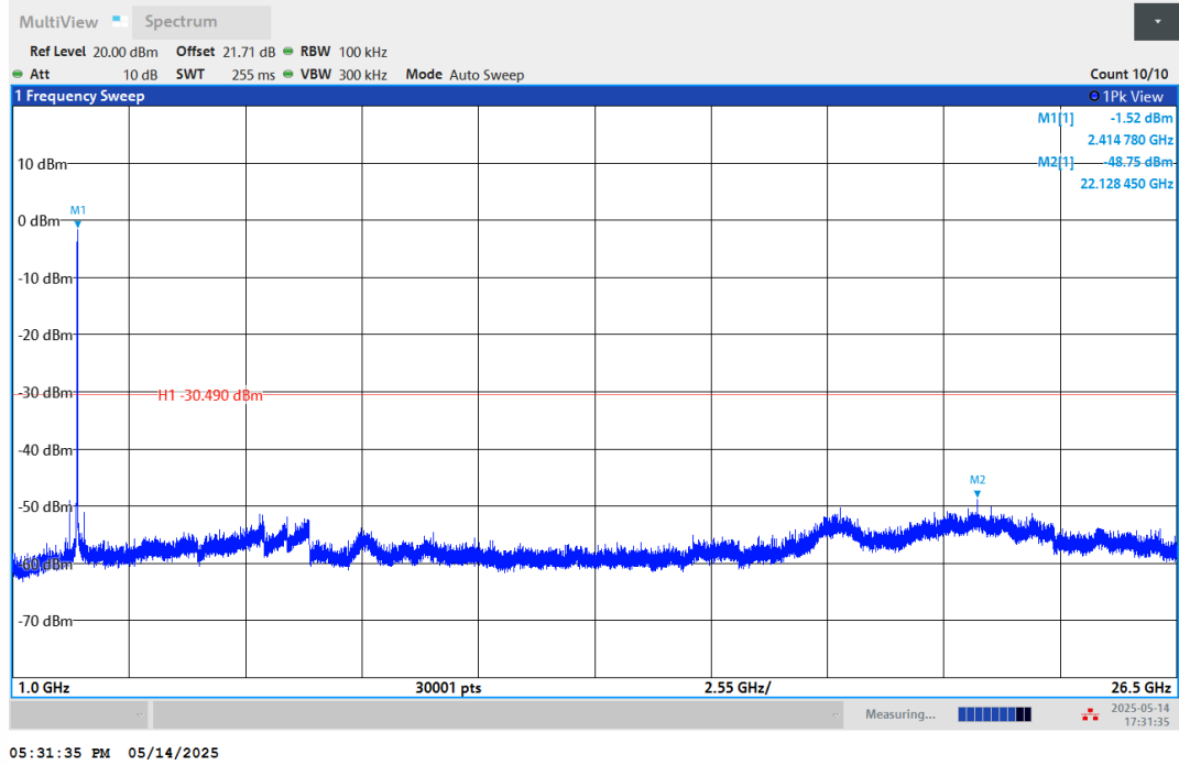
11N20SISO-Ant1-2412-1000~26500-PASS
