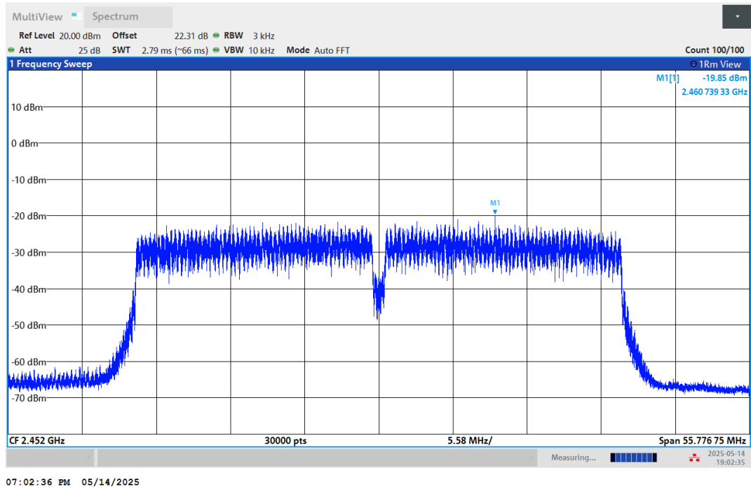
11N40SISO-Ant1-2452-PASS
