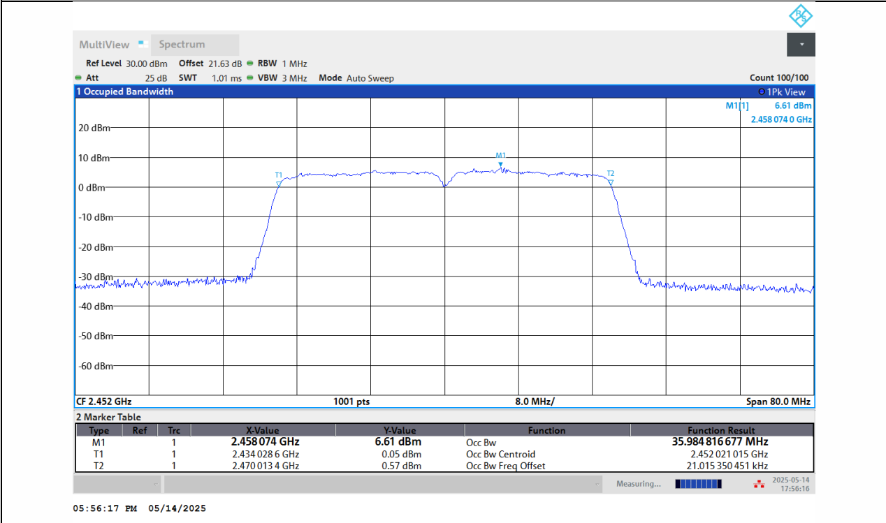
11N40SISO-Ant1-2452
