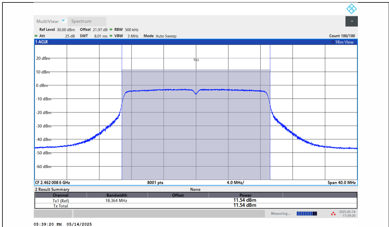
11N20SISO-Ant1-2462-PASS
