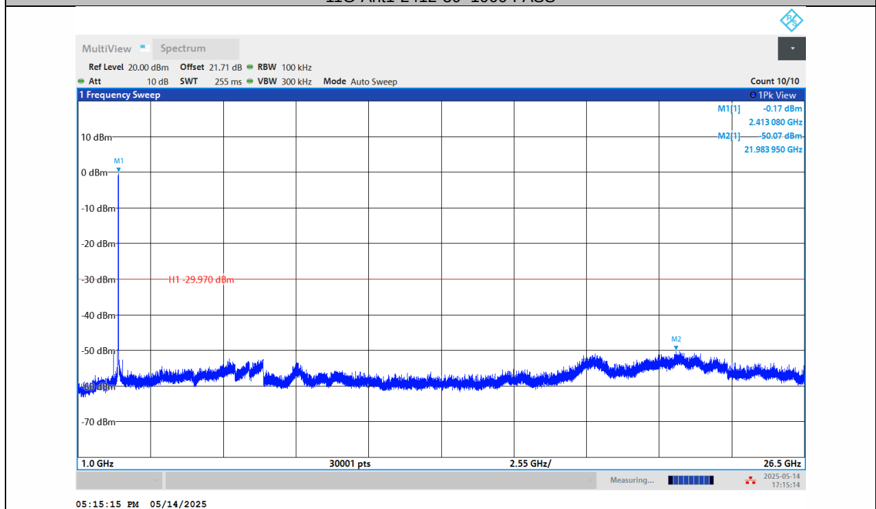
11G-Ant1-2412-1000~26500-PASS
