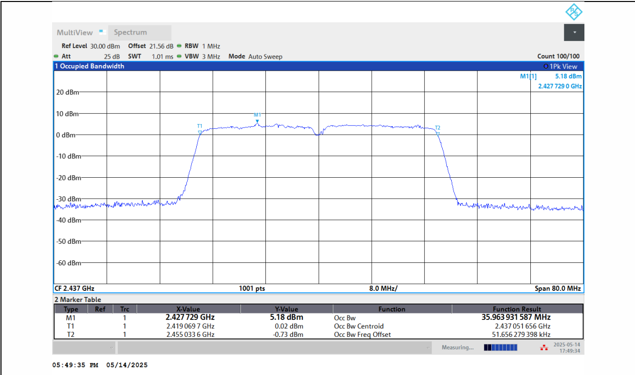
11N40SISO-Ant1-2437
