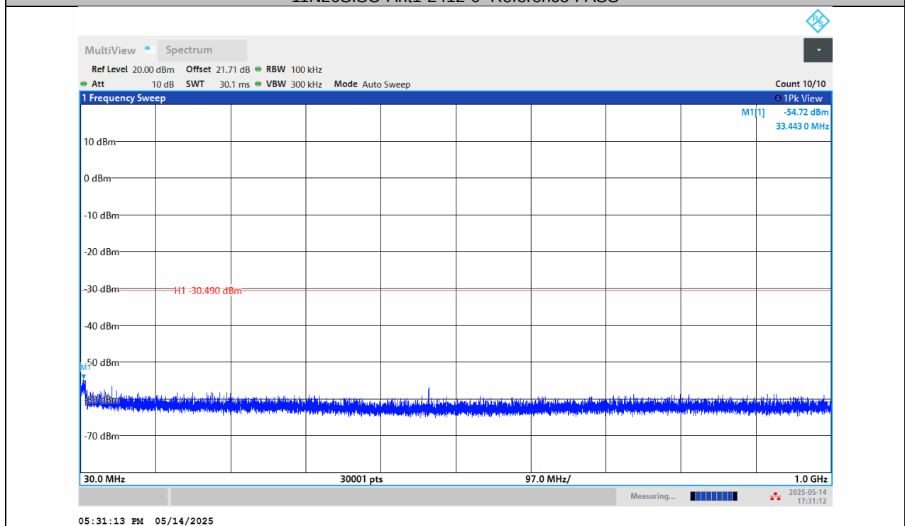
11N20SISO-Ant1-2412-30~1000-PASS
