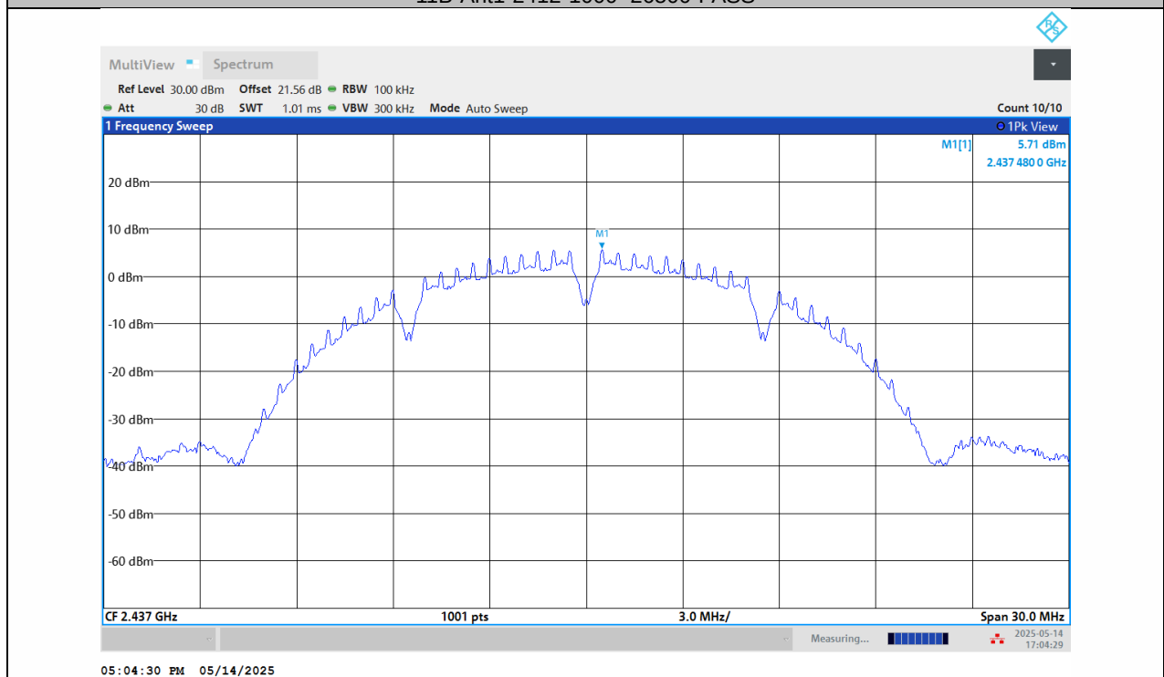
11B-Ant1-2437-0~Reference-PASS
