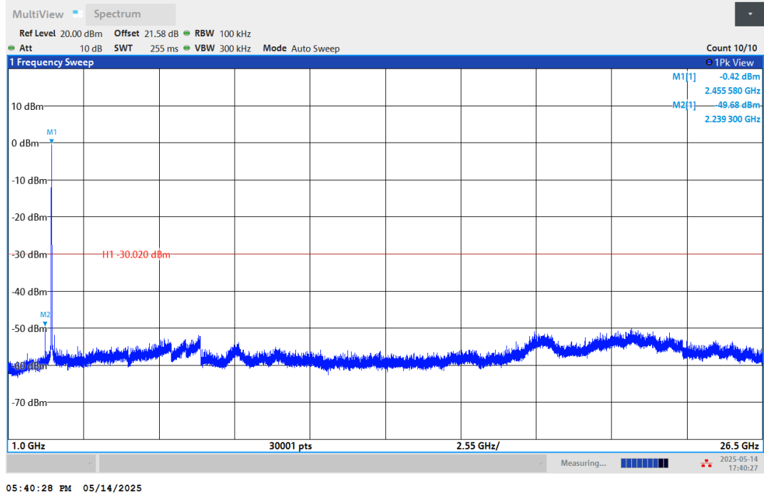
11N20SISO-Ant1-2462-1000~26500-PASS
