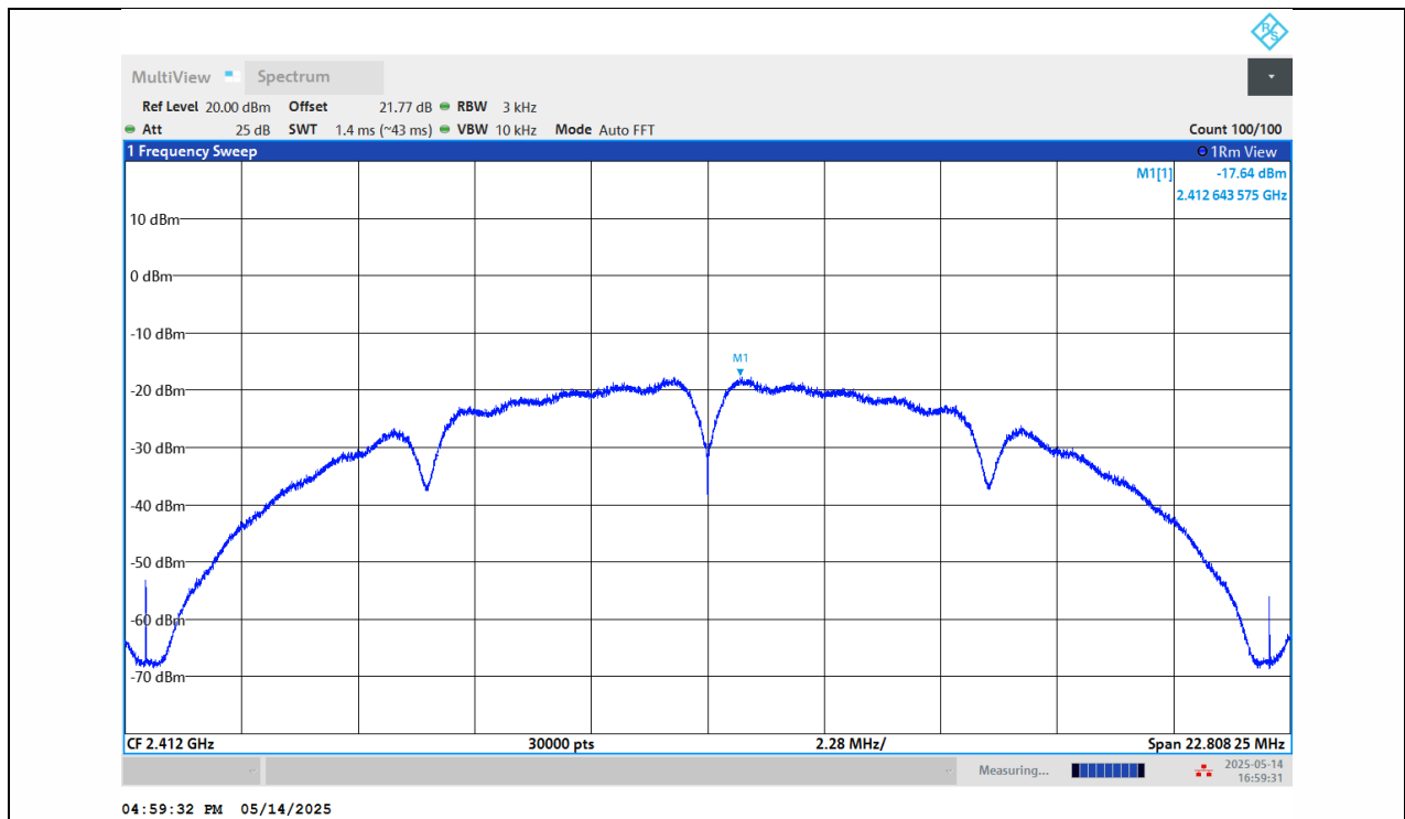
11B-Ant1-2412-PASS
