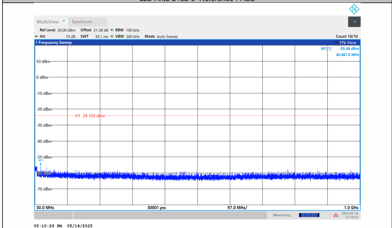
11B-Ant1-2462-30~1000-PASS
