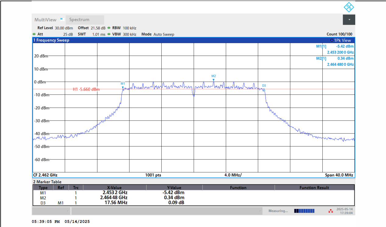
11N20SISO-Ant1-2462-PASS
