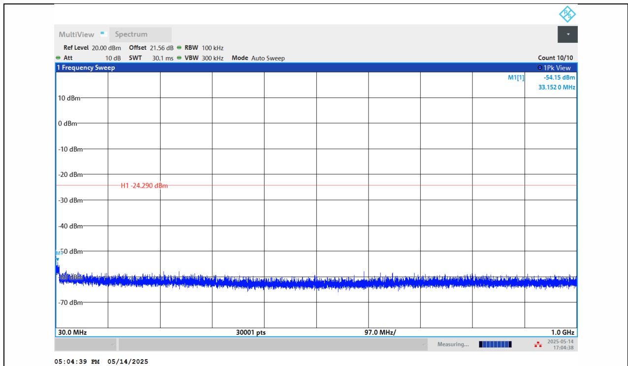
11B-Ant1-2437-30~1000-PASS
