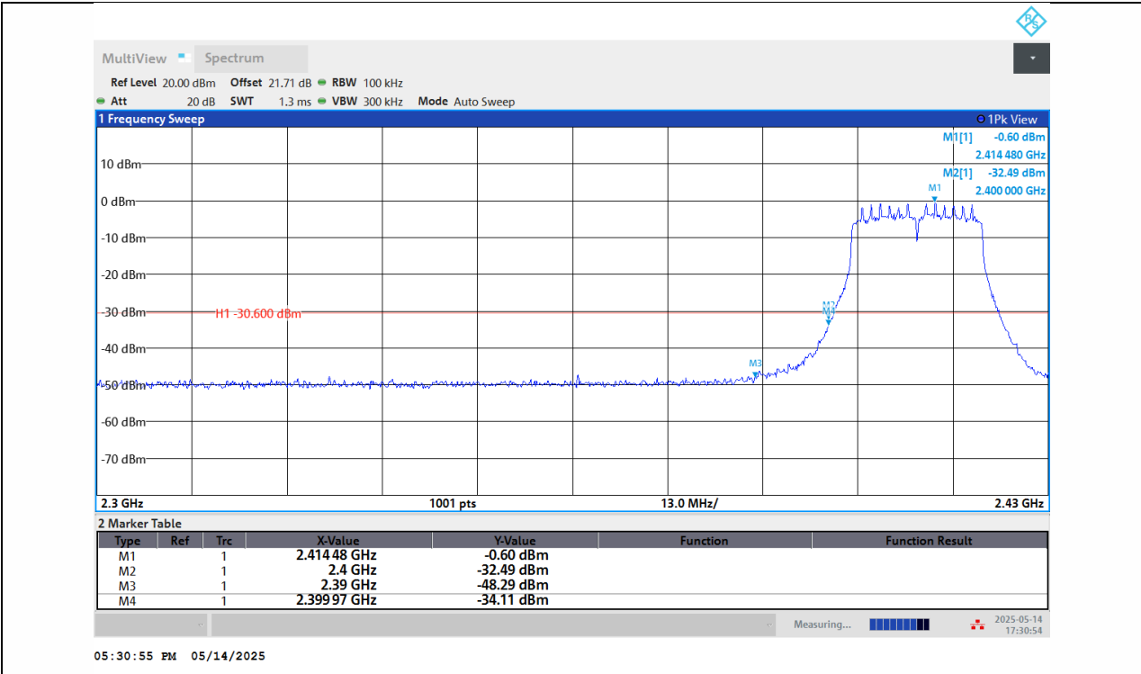
11N20SISO-Ant1-2412-PASS
