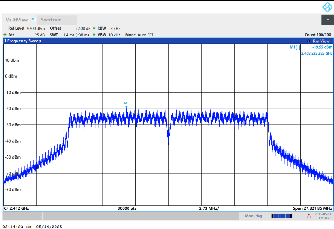
11G-Ant1-2412-PASS
