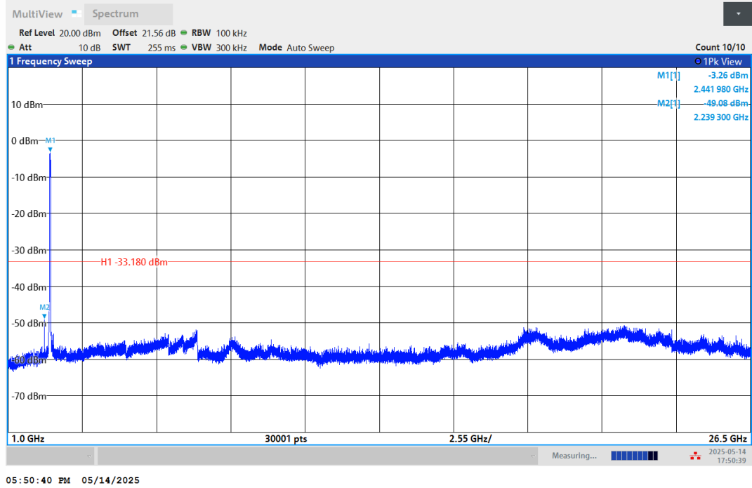
11N40SISO-Ant1-2437-1000~26500-PASS
