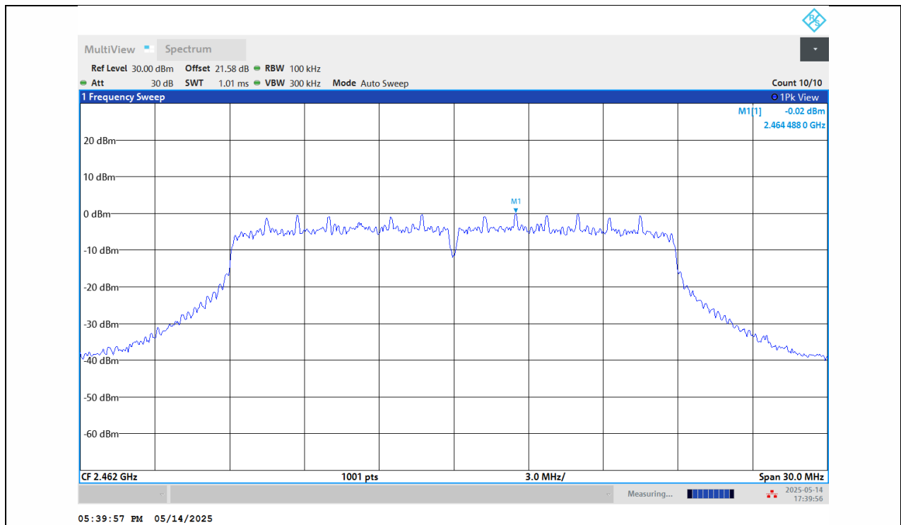
11N20SISO-Ant1-2462-0~Reference-PASS
