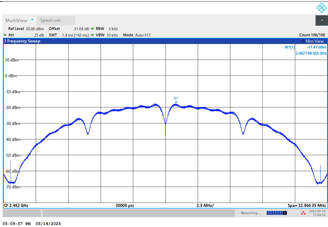
11B-Ant1-2462-PASS
