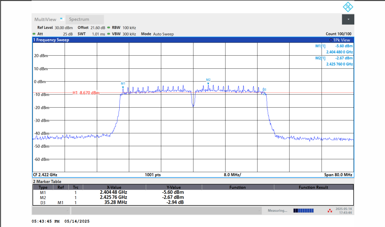
11N40SISO-Ant1-2422-PASS
