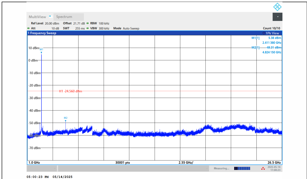
11B-Ant1-2412-1000~26500-PASS
