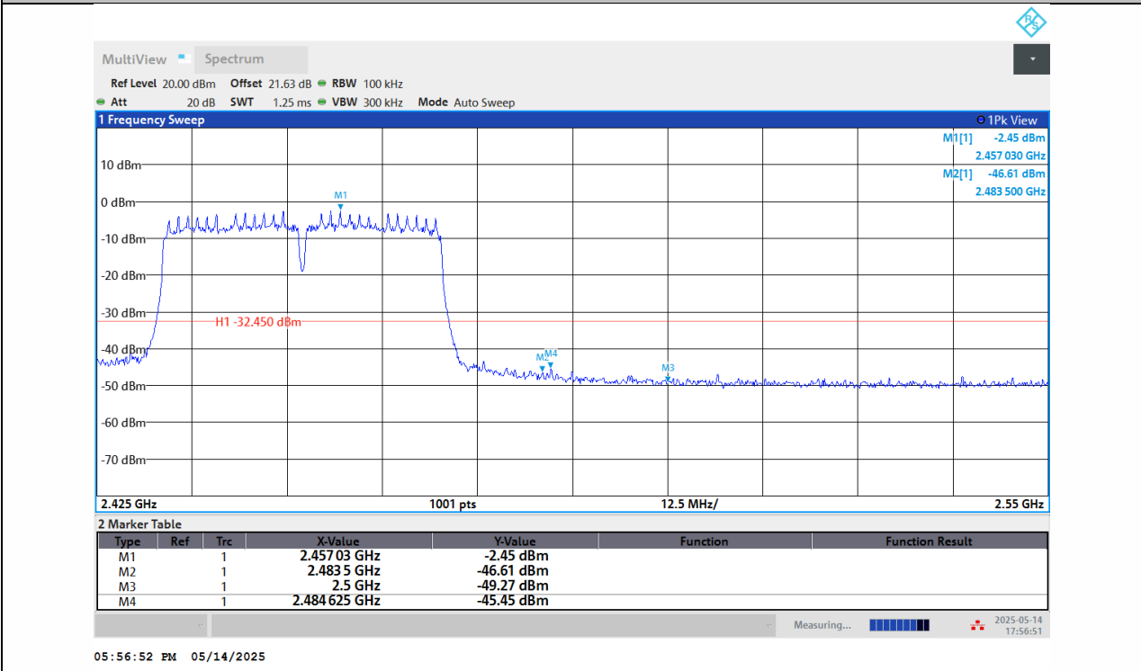
11N40SISO-Ant1-2452-PASS
