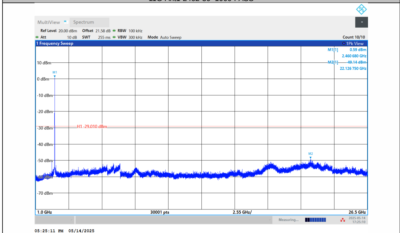
11G-Ant1-2462-1000~26500-PASS
