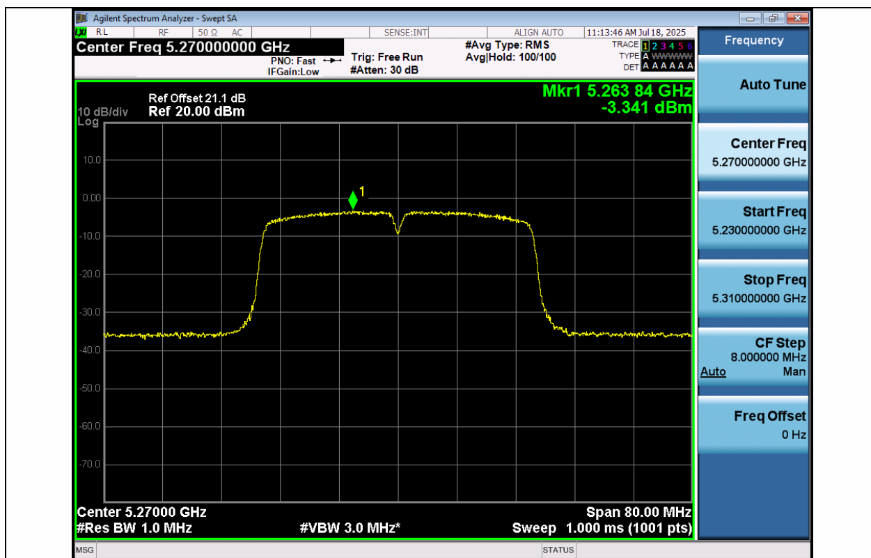
11N40MIMO-Ant1-5270-PASS
