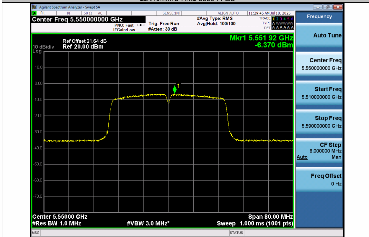
11N40MIMO-Ant2-5550-PASS
