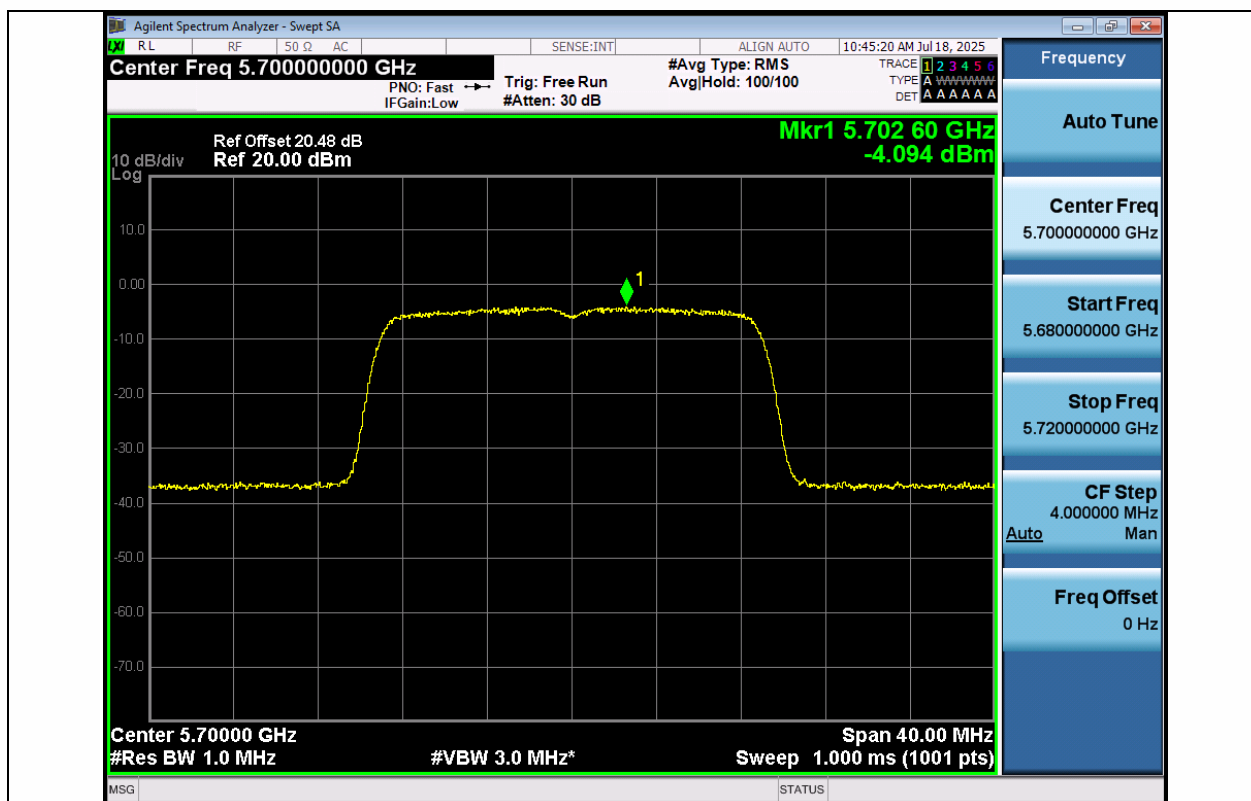
11N20MIMO-Ant1-5700-PASS
