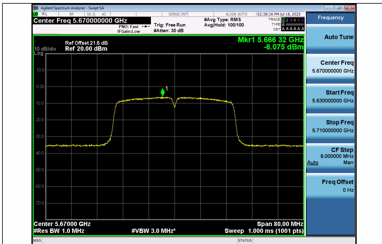
11AC40MIMO-Ant1-5670-PASS
