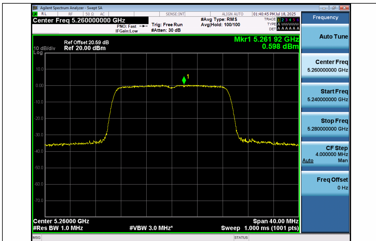
11AC20MIMO-Ant1-5260-PASS
