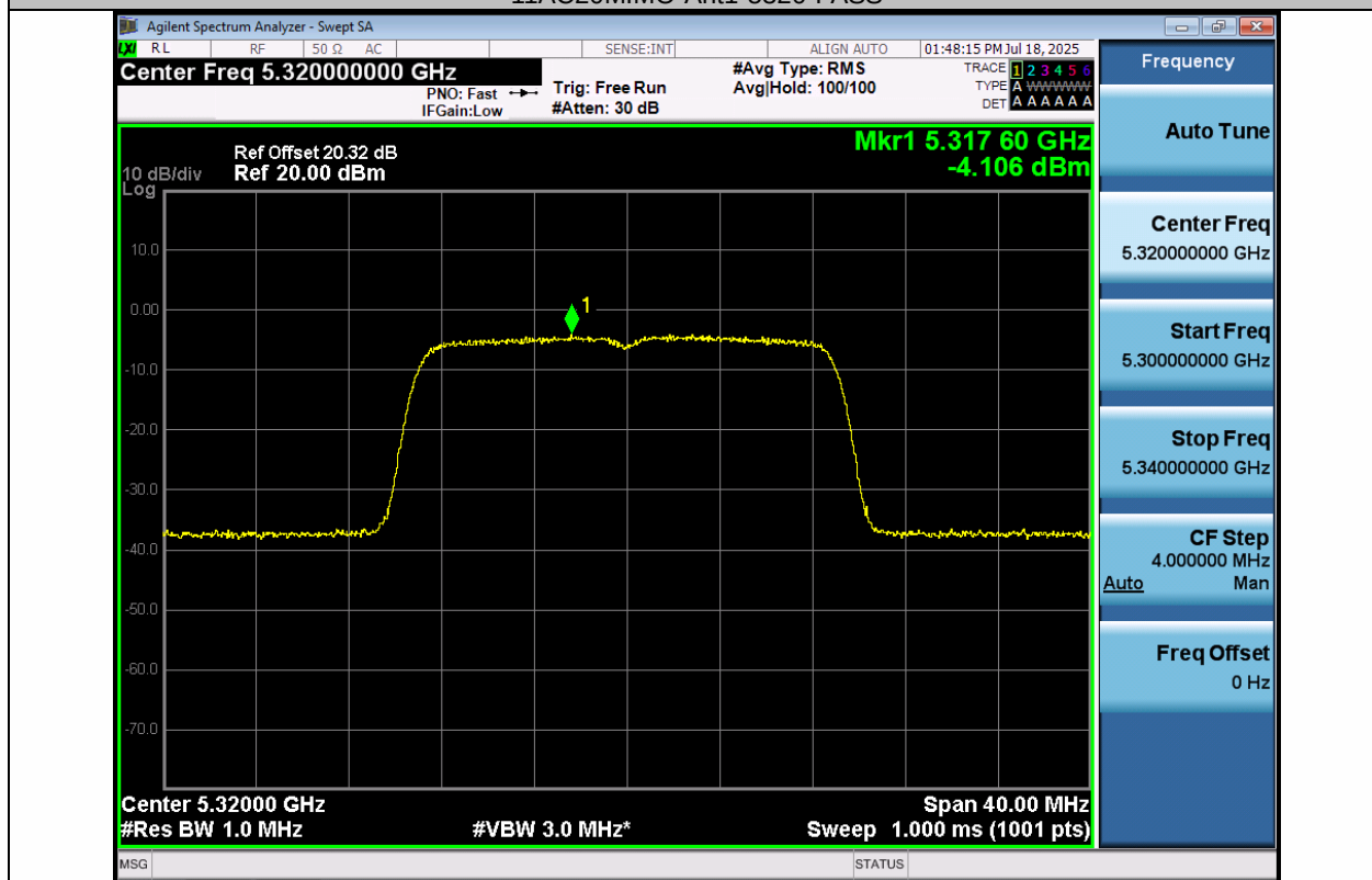
11AC20MIMO-Ant2-5320-PASS
