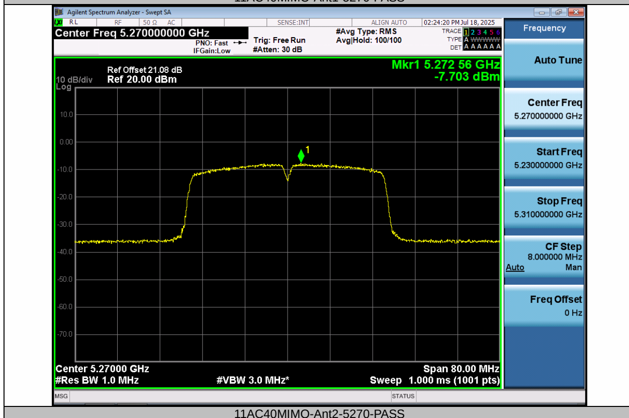
11AC40MIMO-Ant2-5270-PASS
