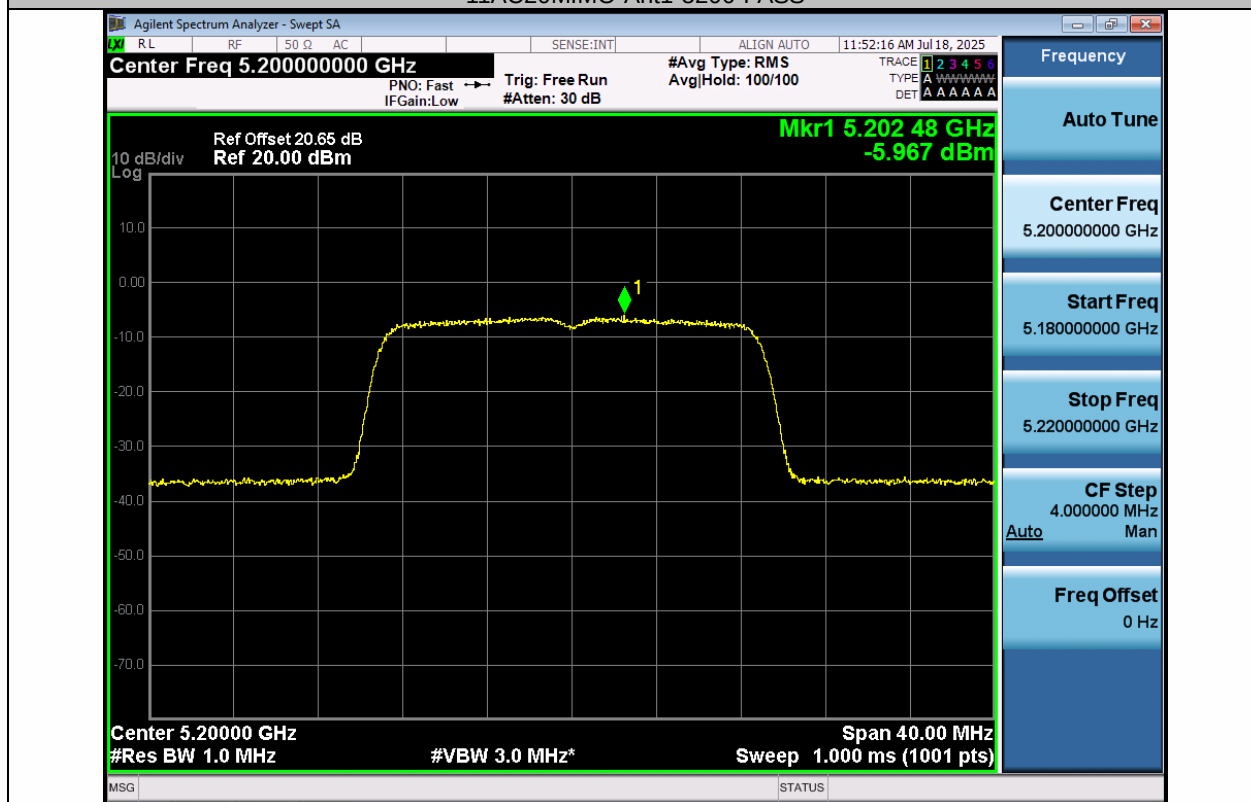
11AC20MIMO-Ant2-5200-PASS
