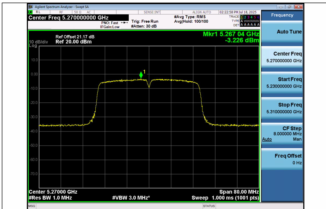
11AC40MIMO-Ant1-5270-PASS
