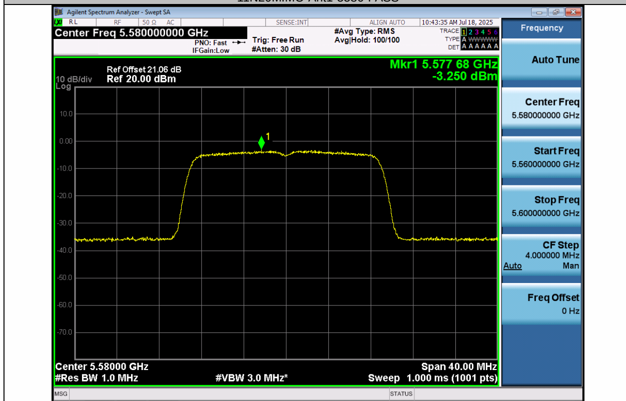
11N20MIMO-Ant2-5580-PASS
