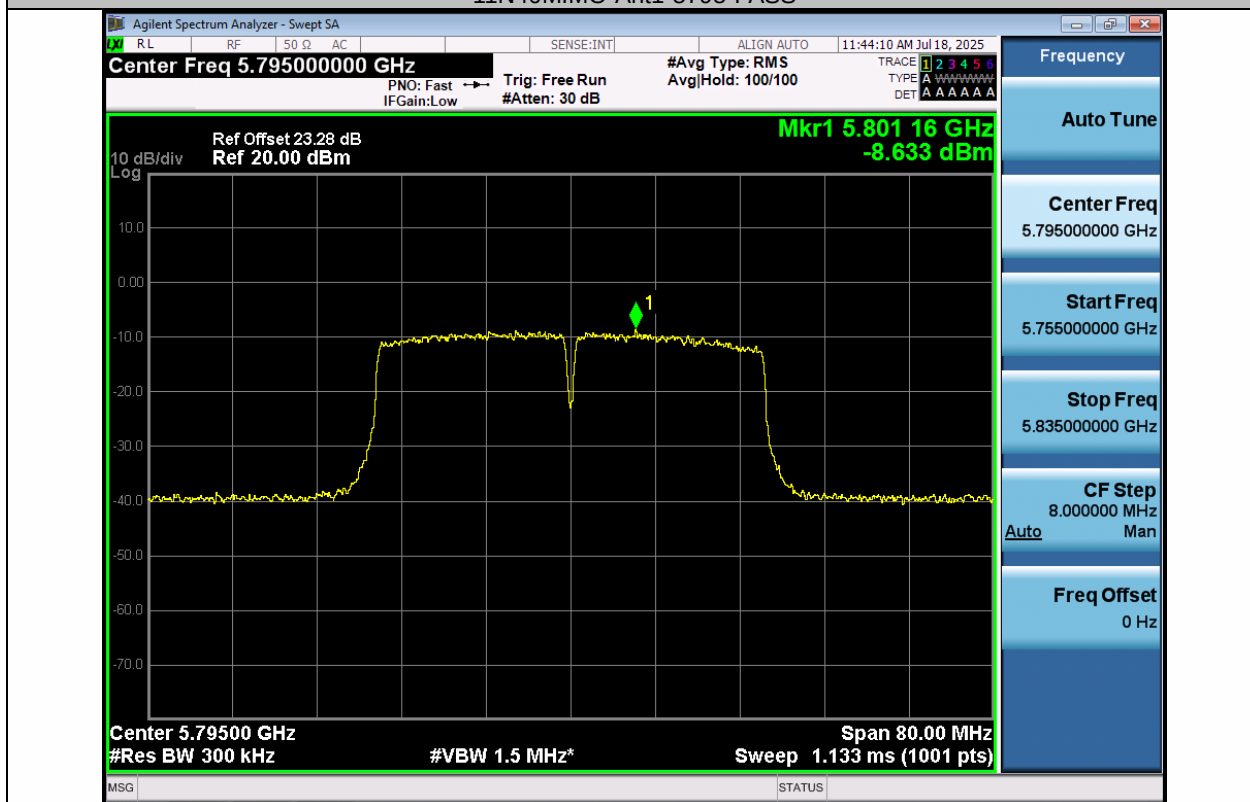
11N40MIMO-Ant2-5795-PASS
