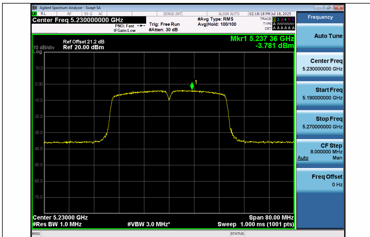
11AC40MIMO-Ant1-5230-PASS
