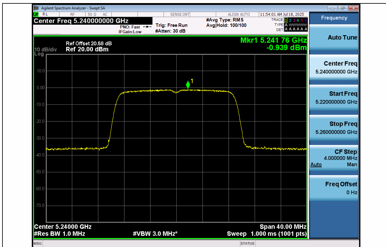
11AC20MIMO-Ant1-5240-PASS
