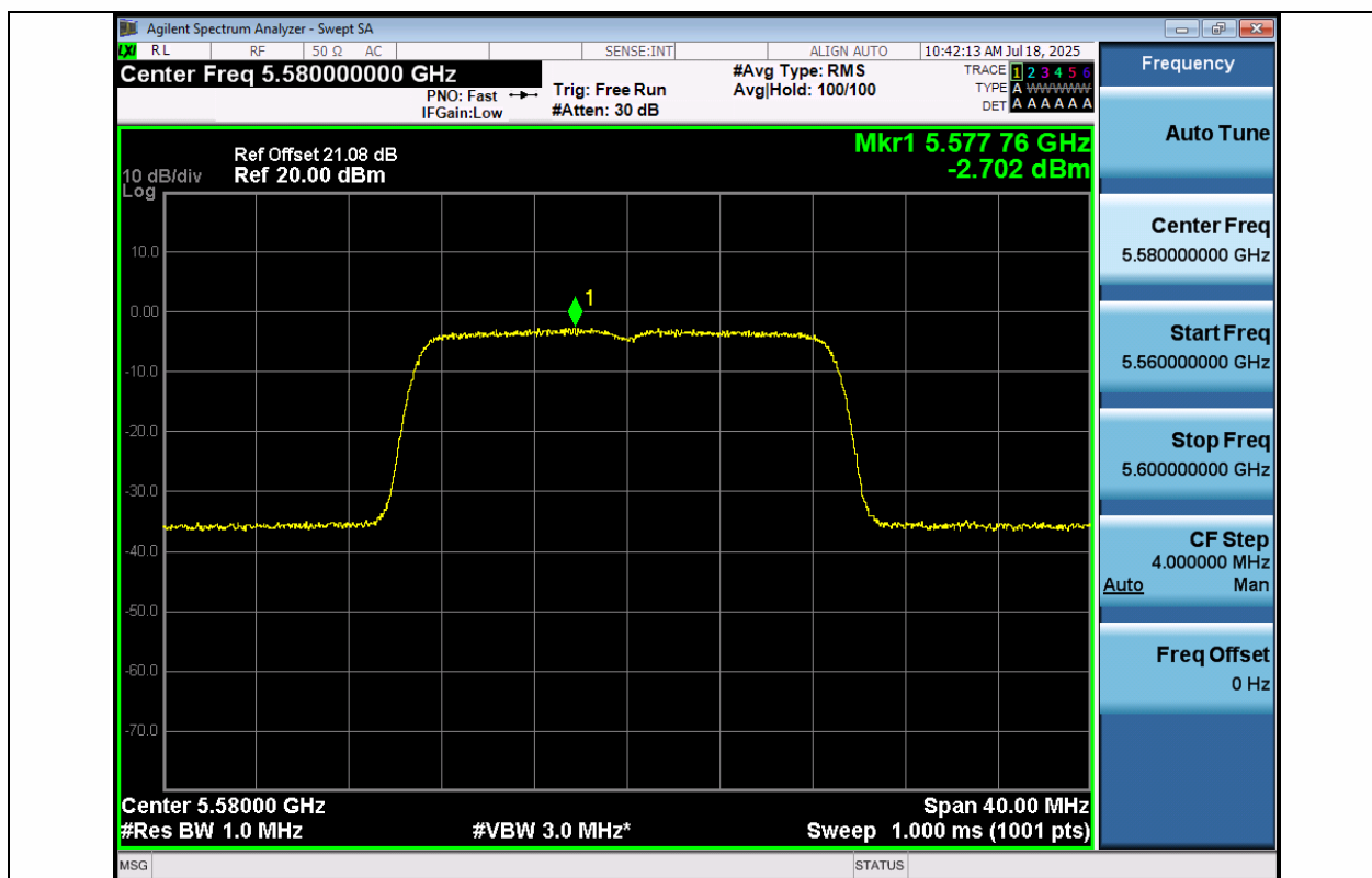
11N20MIMO-Ant1-5580-PASS
