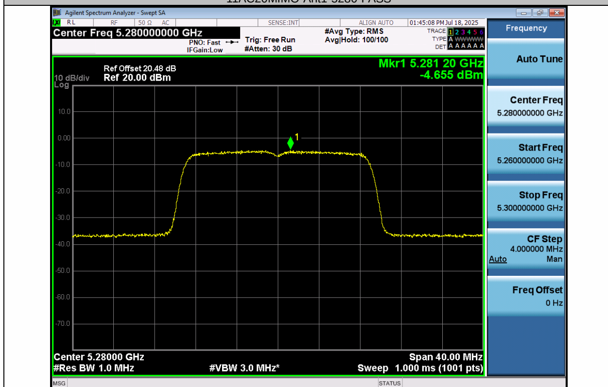
11AC20MIMO-Ant2-5280-PASS
