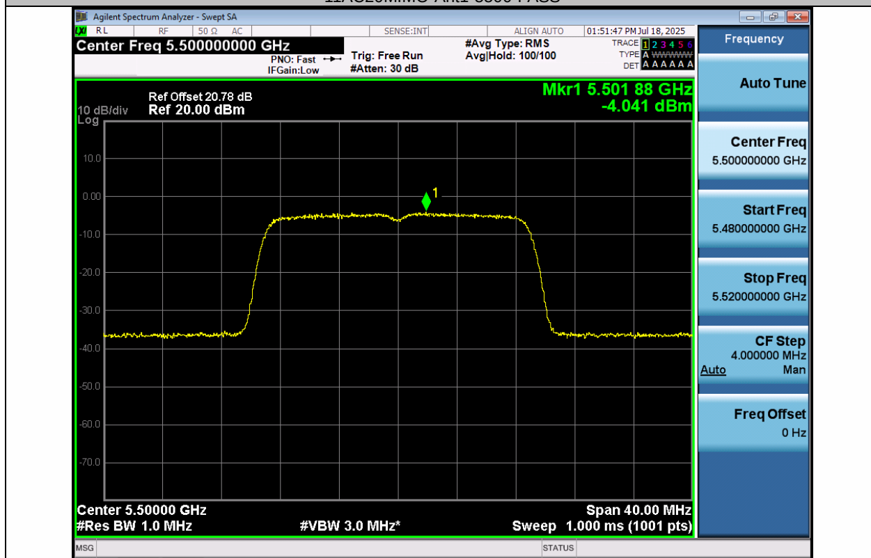
11AC20MIMO-Ant2-5500-PASS
