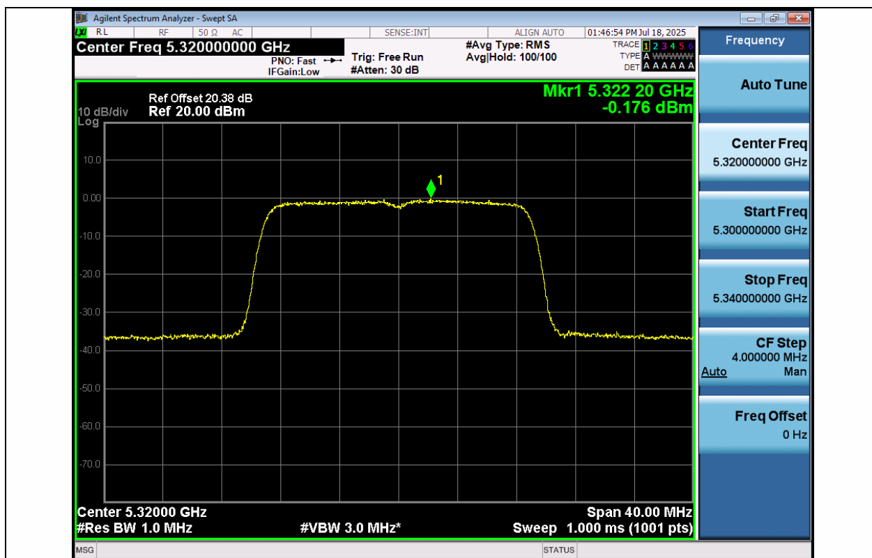
11AC20MIMO-Ant1-5320-PASS
