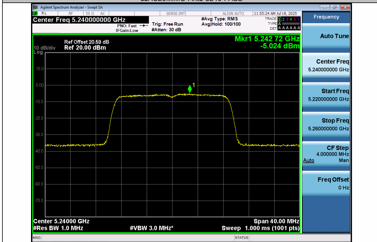
11AC20MIMO-Ant2-5240-PASS
