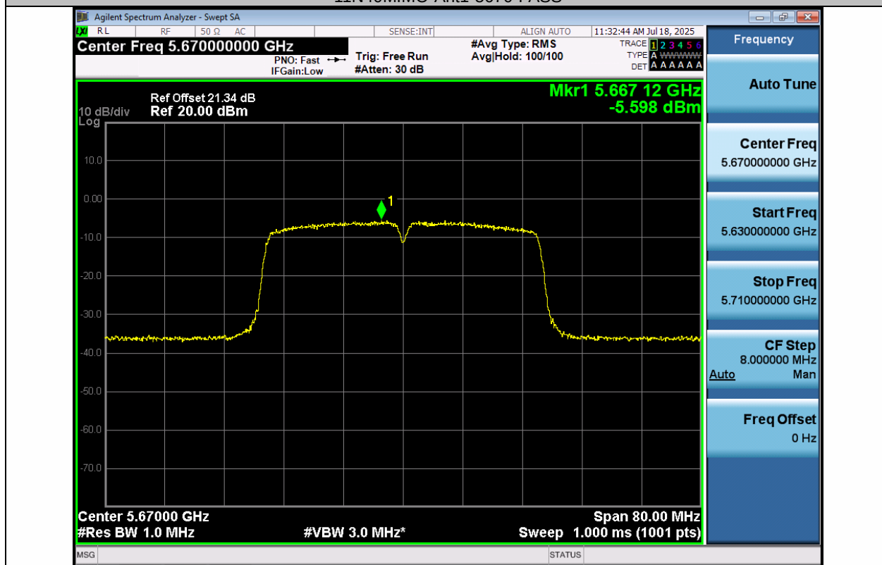
11N40MIMO-Ant2-5670-PASS
