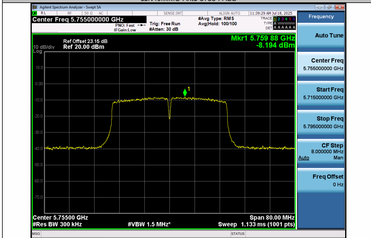
11N40MIMO-Ant2-5755-PASS
