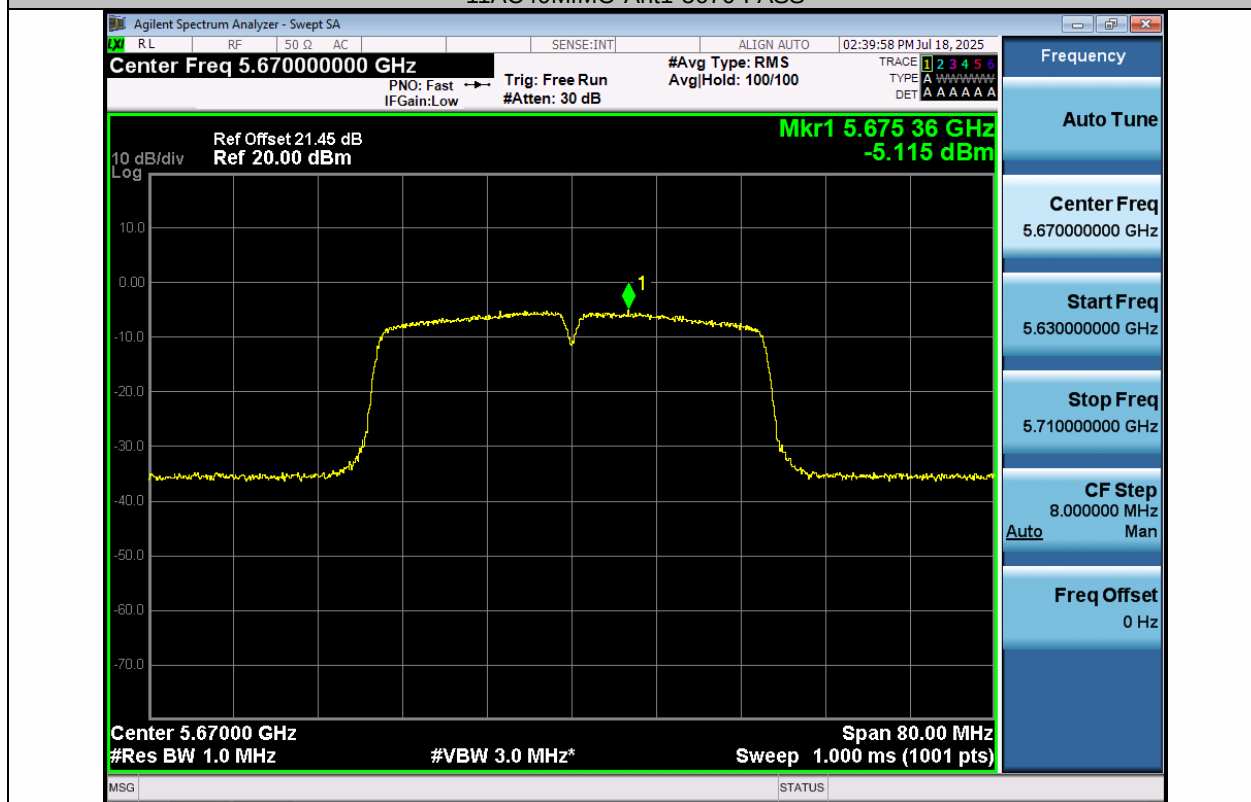
11AC40MIMO-Ant2-5670-PASS
