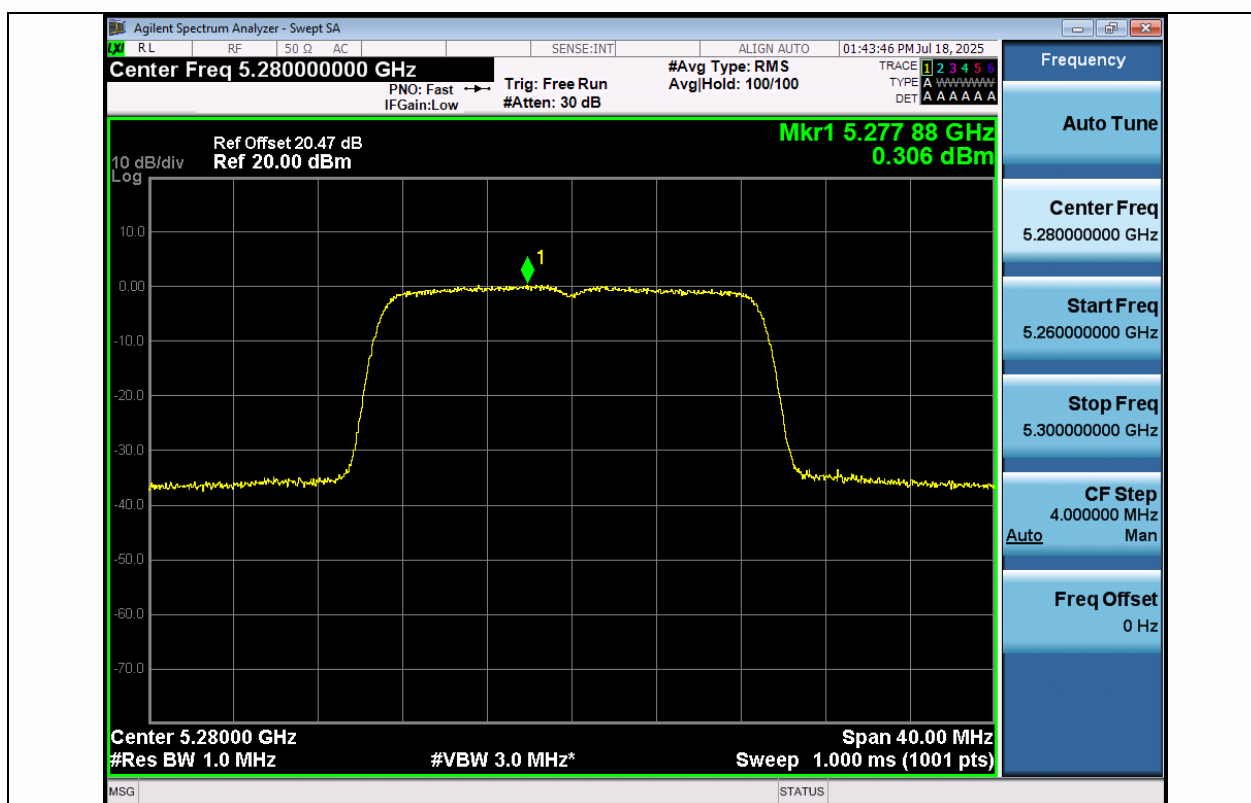
11AC20MIMO-Ant1-5280-PASS
