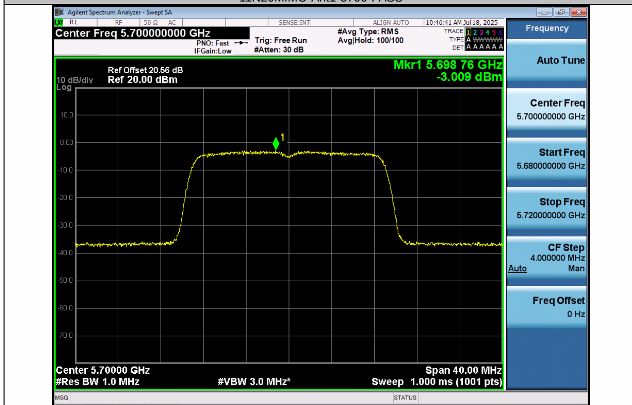
11N20MIMO-Ant2-5700-PASS
