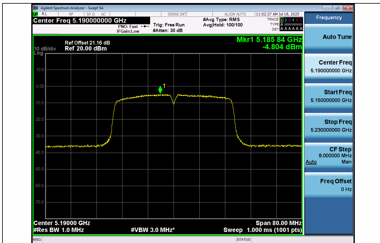
11N40MIMO-Ant1-5190-PASS
