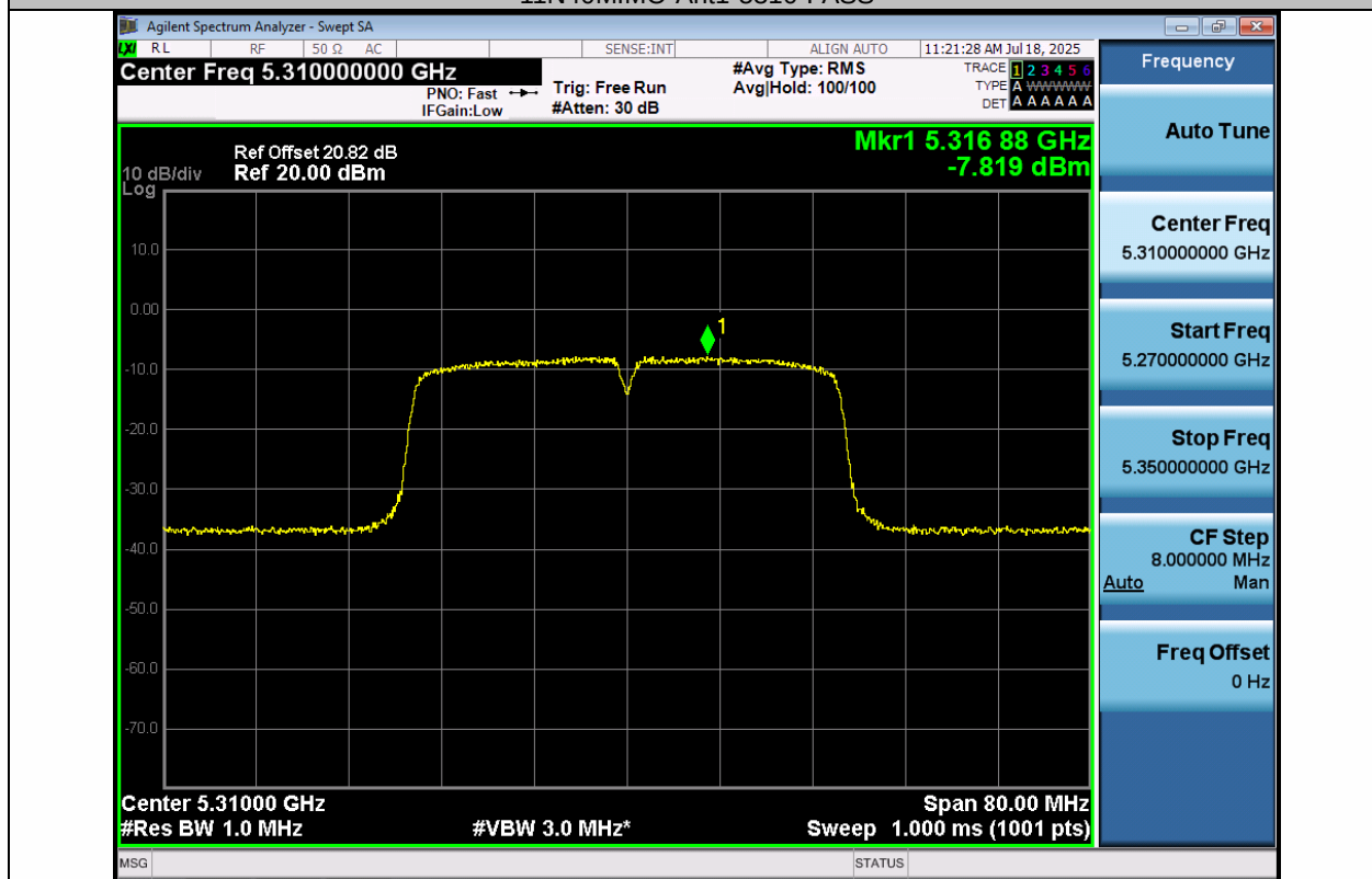
11N40MIMO-Ant2-5310-PASS
