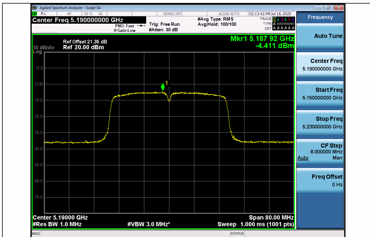
11AC40MIMO-Ant1-5190-PASS
