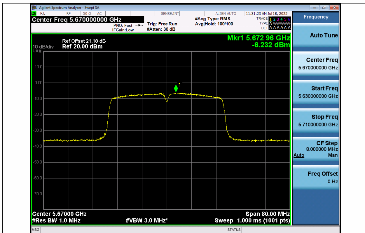
11N40MIMO-Ant1-5670-PASS
