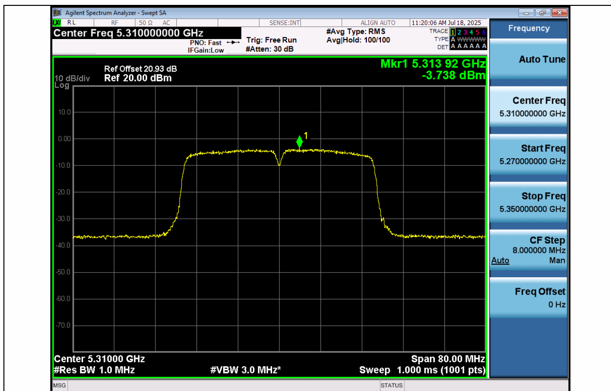
11N40MIMO-Ant1-5310-PASS
