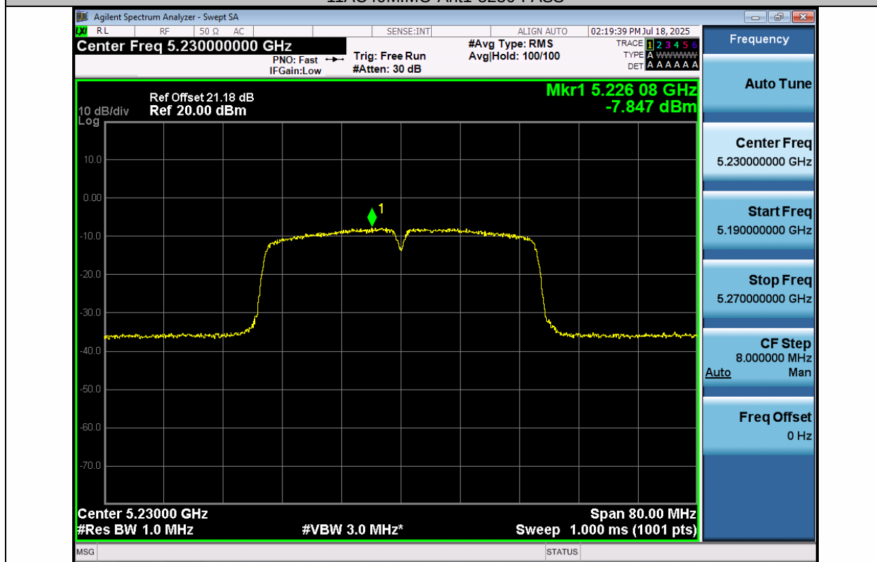
11AC40MIMO-Ant2-5230-PASS
