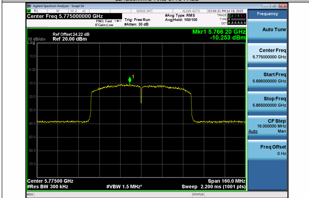
11AC80MIMO-Ant2-5775-PASS
