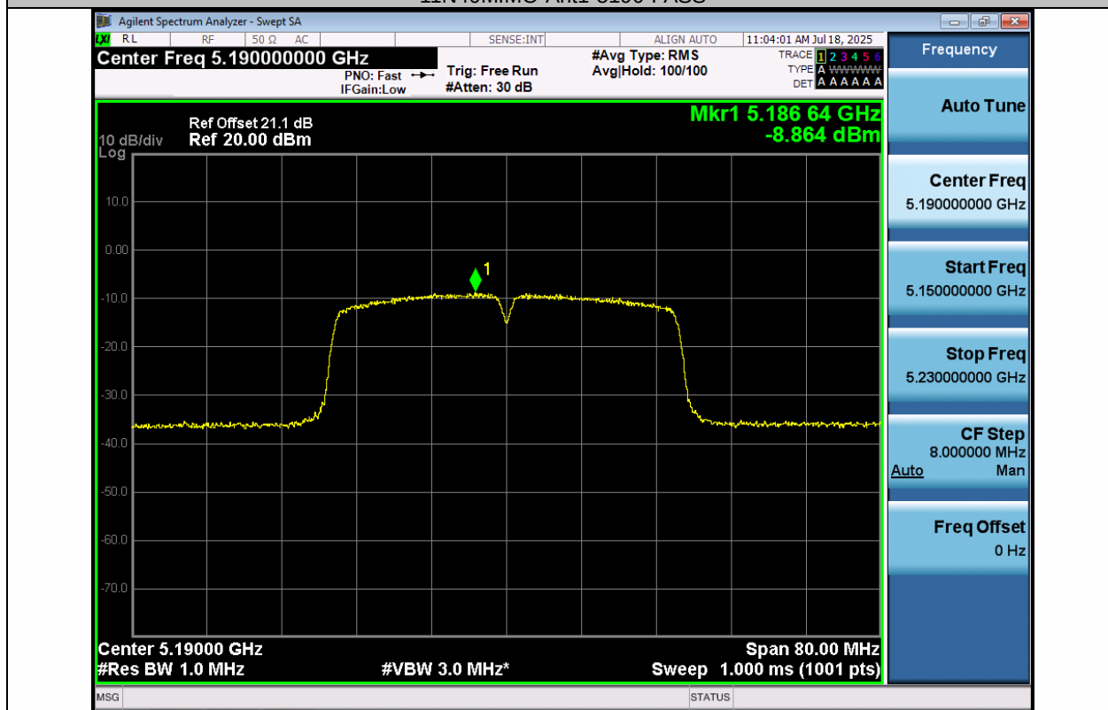
11N40MIMO-Ant2-5190-PASS
