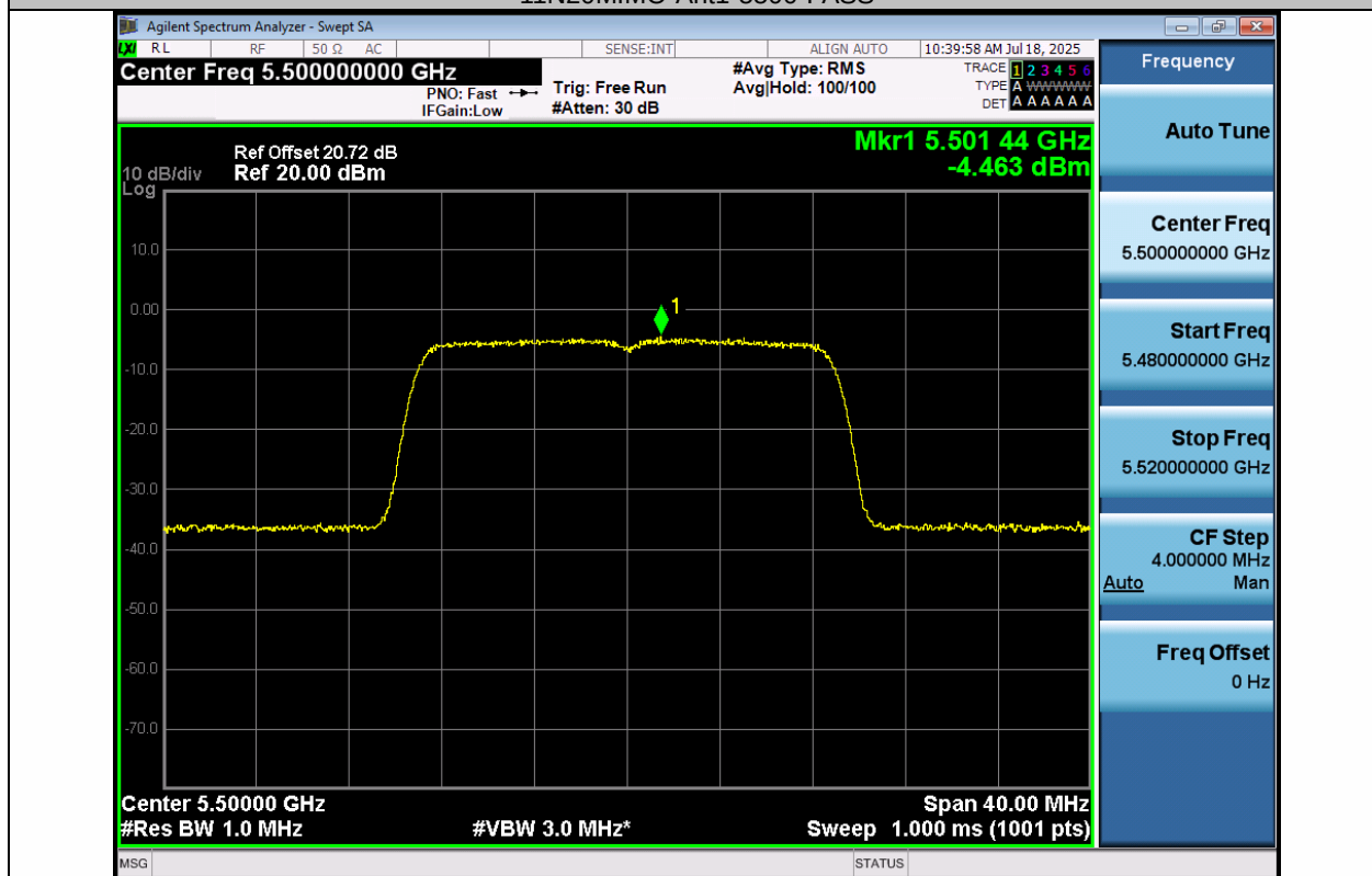
11N20MIMO-Ant2-5500-PASS
