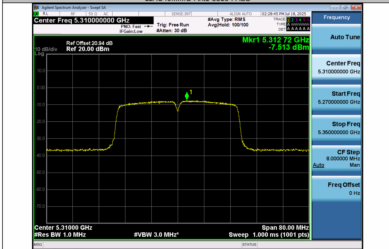
11AC40MIMO-Ant2-5310-PASS
