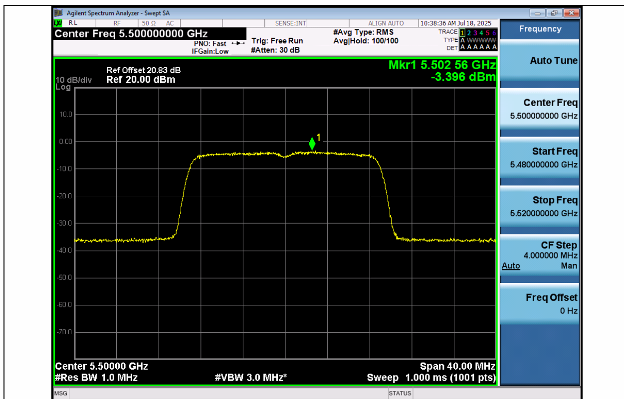
11N20MIMO-Ant1-5500-PASS
