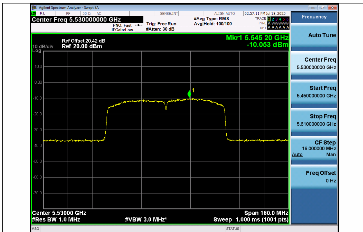
11AC80MIMO-Ant1-5530-PASS
