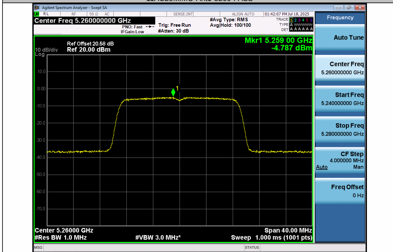
11AC20MIMO-Ant2-5260-PASS
