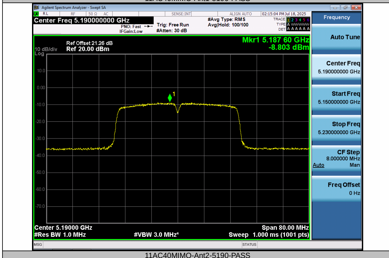
11AC40MIMO-Ant2-5190-PASS
