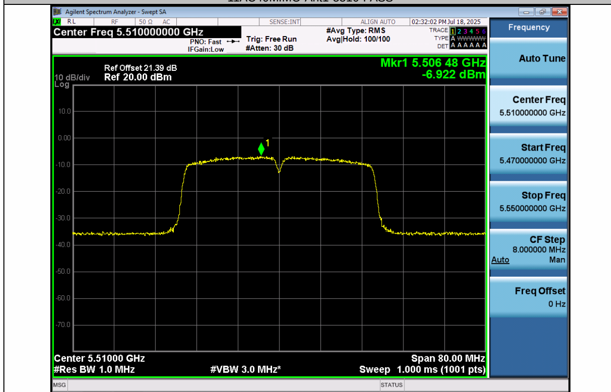
11AC40MIMO-Ant2-5510-PASS
