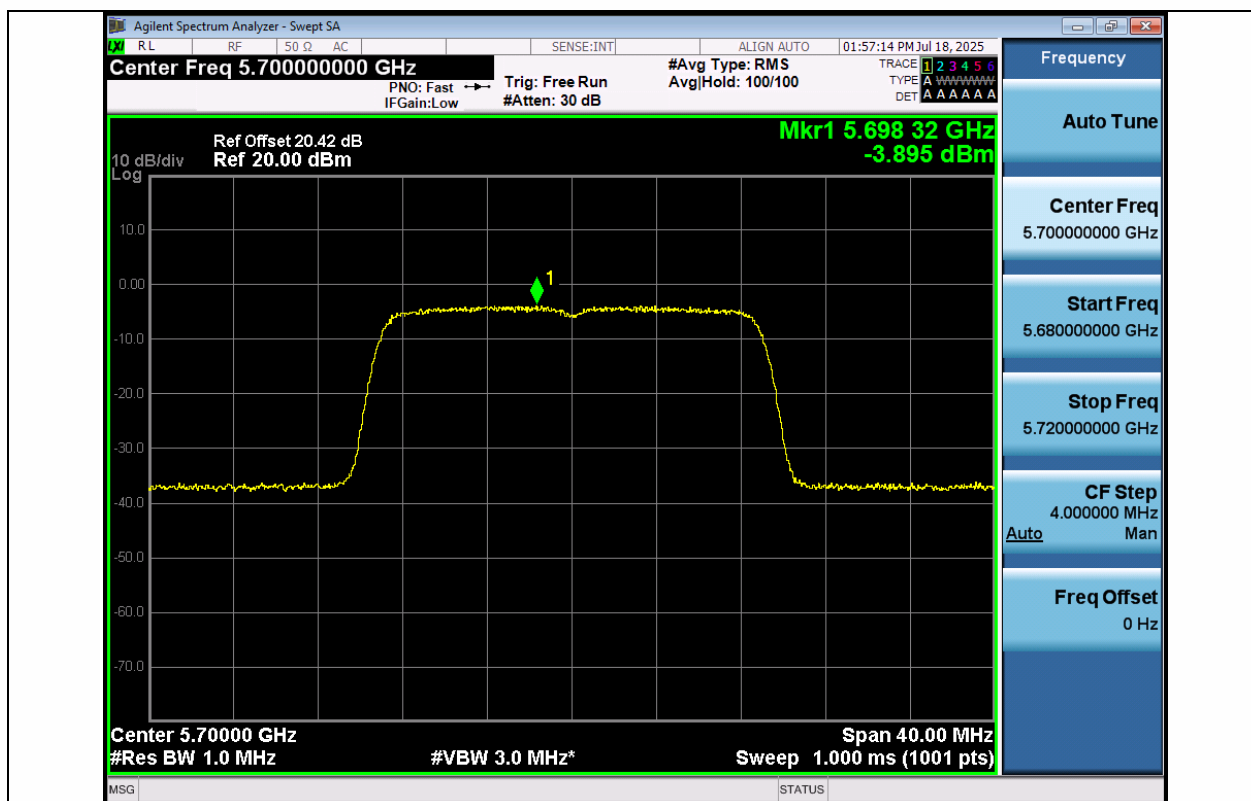
11AC20MIMO-Ant1-5700-PASS
