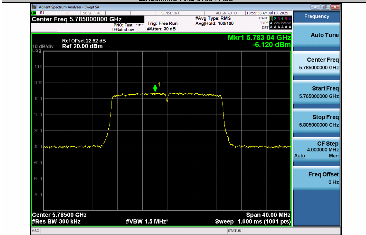
11N20MIMO-Ant2-5785-PASS
