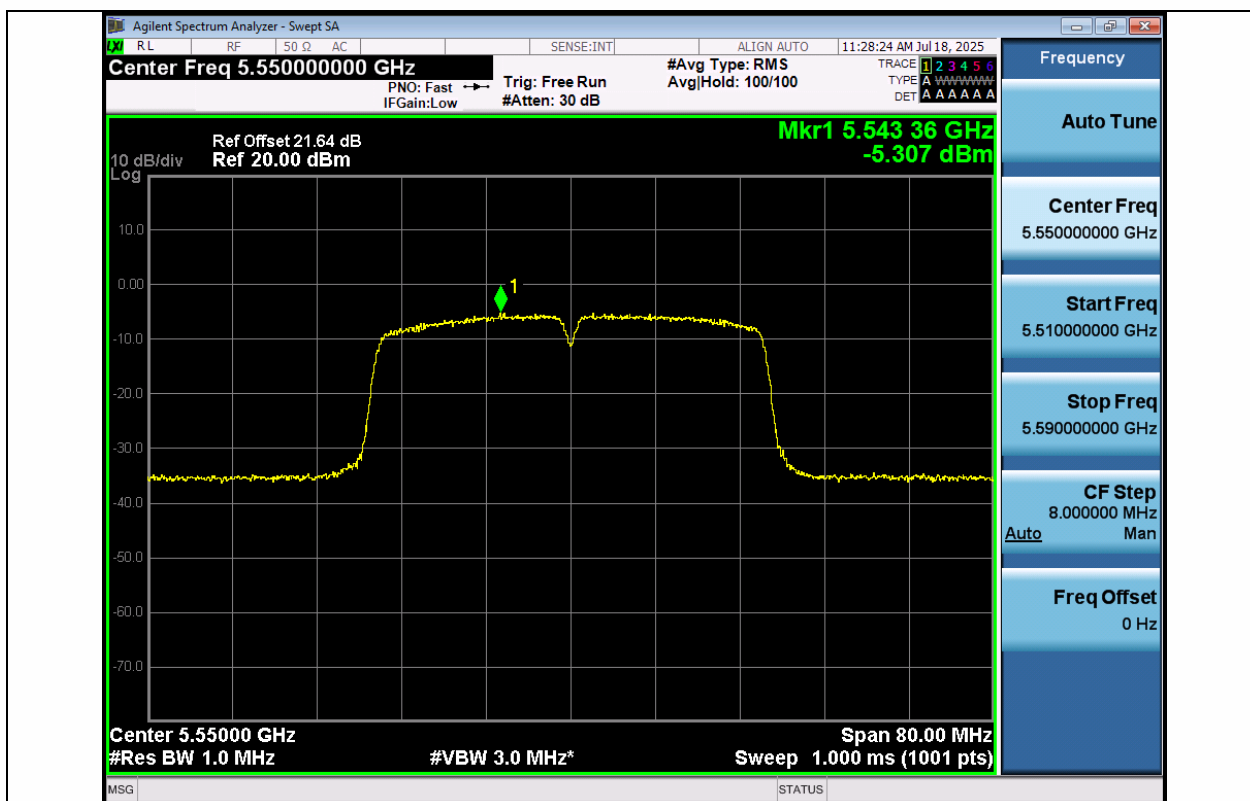
11N40MIMO-Ant1-5550-PASS
