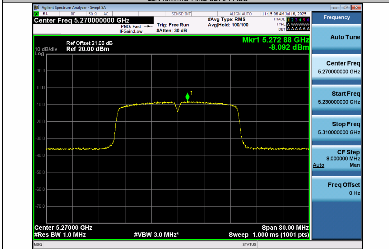
11N40MIMO-Ant2-5270-PASS
