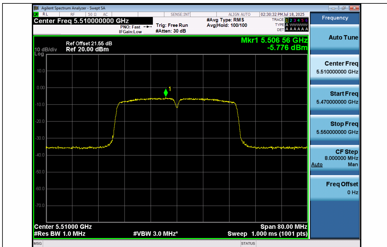
11AC40MIMO-Ant1-5510-PASS
