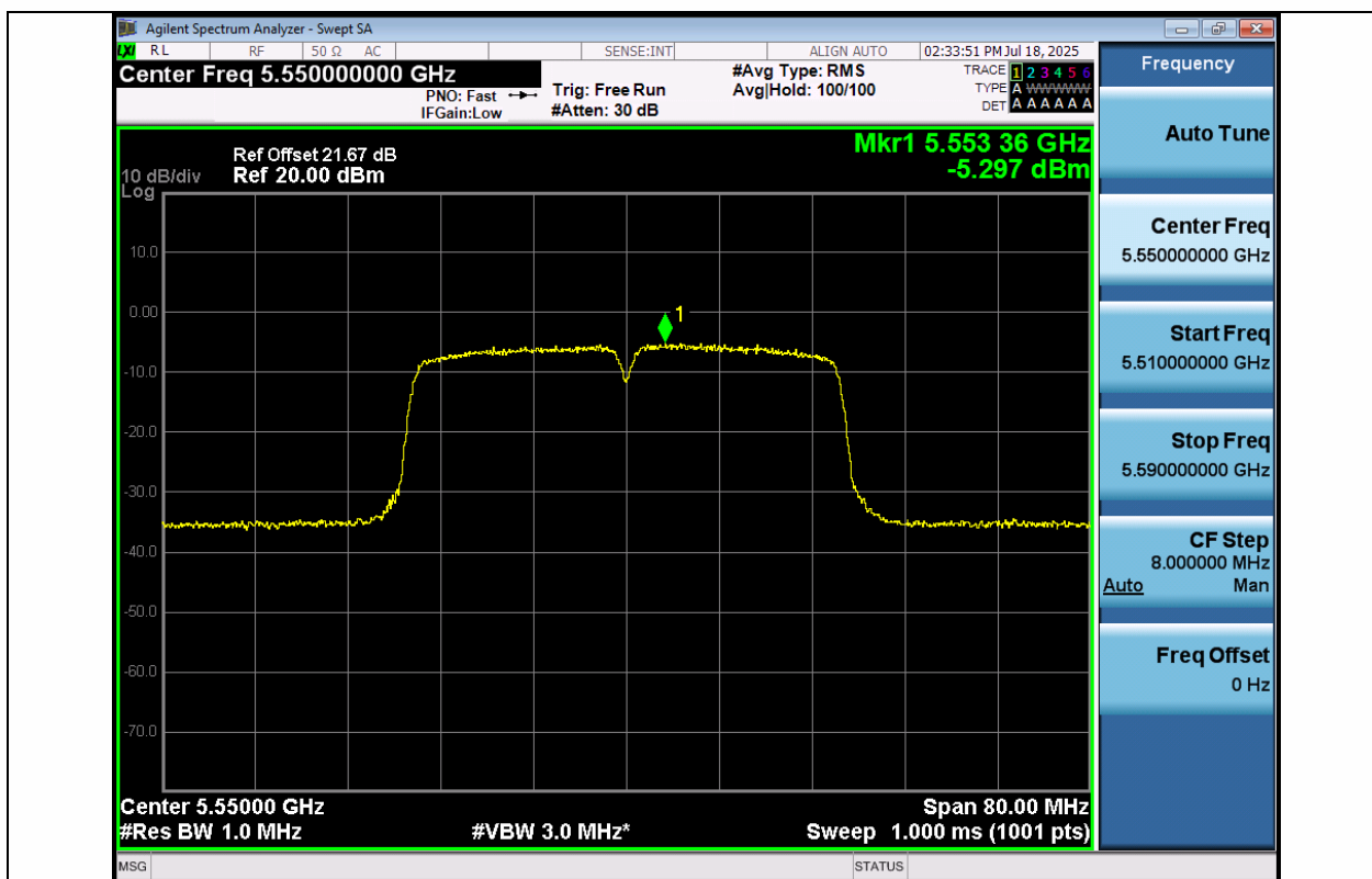
11AC40MIMO-Ant1-5550-PASS
