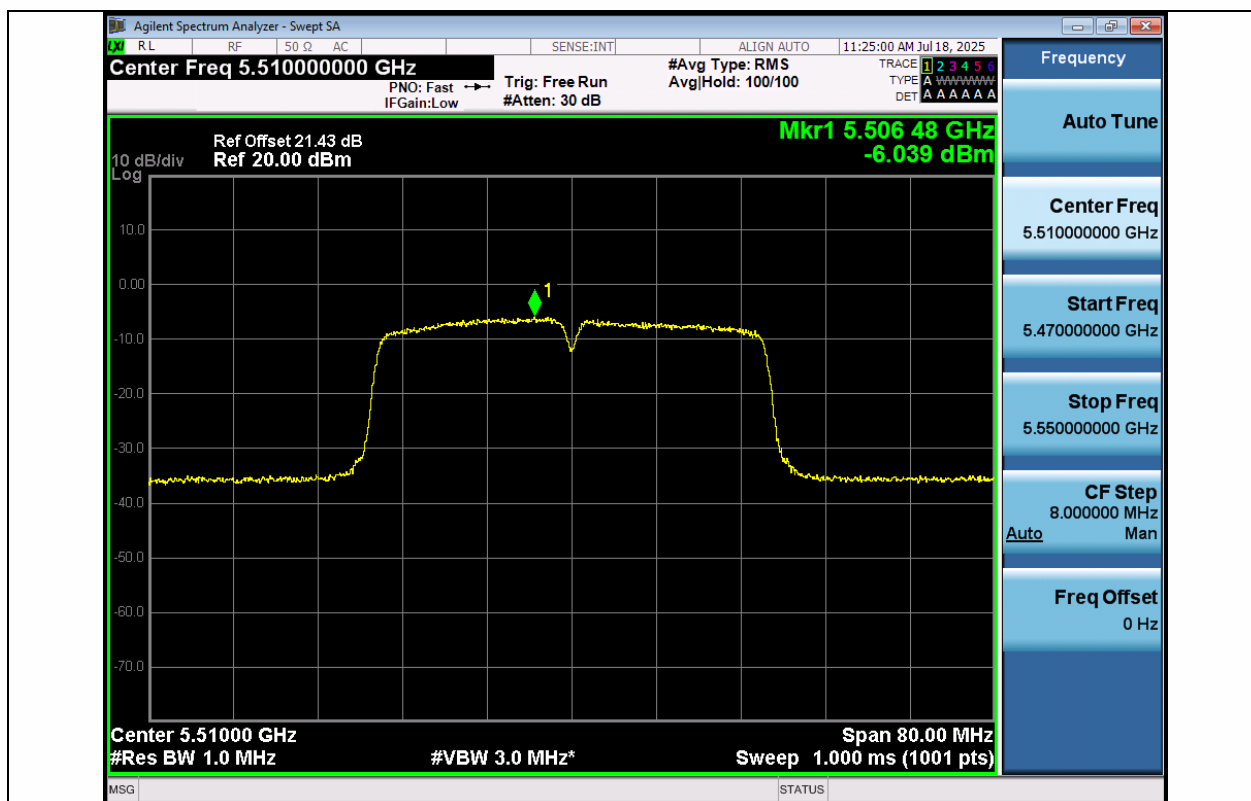
11N40MIMO-Ant1-5510-PASS
