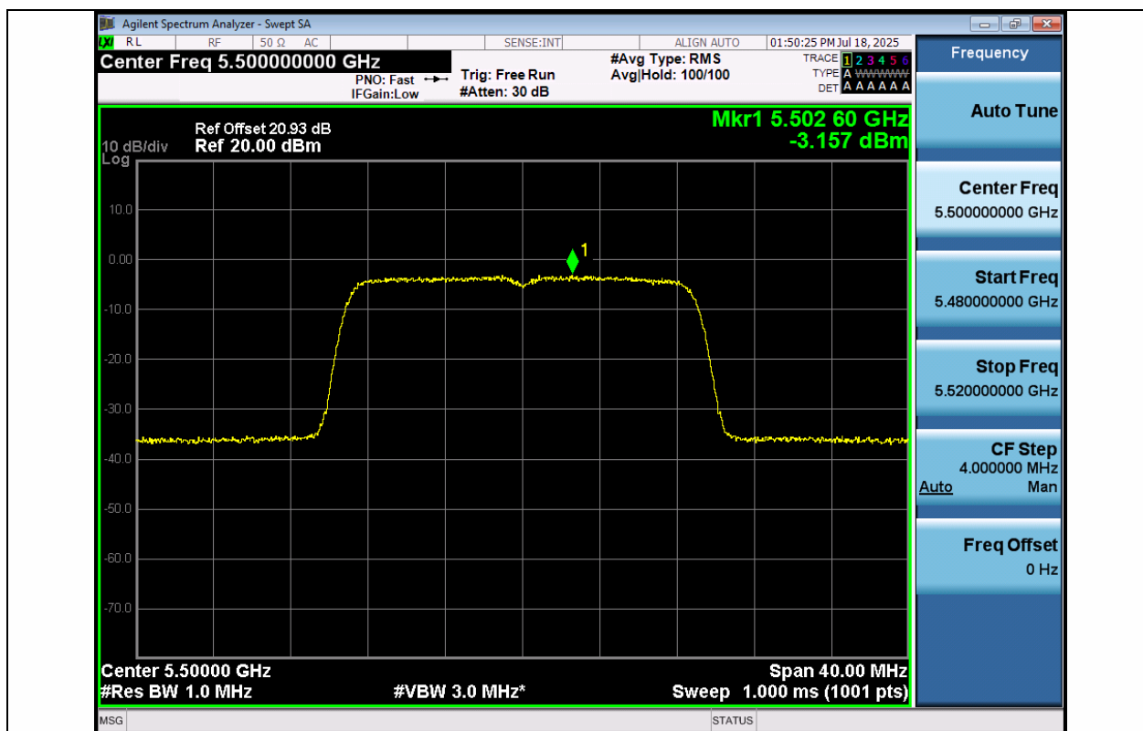
11AC20MIMO-Ant1-5500-PASS
