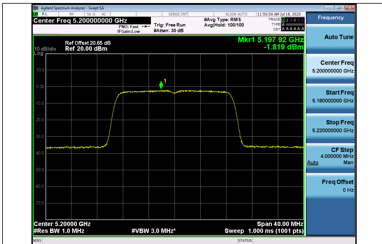
11AC20MIMO-Ant1-5200-PASS
