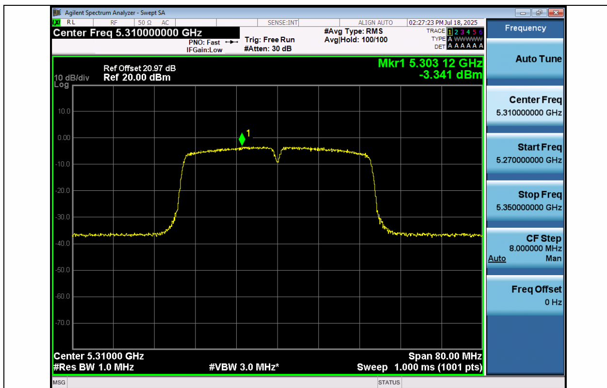
11AC40MIMO-Ant1-5310-PASS
