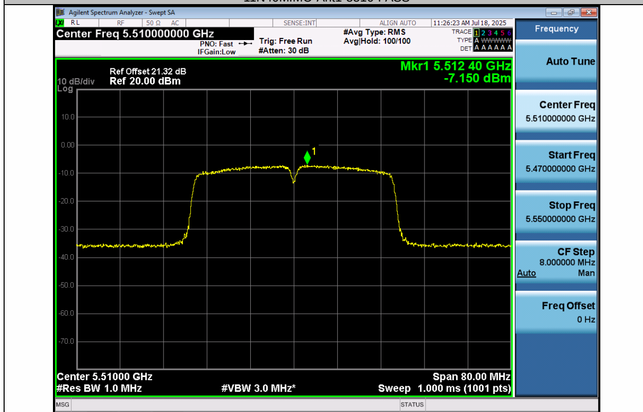
11N40MIMO-Ant2-5510-PASS
