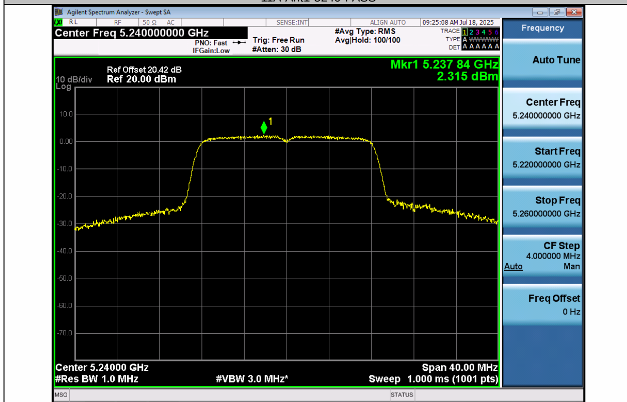
11A-Ant2-5240-PASS
