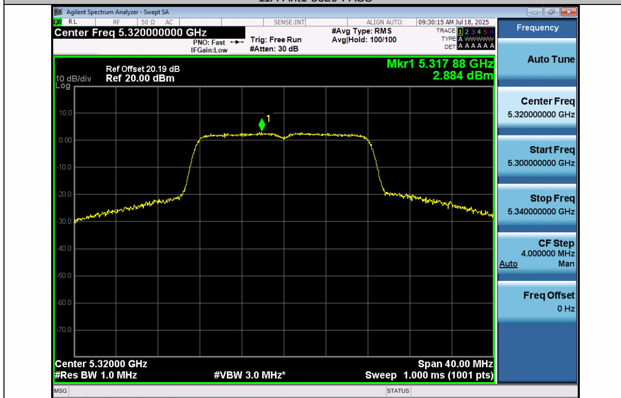
11A-Ant2-5320-PASS
