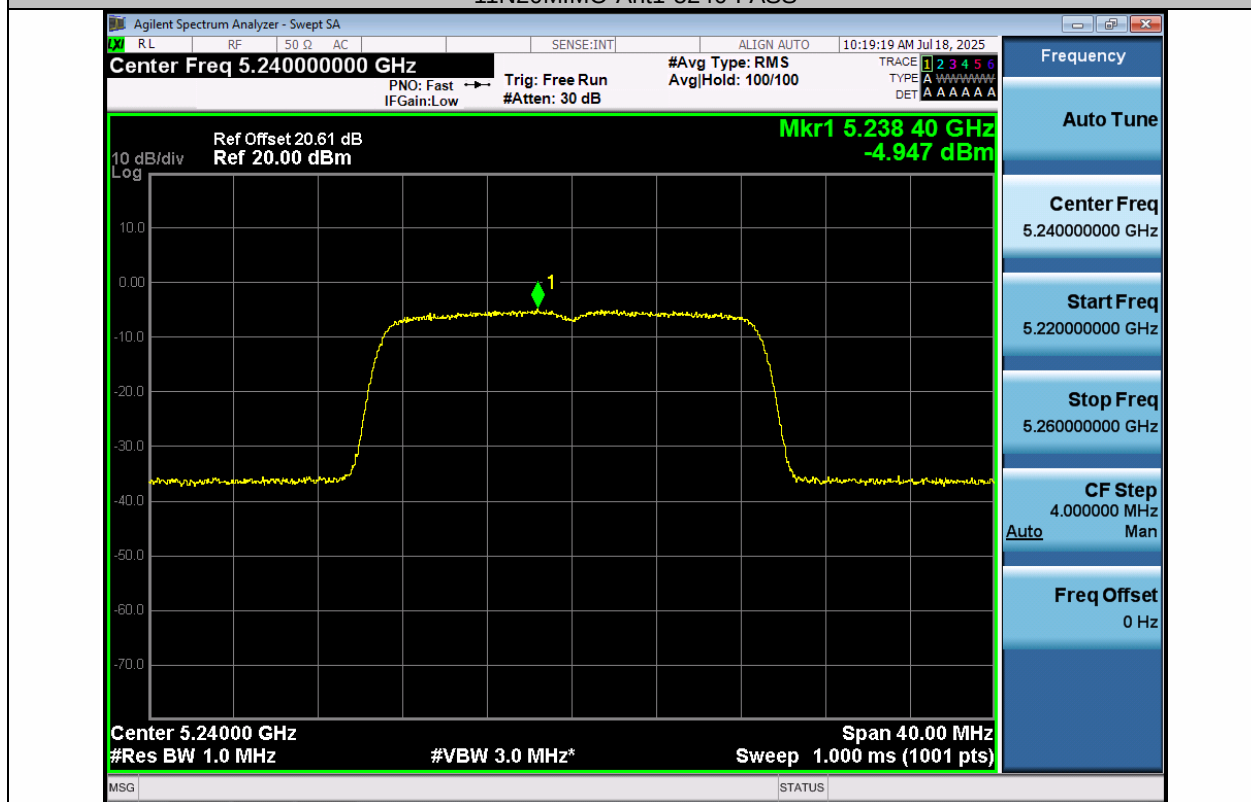
11N20MIMO-Ant2-5240-PASS
