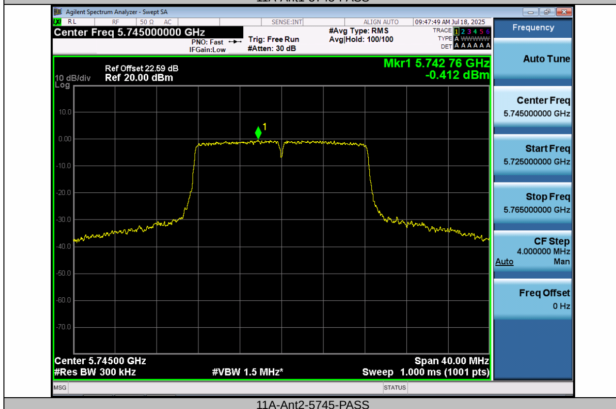
11A-Ant2-5745-PASS
