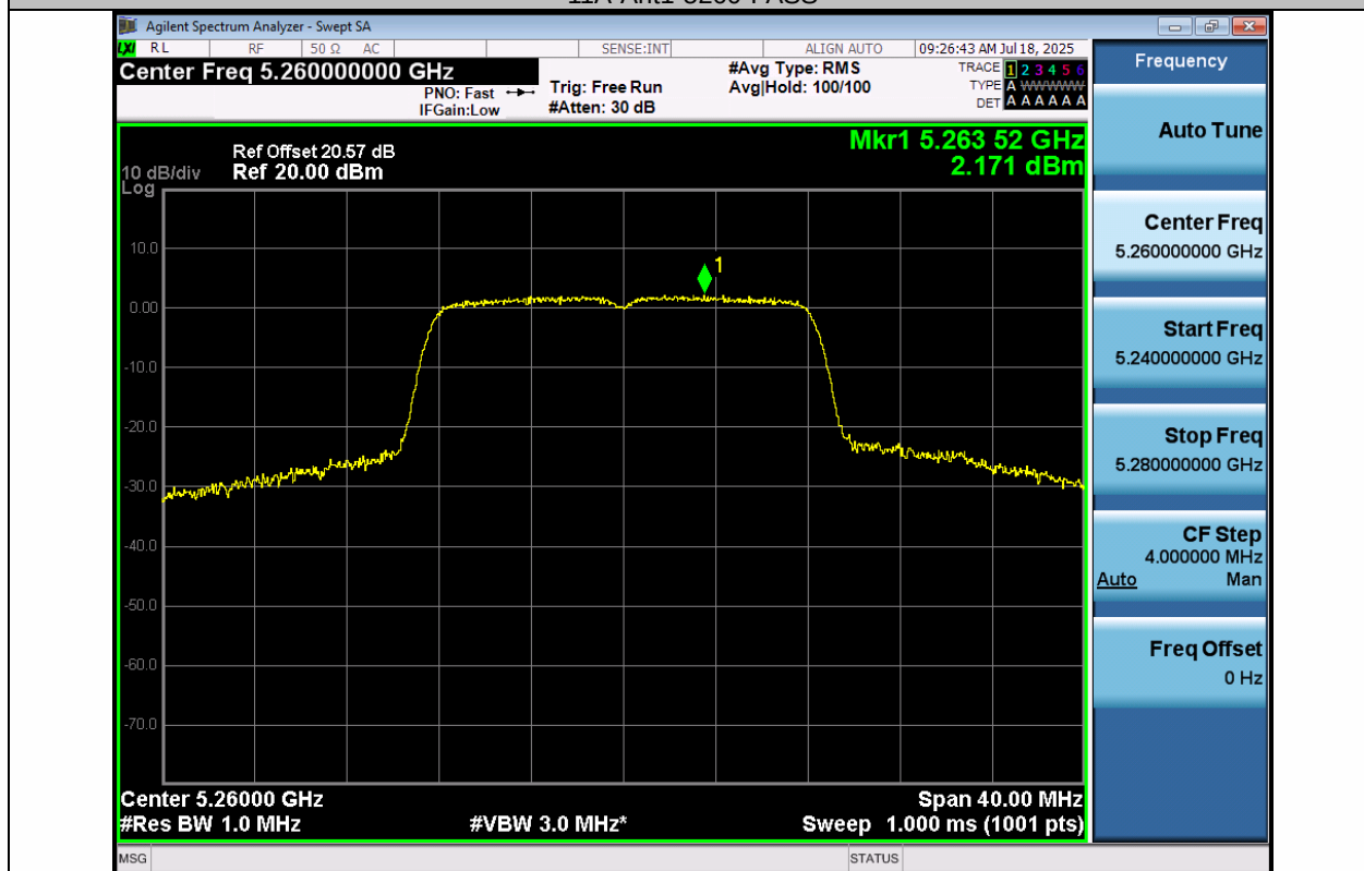
11A-Ant2-5260-PASS
