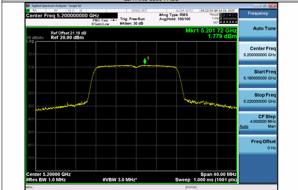
11A-Ant2-5200-PASS
