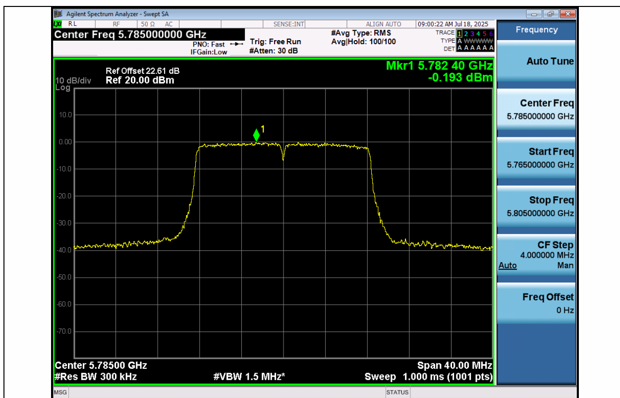
11A-Ant1-5785-PASS
