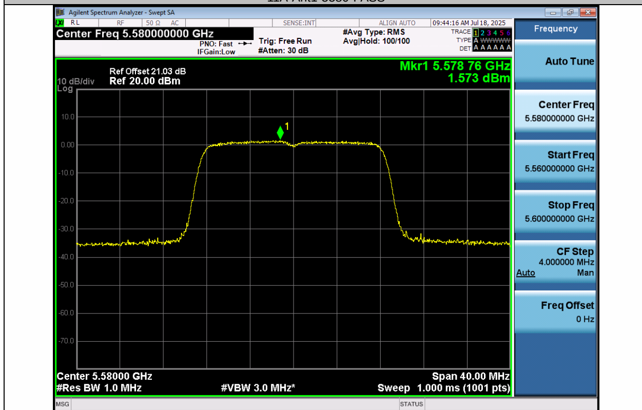
11A-Ant2-5580-PASS
