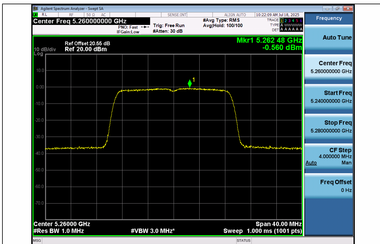
11N20MIMO-Ant1-5260-PASS
