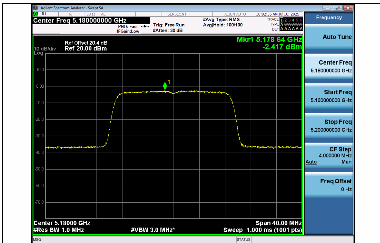
11N20MIMO-Ant1-5180-PASS
