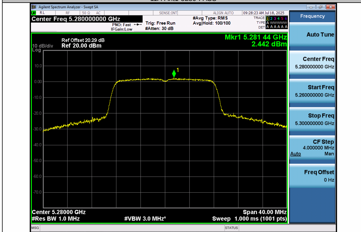
11A-Ant2-5280-PASS
