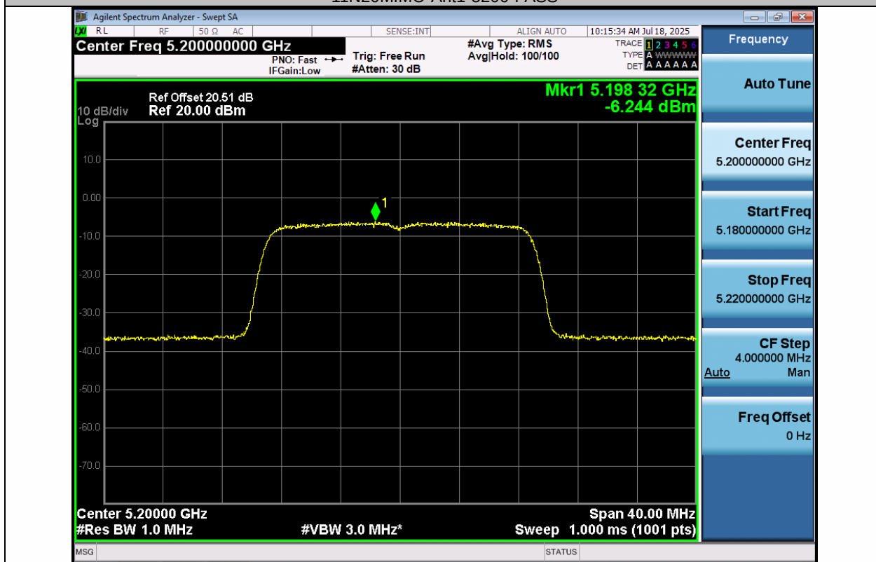
11N20MIMO-Ant2-5200-PASS
