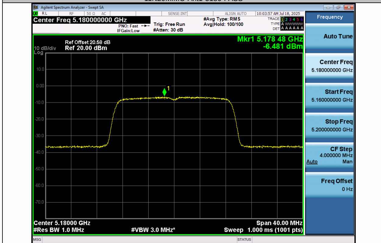
11N20MIMO-Ant2-5180-PASS
