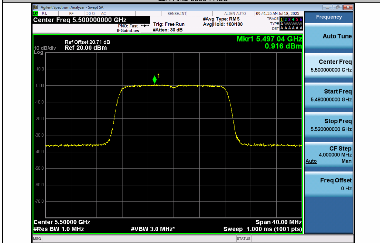
11A-Ant2-5500-PASS
