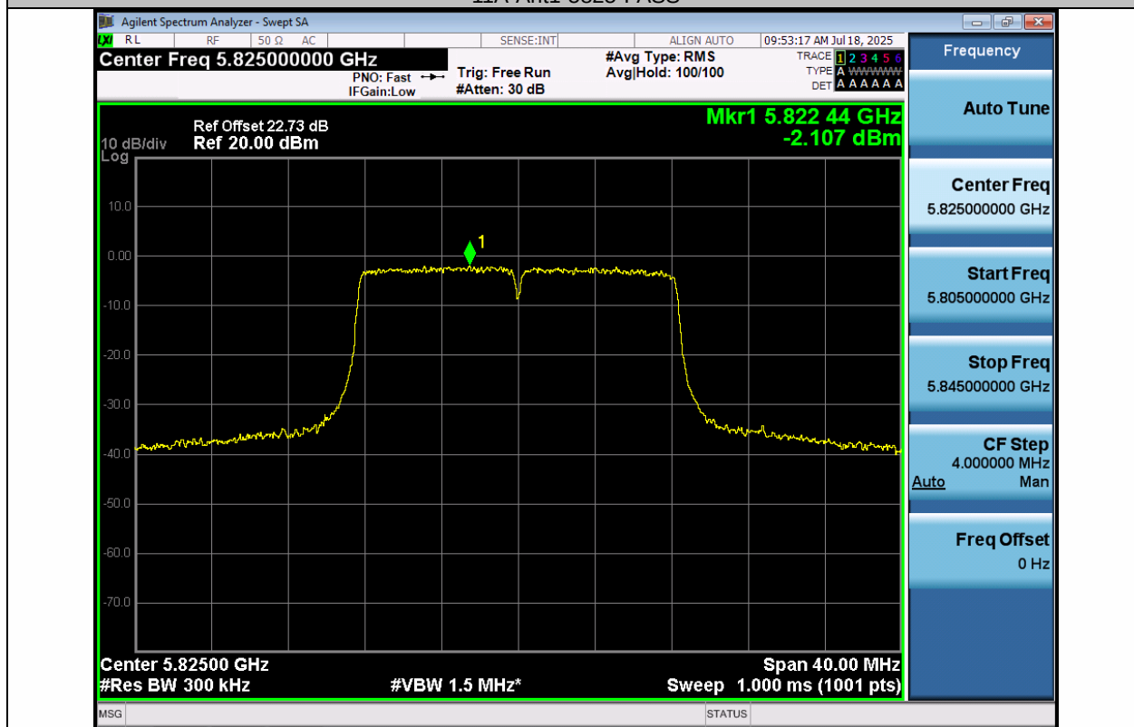
11A-Ant2-5825-PASS
