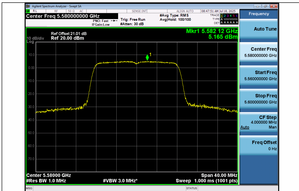
11A-Ant1-5580-PASS
