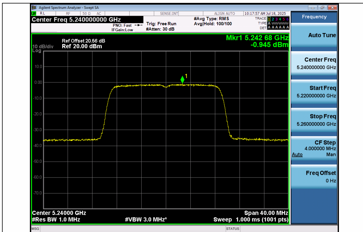
11N20MIMO-Ant1-5240-PASS
