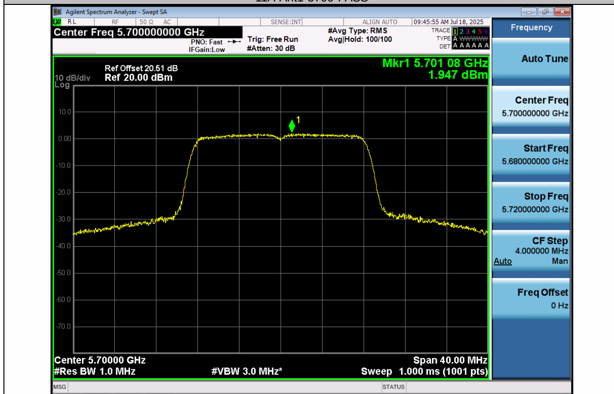
11A-Ant2-5700-PASS
