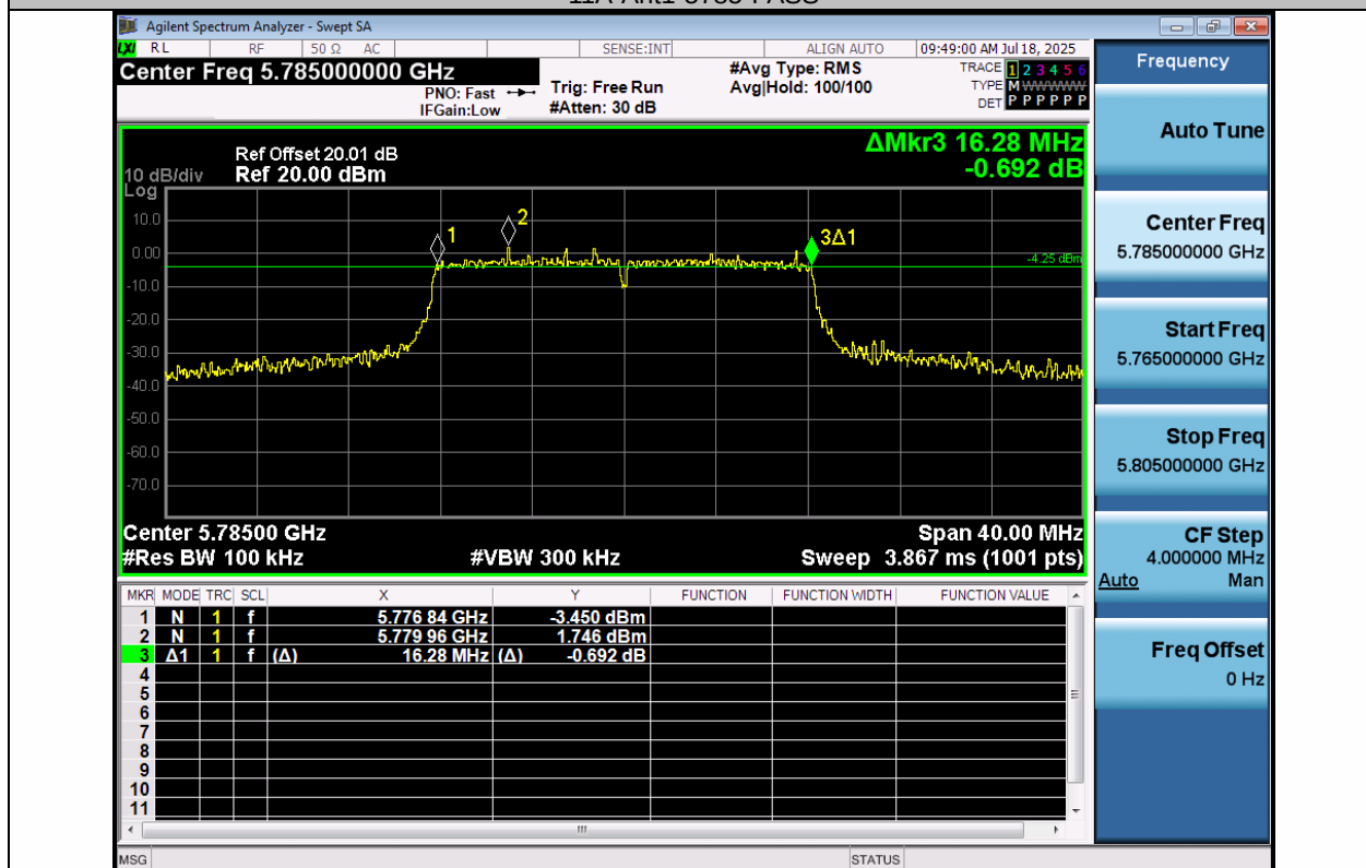
11A-Ant2-5785-PASS
