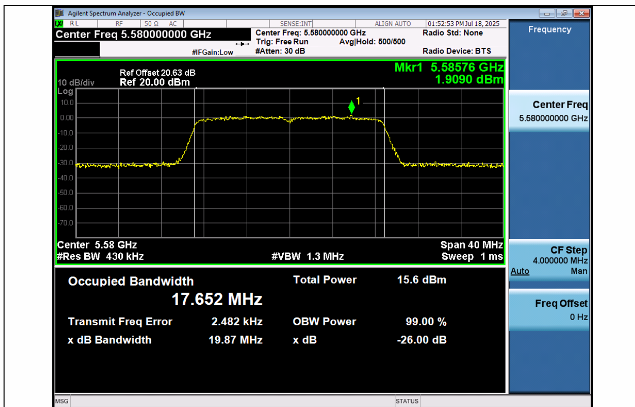
11AC20MIMO-Ant1-5580
