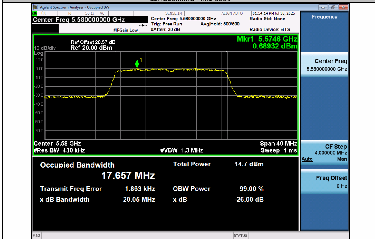
11AC20MIMO-Ant2-5580
