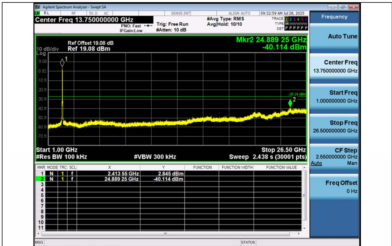
11N40MIMO-Ant1-2422-1000~26500-PASS
