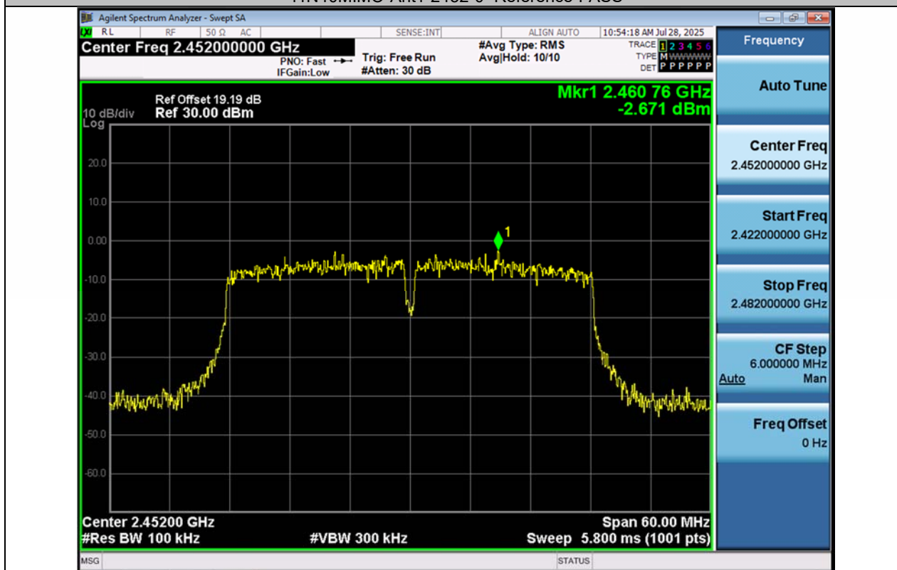
11N40MIMO-Ant2-2452-0~Reference-PASS
