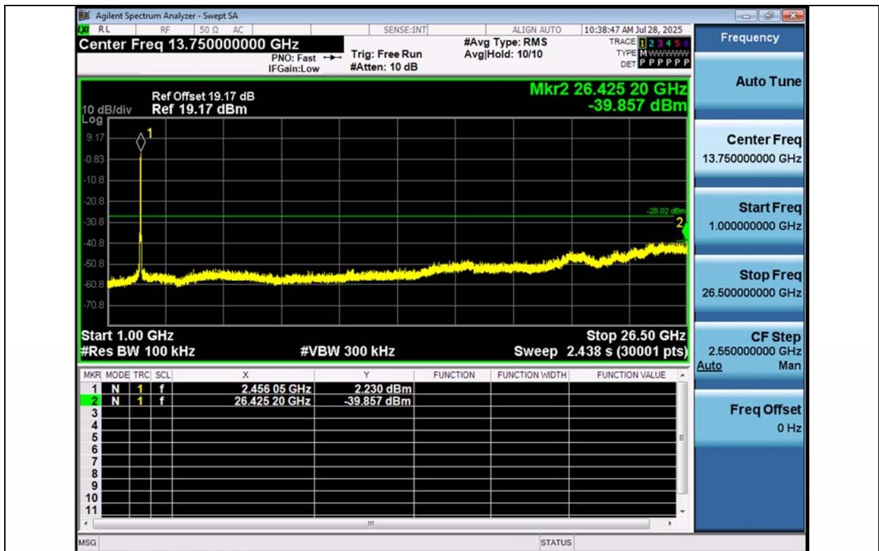
11N40MIMO-Ant1-2452-1000~26500-PASS
