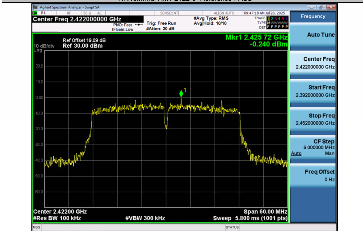
11N40MIMO-Ant2-2422-0~Reference-PASS
