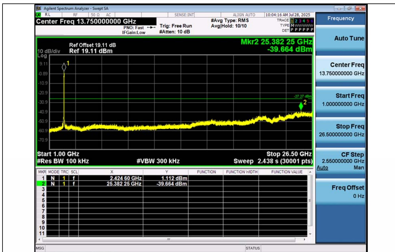
11N40MIMO-Ant1-2437-1000~26500-PASS
