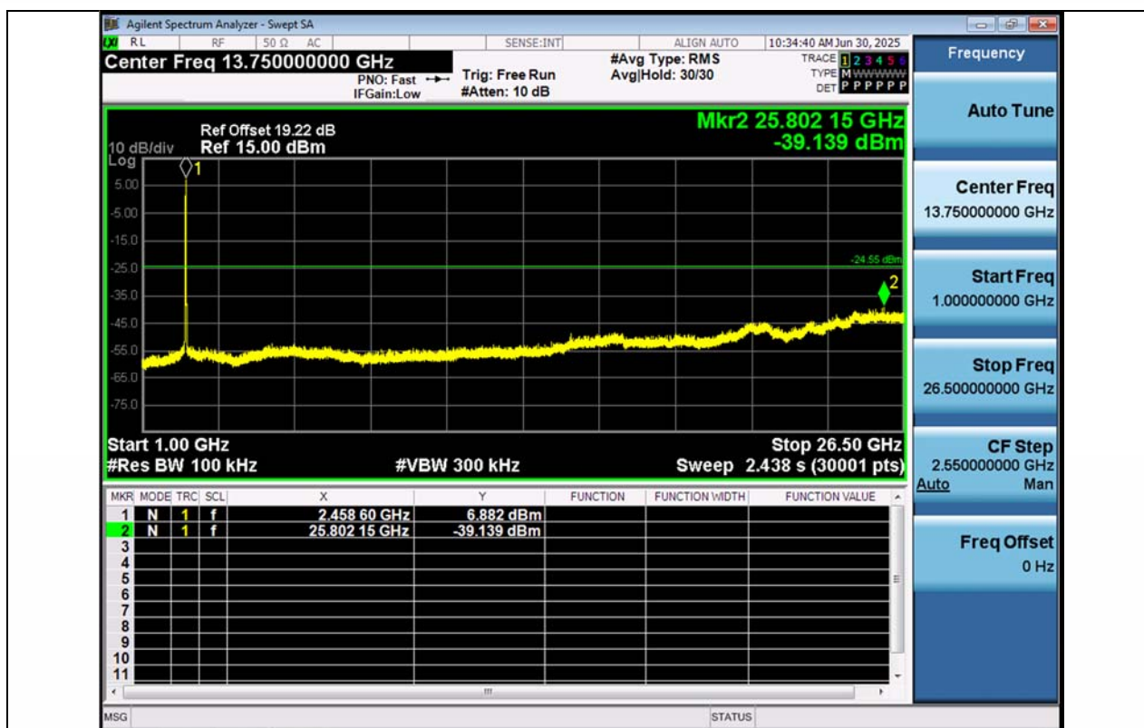
11G-Ant1-2462-1000~26500-PASS
