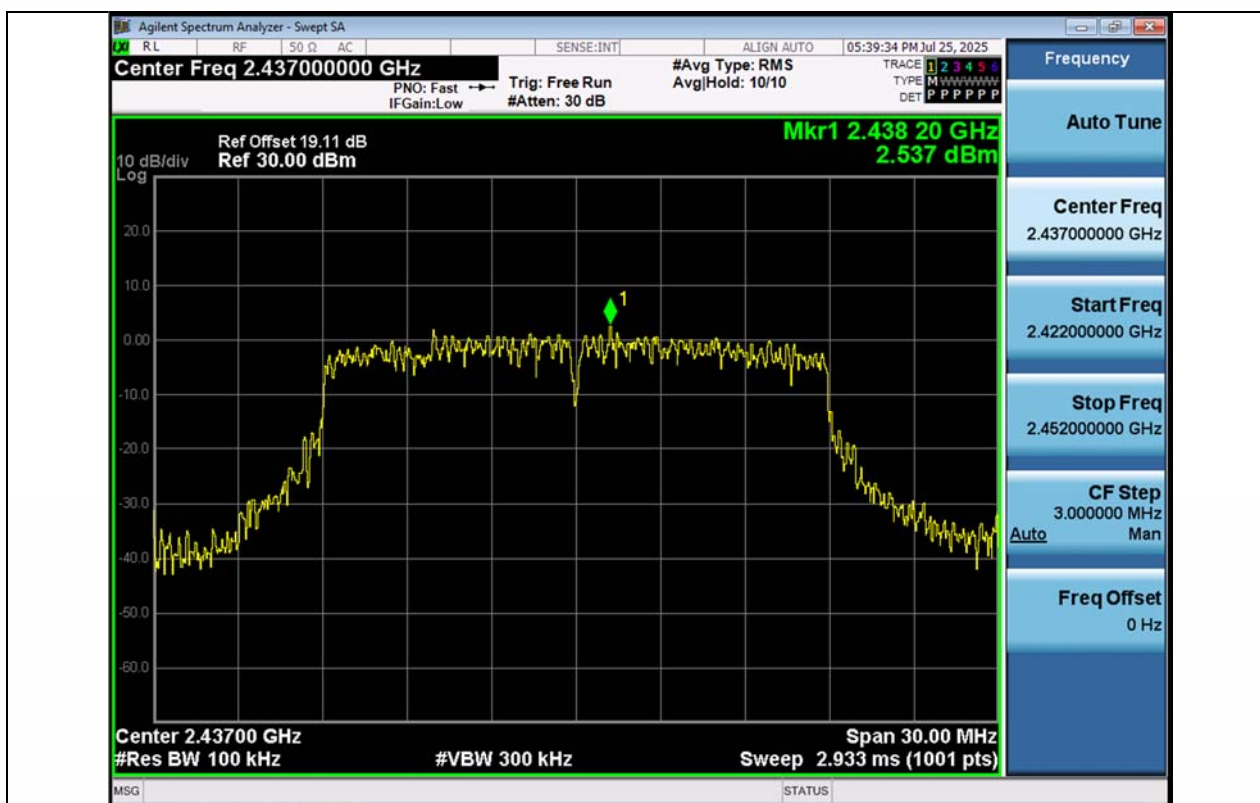
11N20MIMO-Ant1-2437-0~Reference-PASS
