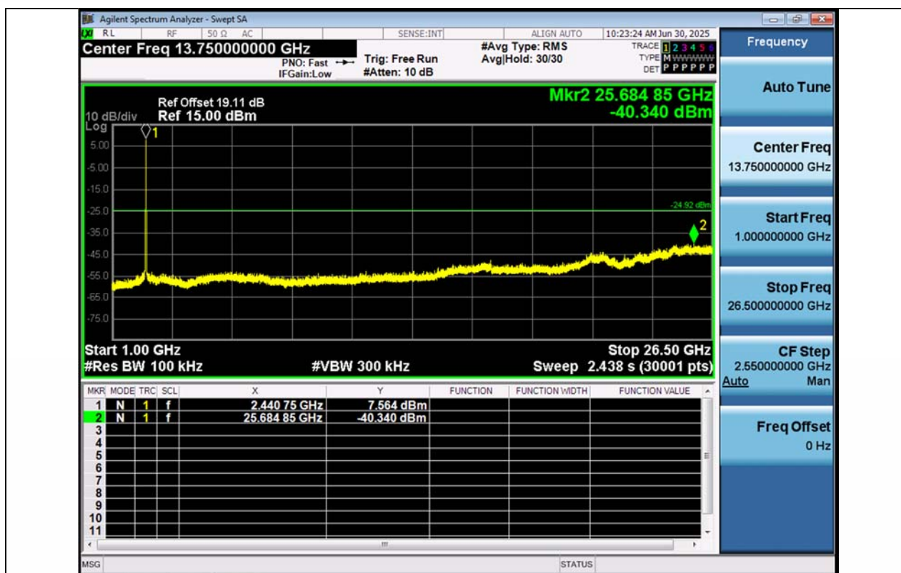
11G-Ant1-2437-1000~26500-PASS
