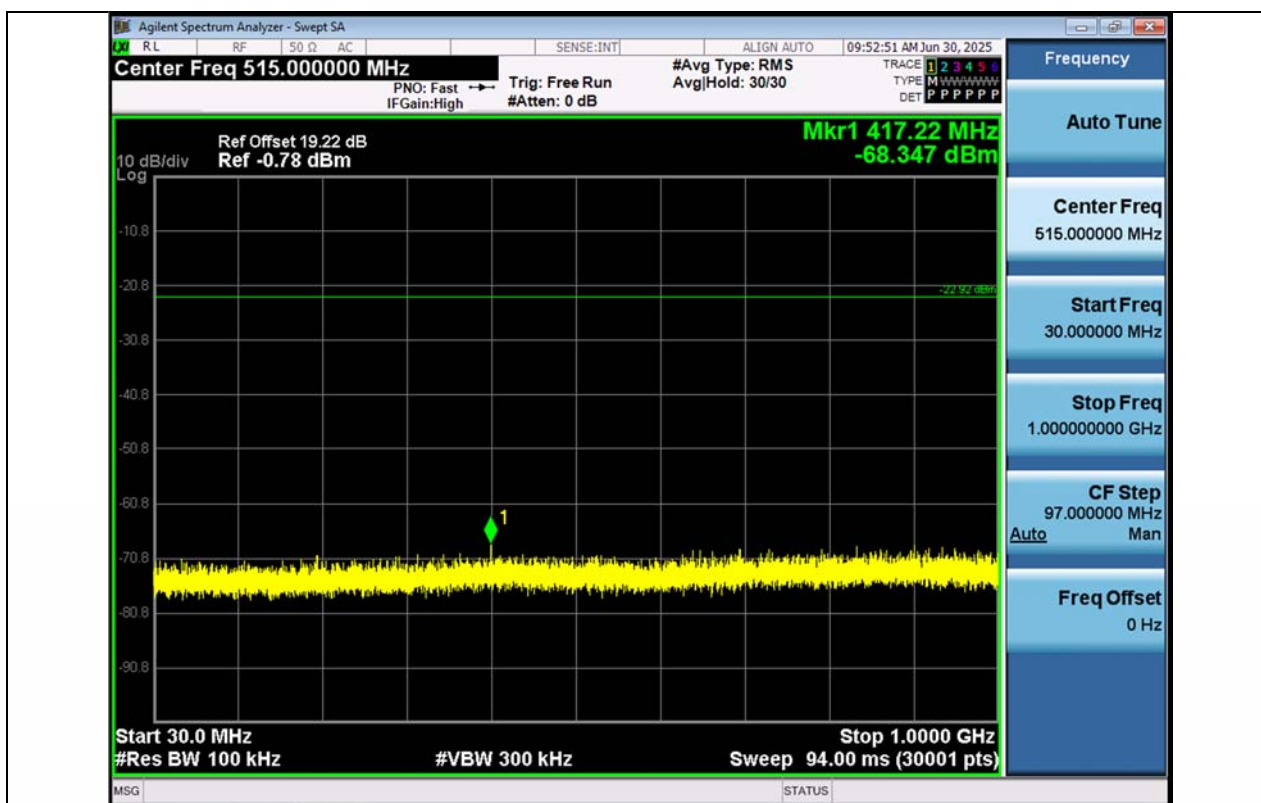
11B-Ant1-2462-30~1000-PASS
