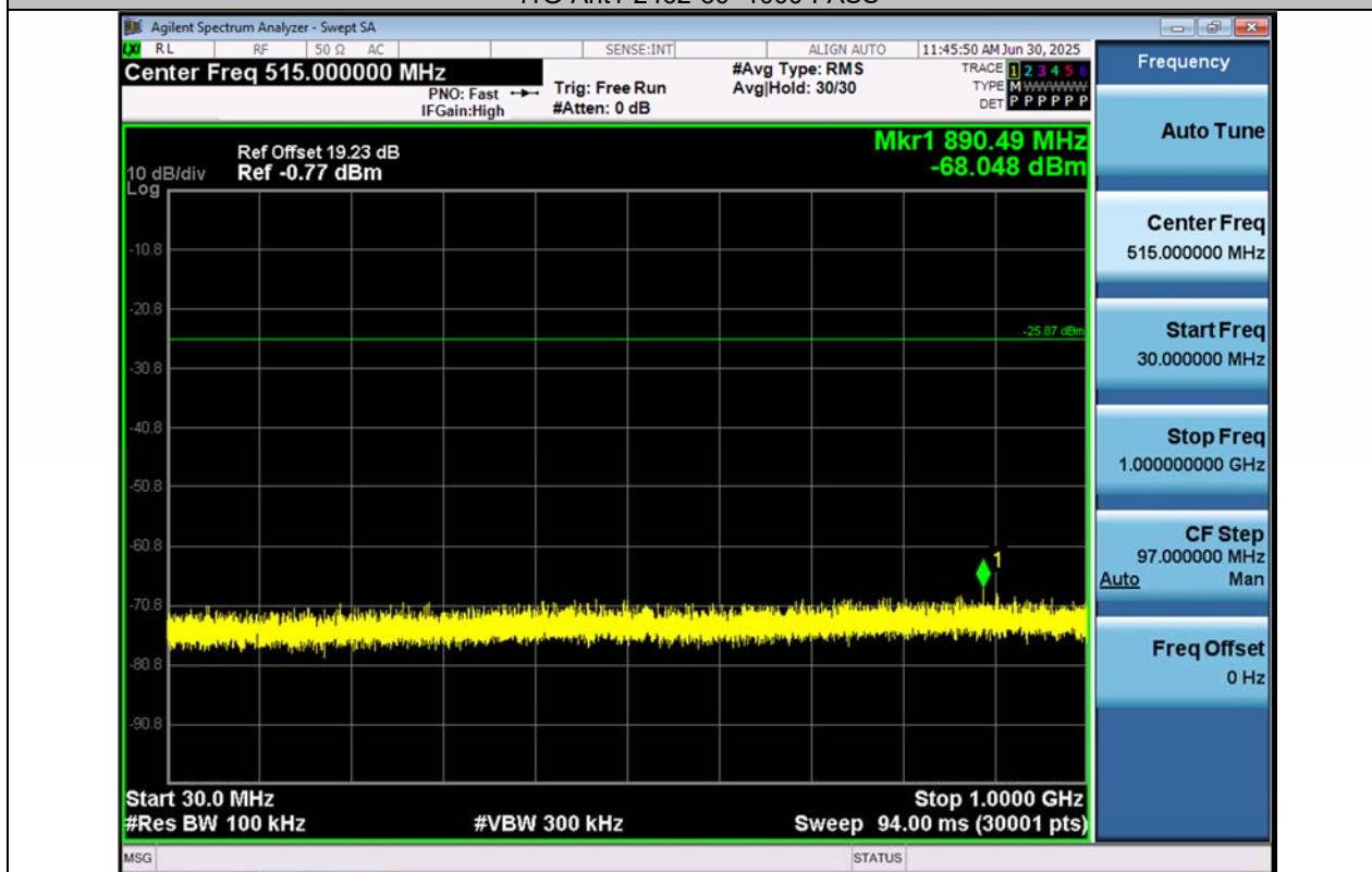
11G-Ant2-2462-30~1000-PASS
