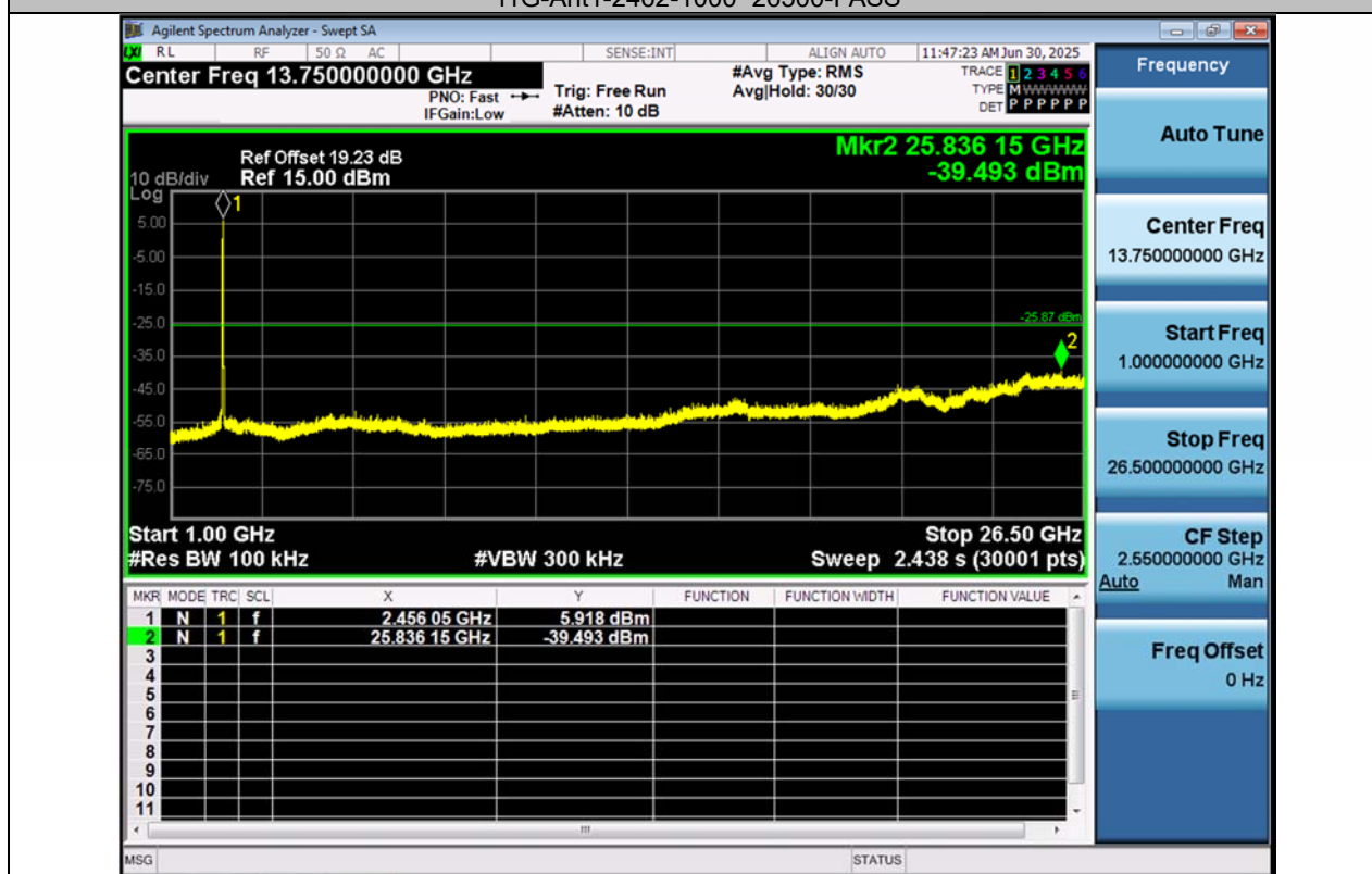
11G-Ant2-2462-1000~26500-PASS
