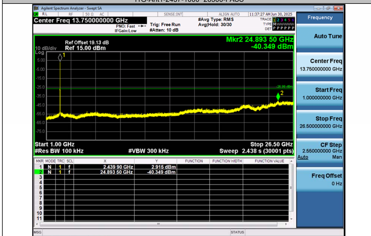
11G-Ant2-2437-1000~26500-PASS
