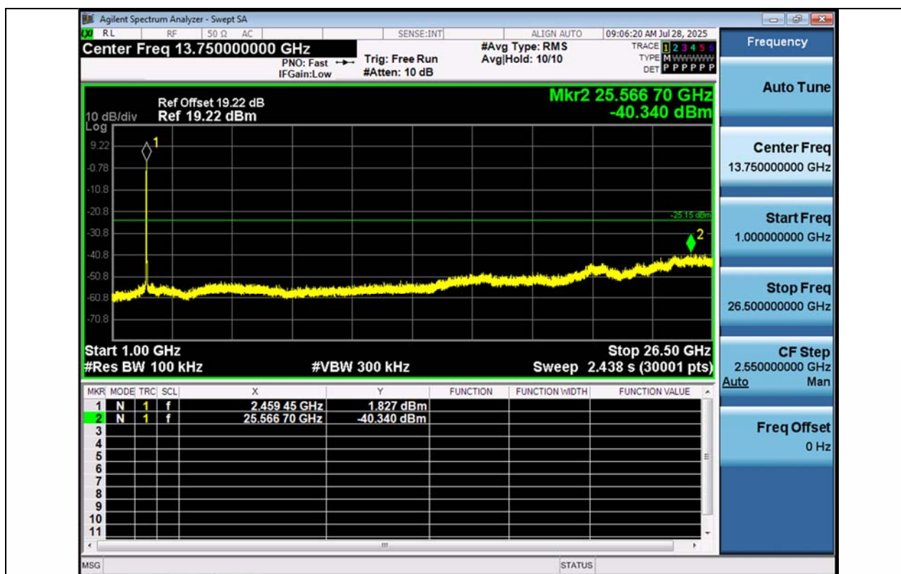
11N20MIMO-Ant1-2462-1000~26500-PASS
