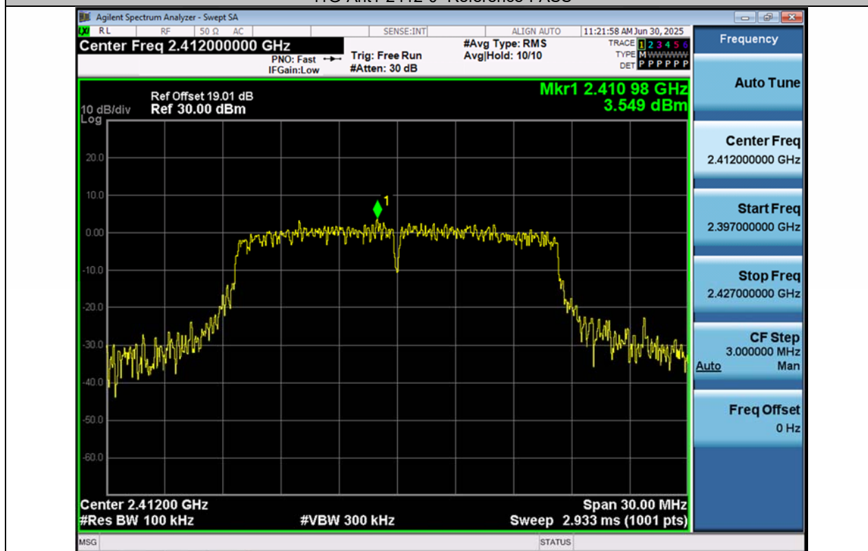
11G-Ant2-2412-0~Reference-PASS
