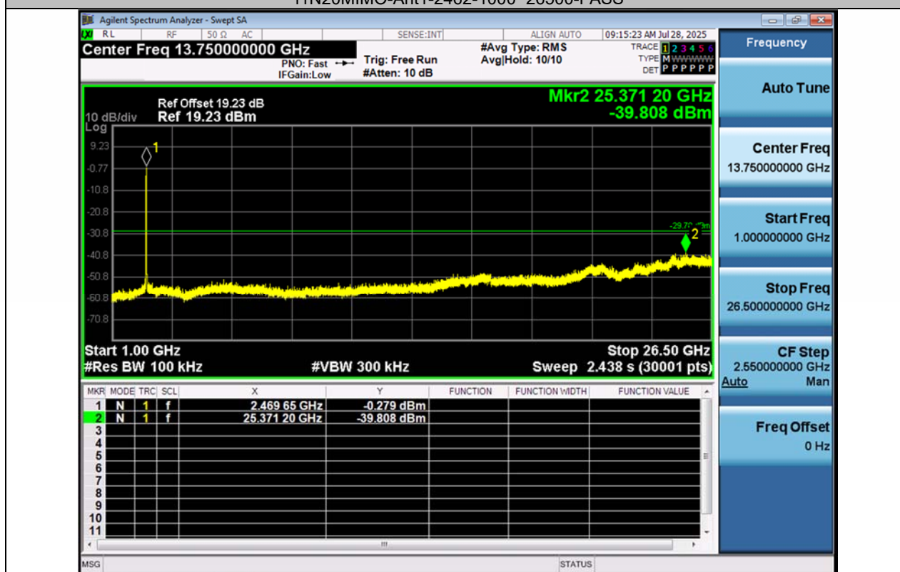
11N20MIMO-Ant2-2462-1000~26500-PASS
