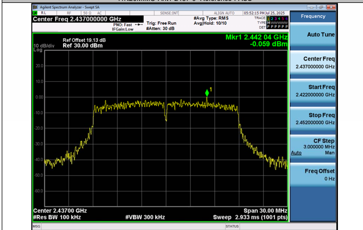
11N20MIMO-Ant2-2437-0~Reference-PASS
