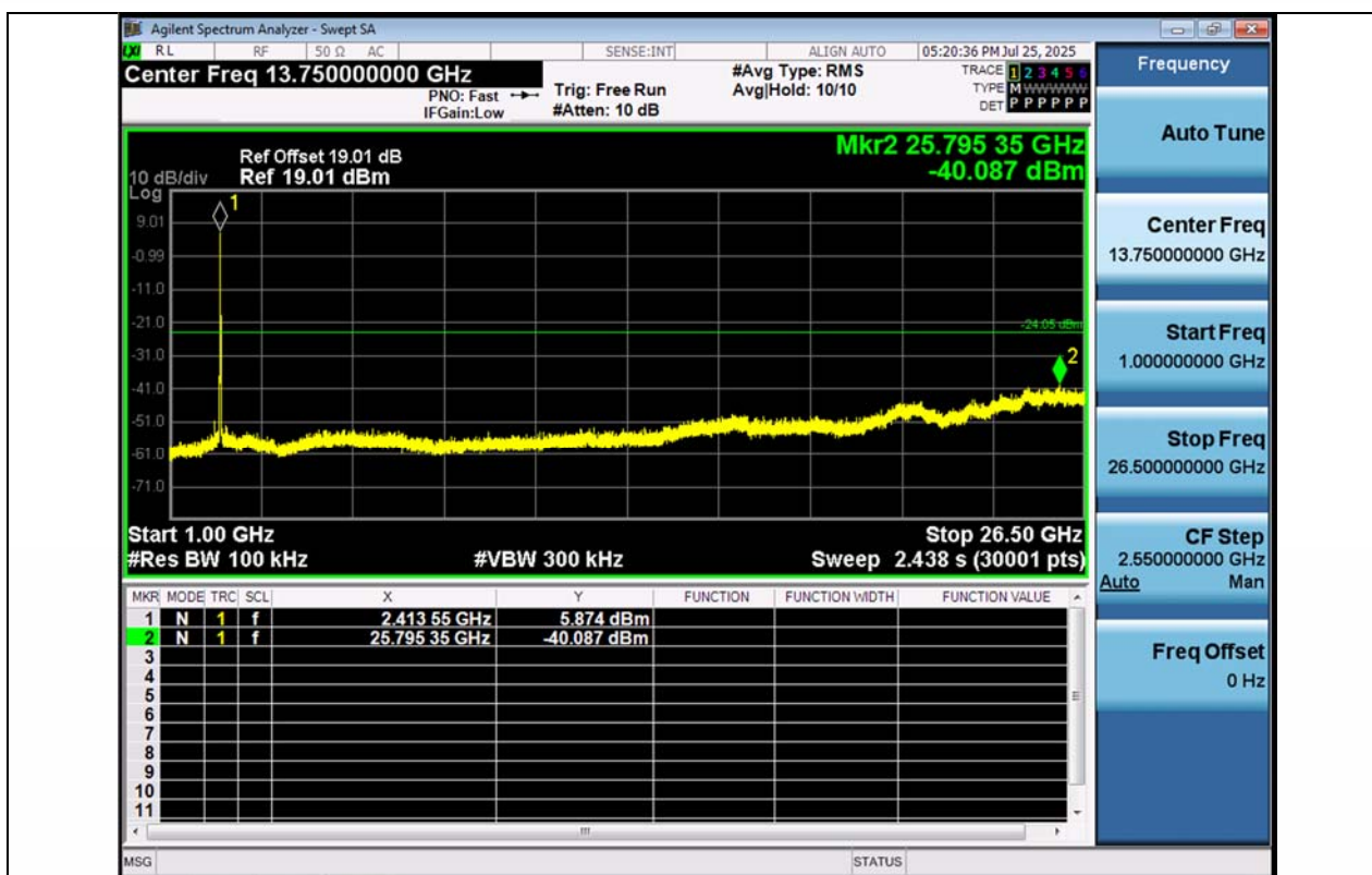
11N20MIMO-Ant1-2412-1000~26500-PASS
