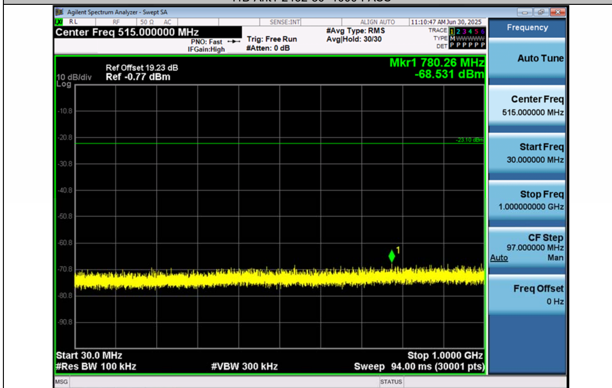
11B-Ant2-2462-30~1000-PASS
