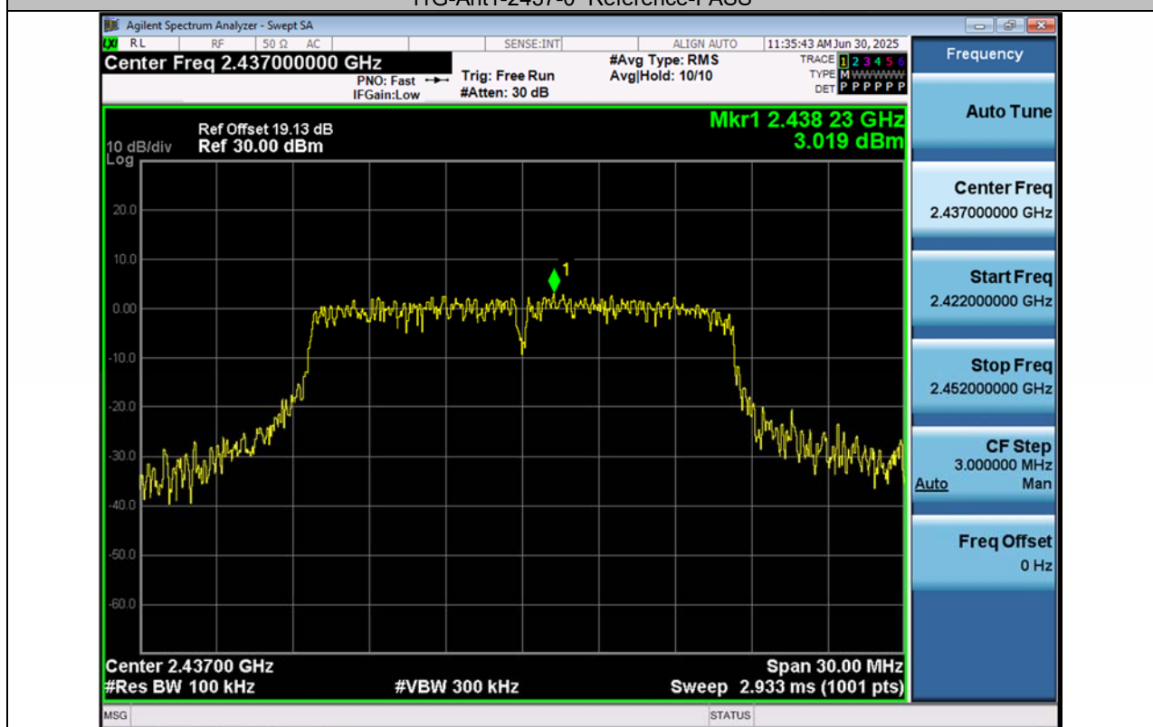
11G-Ant2-2437-0~Reference-PASS
