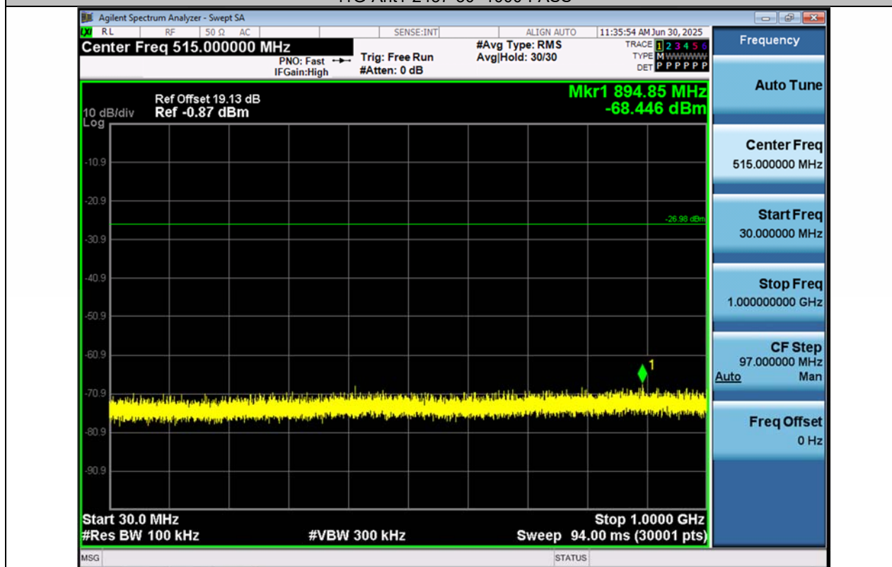
11G-Ant2-2437-30~1000-PASS
