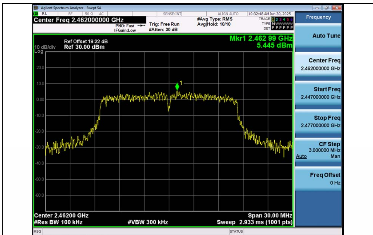
11G-Ant1-2462-0~Reference-PASS
