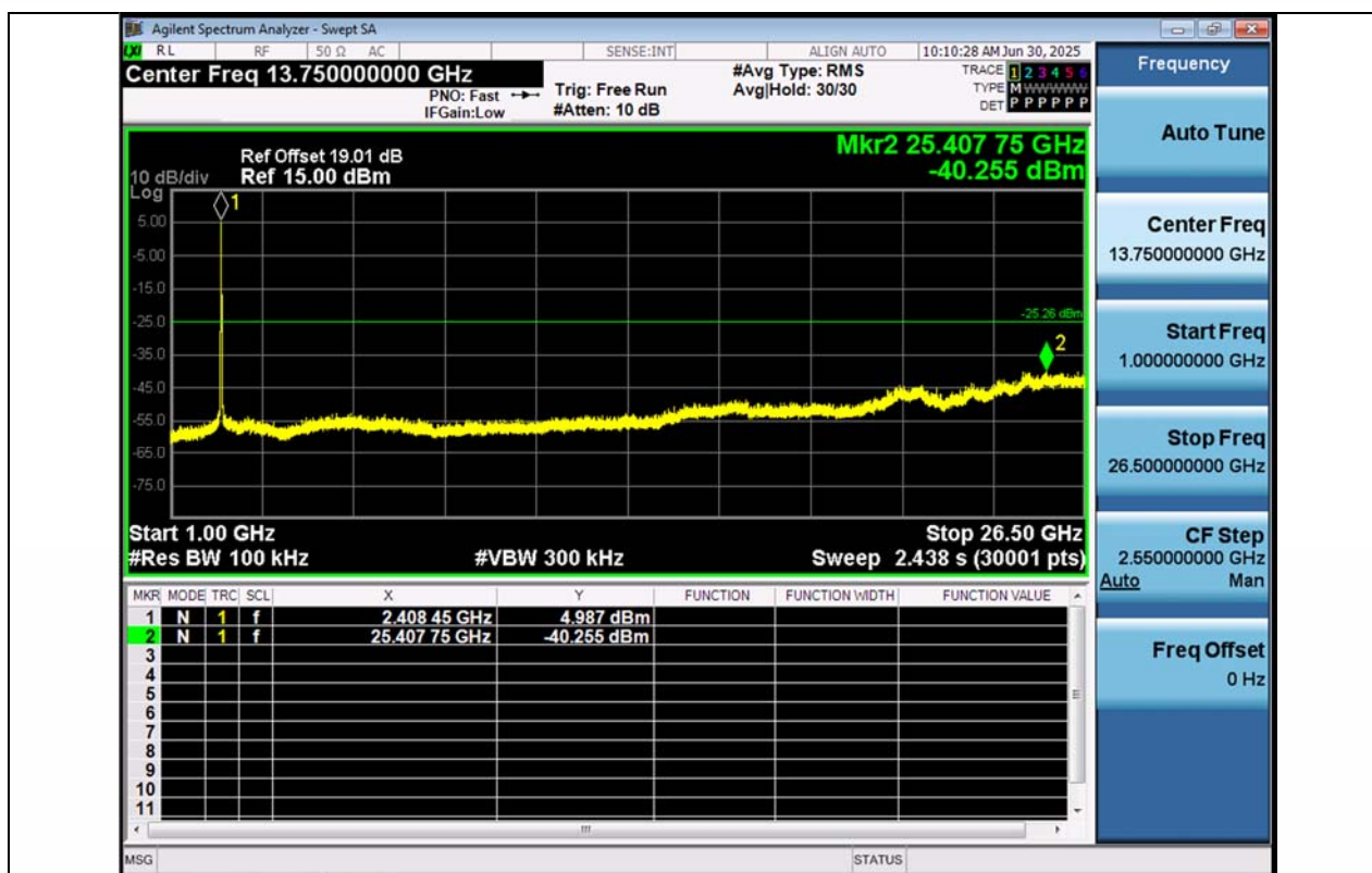
11G-Ant1-2412-1000~26500-PASS
