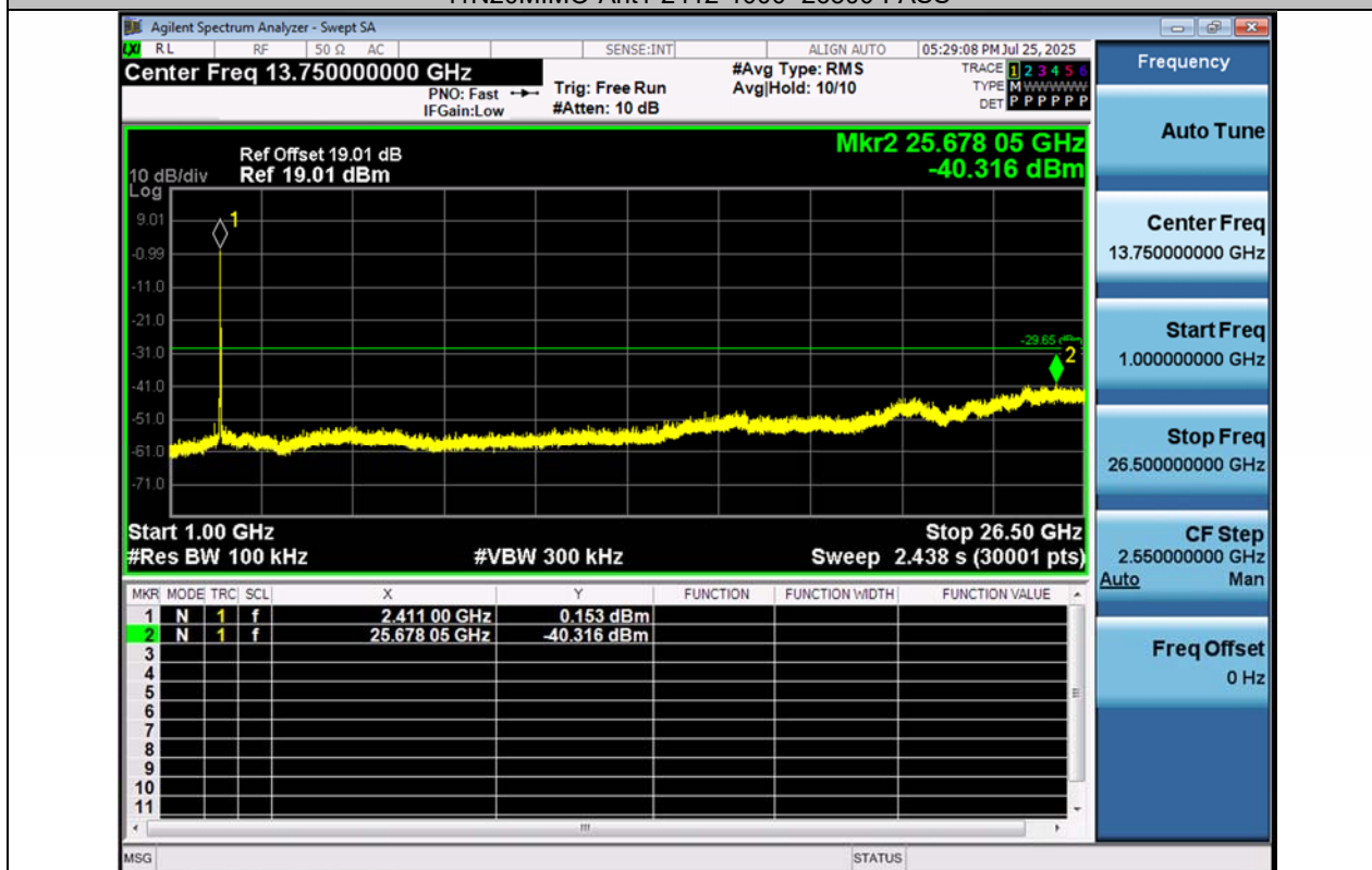
11N20MIMO-Ant2-2412-1000~26500-PASS
