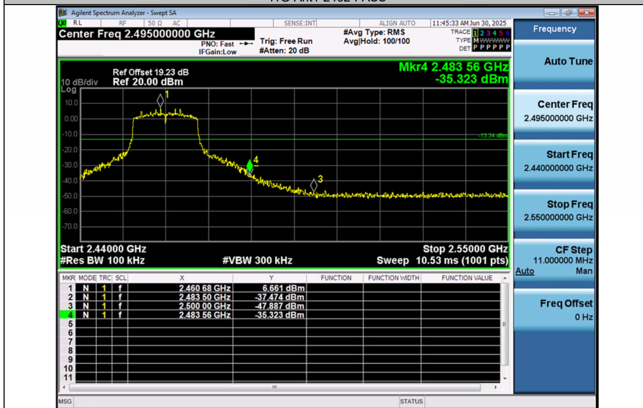
11G-Ant2-2462-PASS
