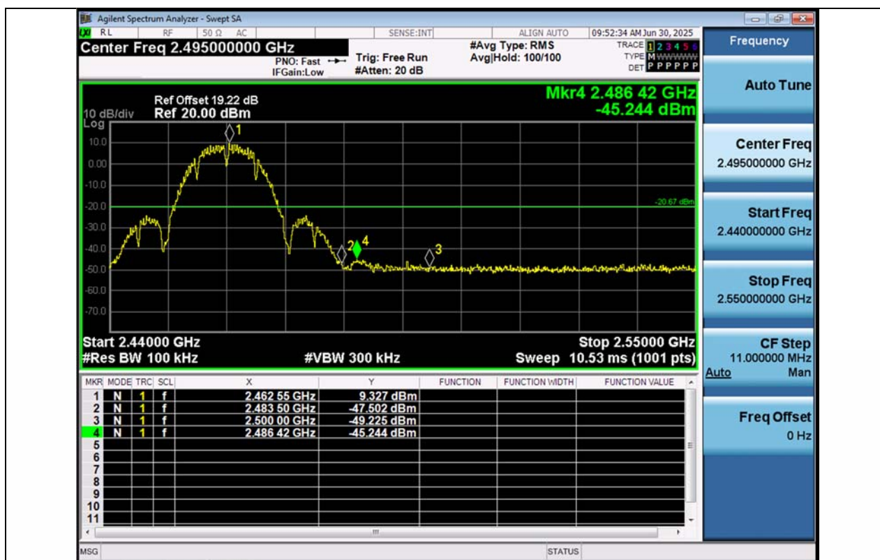
11B-Ant1-2462-PASS
