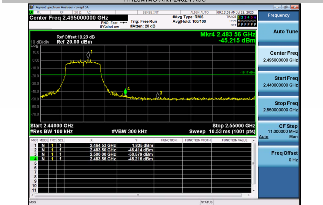
11N20MIMO-Ant2-2462-PASS
