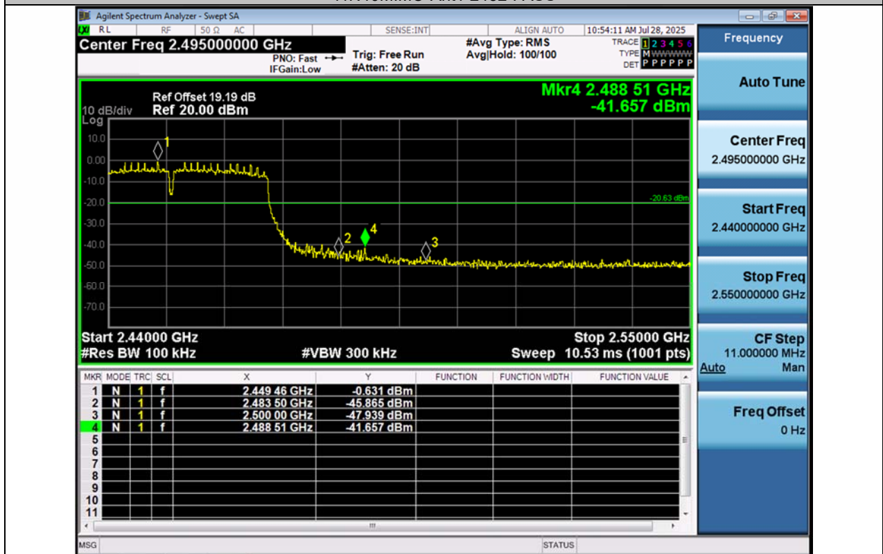
11N40MIMO-Ant2-2452-PASS
