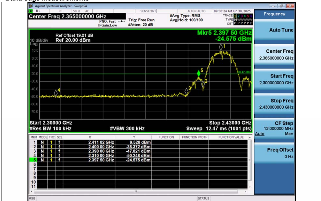
11B-Ant1-2412-PASS
