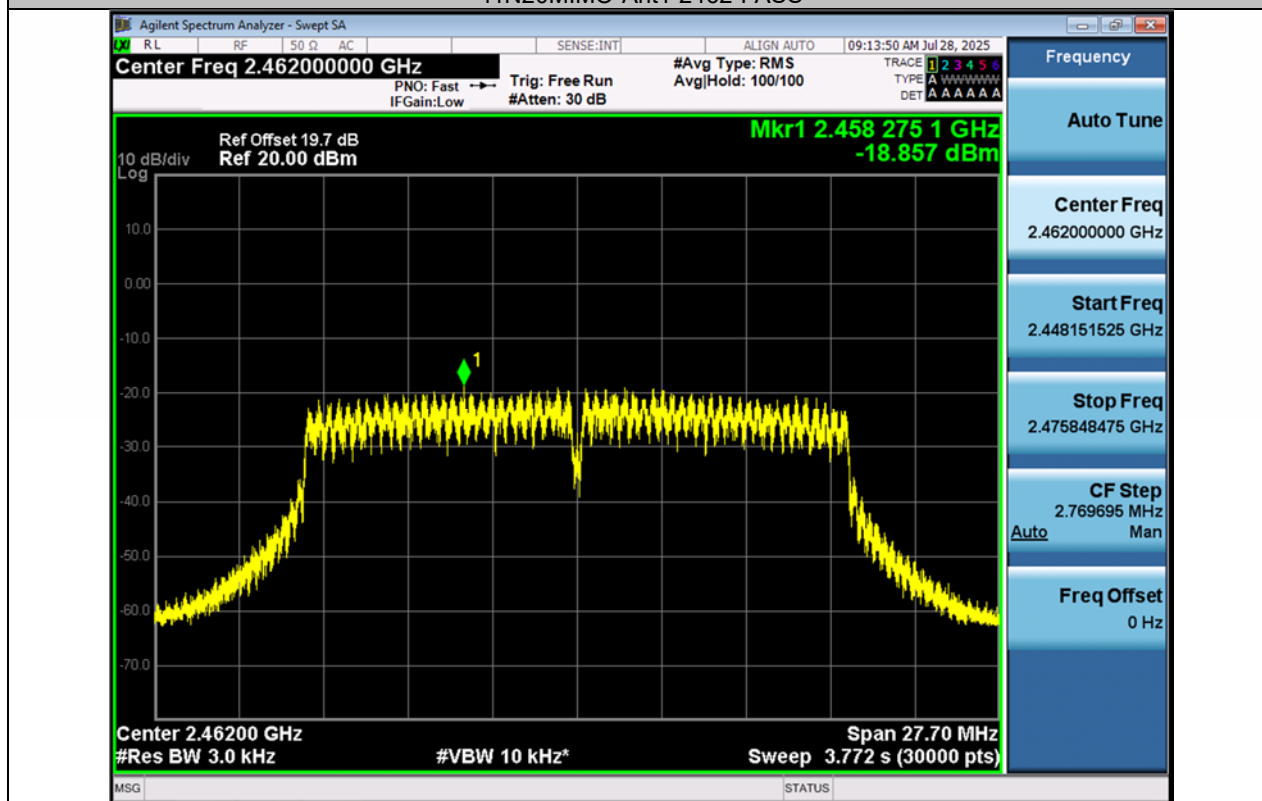
11N20MIMO-Ant2-2462-PASS
