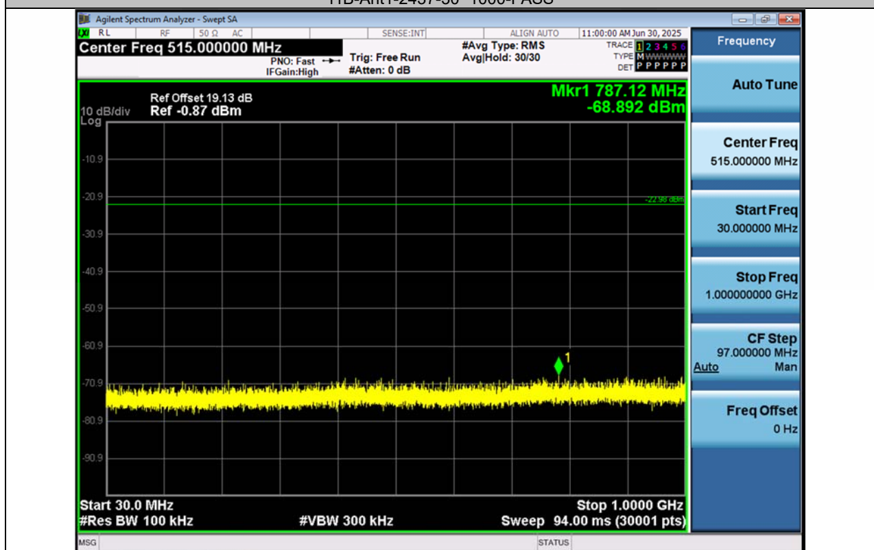
11B-Ant2-2437-30~1000-PASS
