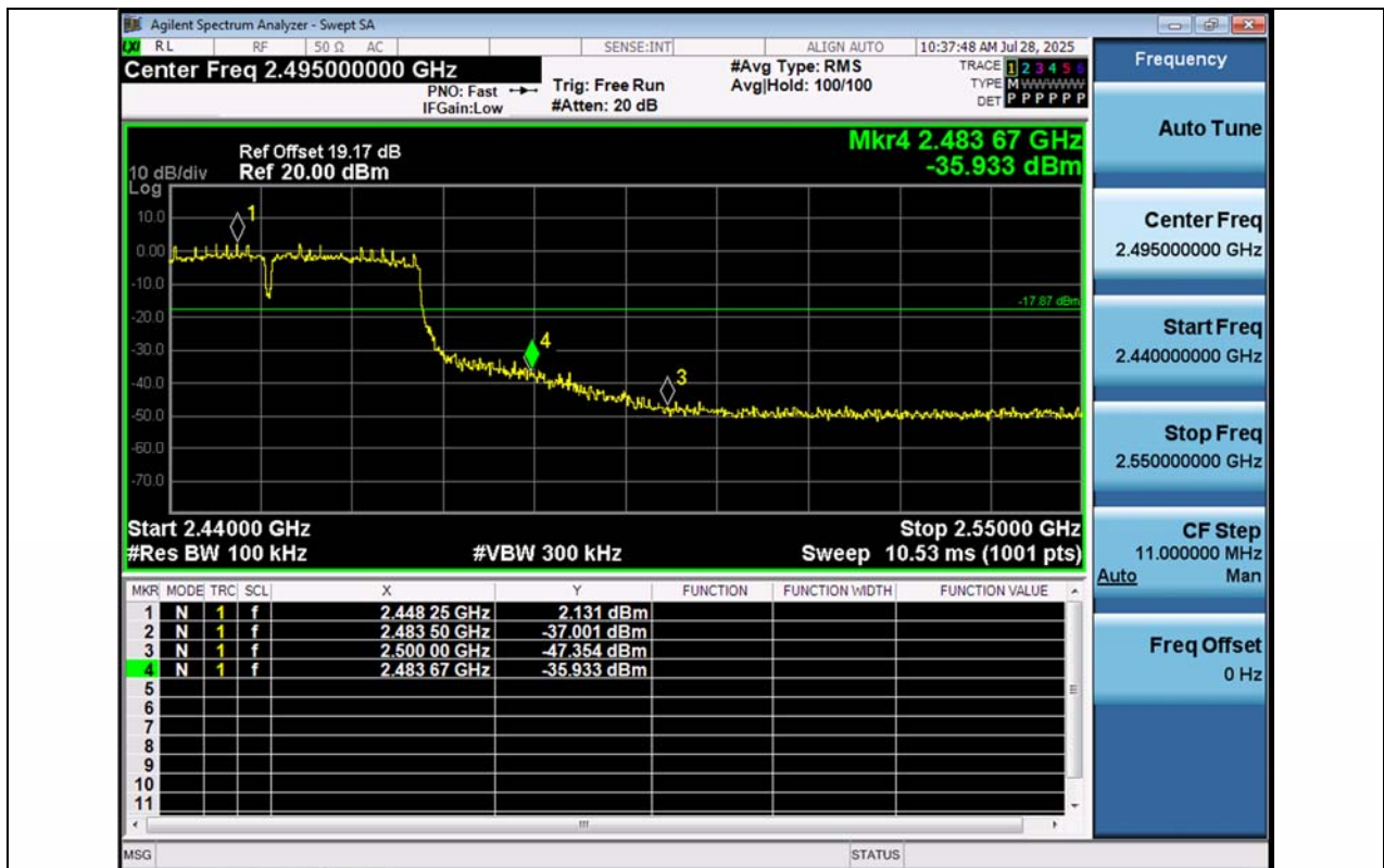
11N40MIMO-Ant1-2452-PASS
