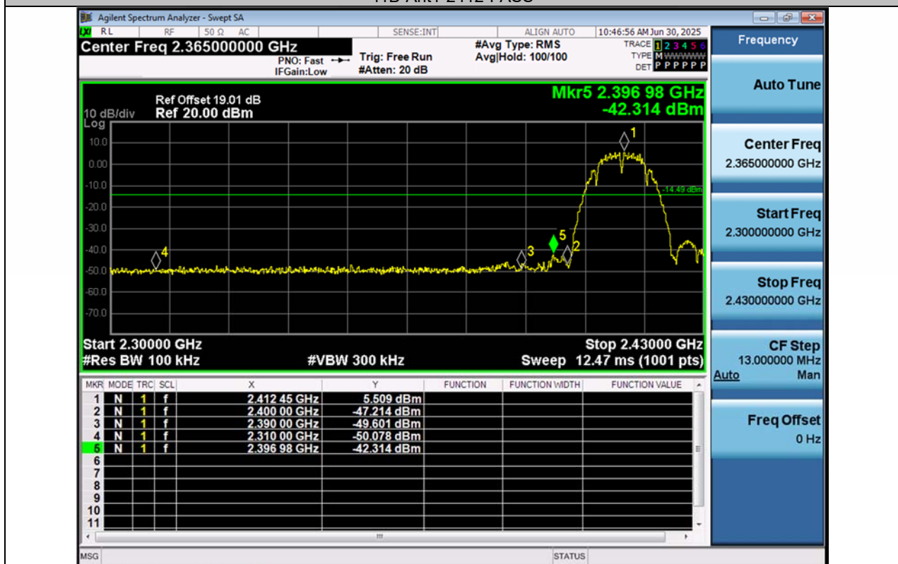
11B-Ant2-2412-PASS
