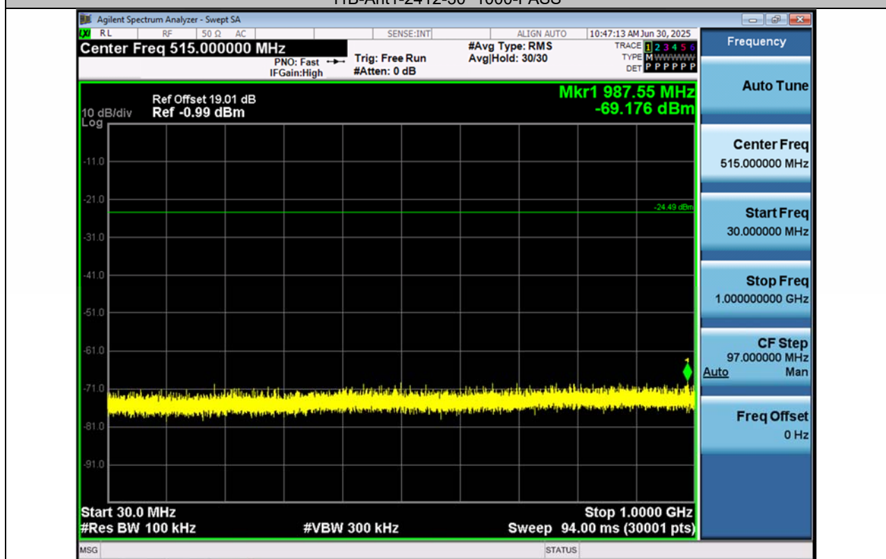
11B-Ant2-2412-30~1000-PASS
