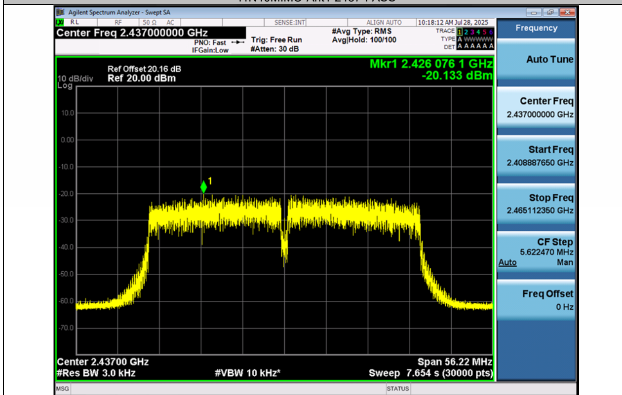
11N40MIMO-Ant2-2437-PASS
