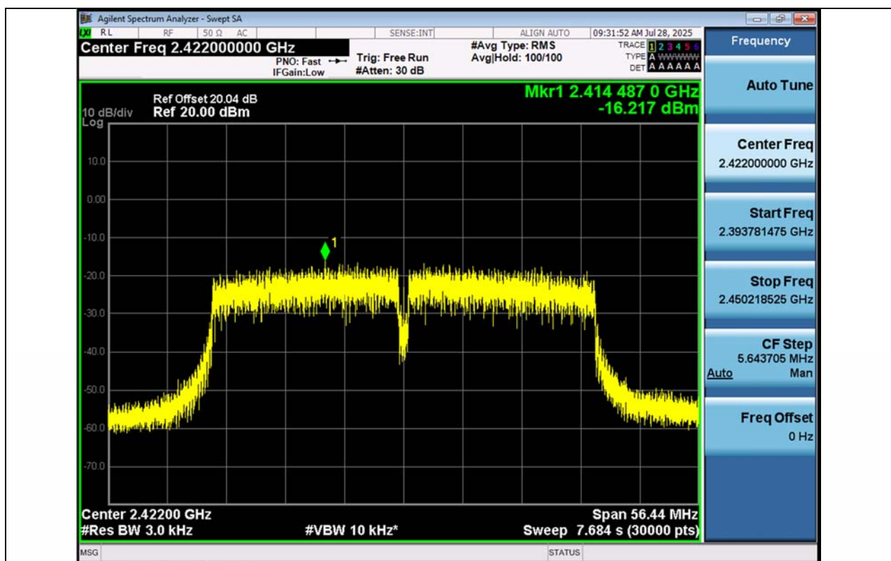
11N40MIMO-Ant1-2422-PASS
