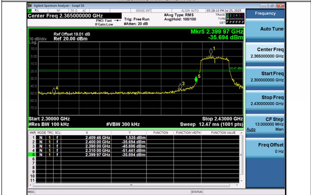
11N20MIMO-Ant2-2412-PASS
