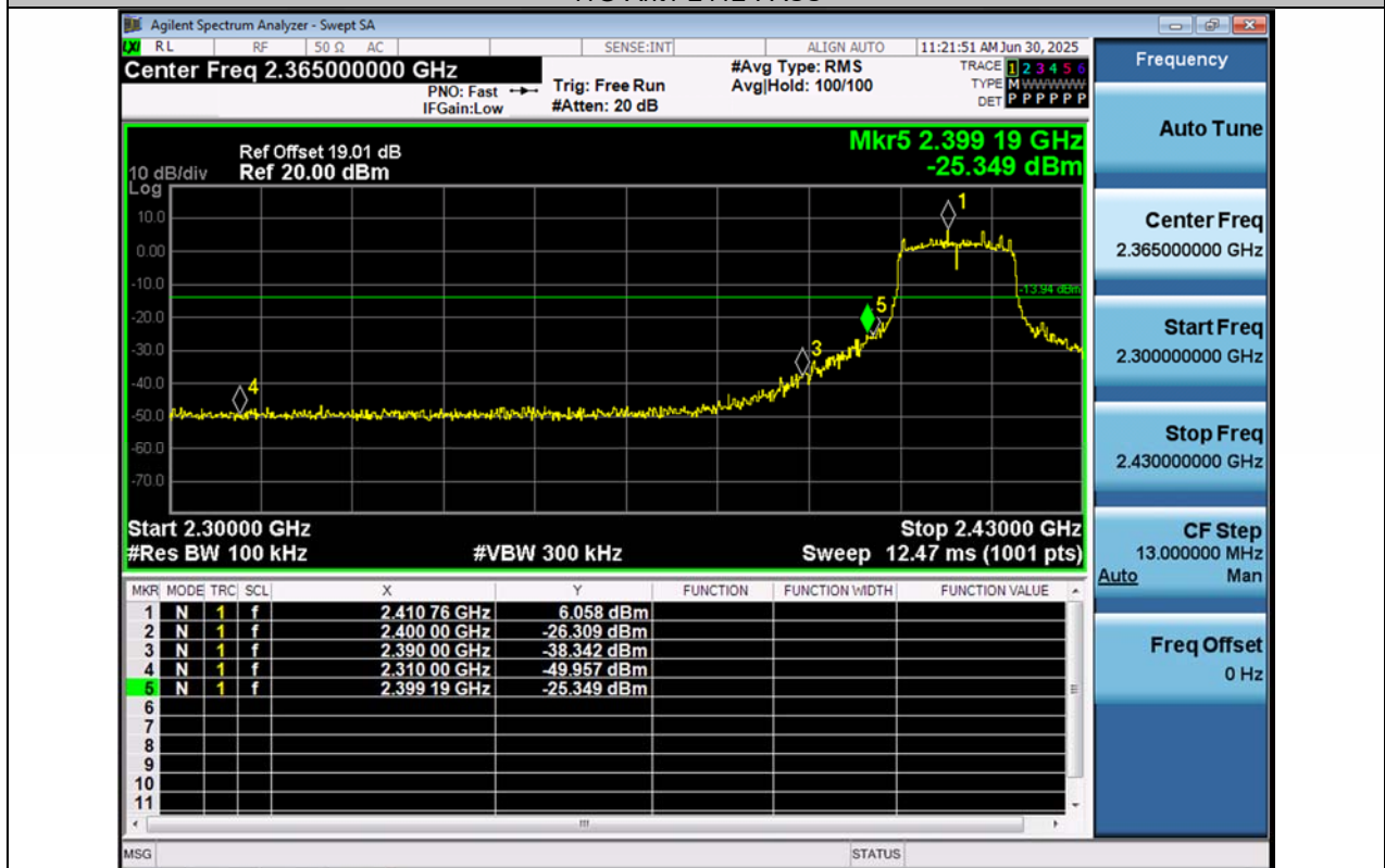
11G-Ant2-2412-PASS
