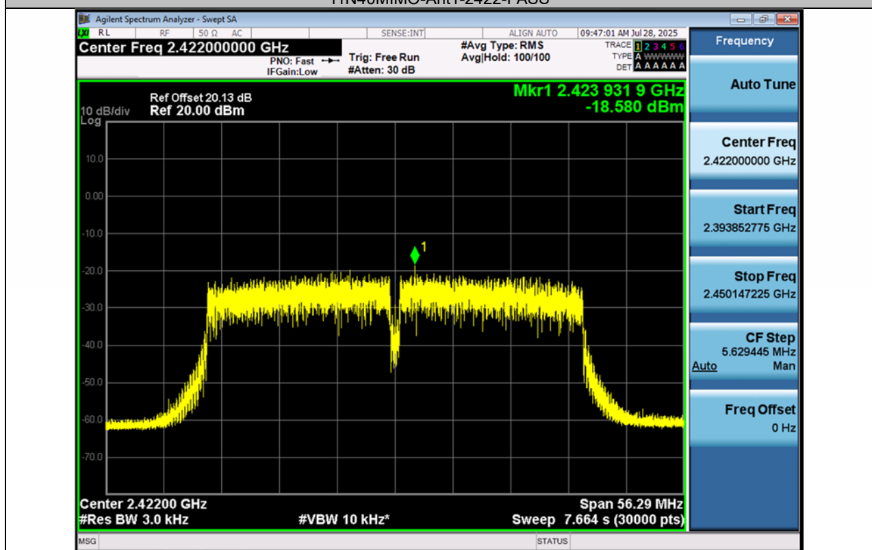
11N40MIMO-Ant2-2422-PASS
