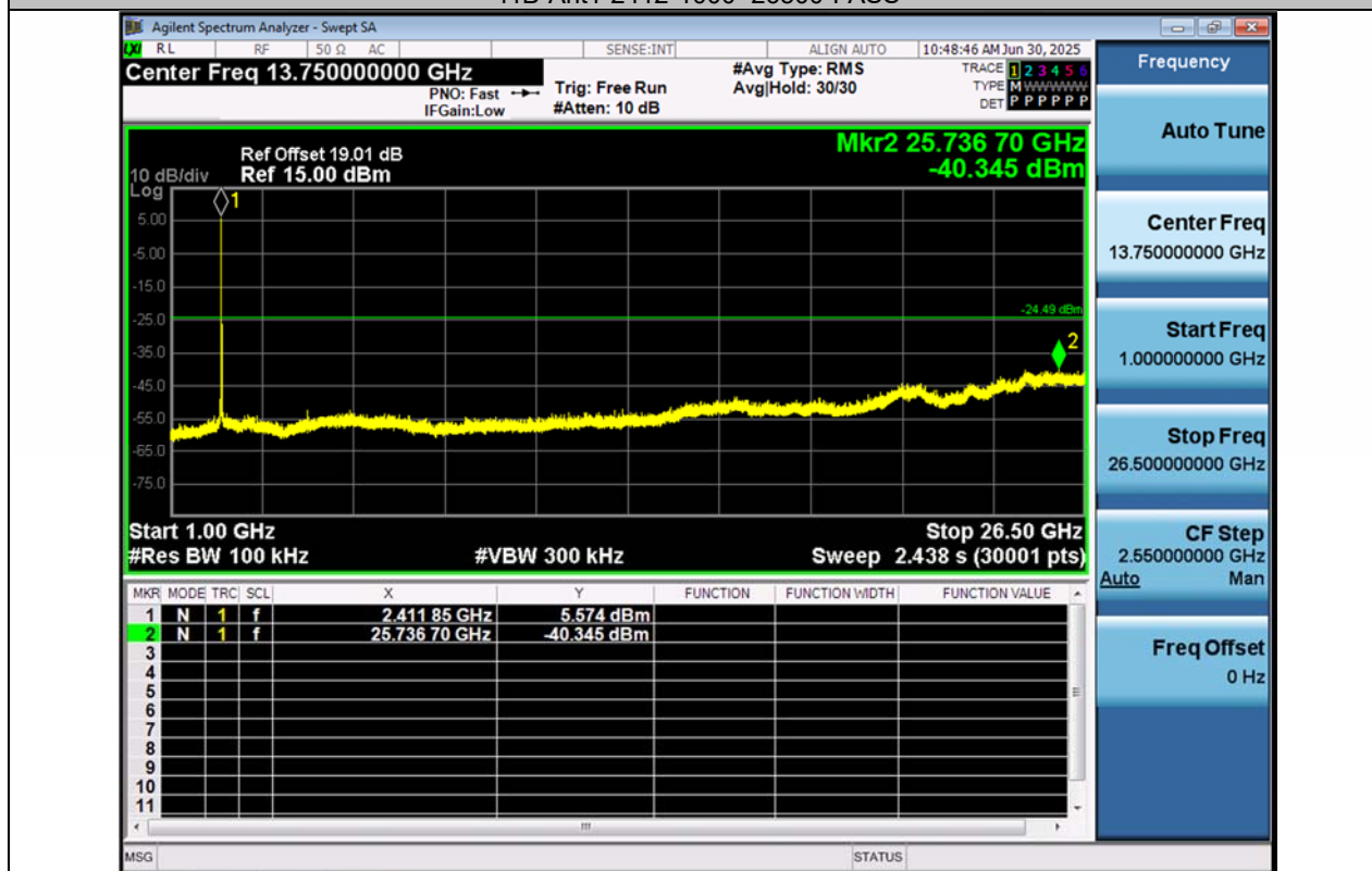
11B-Ant2-2412-1000~26500-PASS
