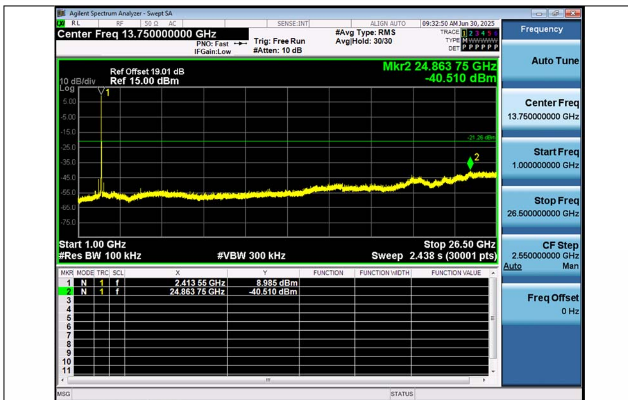
11B-Ant1-2412-1000~26500-PASS
