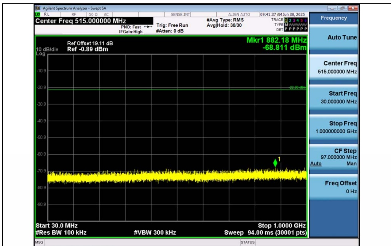
11B-Ant1-2437-30~1000-PASS
