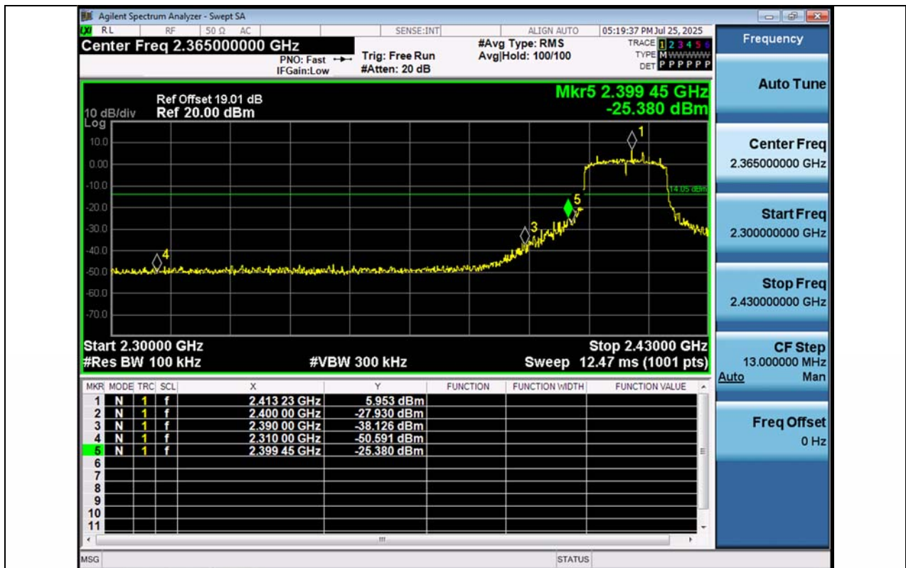
11N20MIMO-Ant1-2412-PASS
