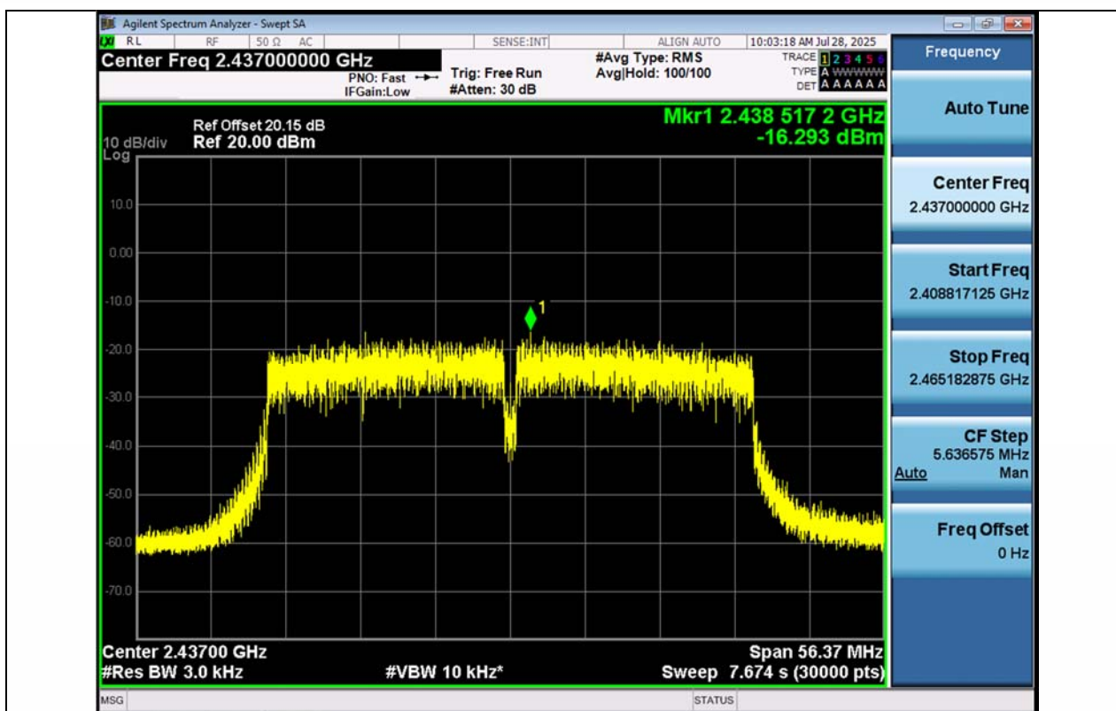
11N40MIMO-Ant1-2437-PASS
