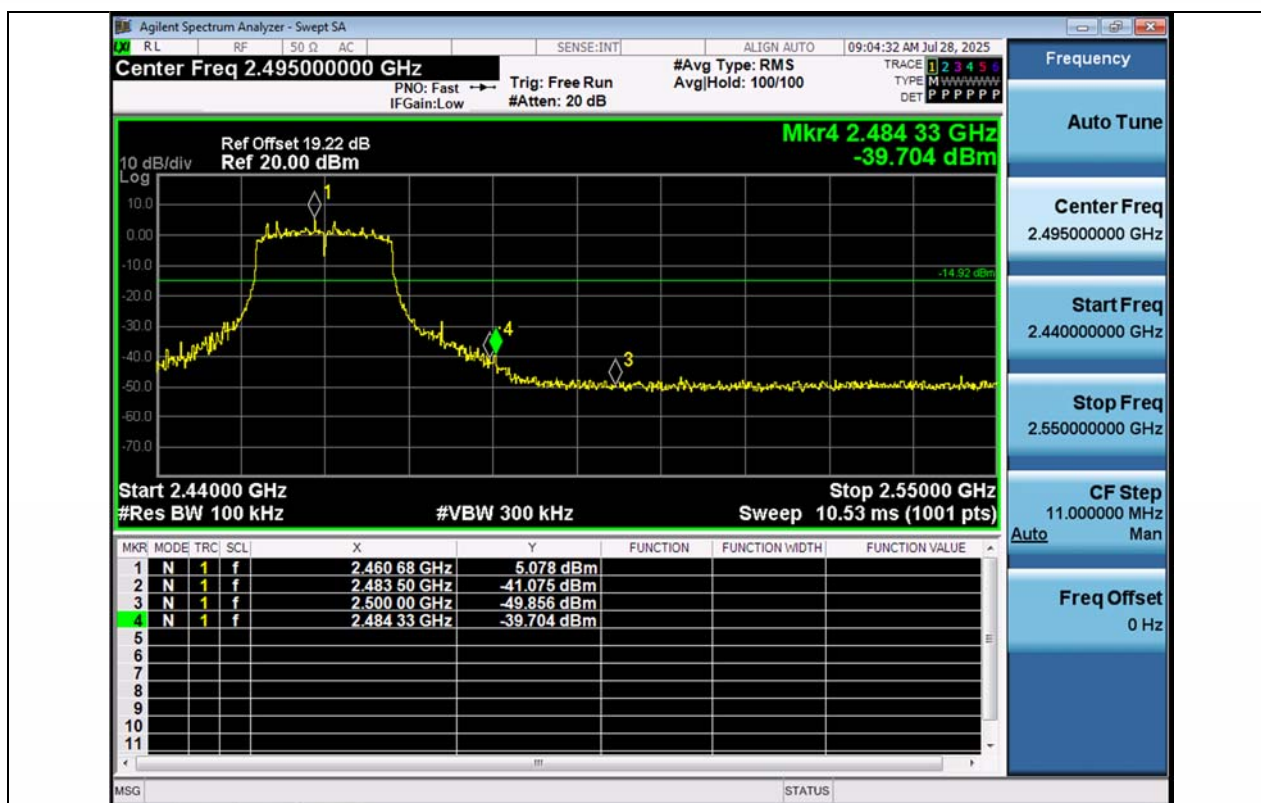
11N20MIMO-Ant1-2462-PASS
