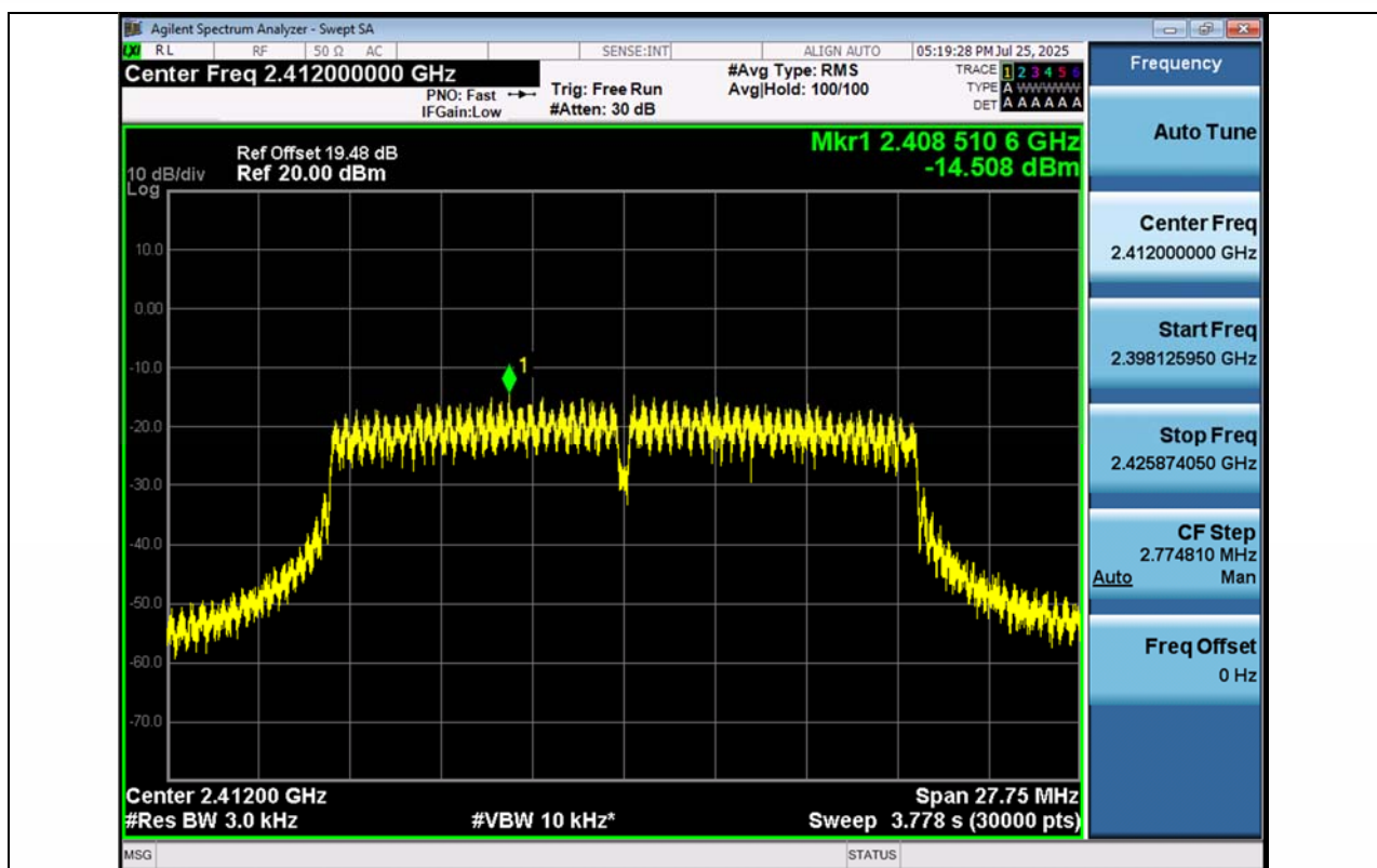
11N20MIMO-Ant1-2412-PASS
