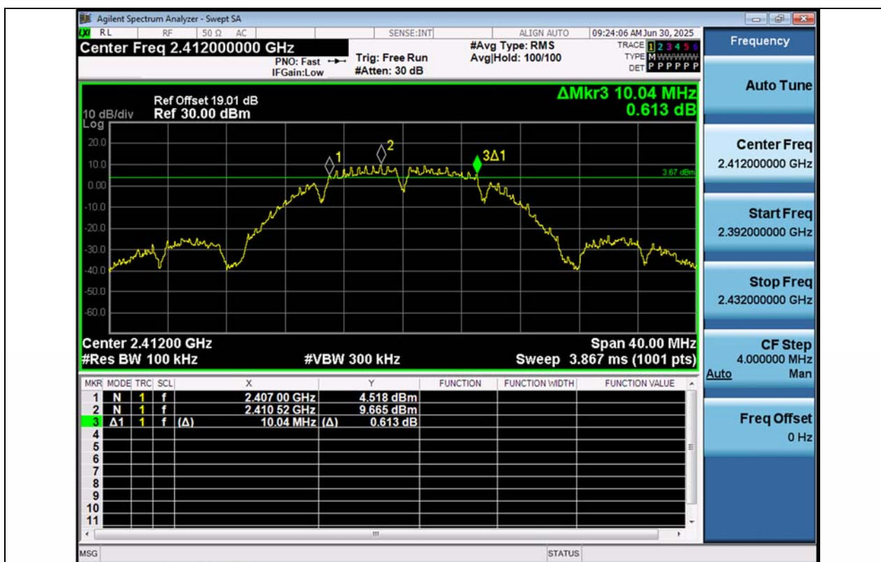
11B-Ant1-2412-PASS
