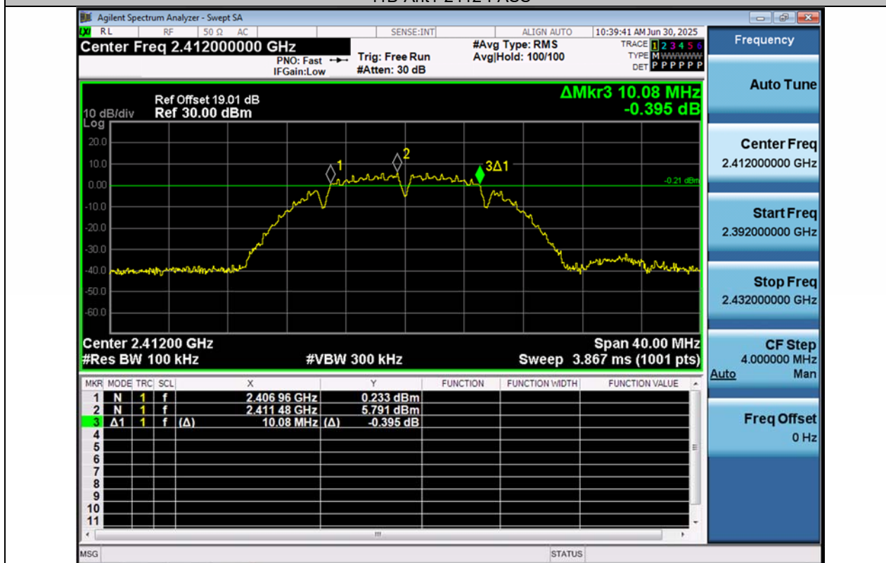
11B-Ant2-2412-PASS
