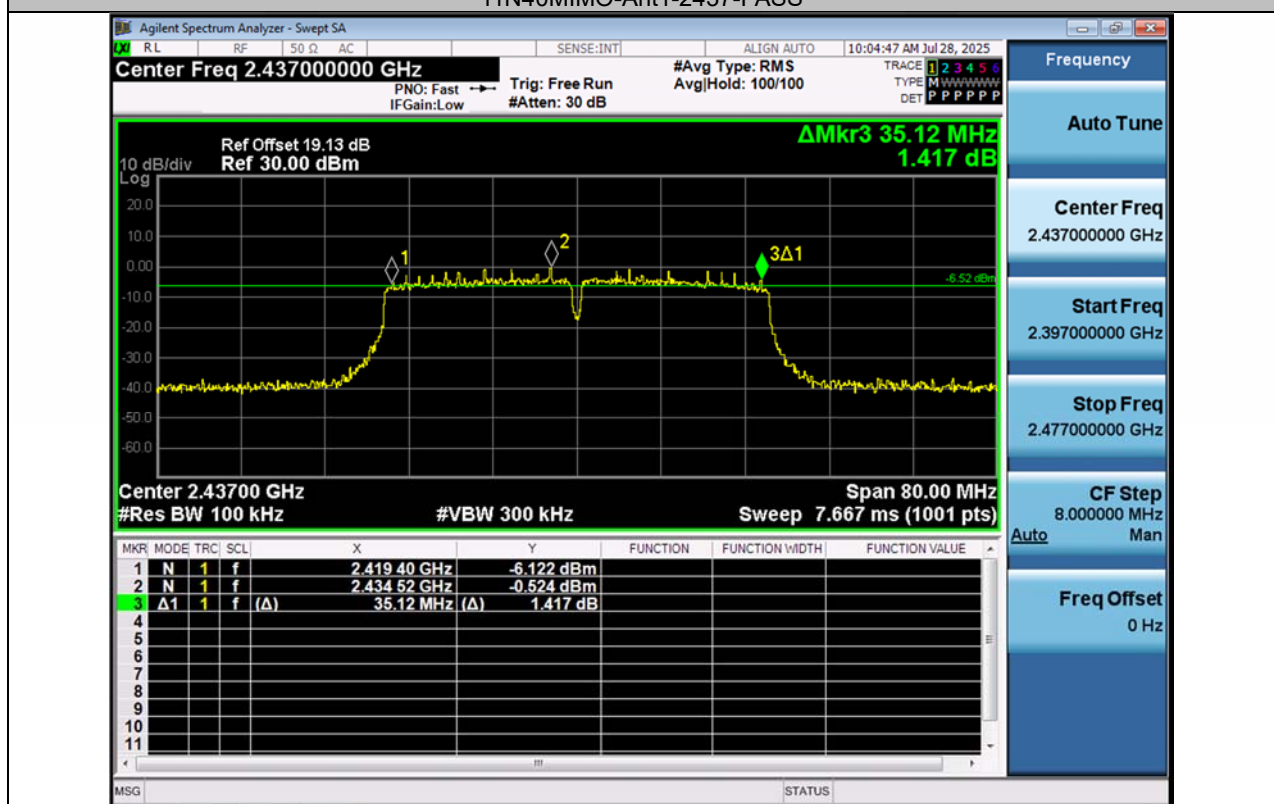
11N40MIMO-Ant2-2437-PASS
