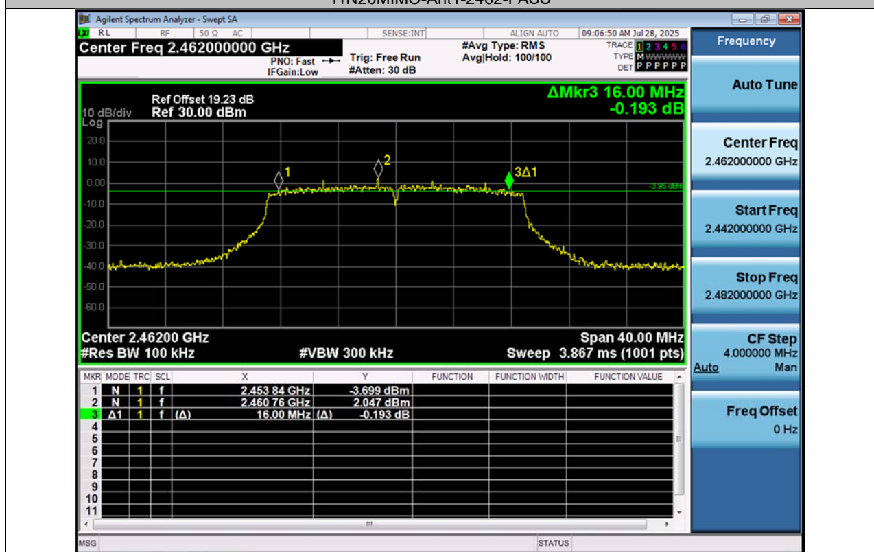
11N20MIMO-Ant2-2462-PASS
