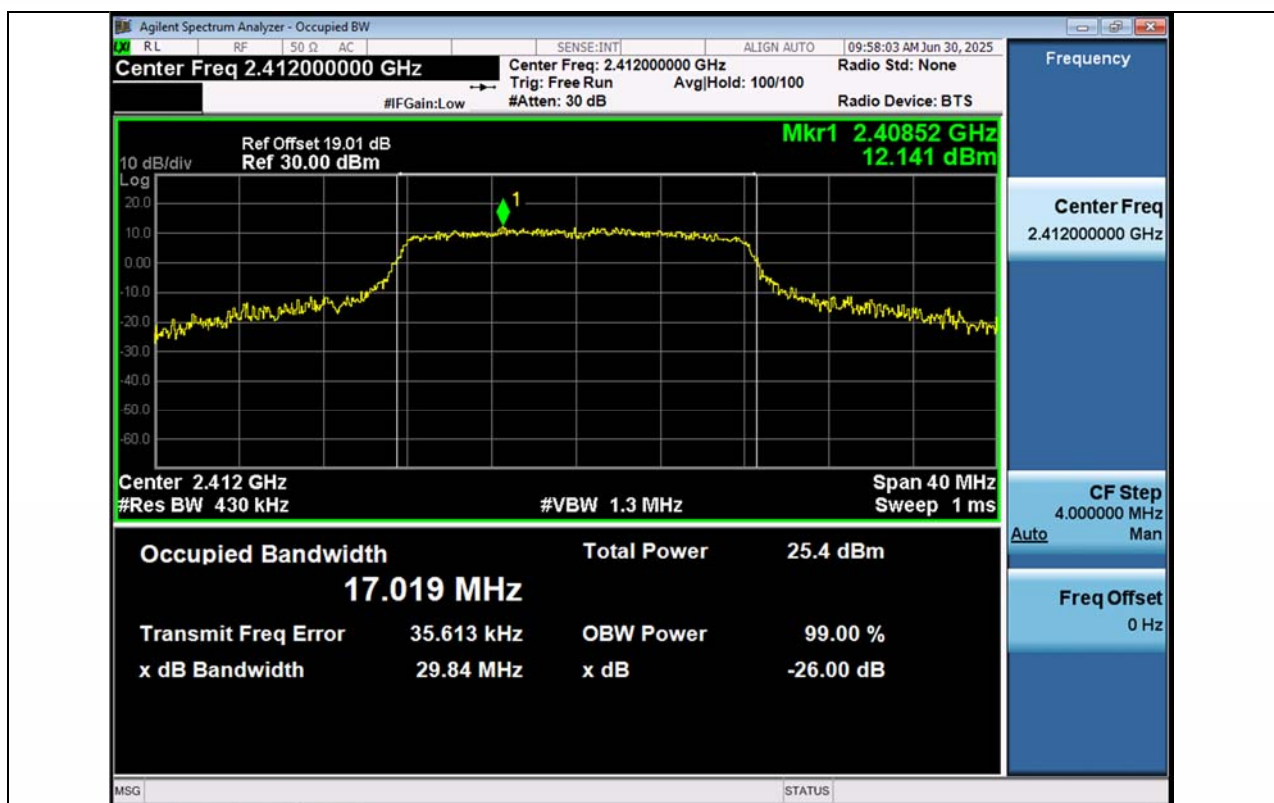
11G-Ant1-2412
