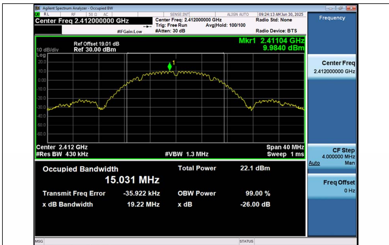
11B-Ant1-2412
