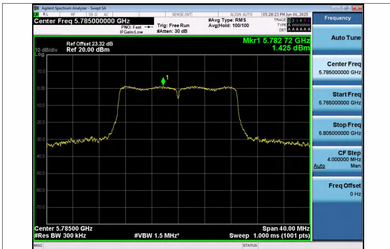
11N20SISO-Ant1-5785-PASS
