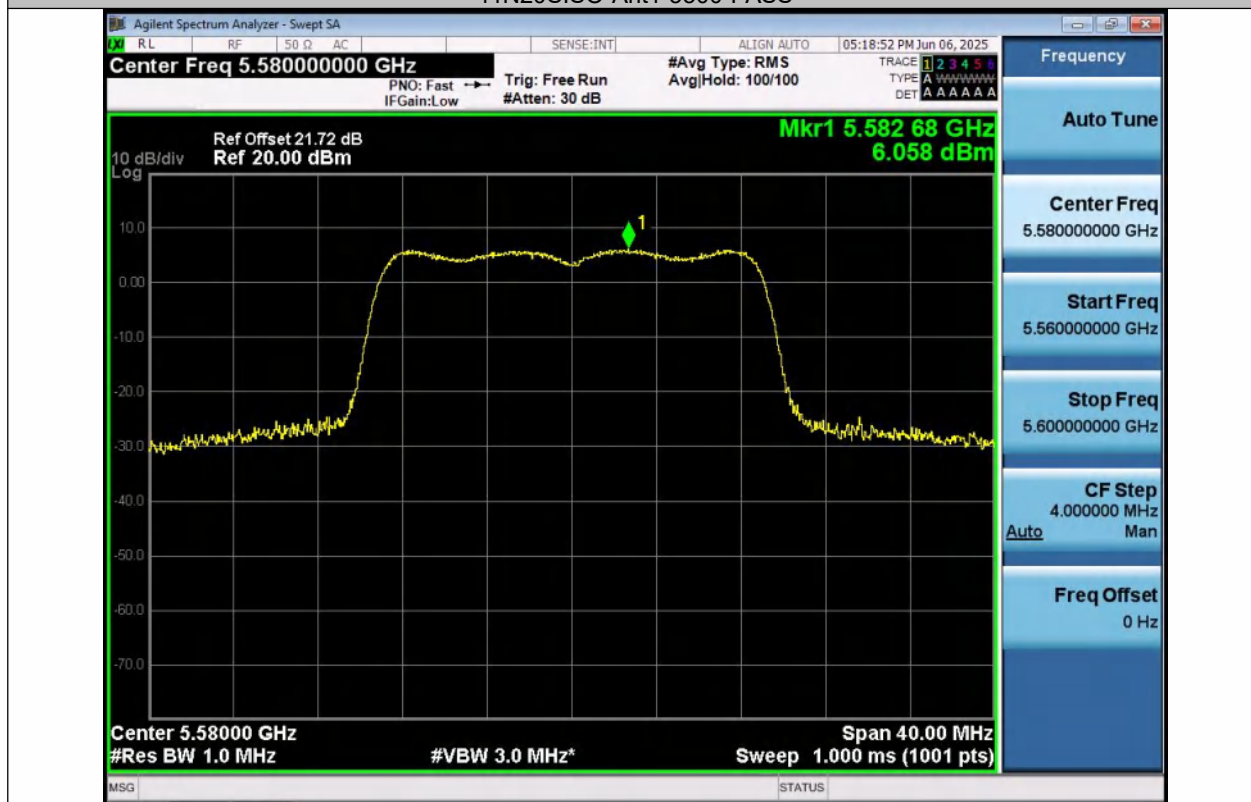
11N20SISO-Ant1-5580-PASS
