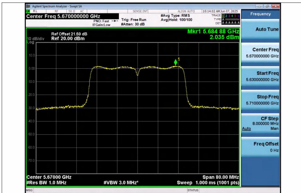
11N40SISO-Ant1-5670-PASS
