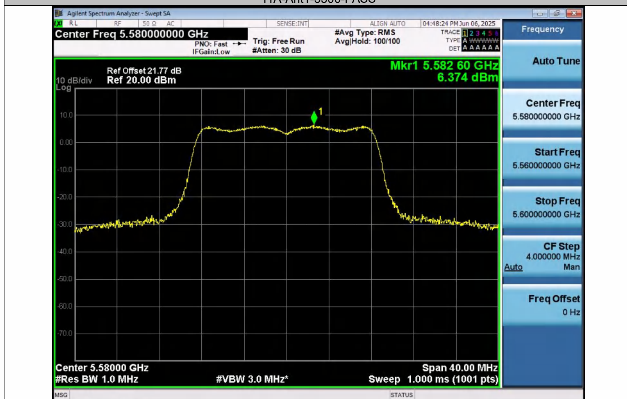
11A-Ant1-5580-PASS
