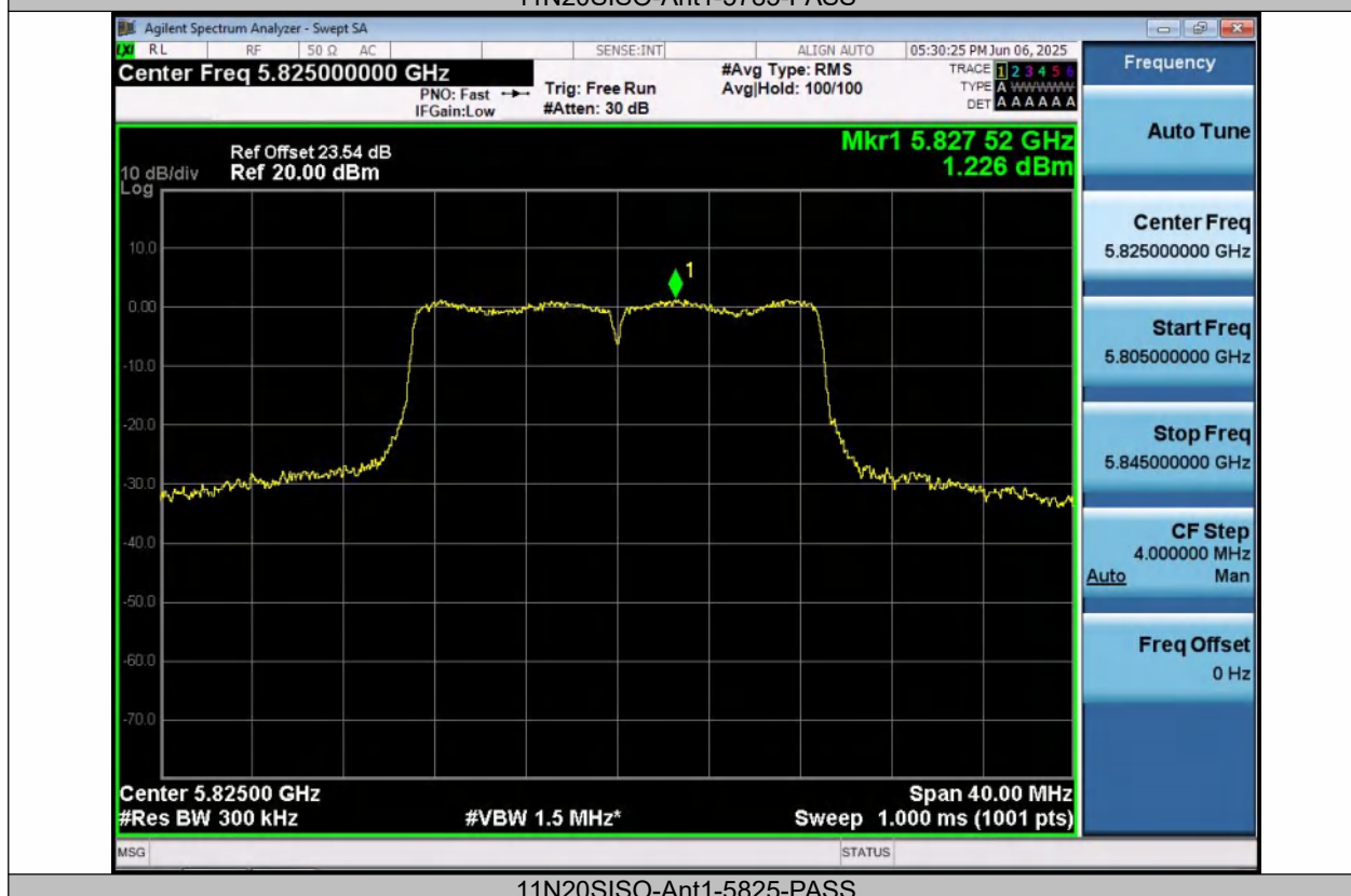
11N20SISO-Ant1-5825-PASS
