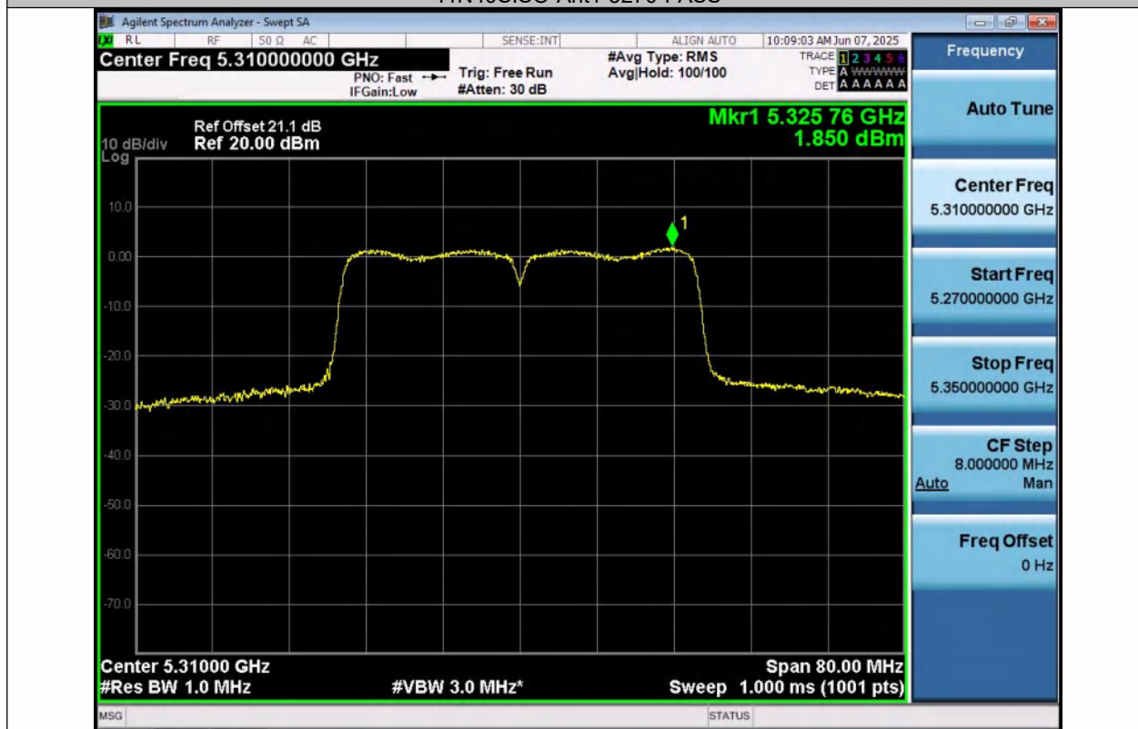
11N40SISO-Ant1-5310-PASS
