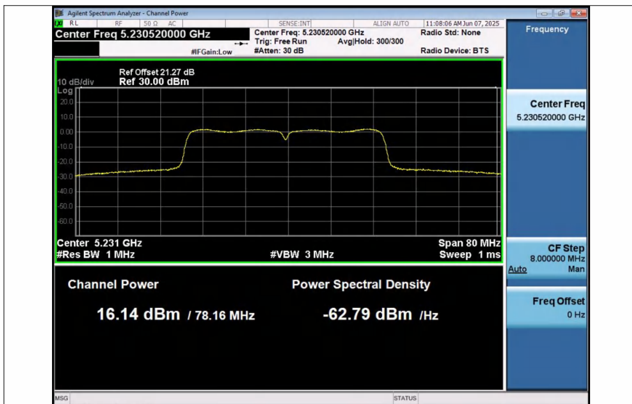
11AC40SISO-Ant1-5230-PASS
