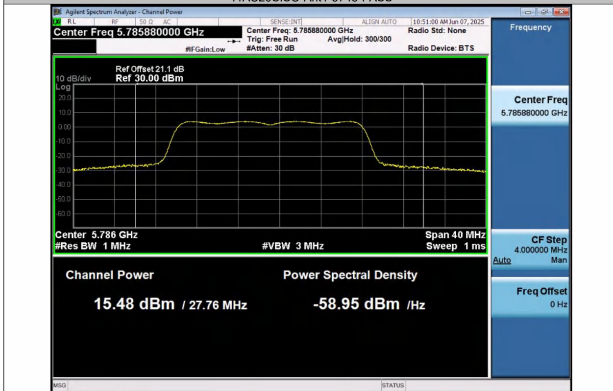
11AC20SISO-Ant1-5785-PASS
