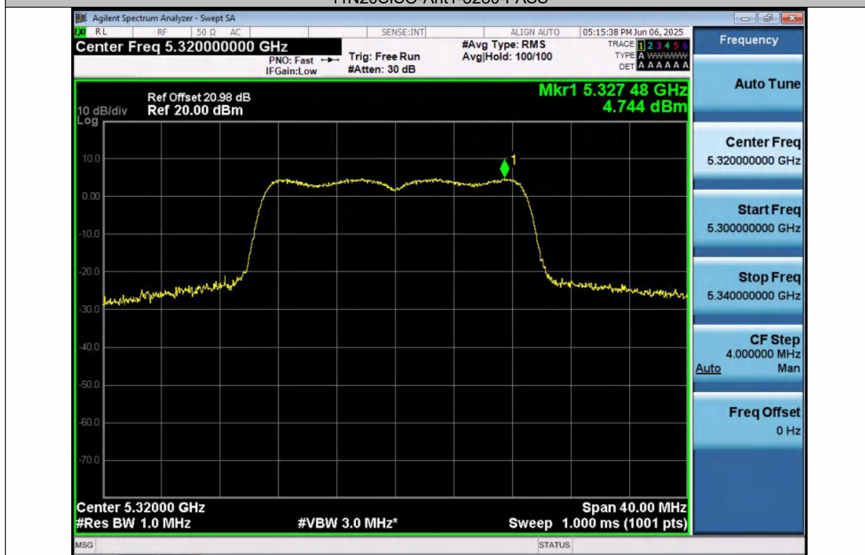
11N20SISO-Ant1-5320-PASS
