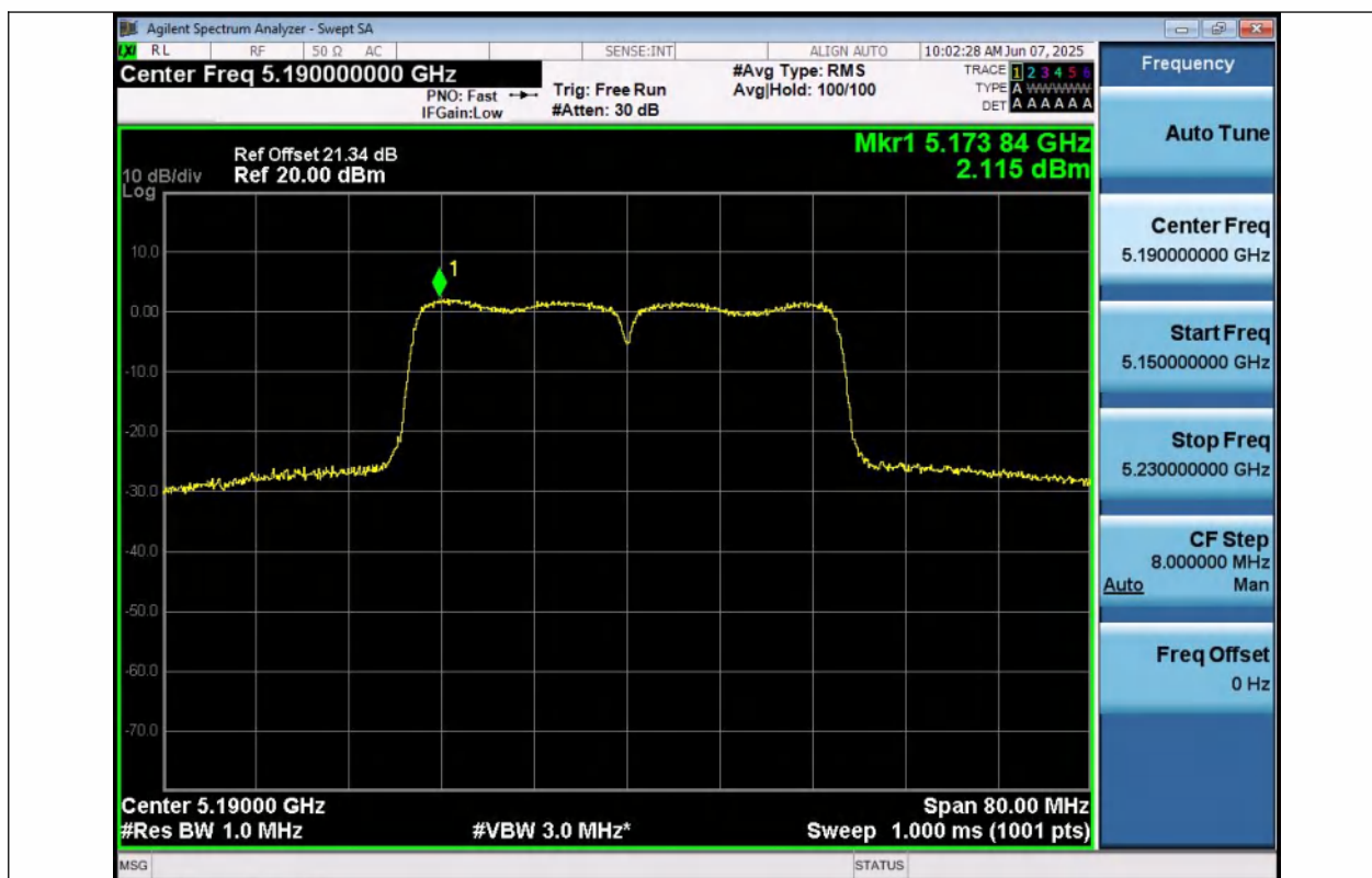
11N40SISO-Ant1-5190-PASS
