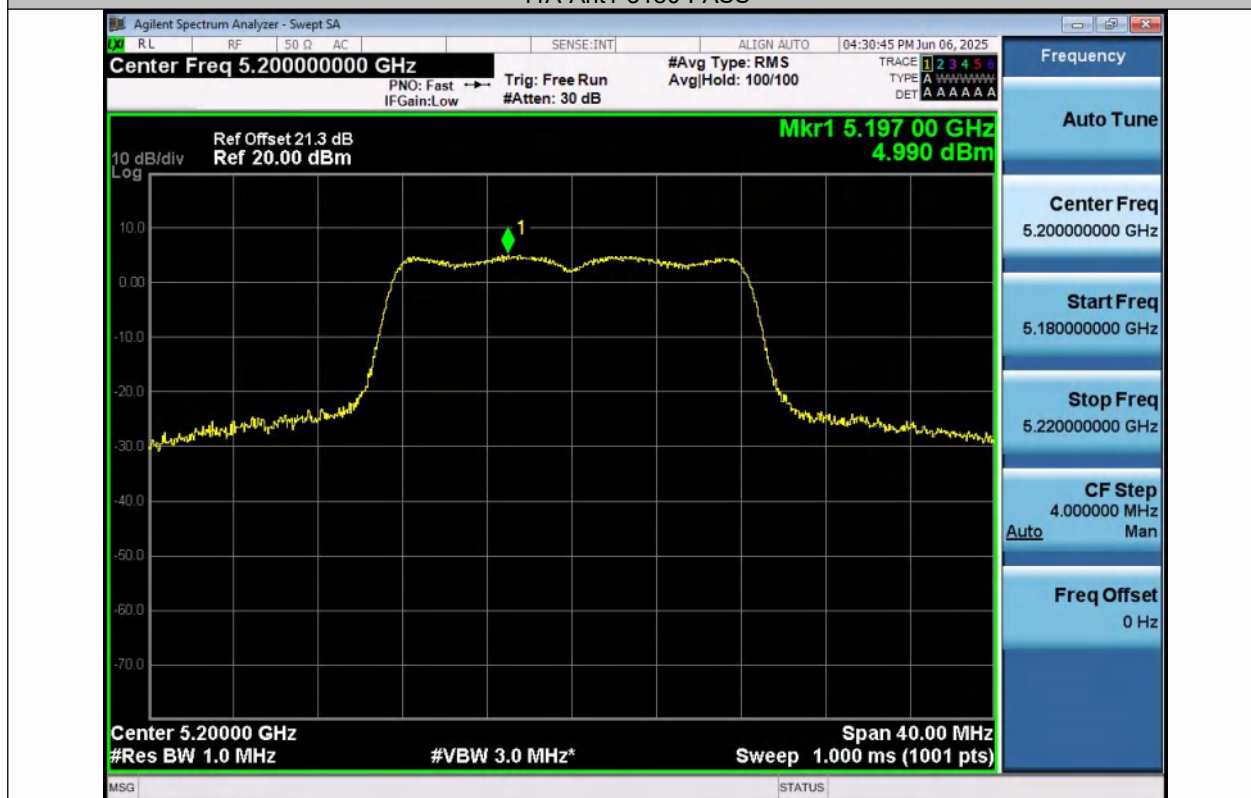
11A-Ant1-5200-PASS
