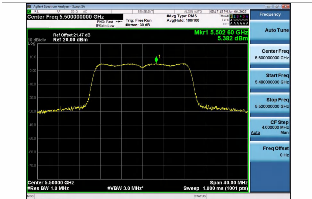
11N20SISO-Ant1-5500-PASS
