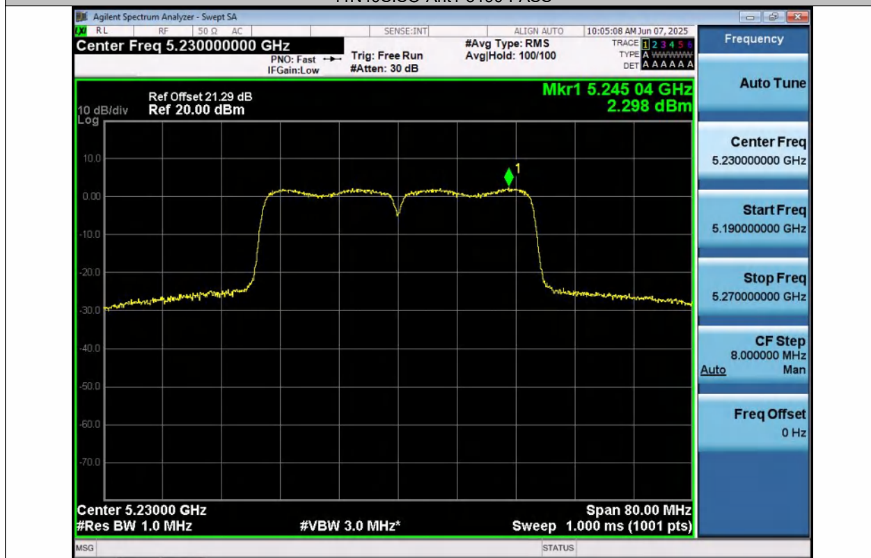
11N40SISO-Ant1-5230-PASS
