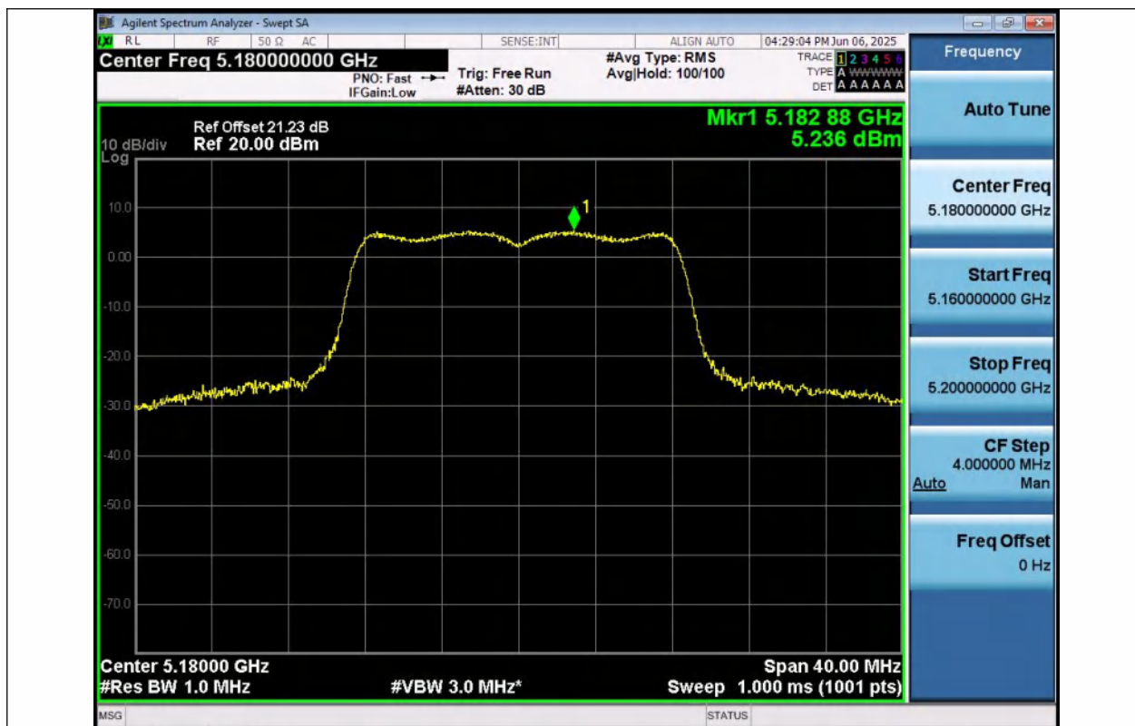
11A-Ant1-5180-PASS
