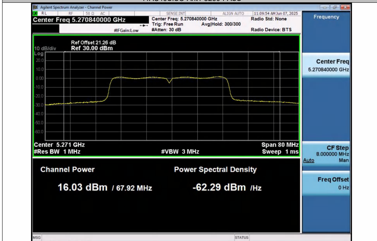
11AC40SISO-Ant1-5270-PASS
