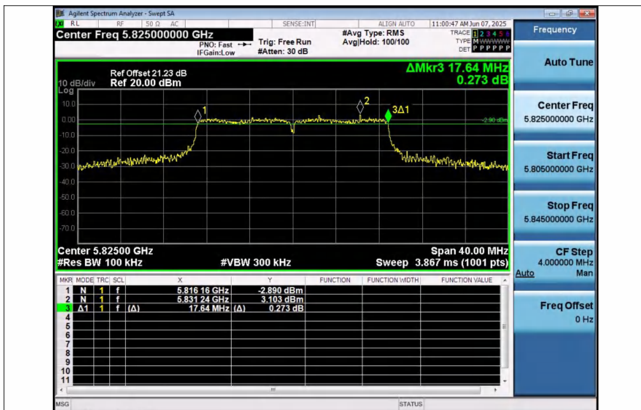
11AC20SISO-Ant1-5825-PASS
