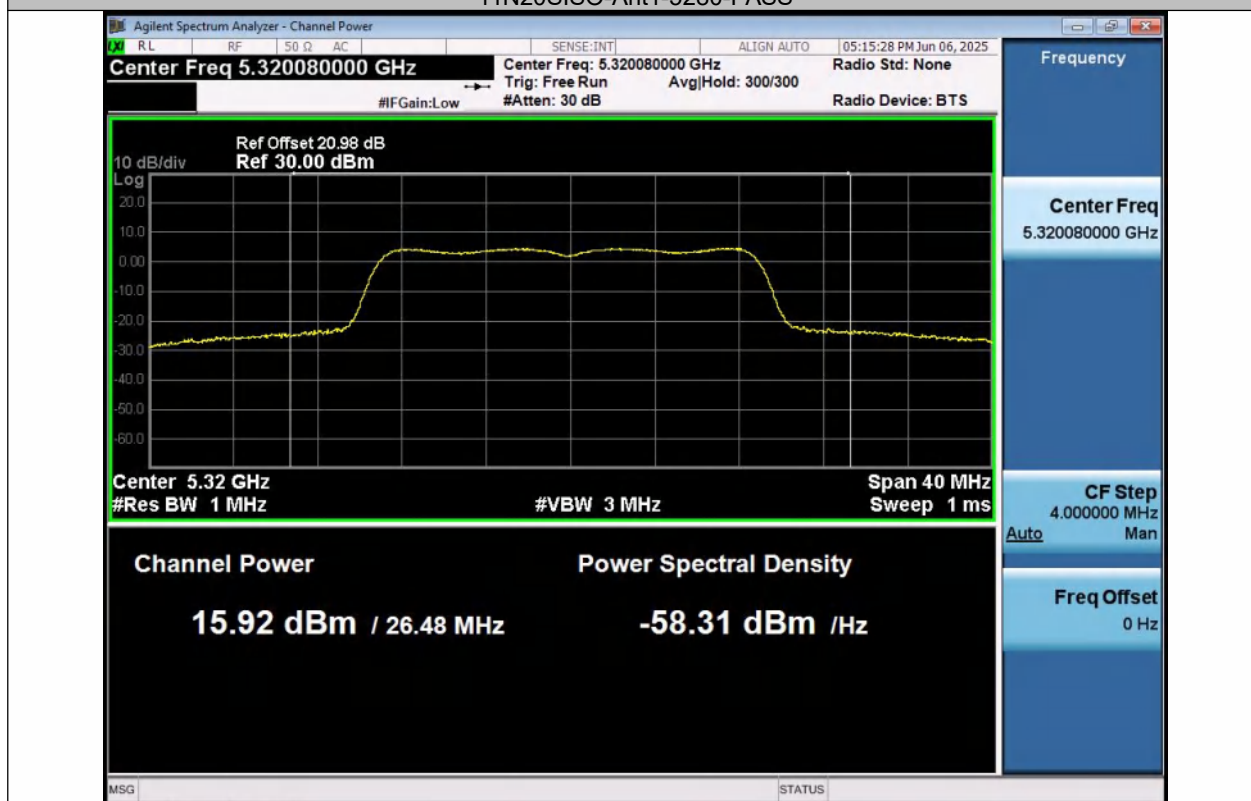
11N20SISO-Ant1-5320-PASS
