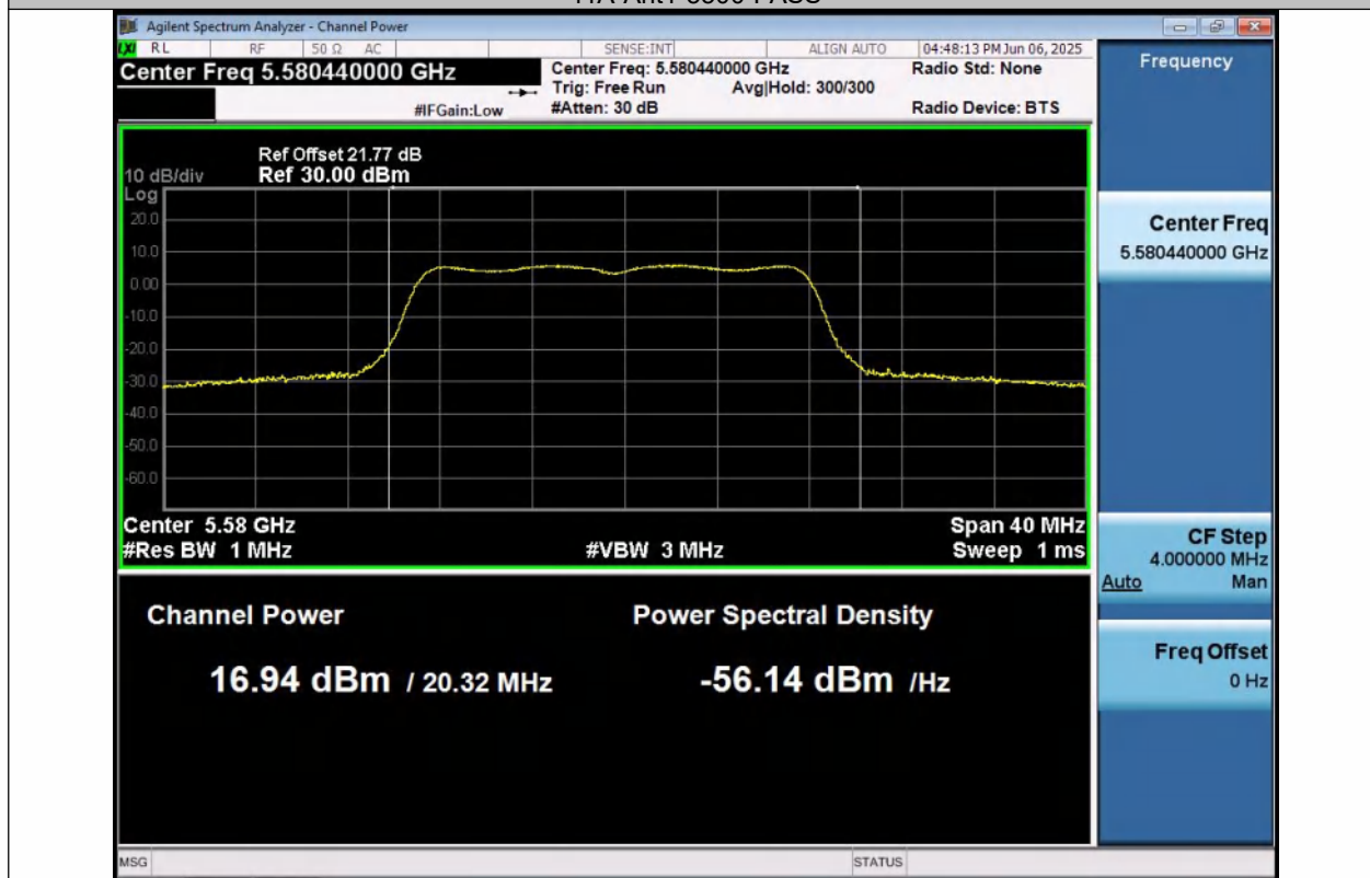
11A-Ant1-5580-PASS
