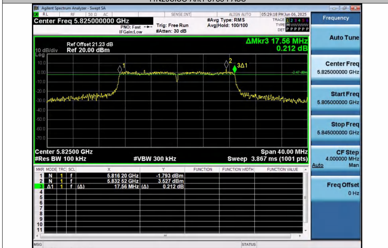
11N20SISO-Ant1-5825-PASS
