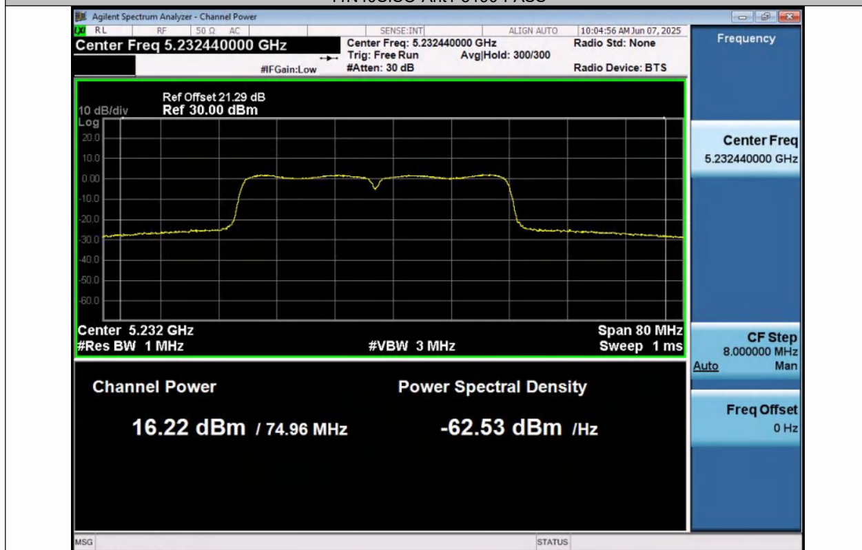
11N40SISO-Ant1-5230-PASS
