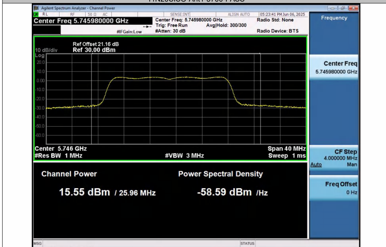
11N20SISO-Ant1-5745-PASS
