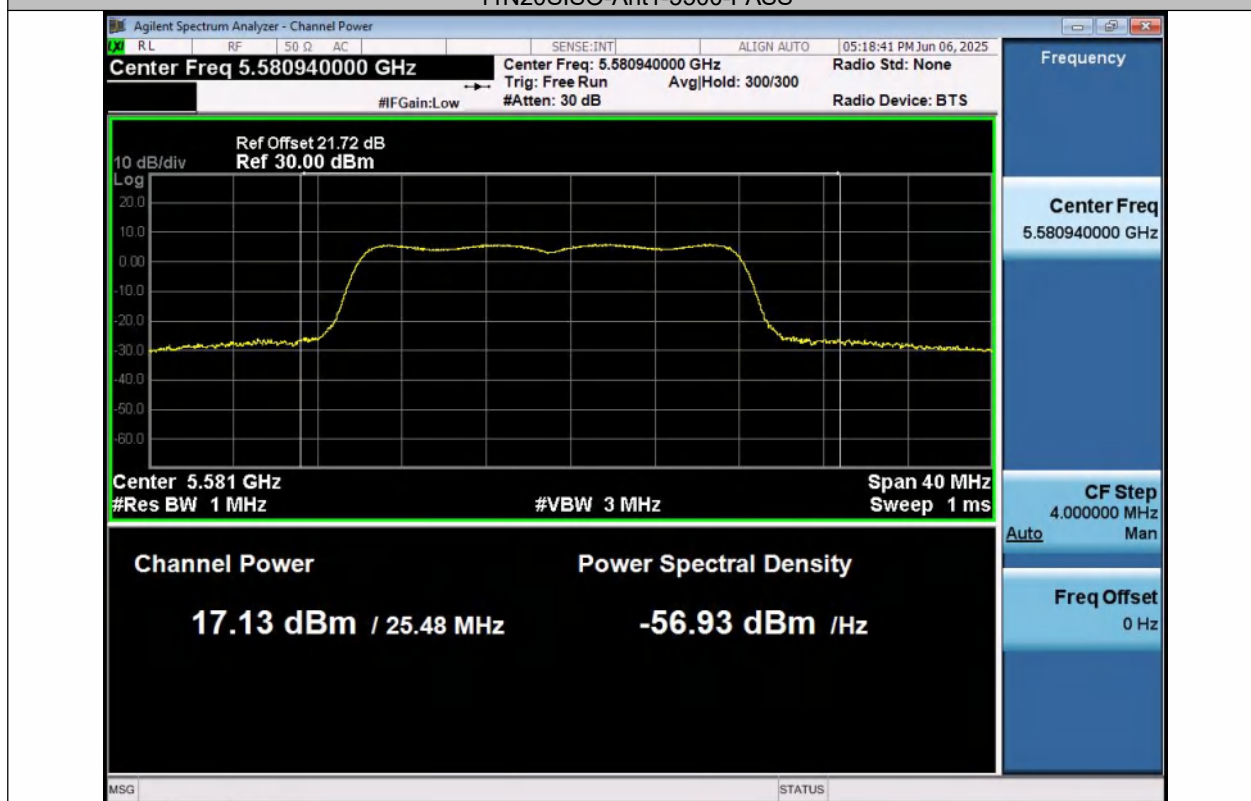
11N20SISO-Ant1-5580-PASS
