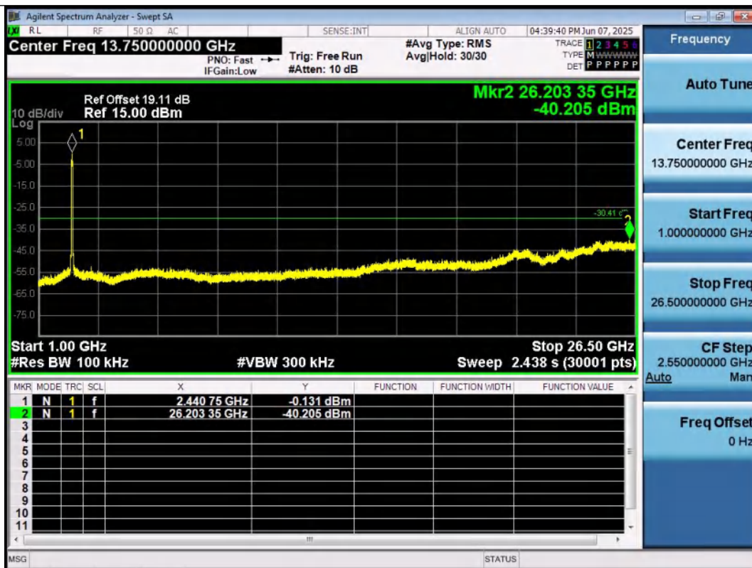
11N40SISO-Ant1-2437-1000~26500-PASS
