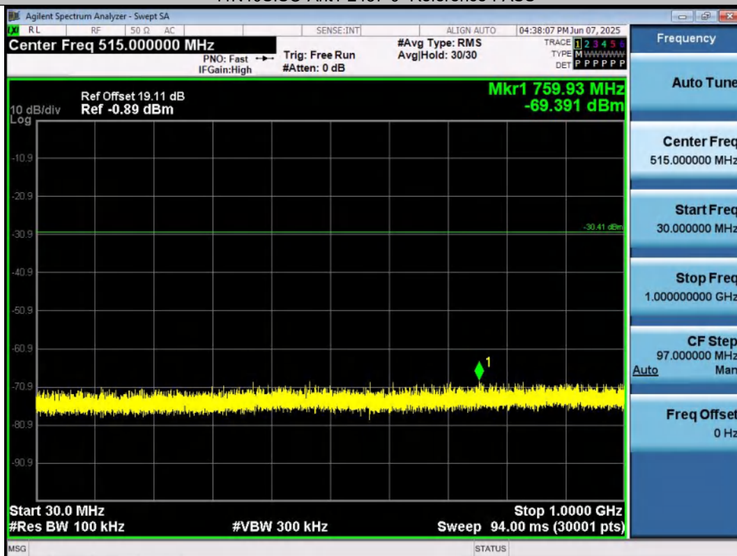
11N40SISO-Ant1-2437-30~1000-PASS
