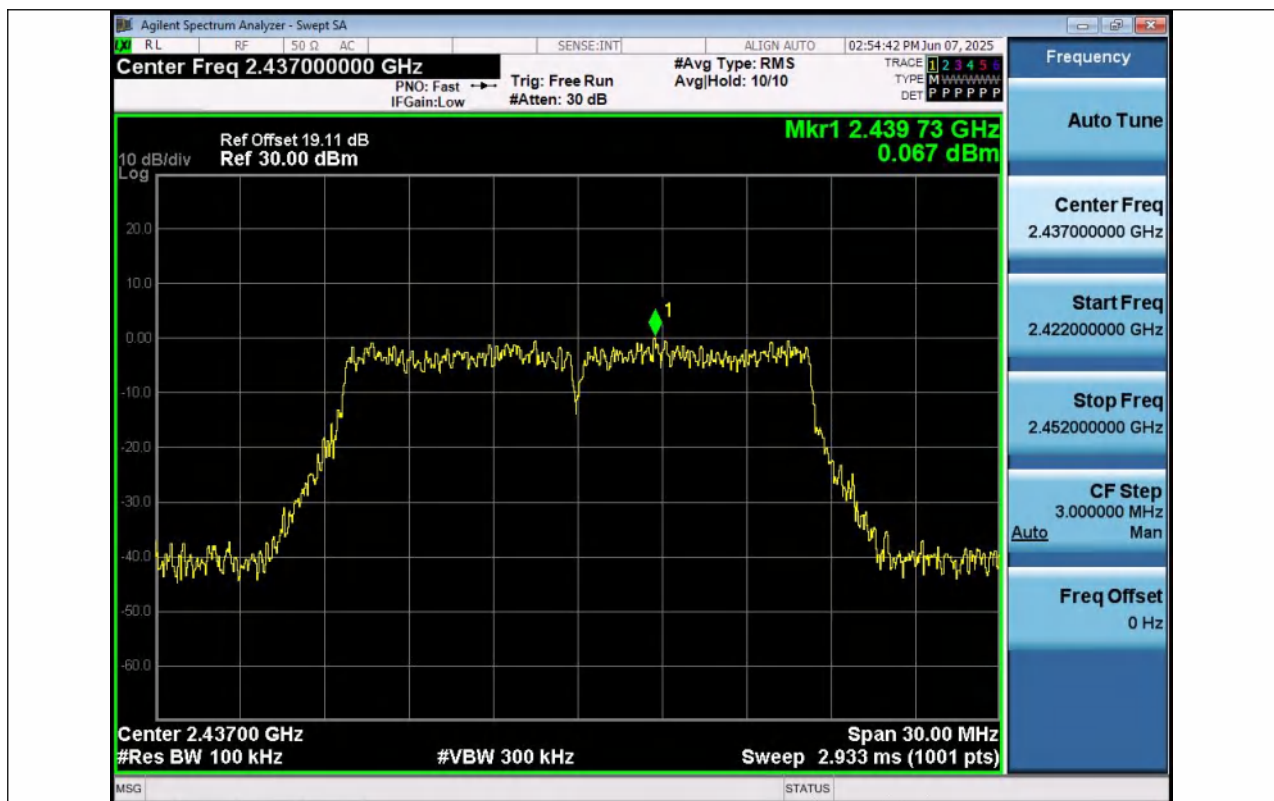
11G-Ant1-2437-0~Reference-PASS
