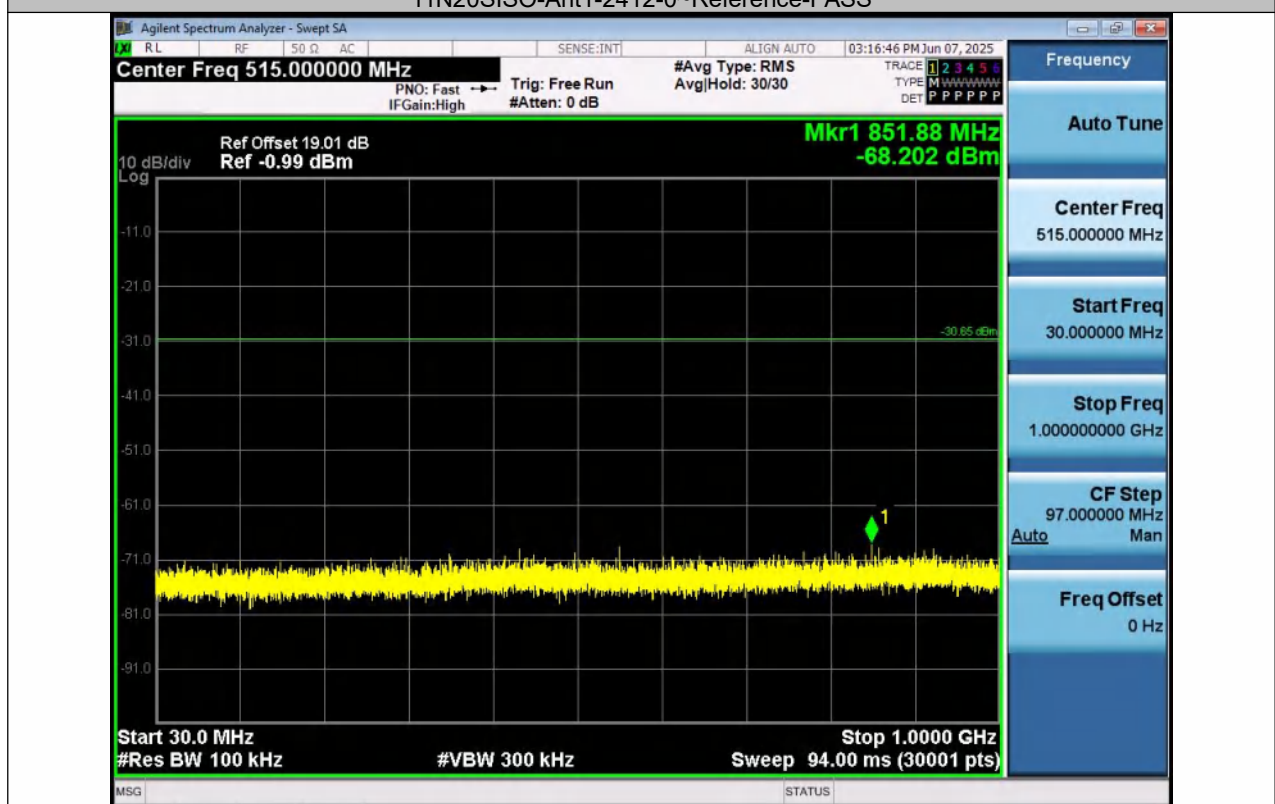
11N20SISO-Ant1-2412-30~1000-PASS
