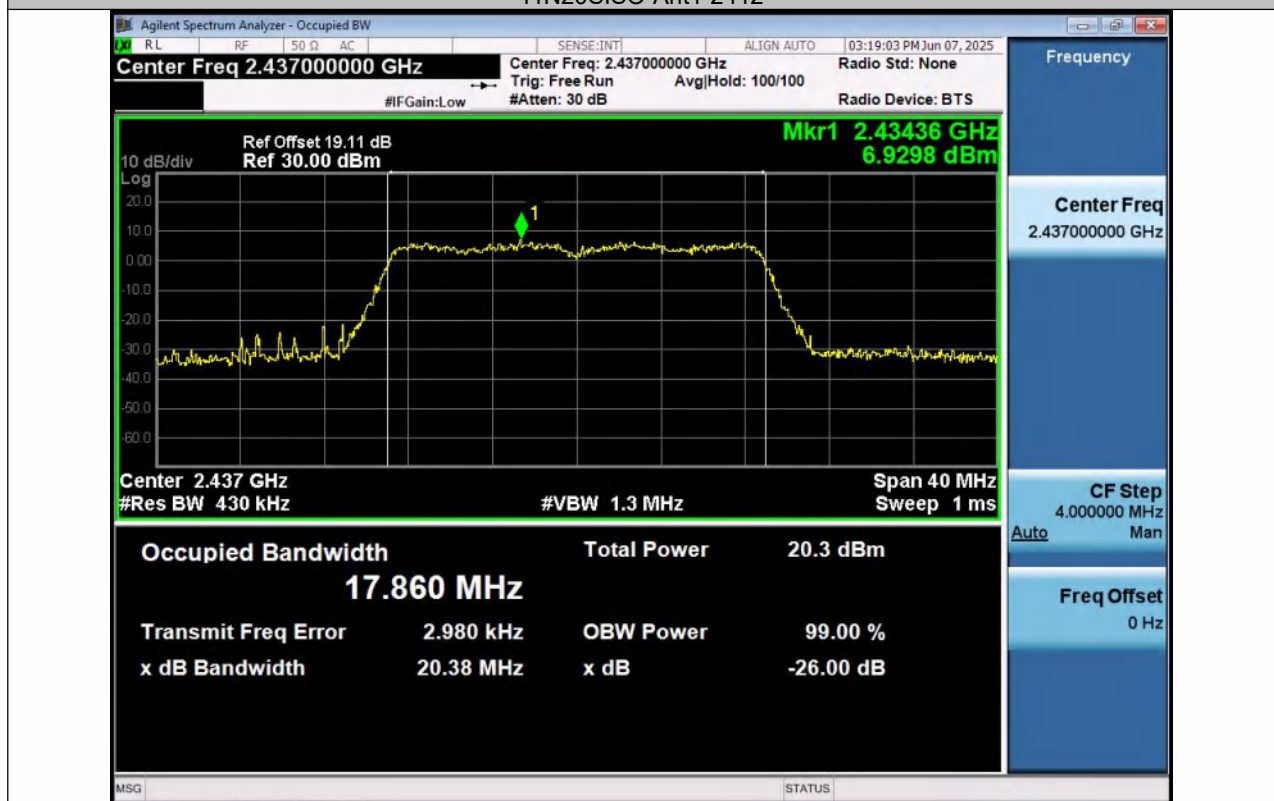
11N20SISO-Ant1-2437
