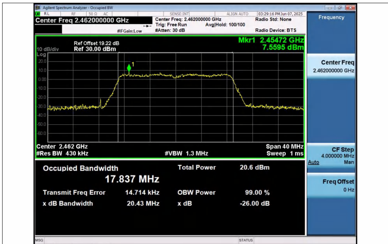
11N20SISO-Ant1-2462
