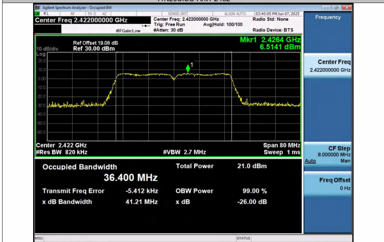
11N40SISO-Ant1-2422
