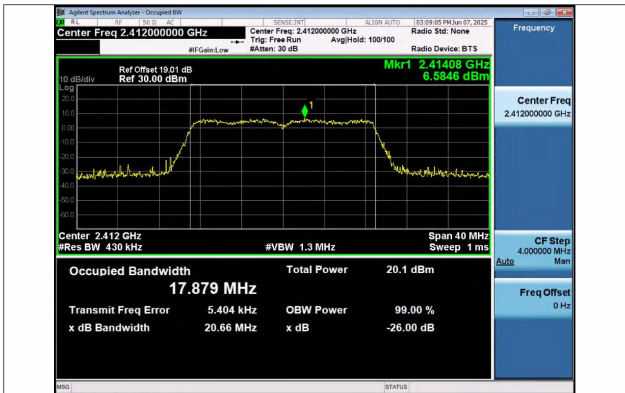
11N20SISO-Ant1-2412
