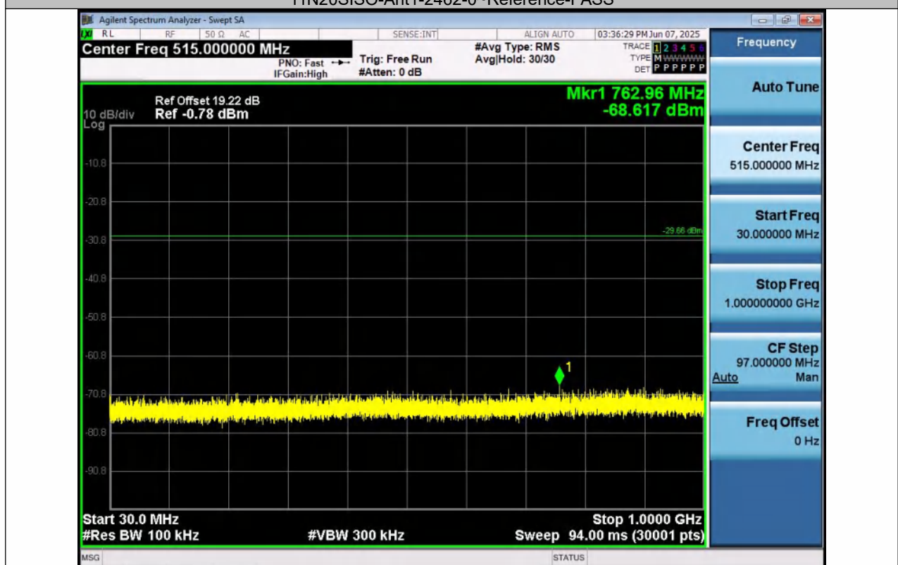
11N20SISO-Ant1-2462-30~1000-PASS
