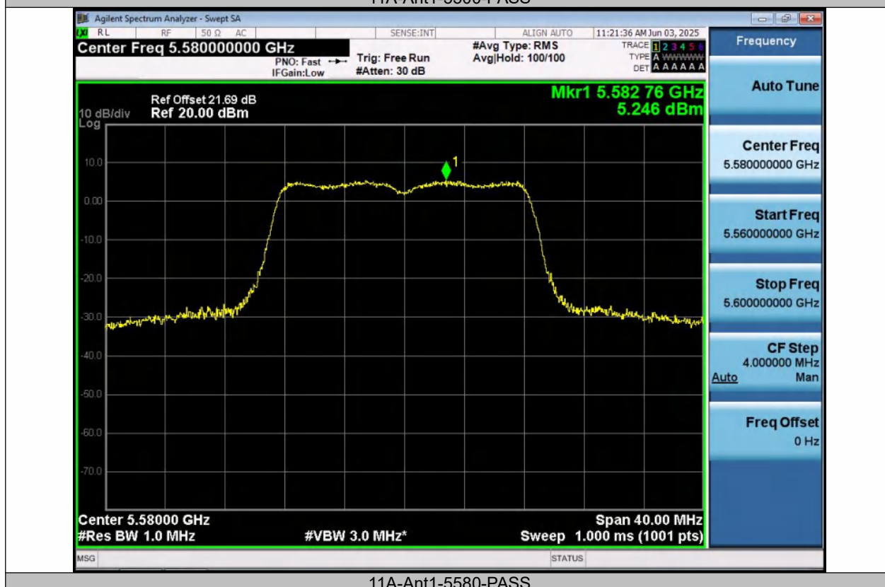
11A-Ant1-5580-PASS
