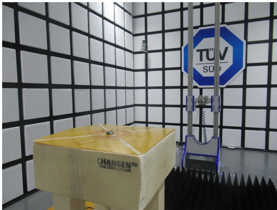
Radiated Emission Test: 18GHz to 40GHz
