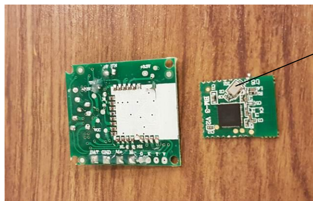
Lock board & radio board (top view)
