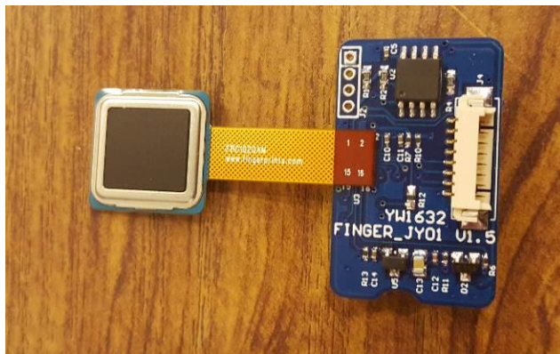
Fingerprint board (bottom view)
