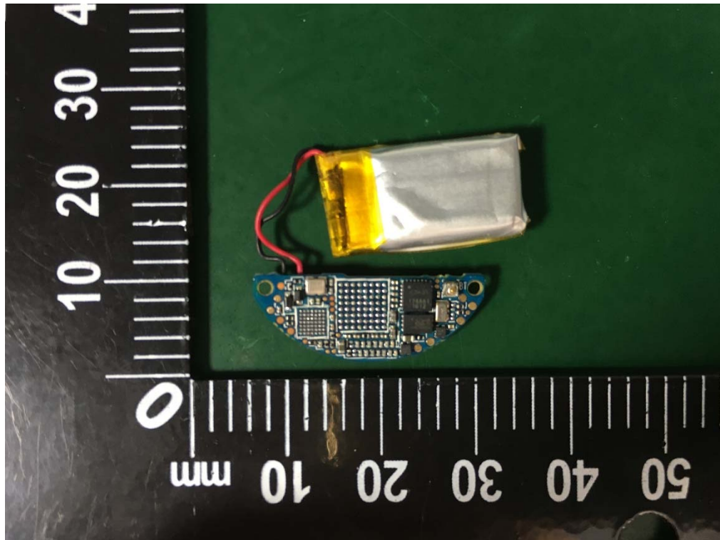
EUT Photo #3 PCB View
