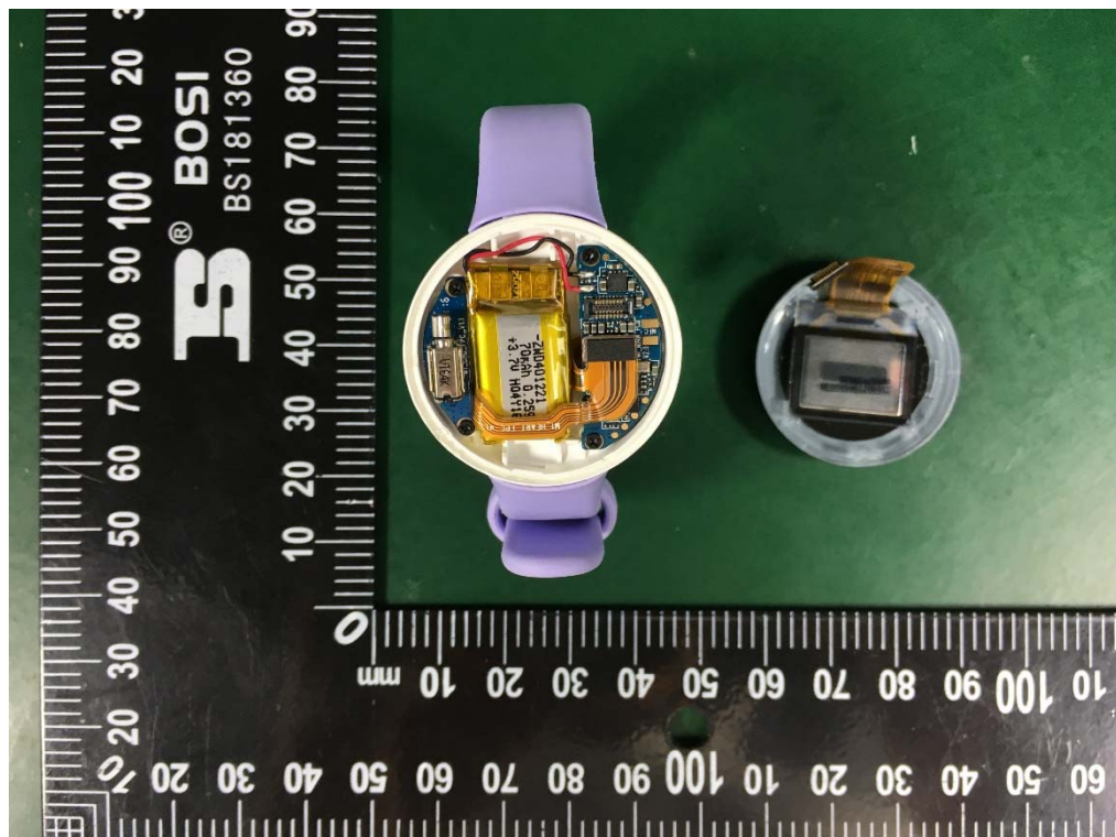
EUT Photo #1 Uncover View
