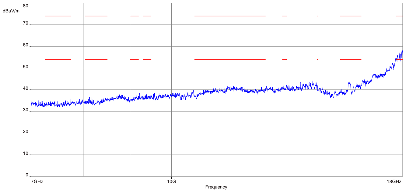
Plot 10: Highest channel, 7 GHz to 18 GHz, vertical & horizontal polarization, peak
