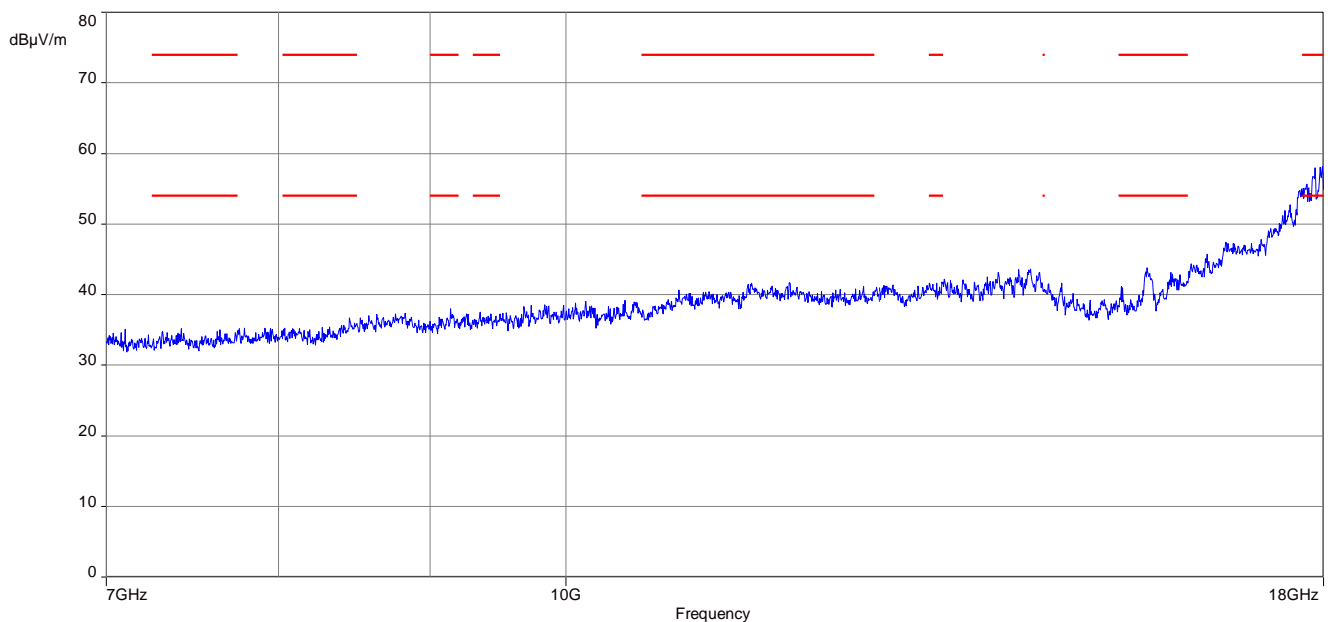
Plot 6: Middle channel, 7 GHz to 18 GHz, vertical & horizontal polarization, peak
