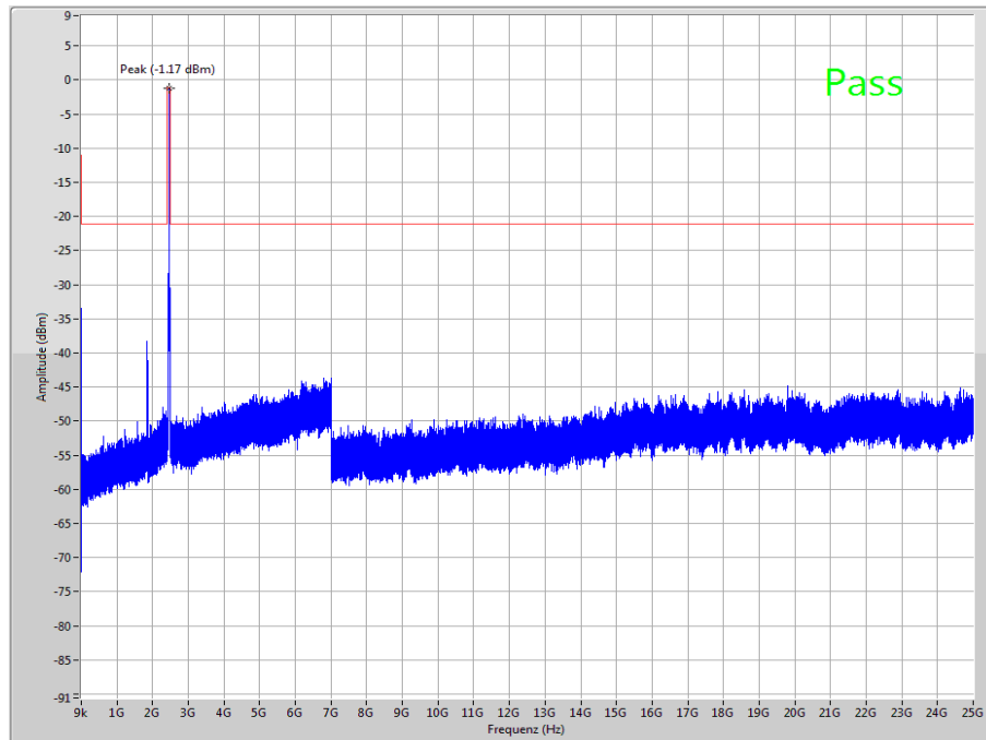
Plot 5: Channel 11, 2462 MHz, up to 25 GHz
