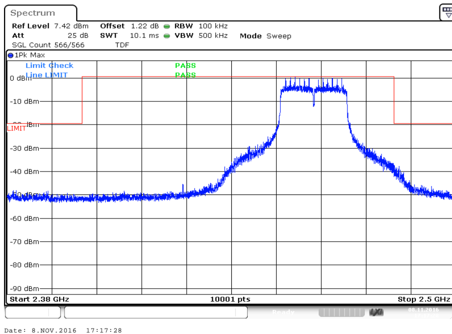
Plot 6: Channel 11, 2462 MHz, zoomed carrier
