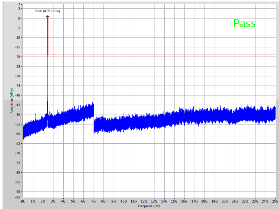
Plot 3: Channel 6, 2437 MHz, up to 25 GHz
