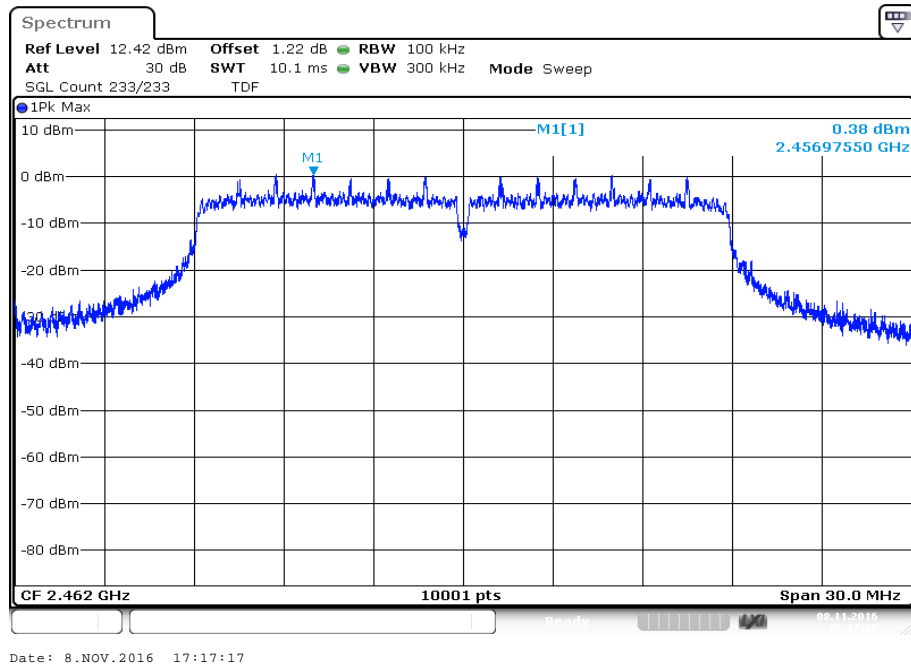
Plot 3: Channel 11, 2462 MHz
