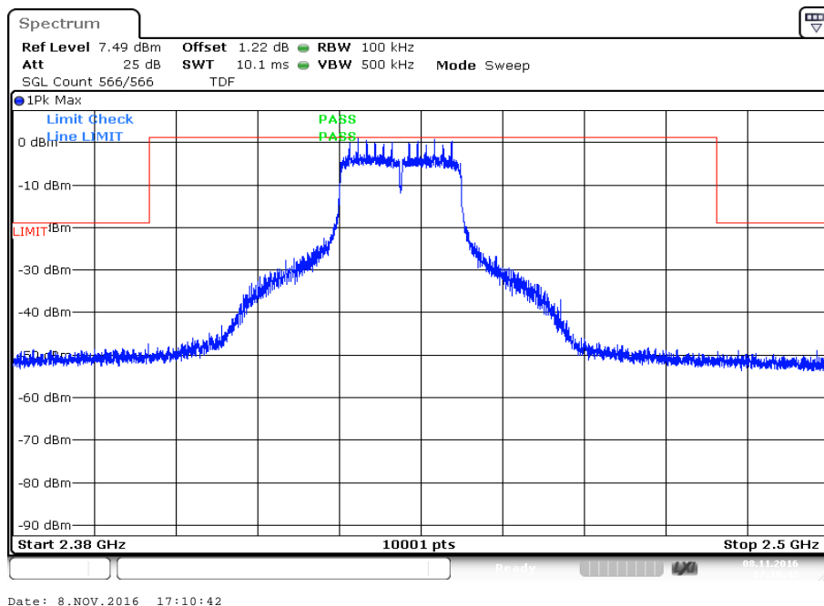
Plot 4: Channel 6, 2437 MHz, zoomed carrier
