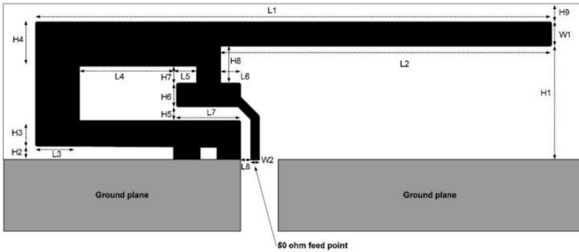
Figure 4: Antenna Dimensions
