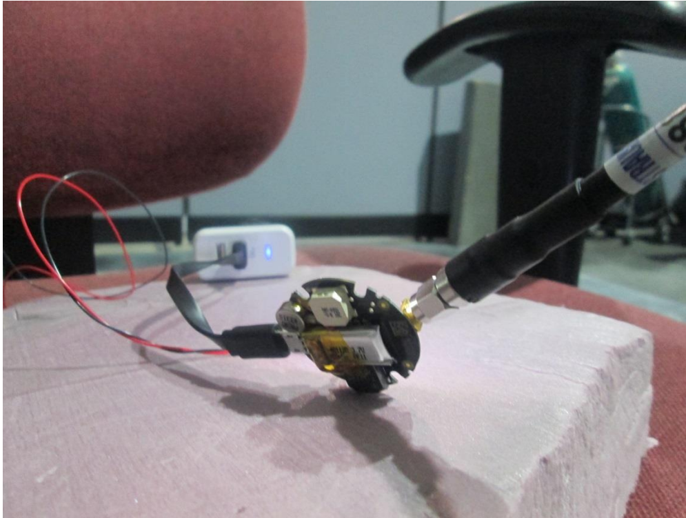
Conducted Emission at the Antenna Port (Close-up View)
