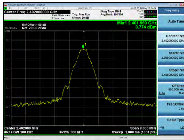
Reference Power
