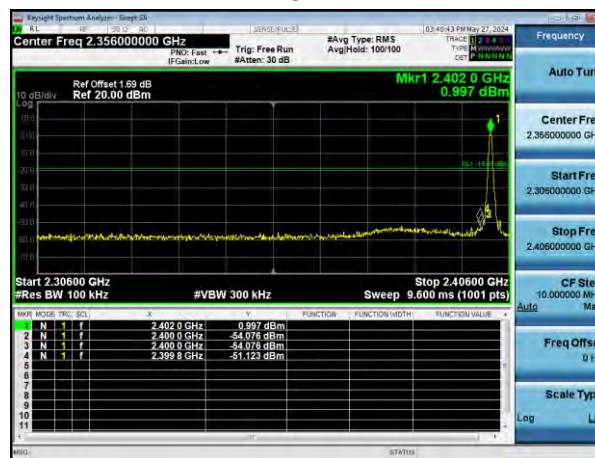
Band-edge Emission
