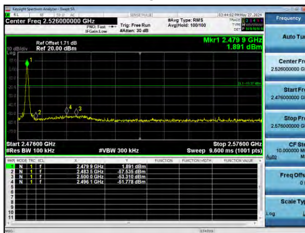
Band-edge Emission
