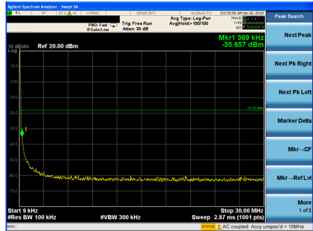
O-QPSK on channel 15
