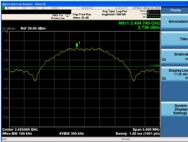
O-QPSK on channel 00
