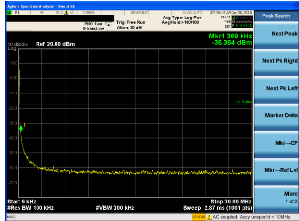
O-QPSK on channel 00
