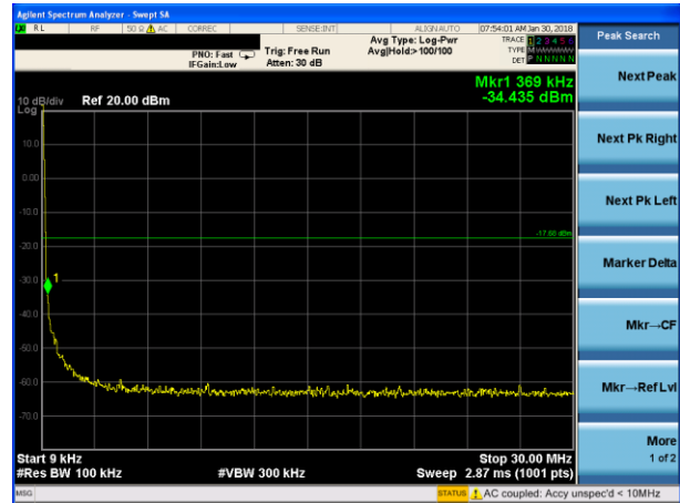
O-QPSK on channel 07
