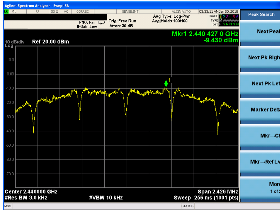
Power spectral density plot on channel 07
