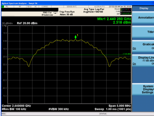
O-QPSK on channel 07
