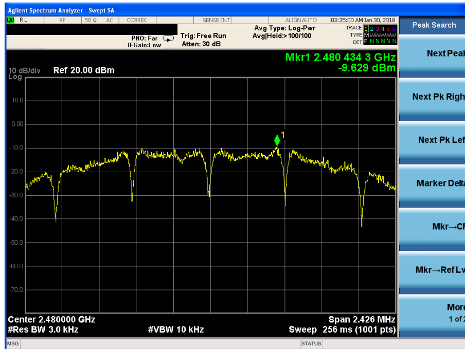
Power spectral density plot on channel 15
