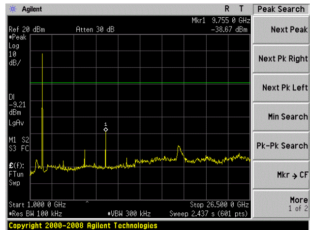
O-QPSK on channel 8
