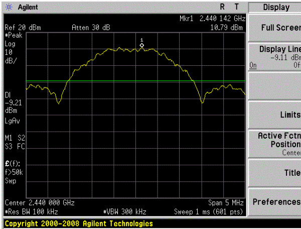
O-QPSK on channel 8
