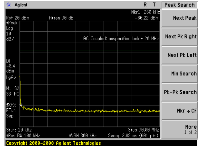
O-QPSK on channel 01
