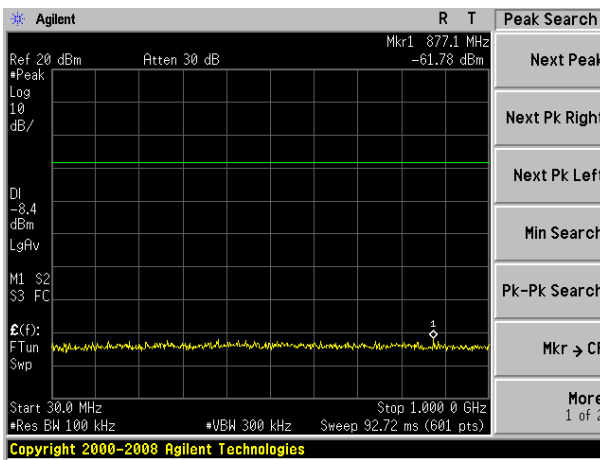
O-QPSK on channel 01
