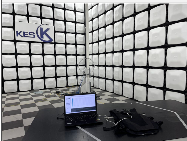
Radiated test
