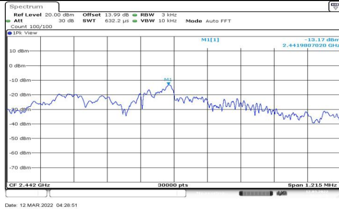
2M_Ant1_2442
