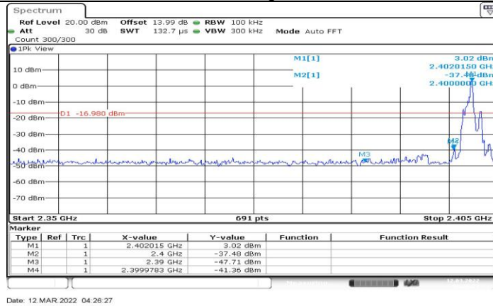
2M_Ant1_Low_2402
