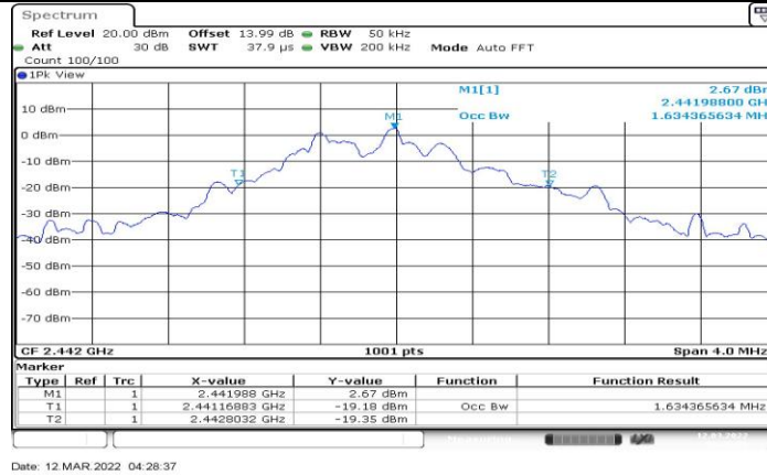
2M_Ant1_2442
