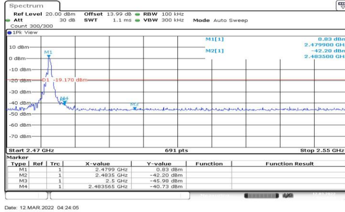
1M_Ant1_High_2480
