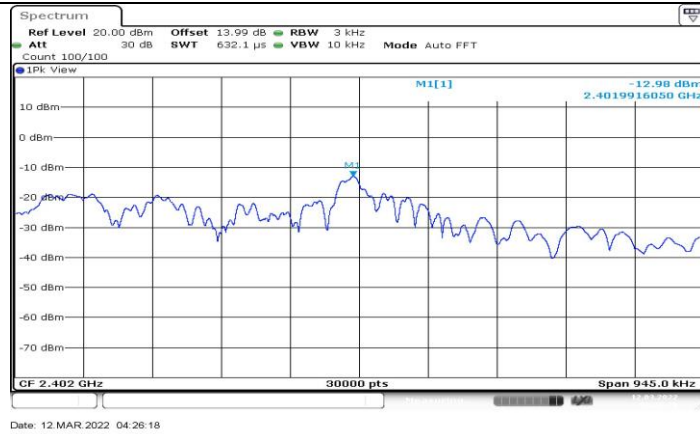
2M_Ant1_2402
