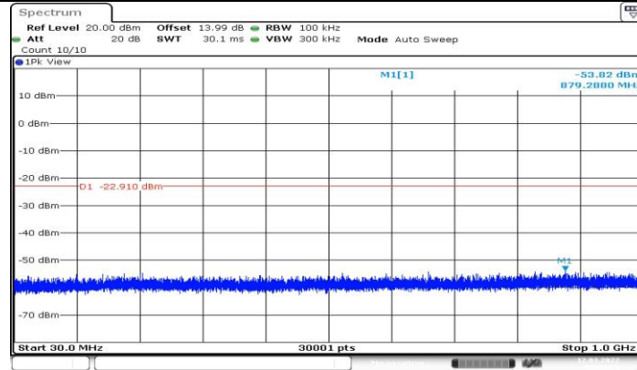
250K_Ant1_2442_0~Reference
