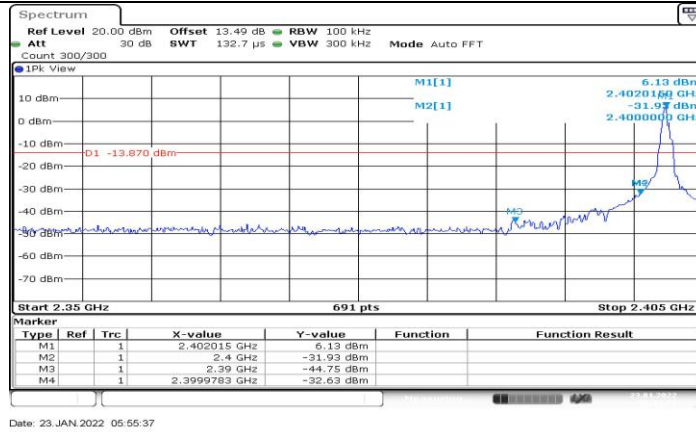
1M_Ant1_Low_2402
