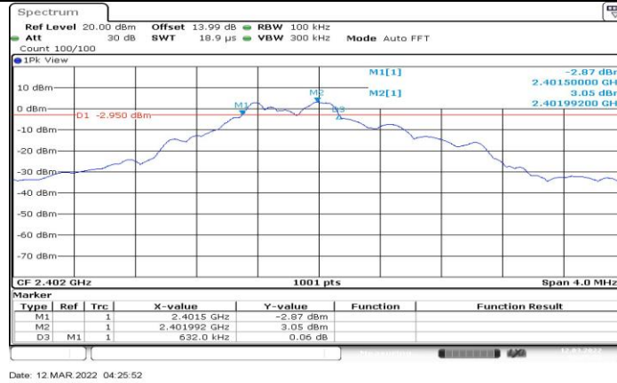
2M_Ant1_2402
