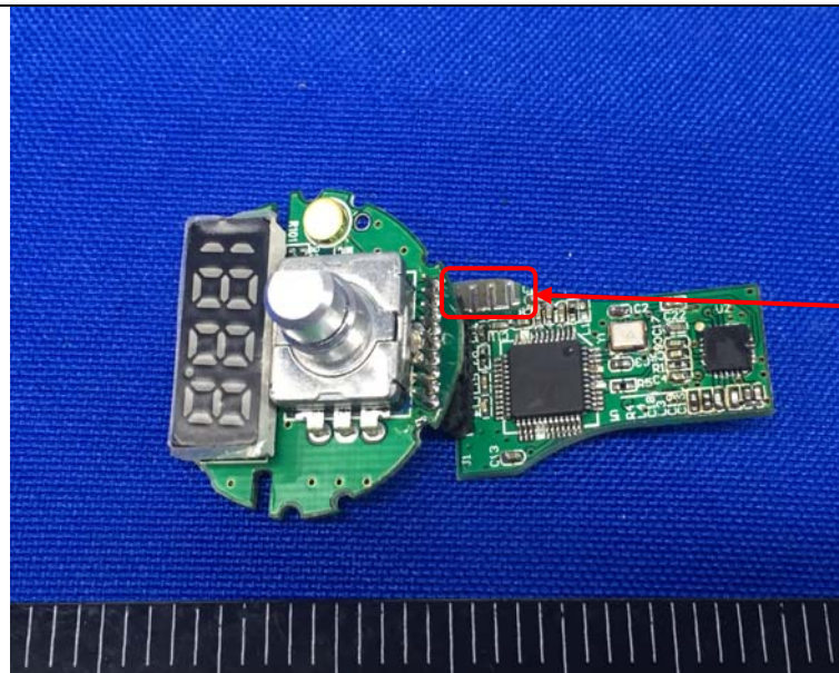
BT Antenna
