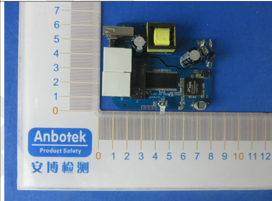
2. Figure The EUT-PCB View
