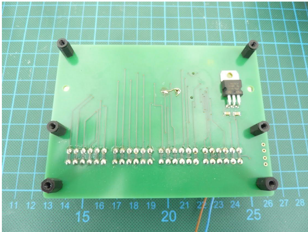
Bottom view Host
