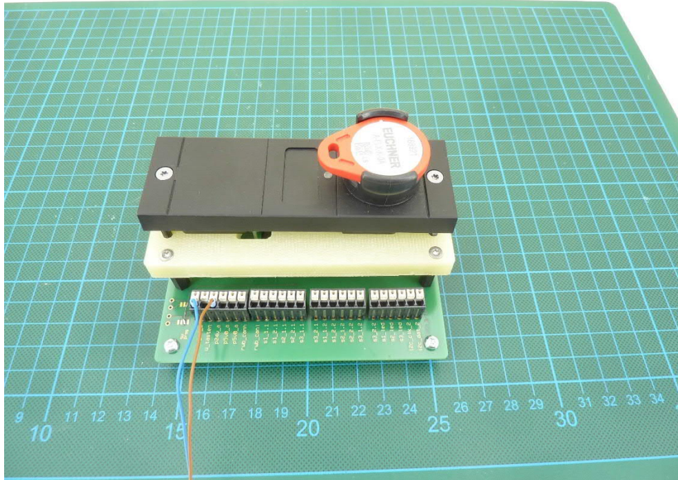
Test setup view with Host
