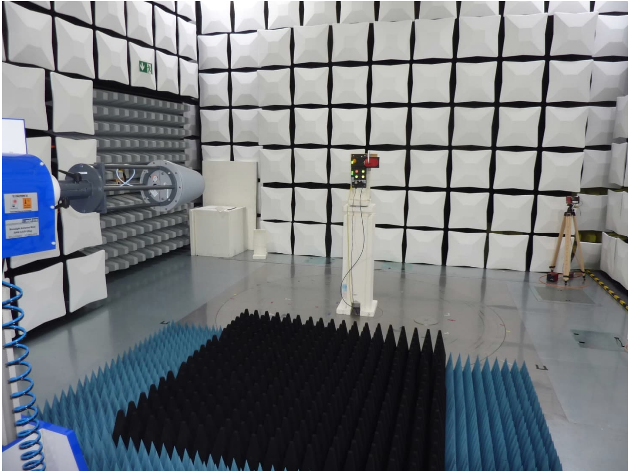
Test setup semi anechoic chamber (1 GHz to 2 GHz)
