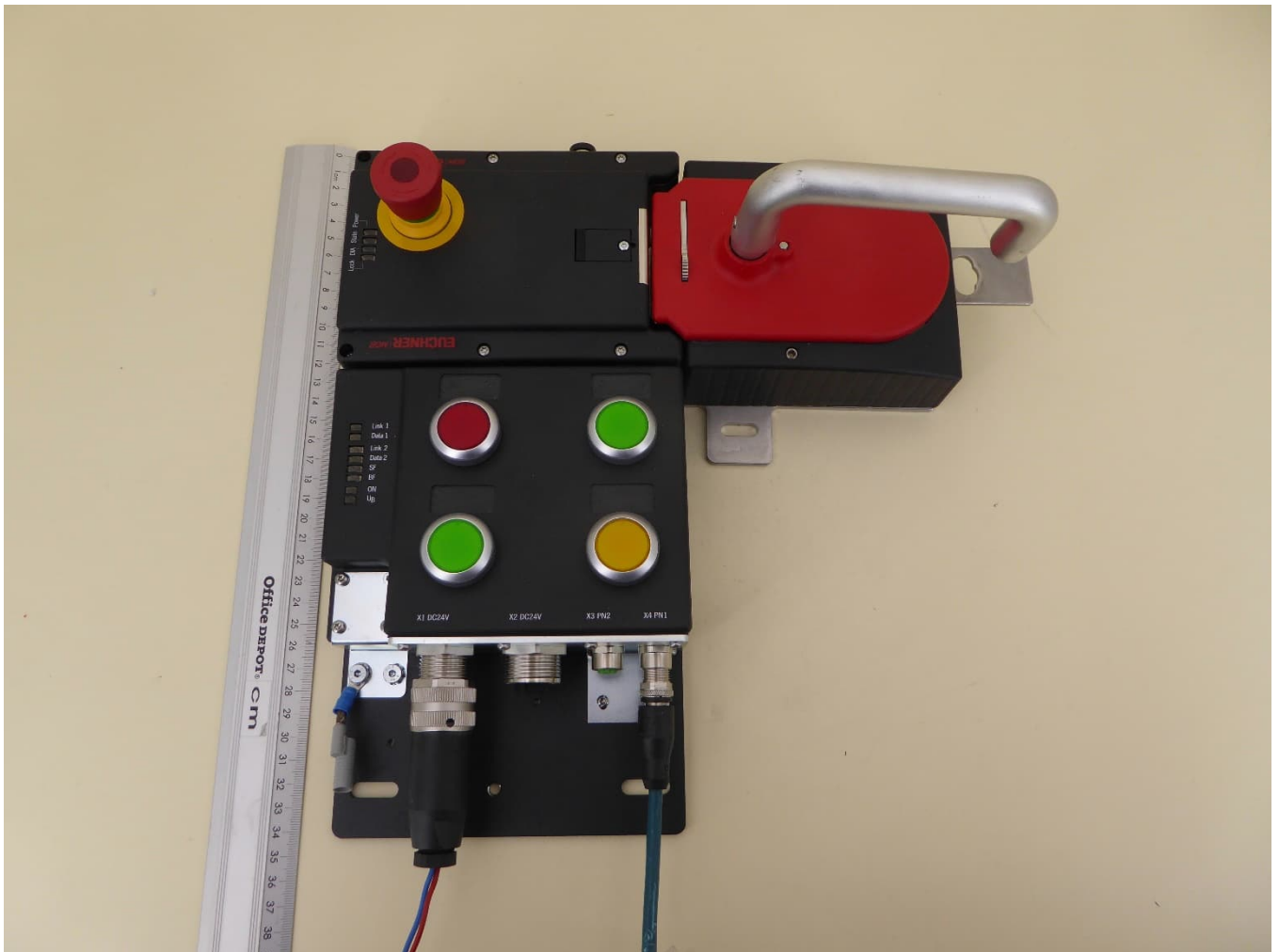
Test setup with handle module
