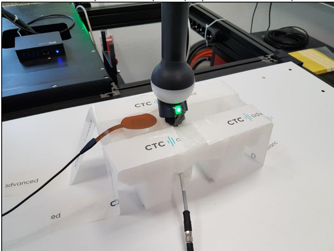
Photo 4: Test pictures – Start position (use position – 0mm distance)
