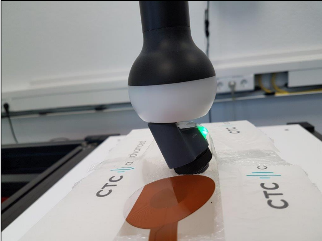
Photo 6: Test pictures – Start position (use position – 0mm distance)
