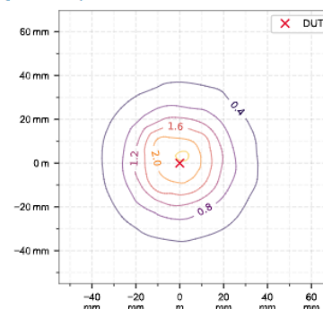
H-field magnitude [RMS] at lowest plane
