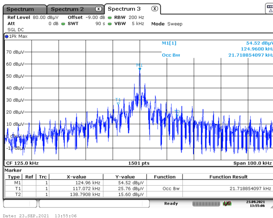
Plot 2: 99 % emission bandwidth with tag
