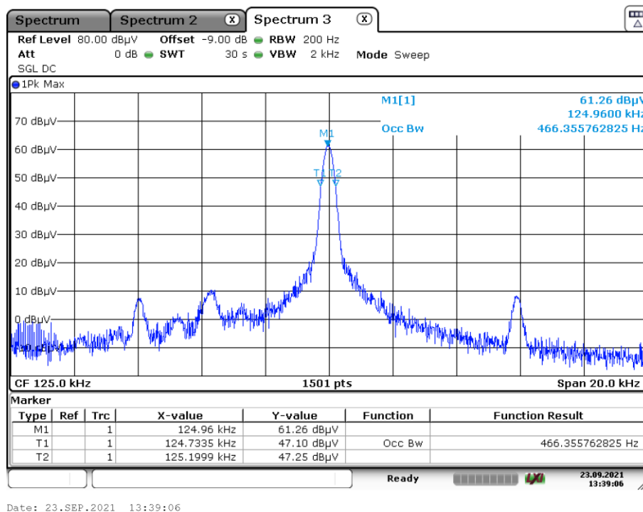
Plot 1: 99 % emission bandwidth without tag
