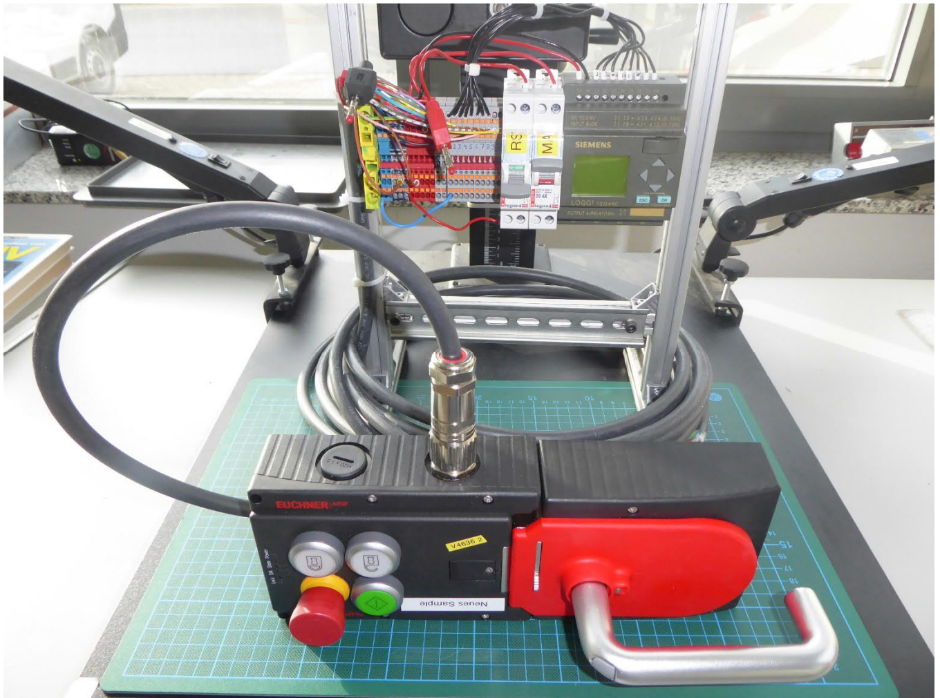
EUT with ancillary device and handle module
