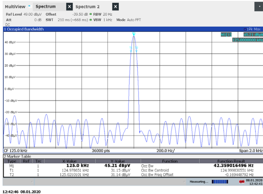
Plot 1: 99 % emission bandwidth with applied tag
