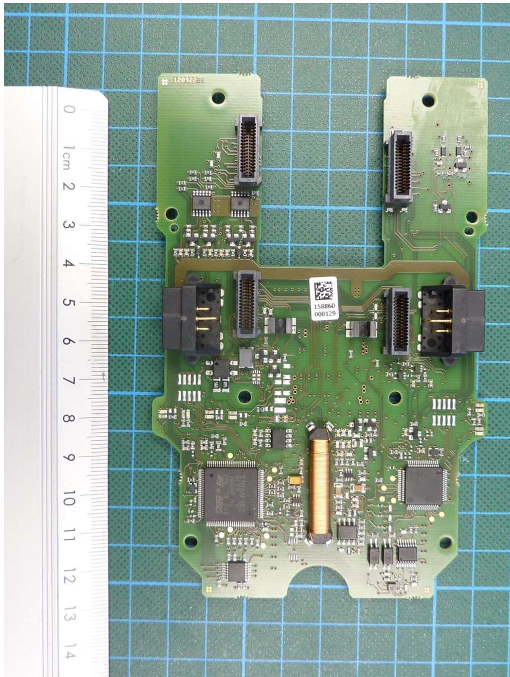
180889_9.jpg: MGB2-L2-MLI-U-Y0000-BJ-156392, PCB, top view
