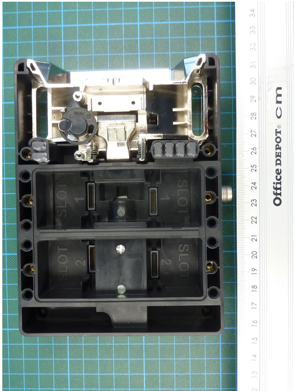
180889_5.jpg: MGB2-L2-MLI-U-Y0000-BJ-156392, internal view 1 (top covers removed)
