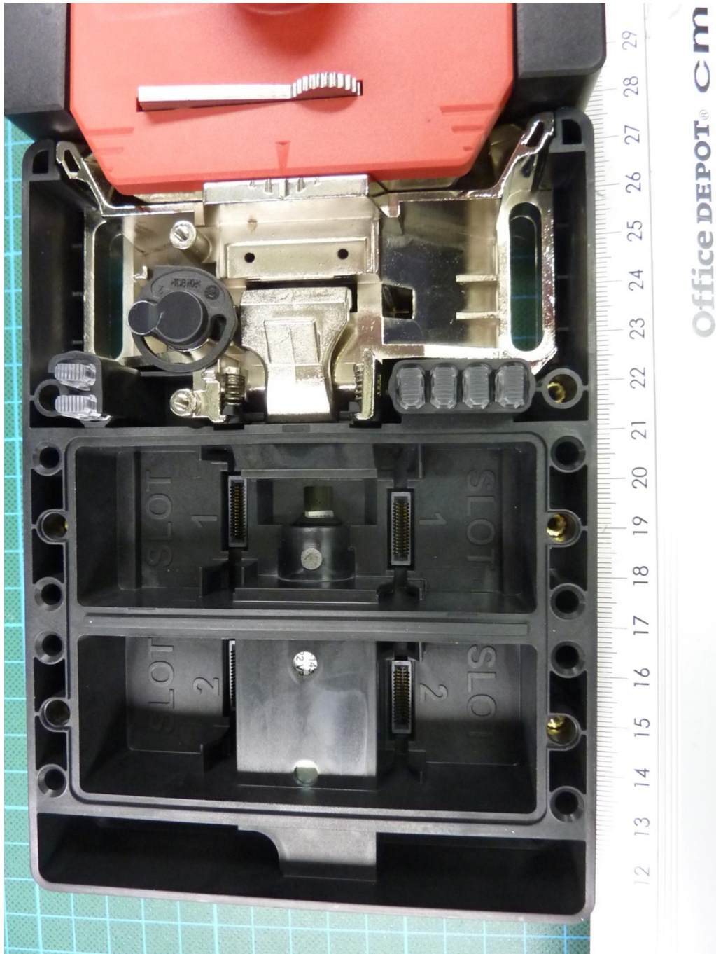
180889_23.jpg: MGB2-L2-MLI-U-Y0000-BJ-156392 with MGB2-H-BA1A3-R-136691
