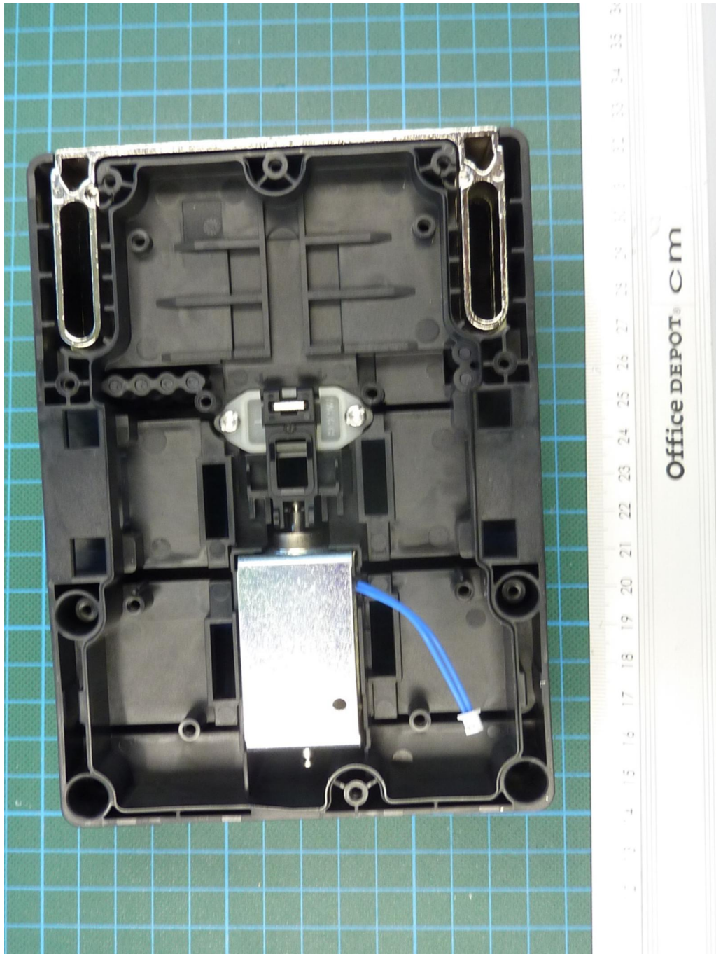
180889_4.jpg: MGB2-L2-MLI-U-Y0000-BJ-156392, internal view 3 (PCB removed)
