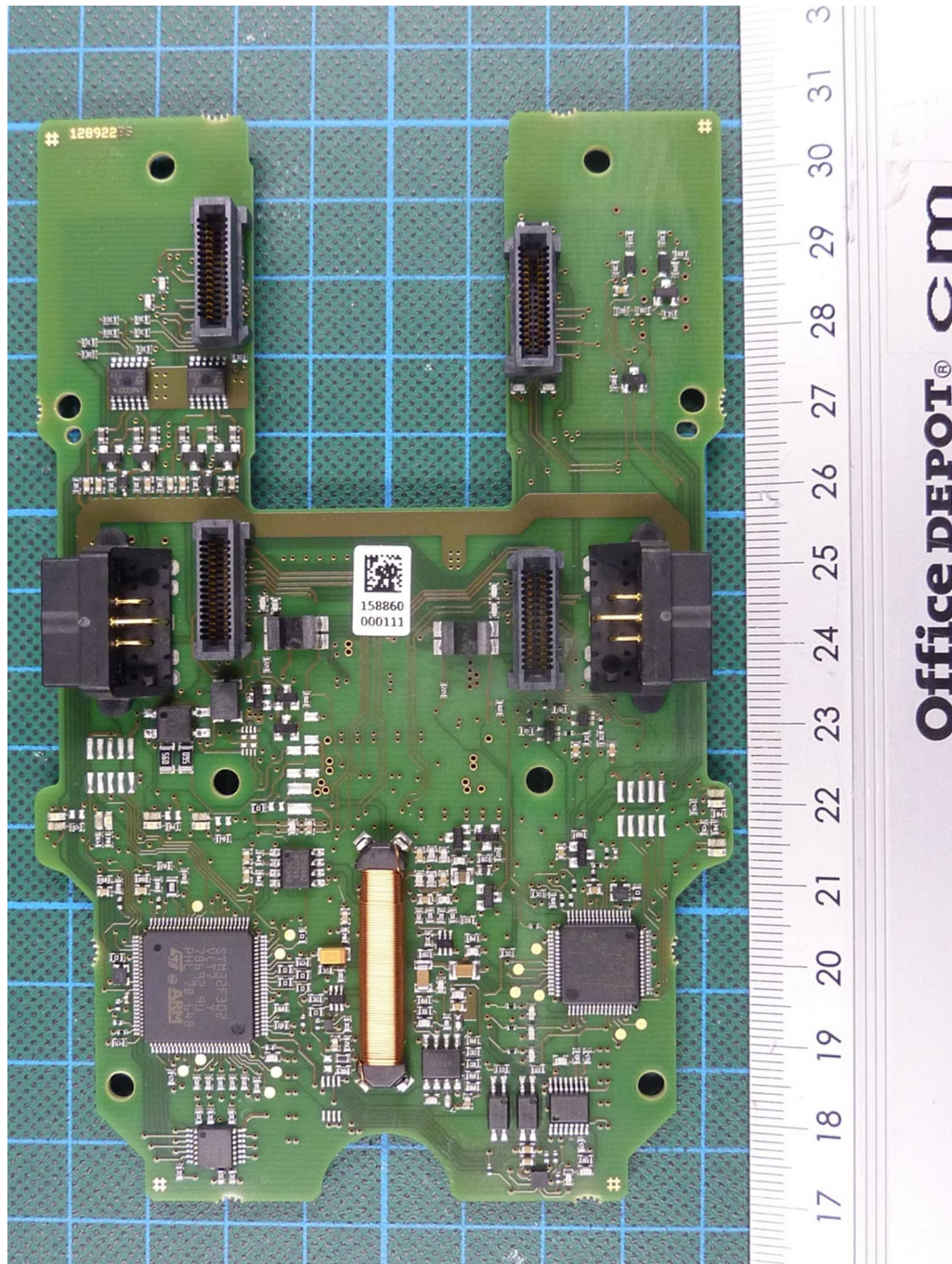
180889_21.jpg: MGB2-L1-MLI-U-Y0000-BJ-136776, PCB, top view
