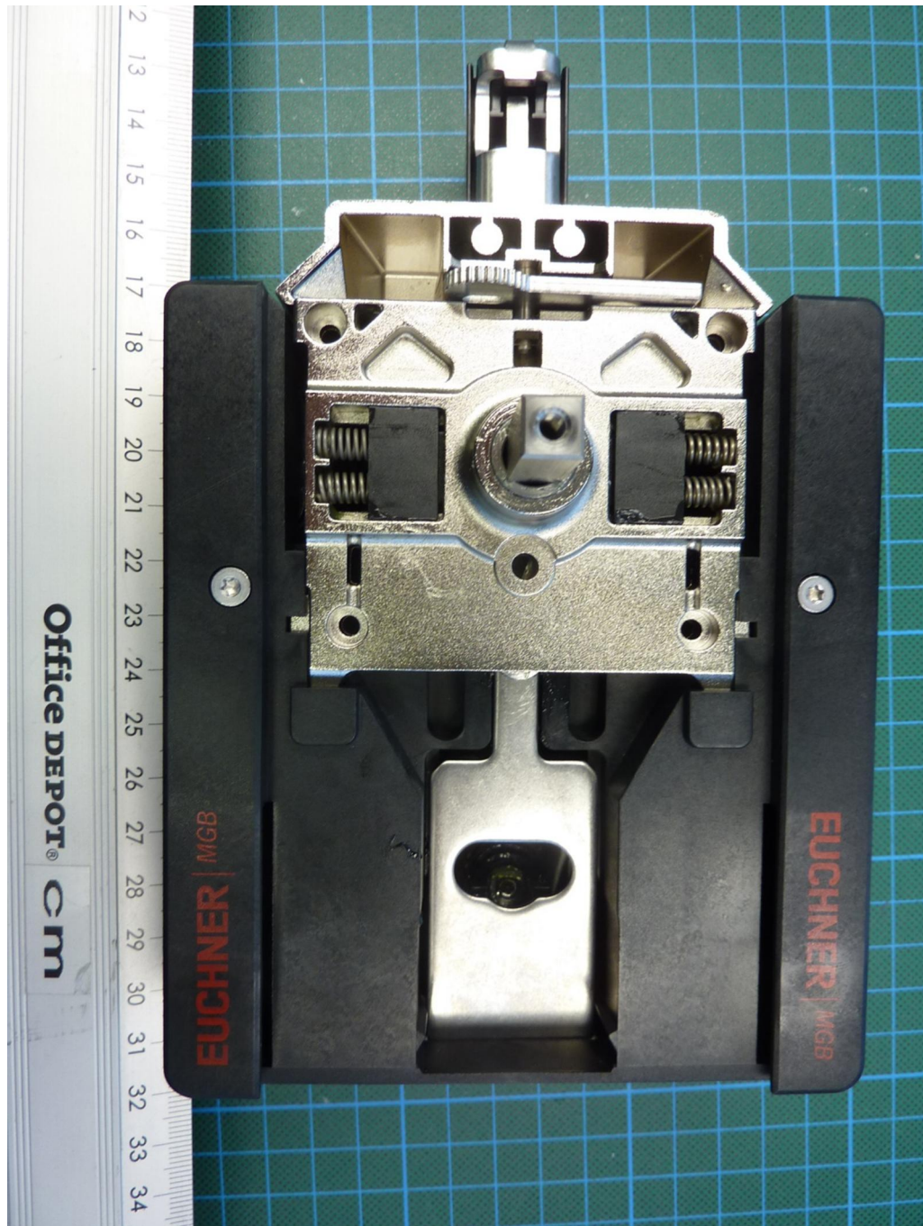
180889_13.jpg: MGB2-H-BA1A3-R-136691, internal view
