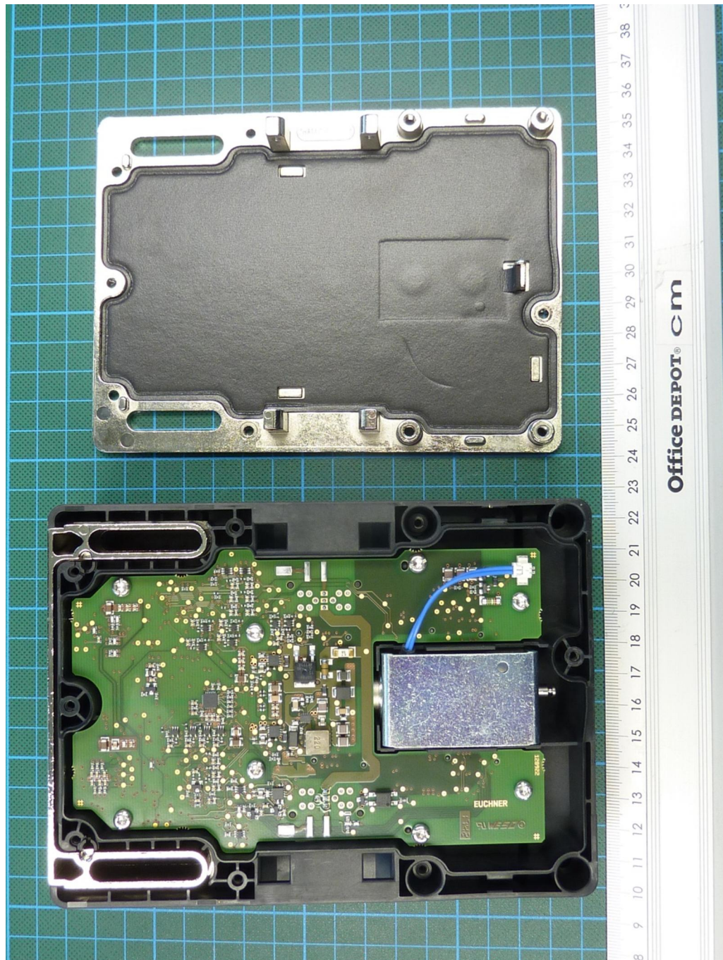
180889_6.jpg: MGB2-L2-MLI-U-Y0000-BJ-156392, internal view 2 (bottom cover removed)
