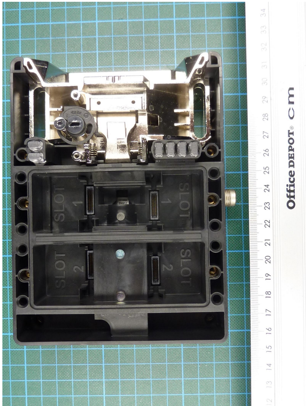
180889_18.jpg: MGB2-L1-MLI-U-Y0000-BJ-136776, internal view 1 (top covers removed)
