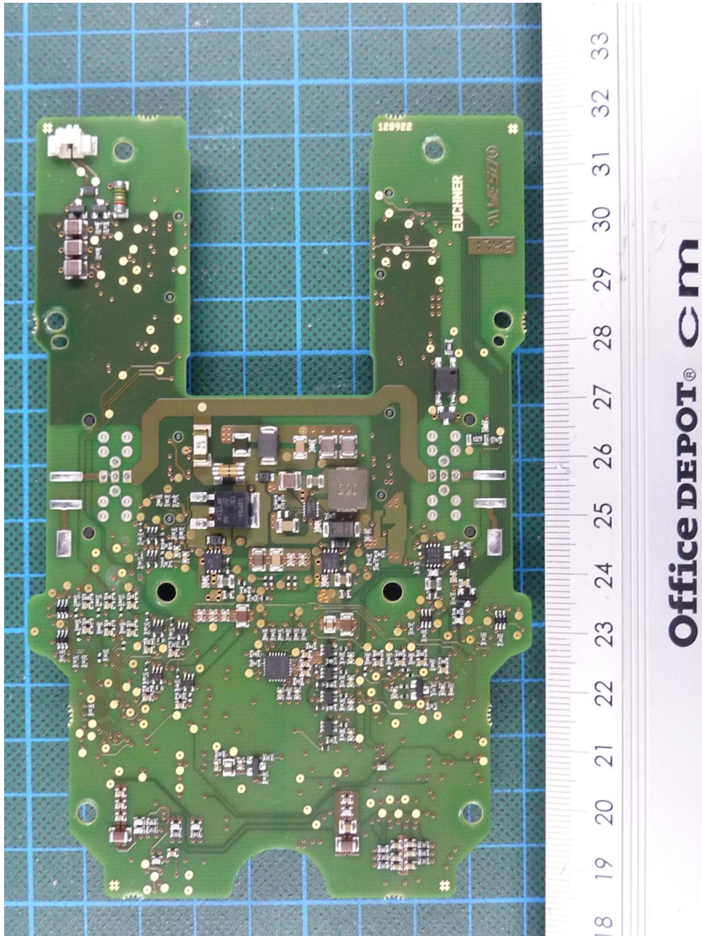
180889_22.jpg: MGB2-L1-MLI-U-Y0000-BJ-136776, PCB, bottom view
