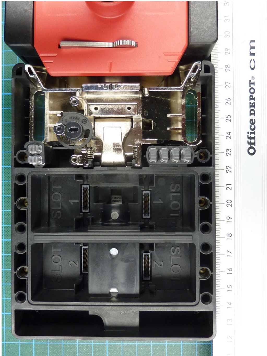
180889_24.jpg: MGB2-L1-MLI-U-Y0000-BJ-136776 with MGB2-H-BA1A3-R-136691
