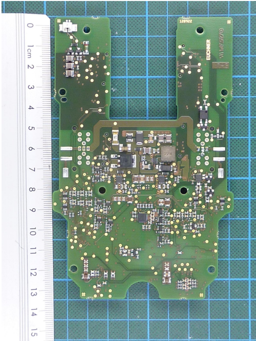
180889_10.jpg: MGB2-L2-MLI-U-Y0000-BJ-156392, PCB, bottom view
