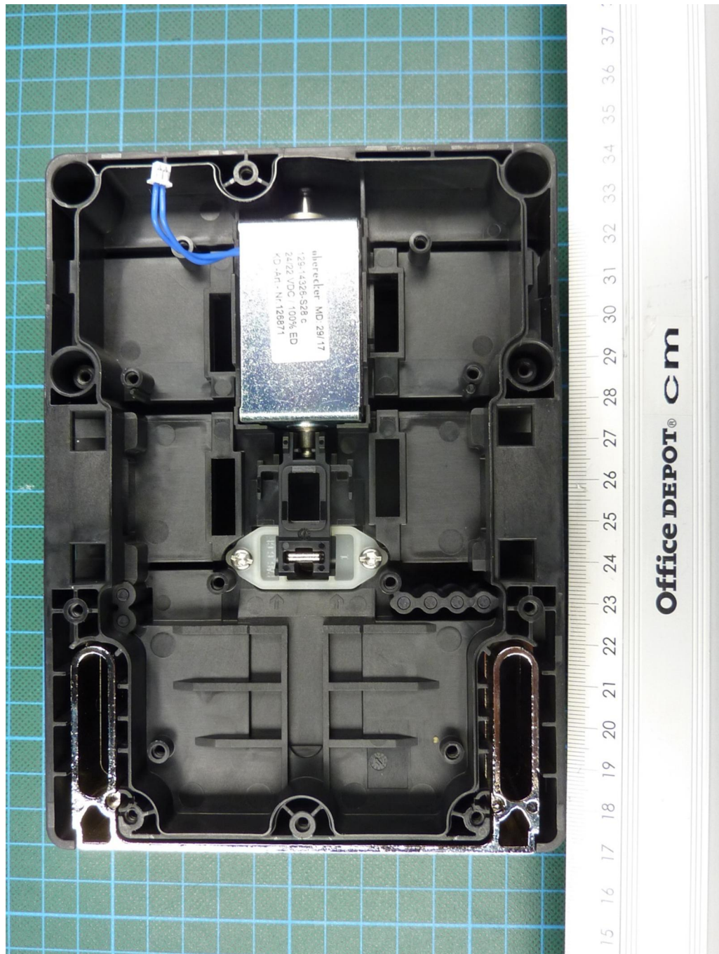
180889_20.jpg: MGB2-L1-MLI-U-Y0000-BJ-136776, internal view 3 (PCB removed)
