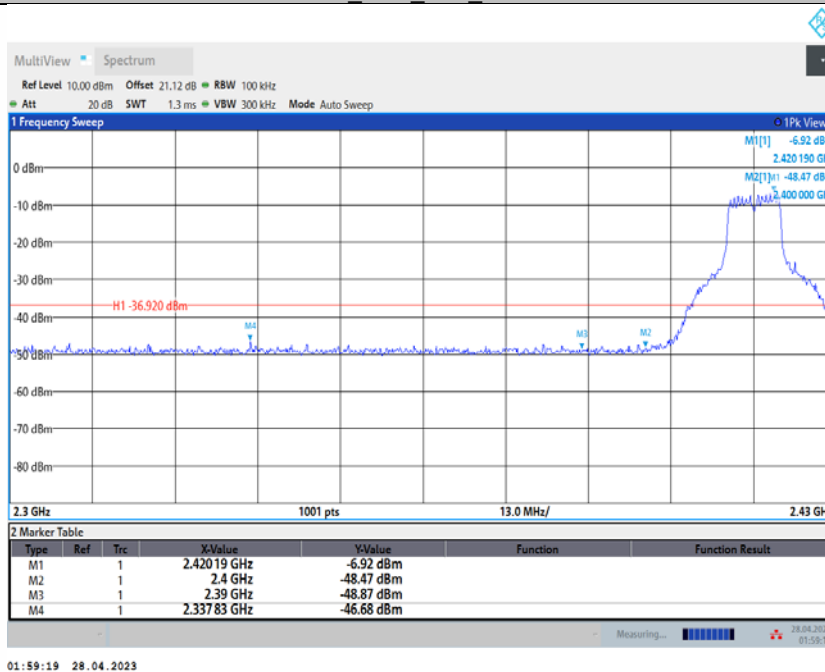
11N20SISO_Ant1_Low_2417
