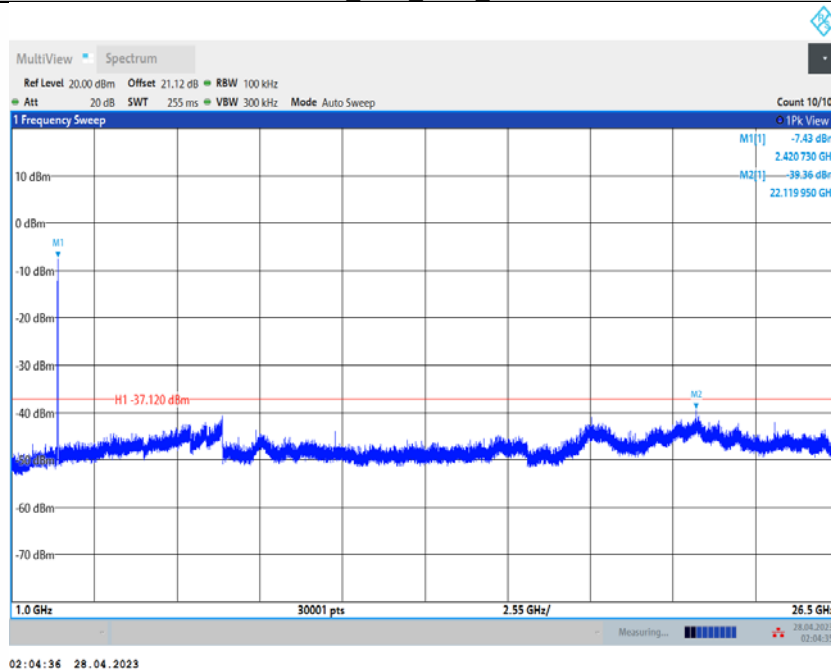
11N20SISO_Ant2_2417_1000~26500
