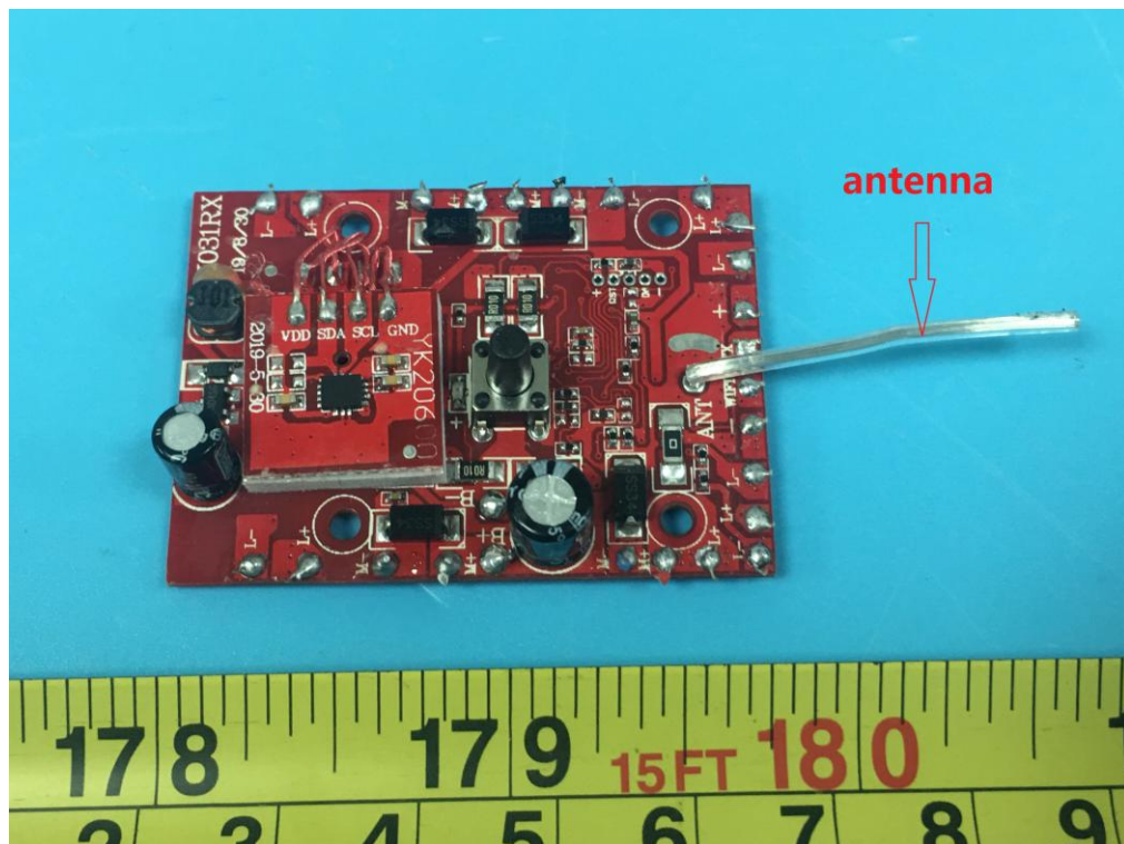
2.4G RX Antenna
