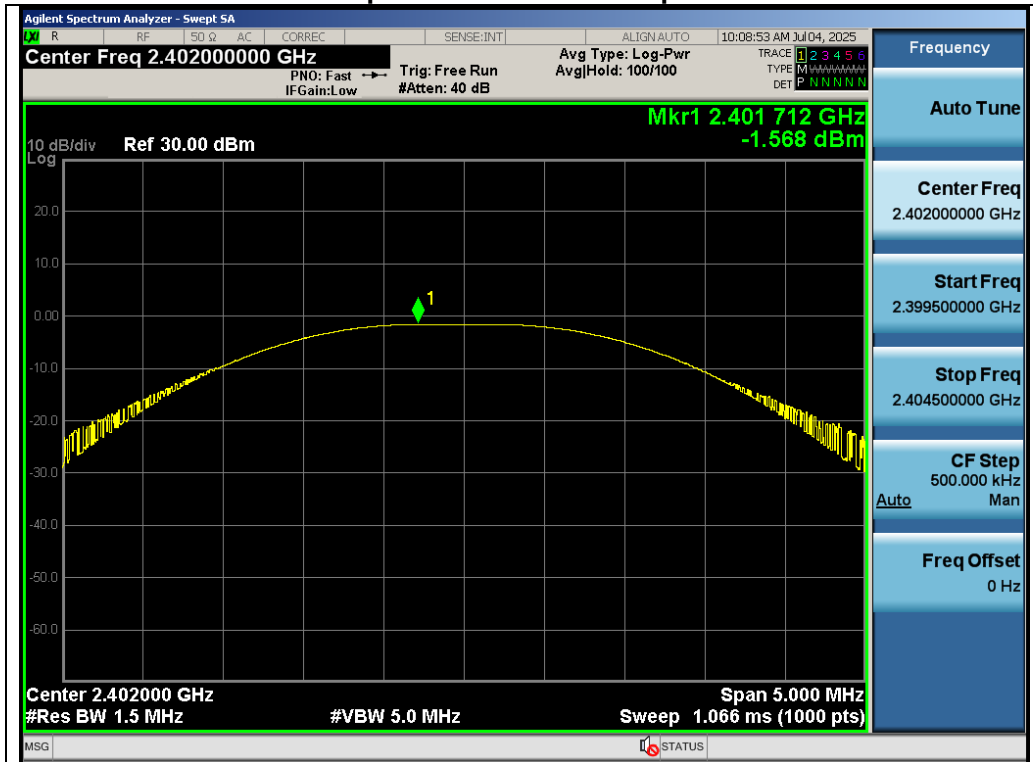
Test_Graph_LE1M_ANT1_2402_1Mbps_Peak Power
