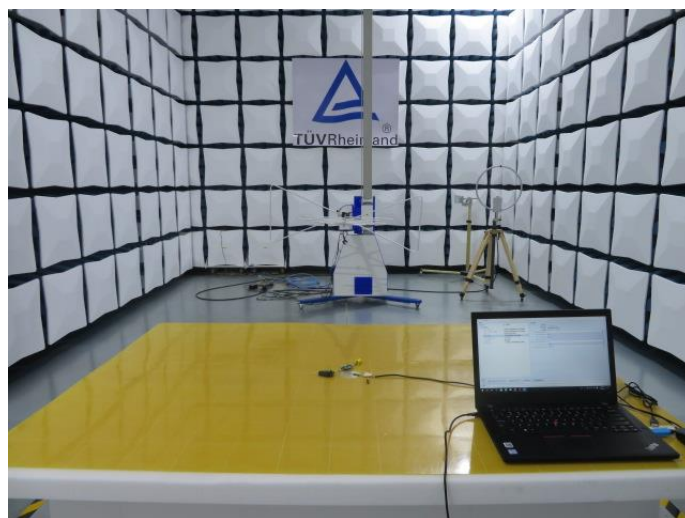
Photograph 4: Set-up for Radiated Spurious Emission, 30MHz - 1GHz
