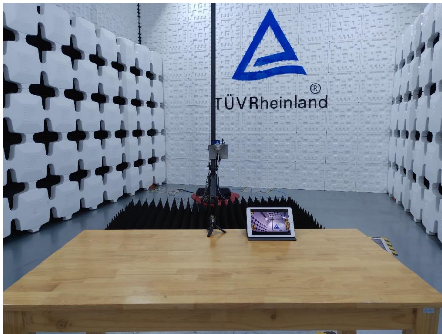
Photograph 4: Set-up for Radiated Spurious Emission, 30MHz - 1GHz
